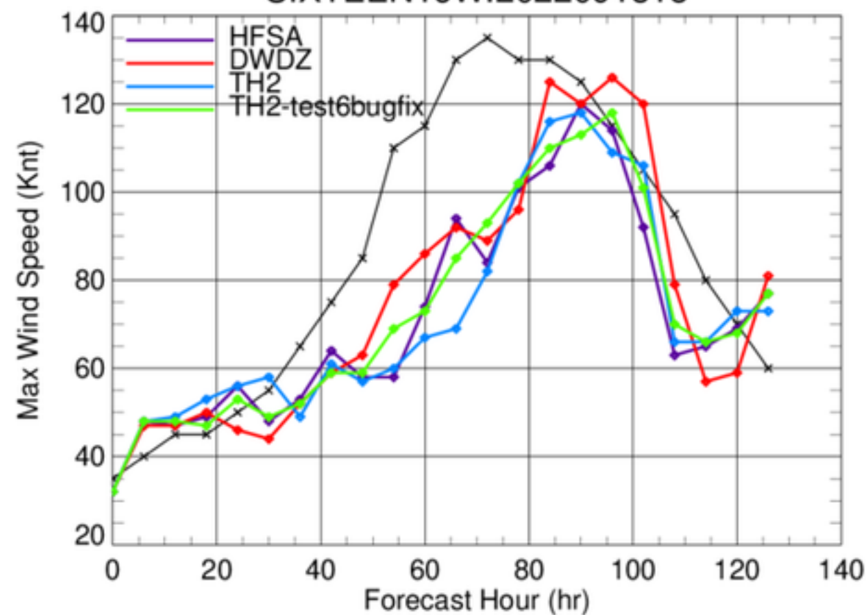
SIXTEEN16W.2022091318
