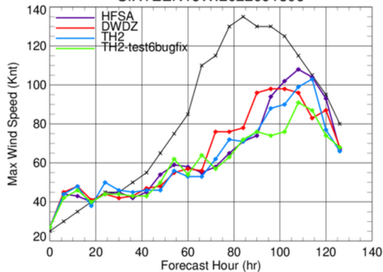
SIXTEEN16W.2022091306
