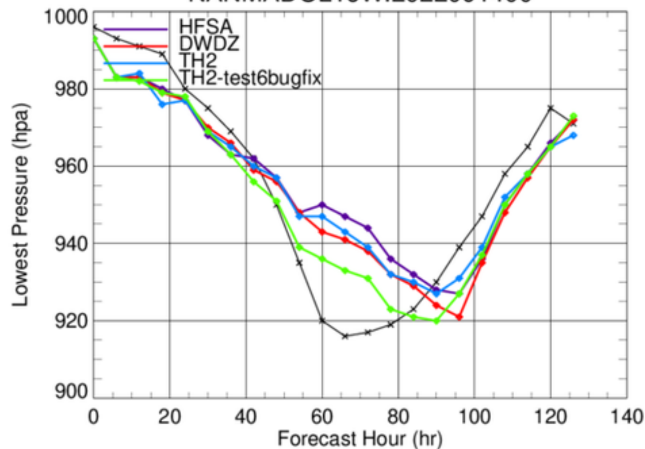
NANMADOL16W.2022091400
