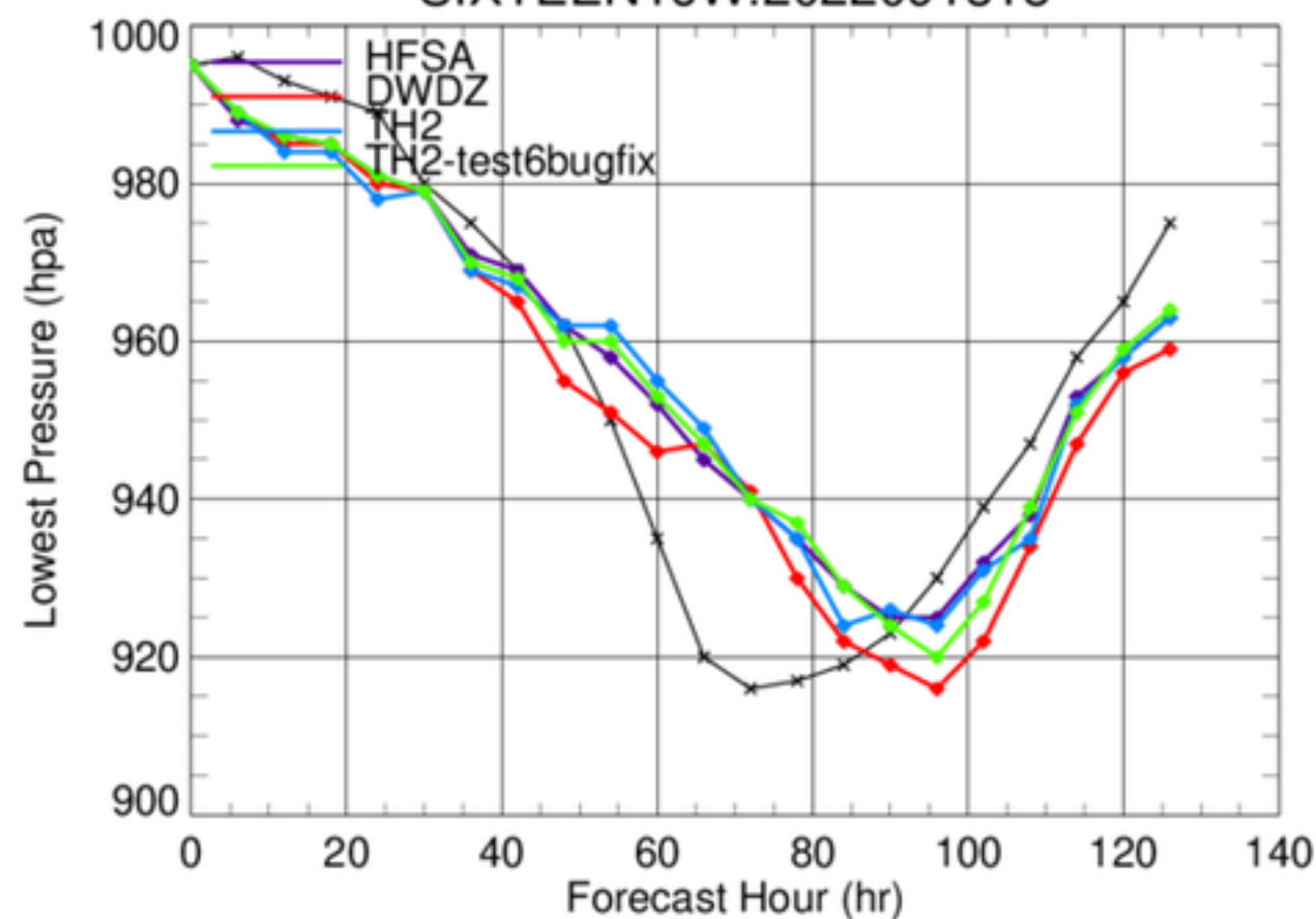
SIXTEEN16W.2022091318
