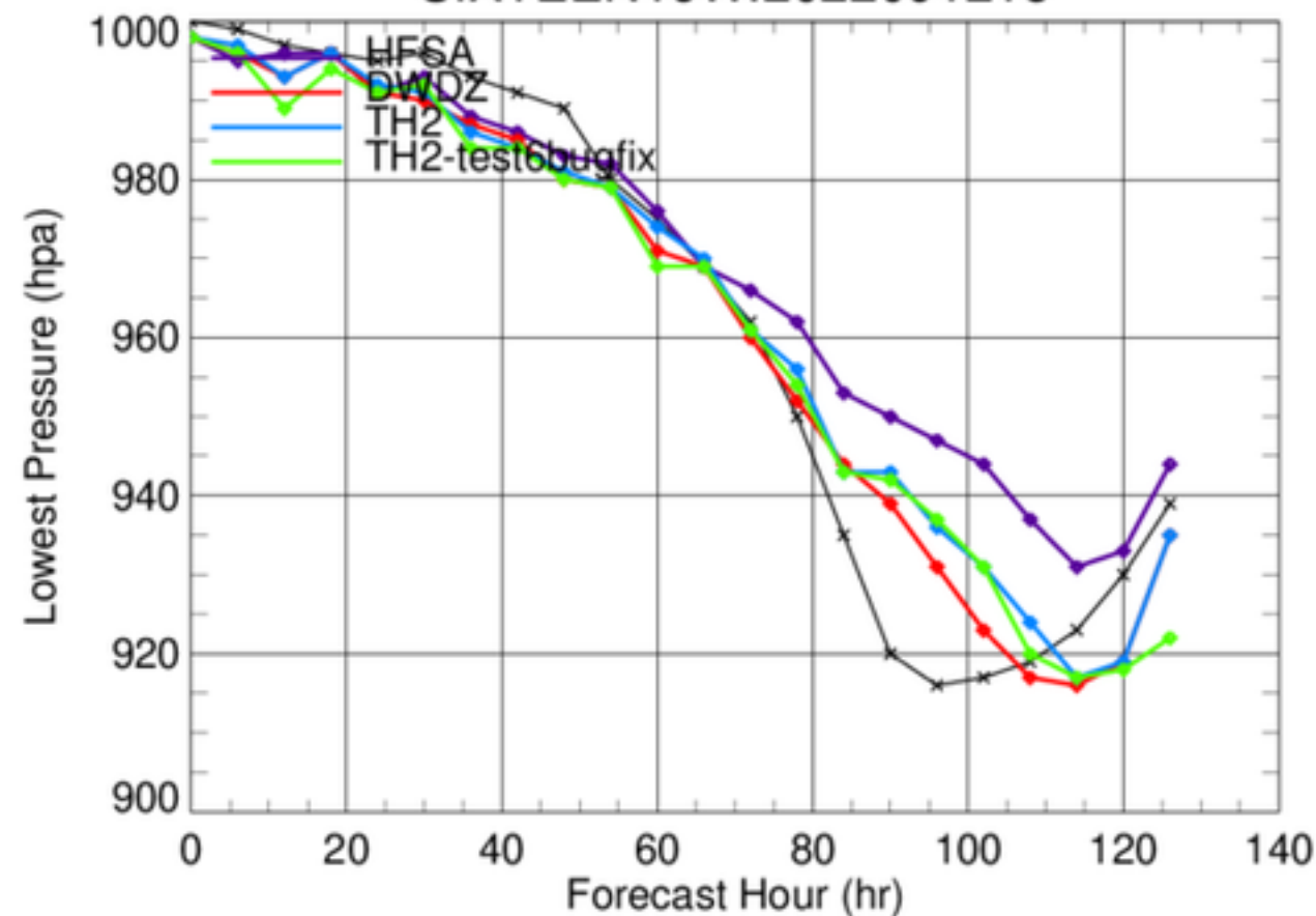
SIXTEEN16W.2022091218
