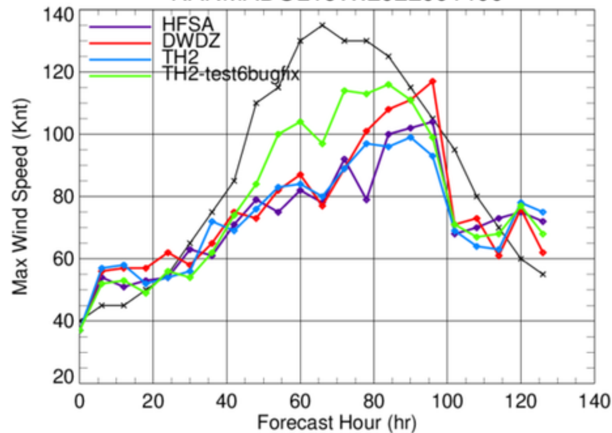
NANMADOL16W.2022091400
