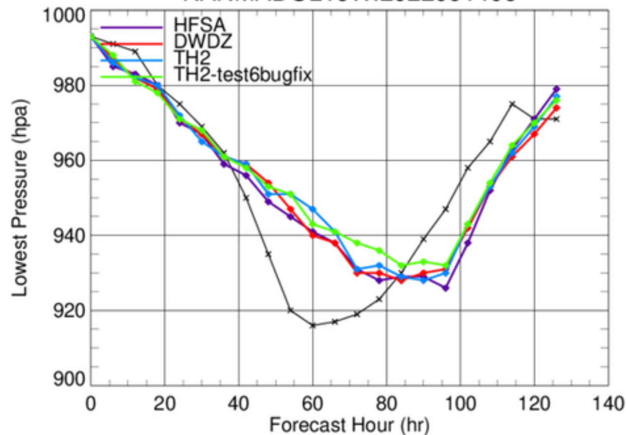
NANMADOL16W.2022091406
