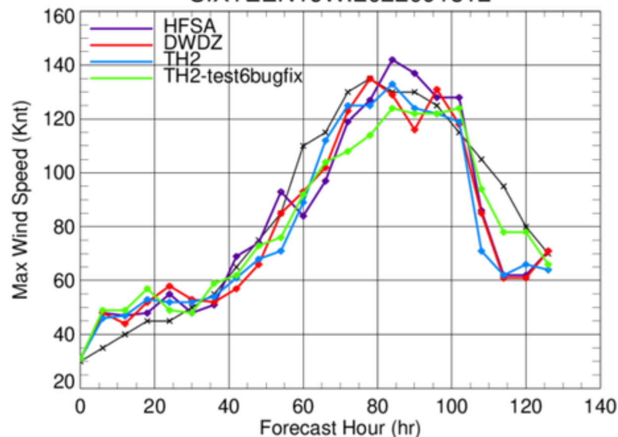
SIXTEEN16W.2022091312
