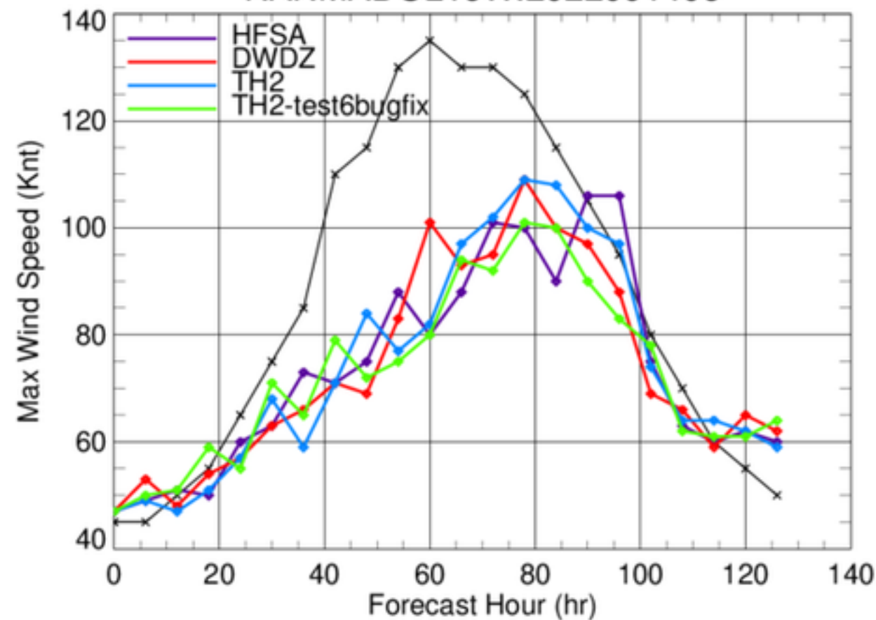
NANMADOL16W.2022091406
