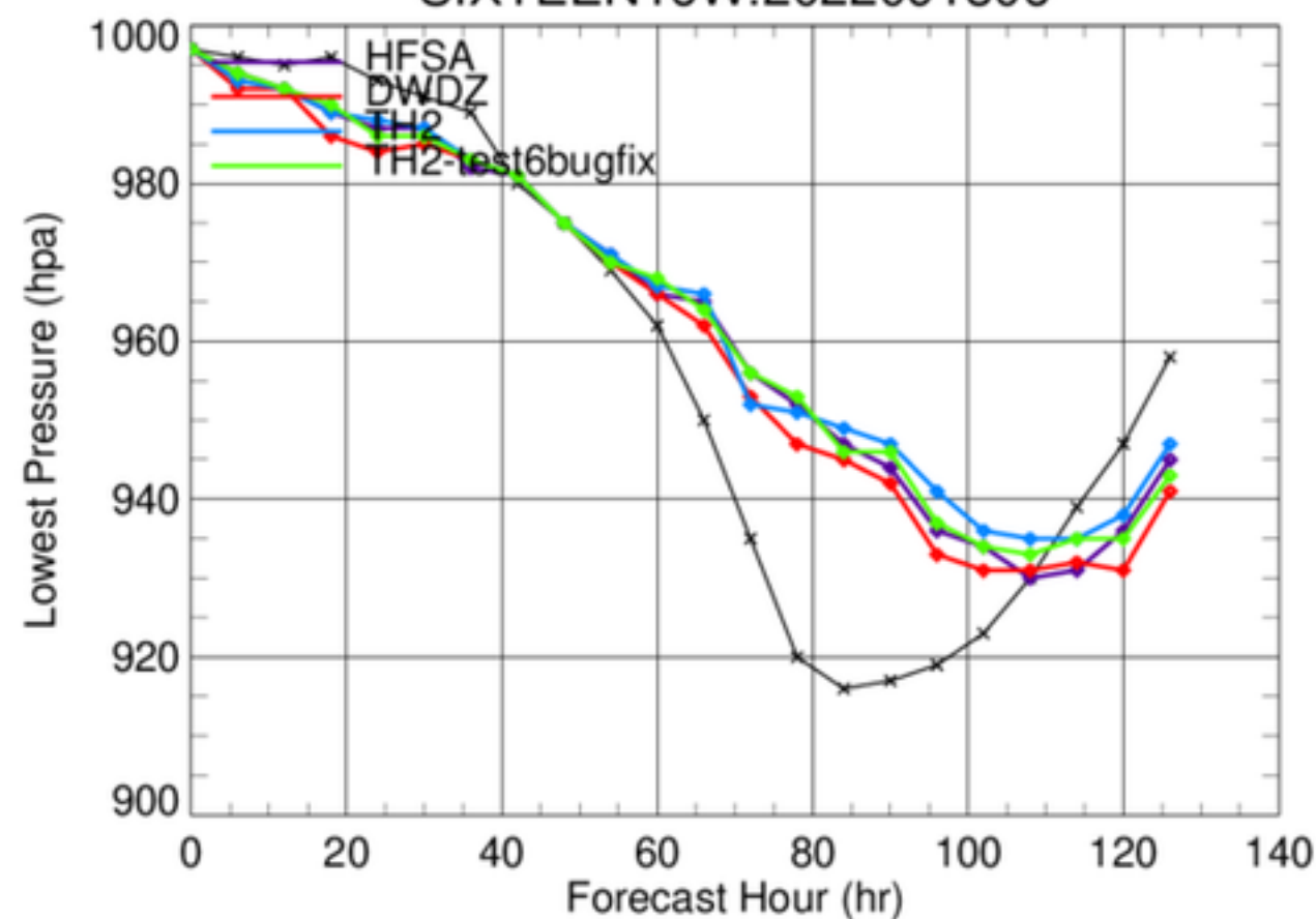
SIXTEEN16W.2022091306
