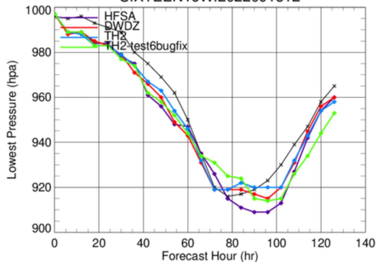
SIXTEEN16W.2022091312
