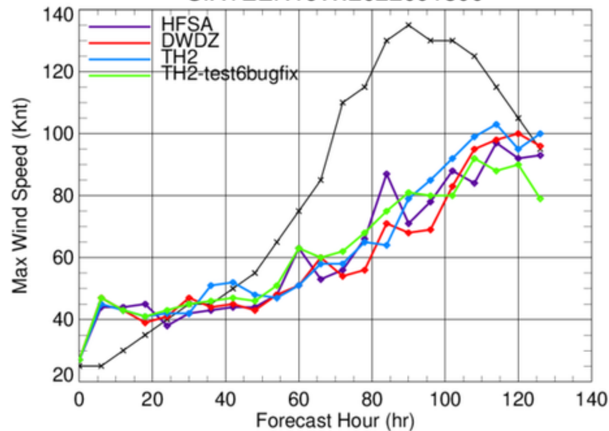
SIXTEEN16W.2022091300
