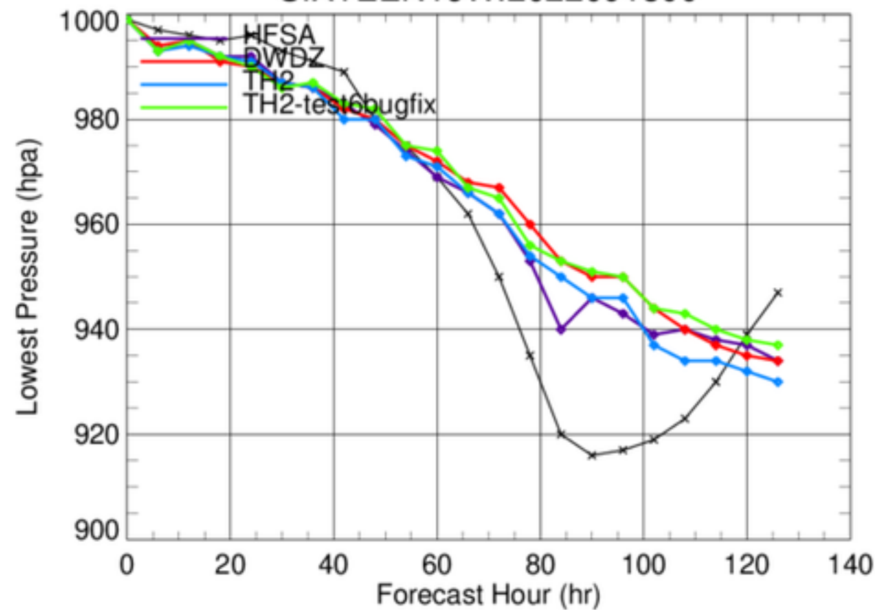
SIXTEEN16W.2022091300
