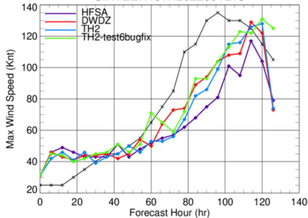
SIXTEEN16W.2022091218
