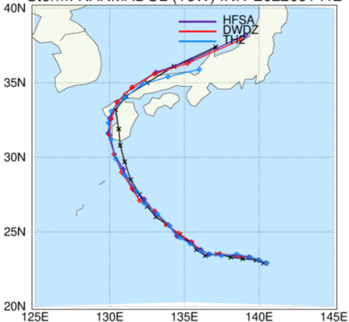
HAFS: TC Tracks Storm: NANMADOL (16W) INIT 2022091412
