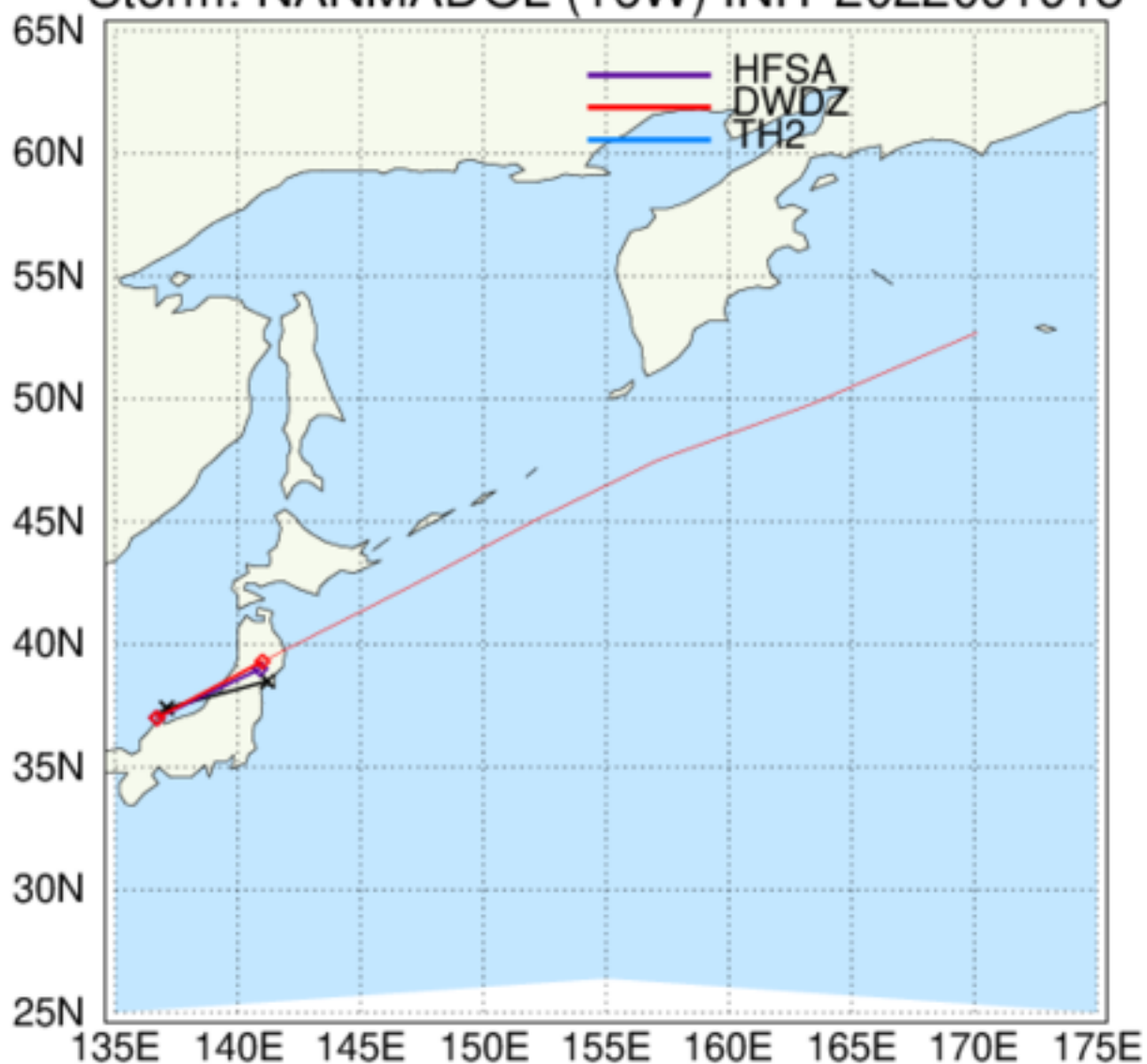
HAFS: TC Tracks Storm: NANMADOL (16W) INIT 2022091918
