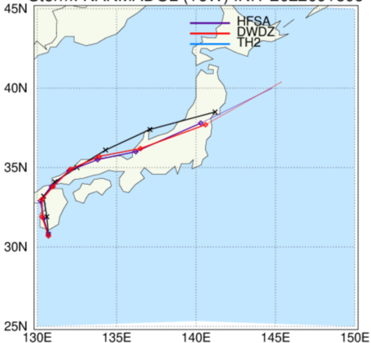
HAFS: TC Tracks Storm: NANMADOL (16W) INIT 2022091806
