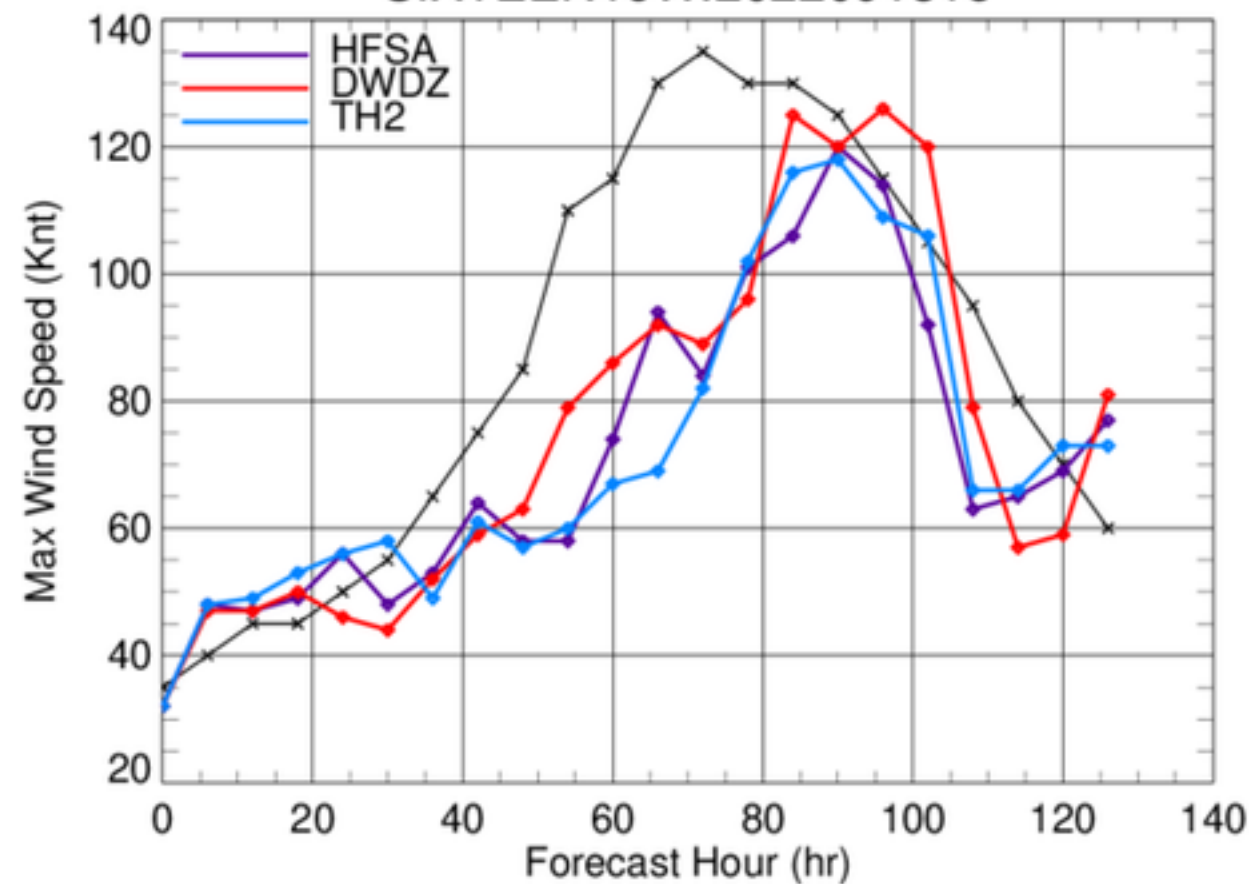
SIXTEEN16W.2022091318
