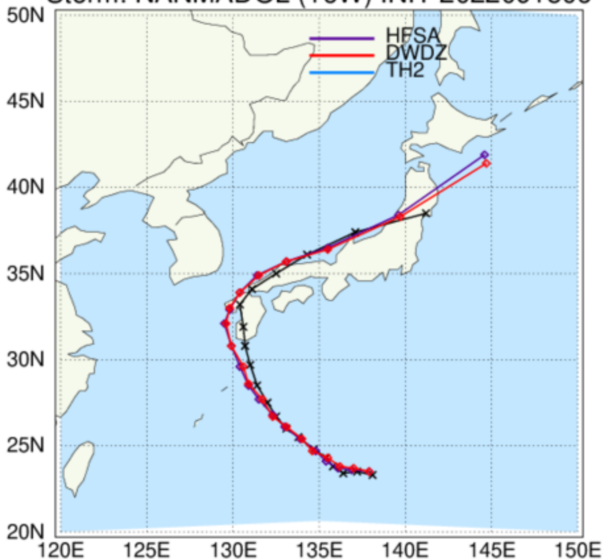
HAFS: TC Tracks Storm: NANMADOL (16W) INIT 2022091506
