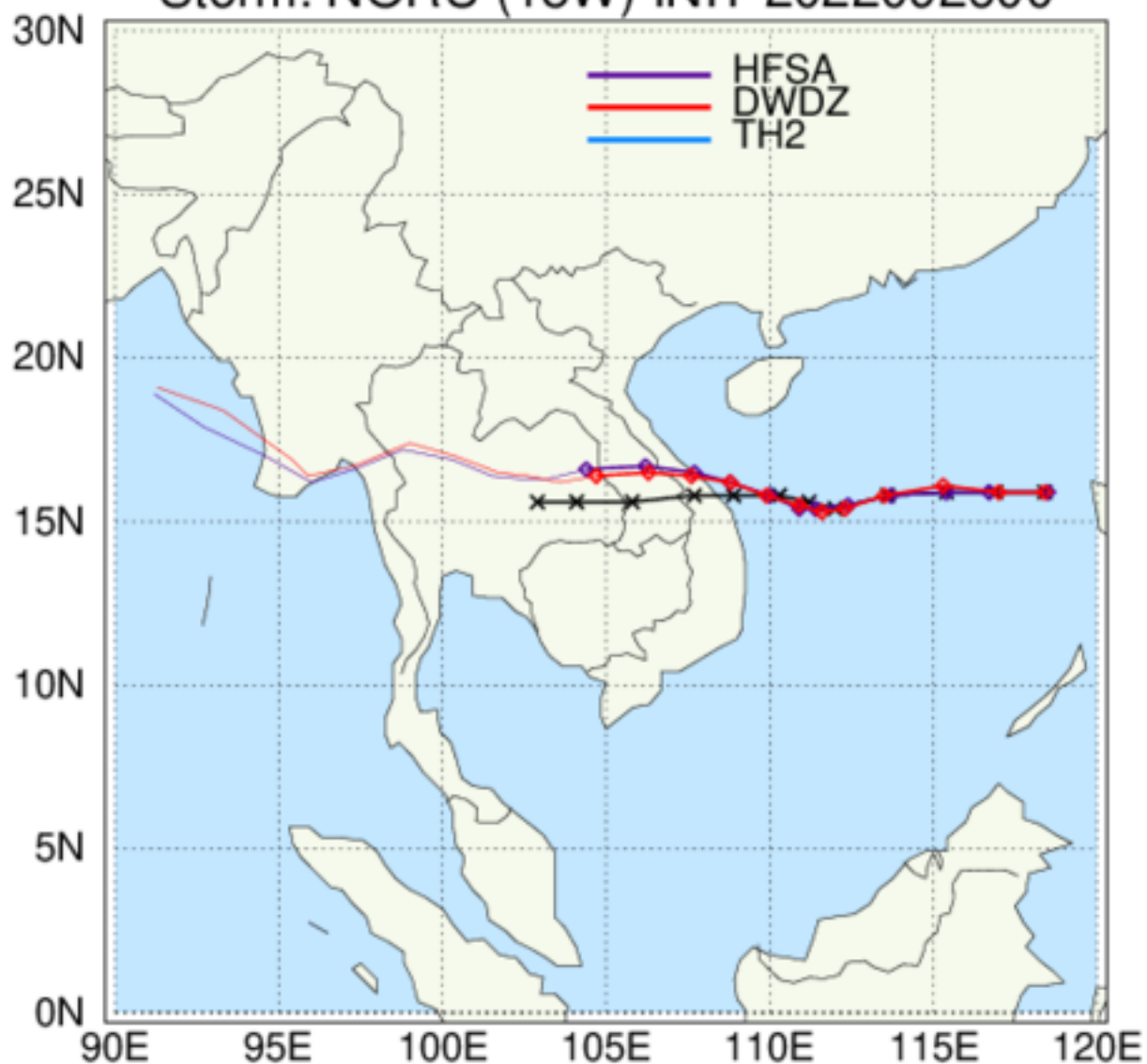
HAFS: TC Tracks Storm: NORU (18W) INIT 2022092600
