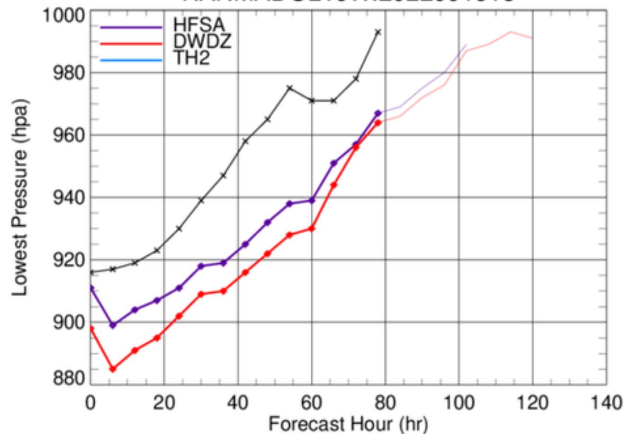
NANMADOL16W.2022091618
