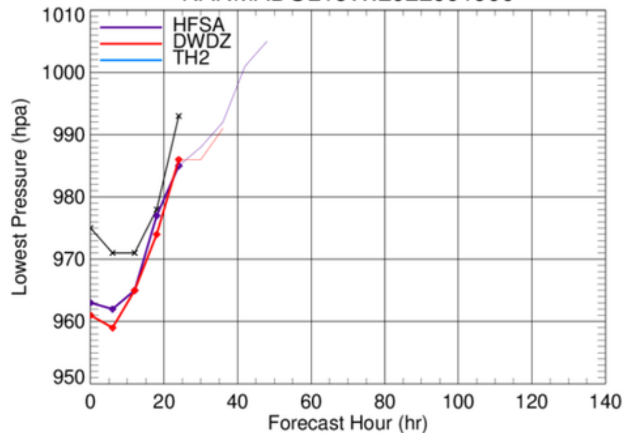
NANMADOL16W.2022091900
