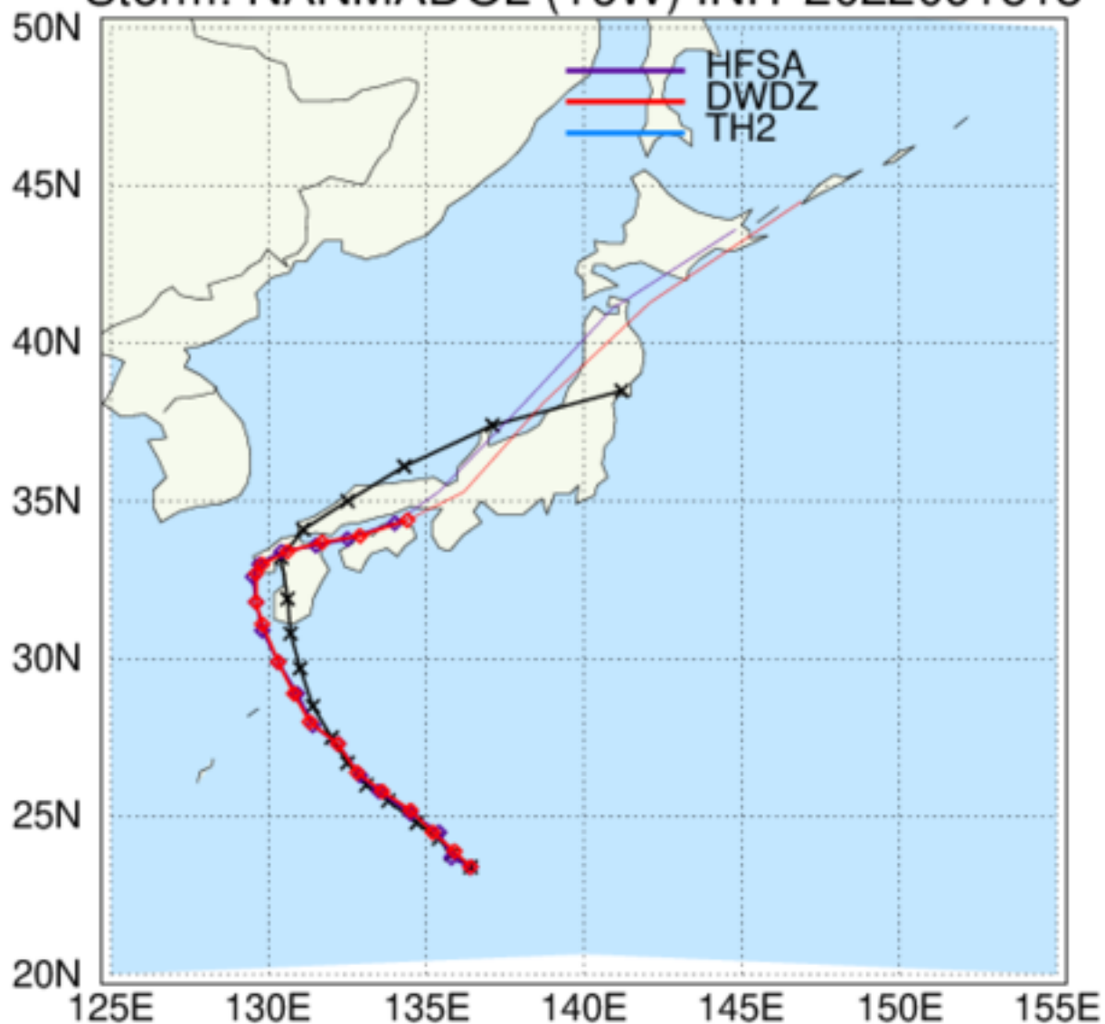
HAFS: TC Tracks Storm: NANMADOL (16W) INIT 2022091518
