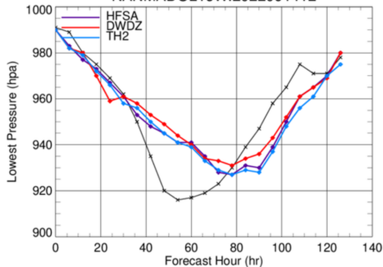
NANMADOL16W.2022091412
