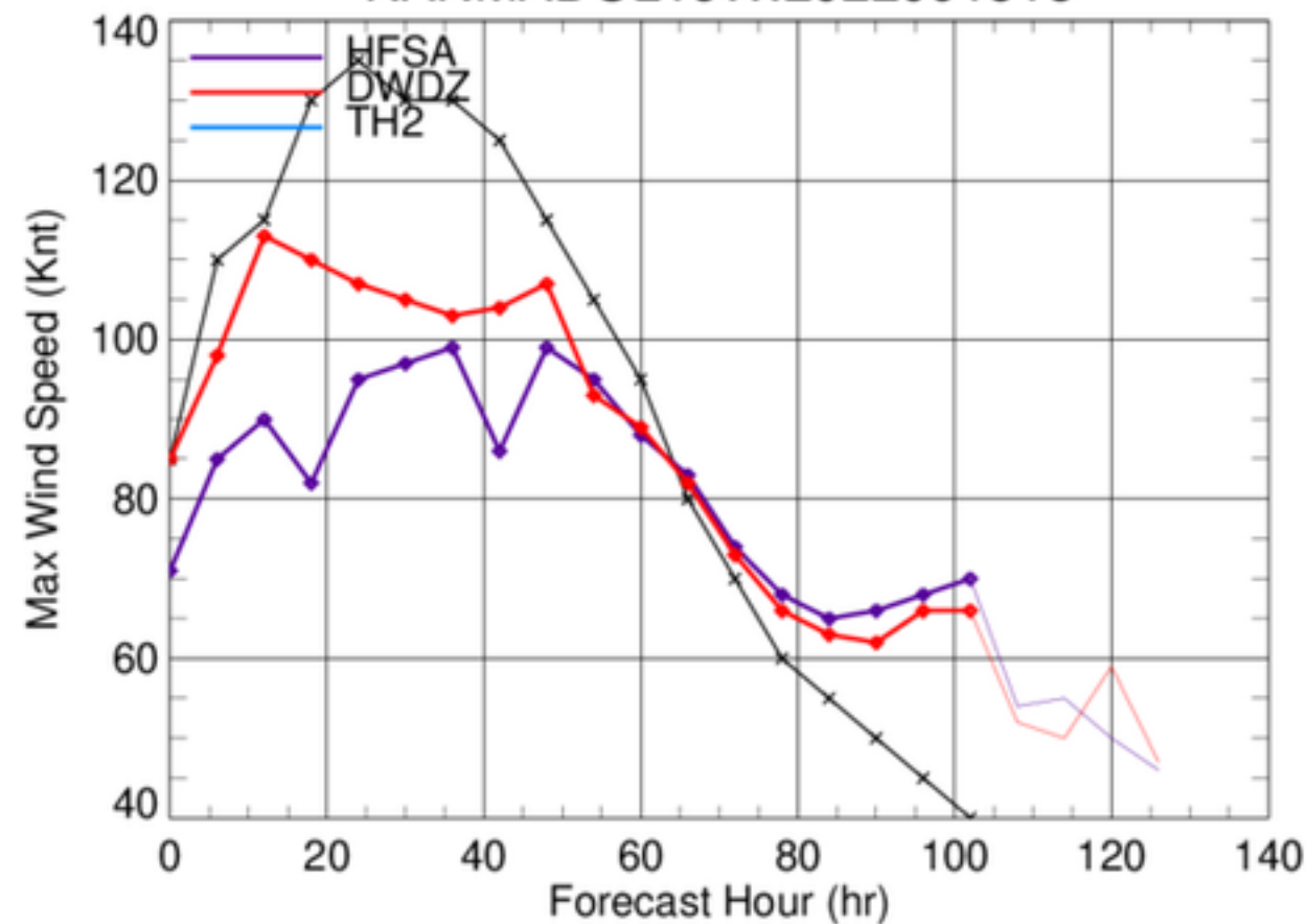
NANMADOL16W.2022091518
