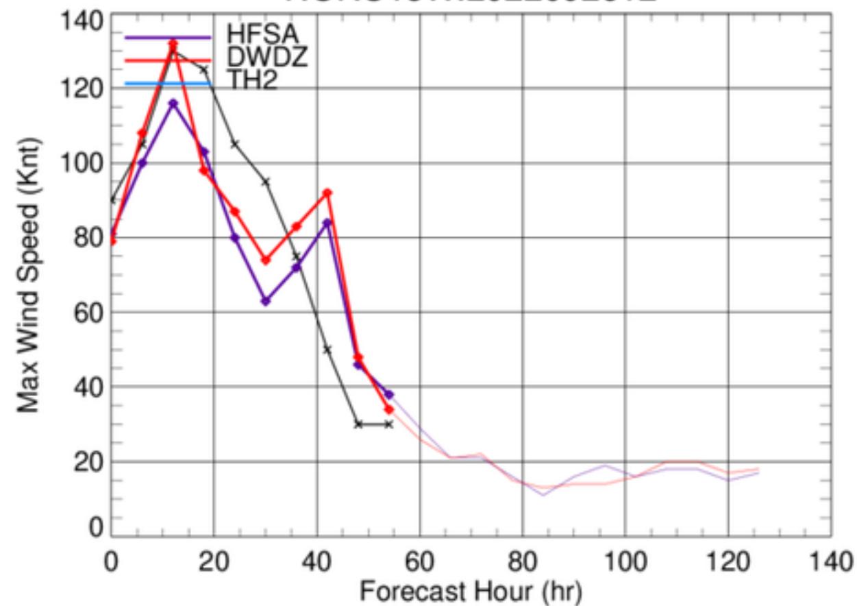
NORU18W.2022092612
