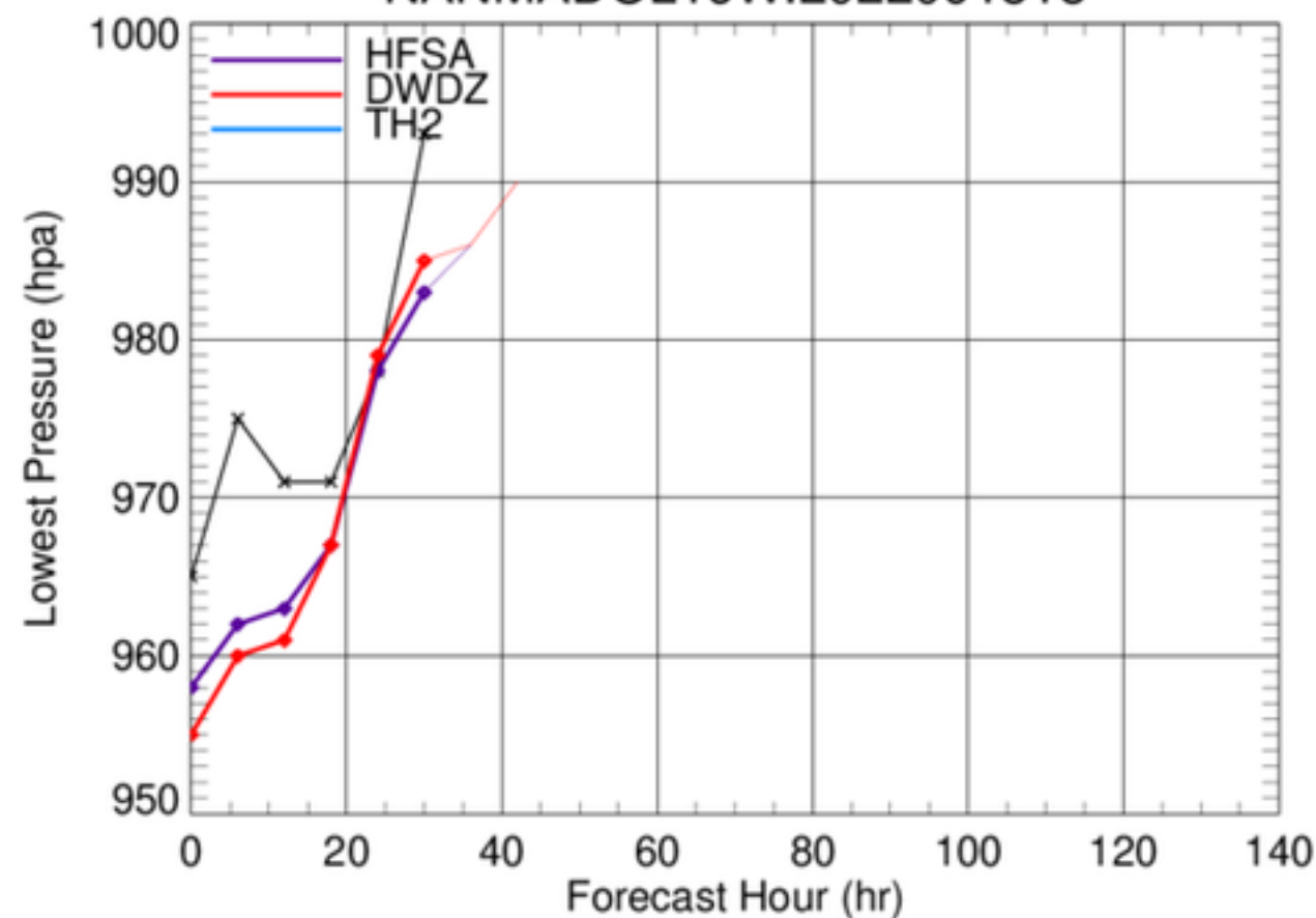
NANMADOL16W.2022091818
