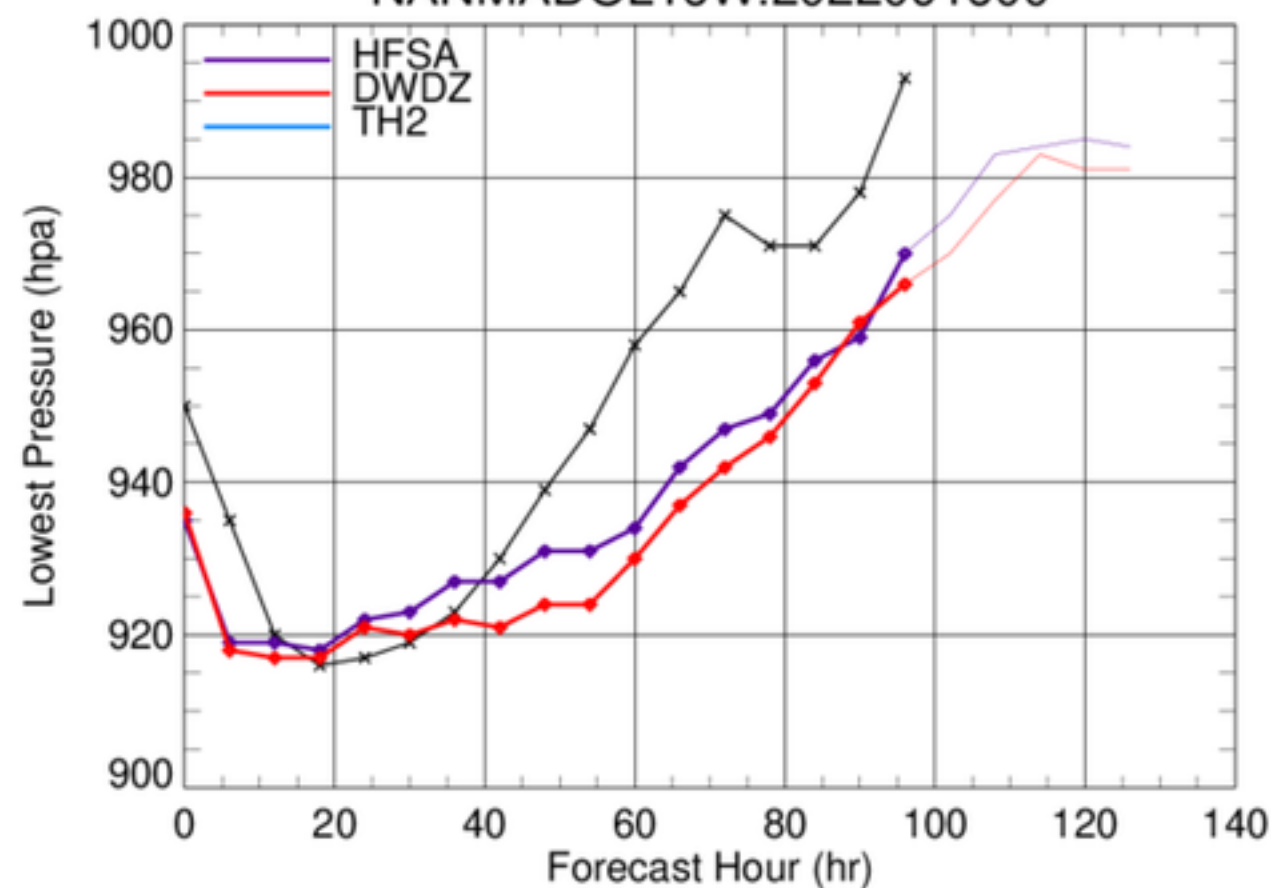
NANMADOL16W.2022091600
