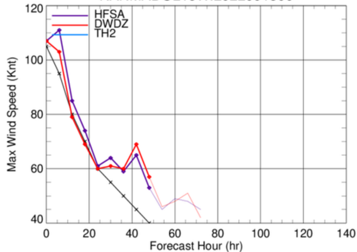
NANMADOL16W.2022091800
