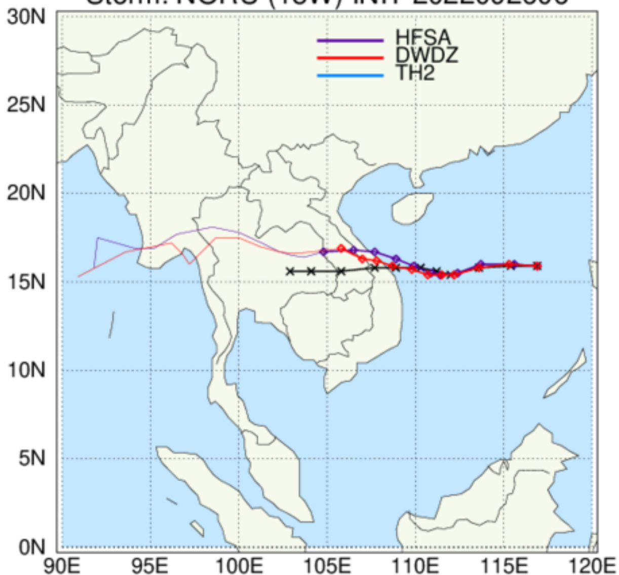
HAFS: TC Tracks Storm: NORU (18W) INIT 2022092606
