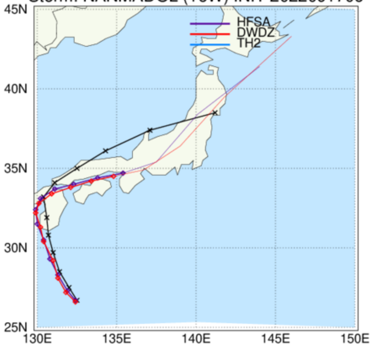
HAFS: TC Tracks Storm: NANMADOL (16W) INIT 2022091706
