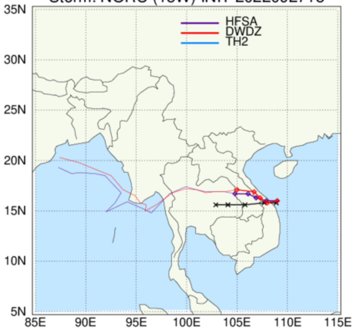
HAFS: TC Tracks Storm: NORU (18W) INIT 2022092718
