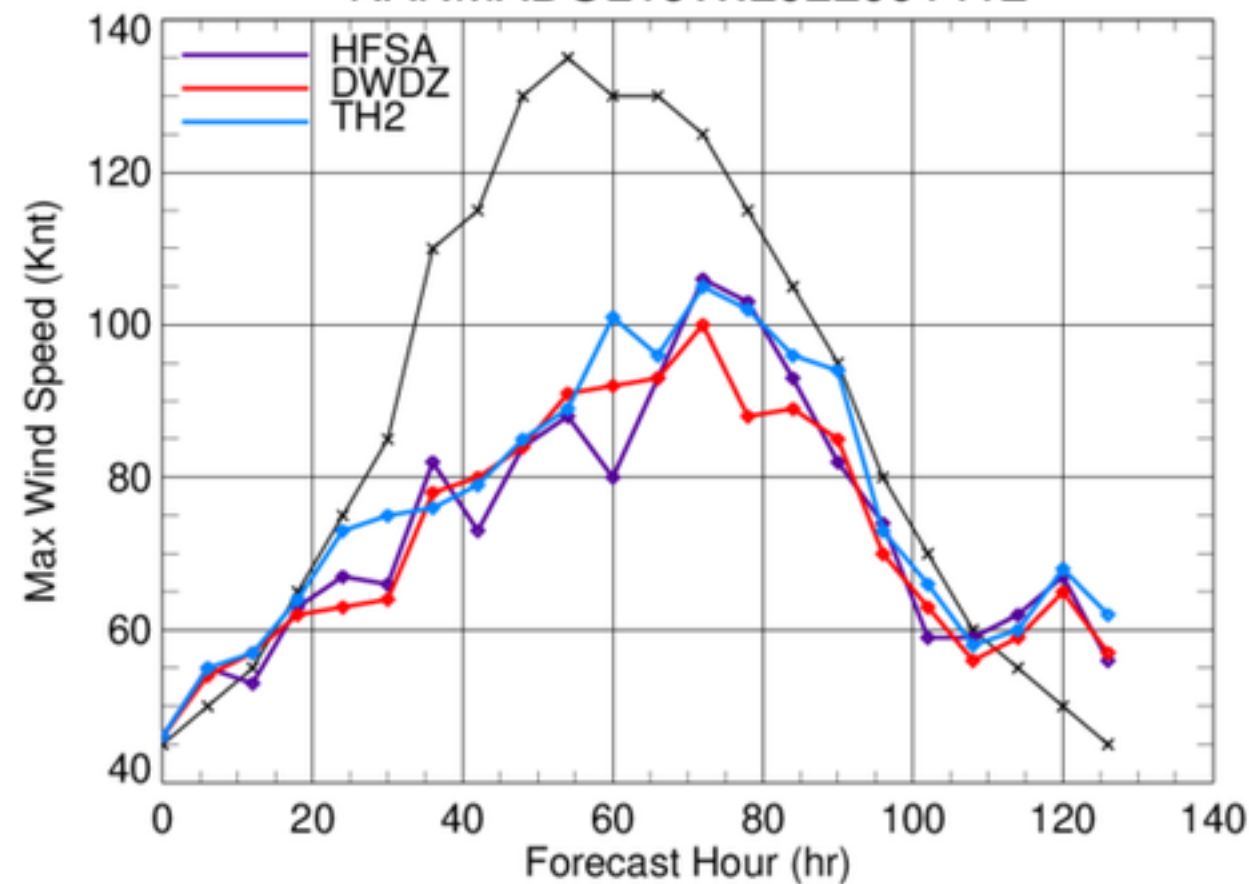
NANMADOL16W.2022091412
