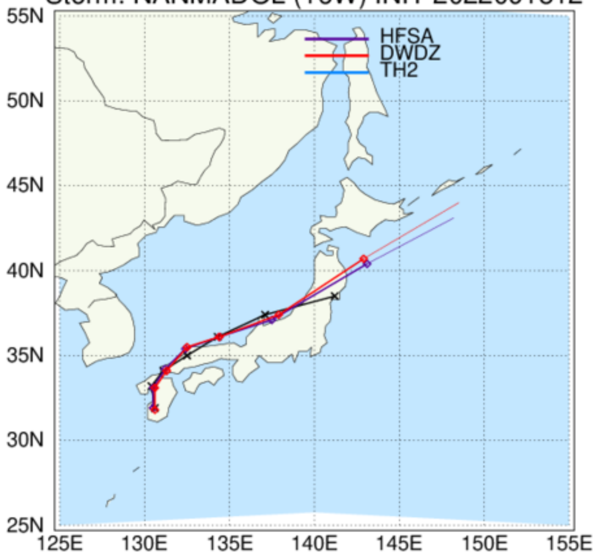
HAFS: TC Tracks Storm: NANMADOL (16W) INIT 2022091812
