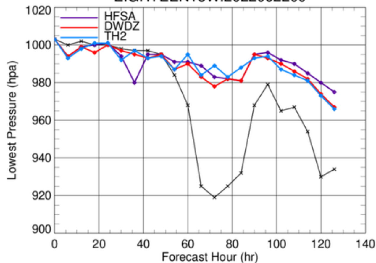
EIGHTEEN18W.2022092200
