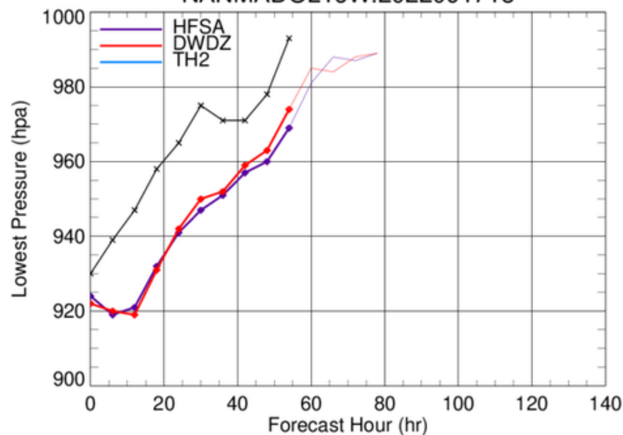
NANMADOL16W.2022091718
