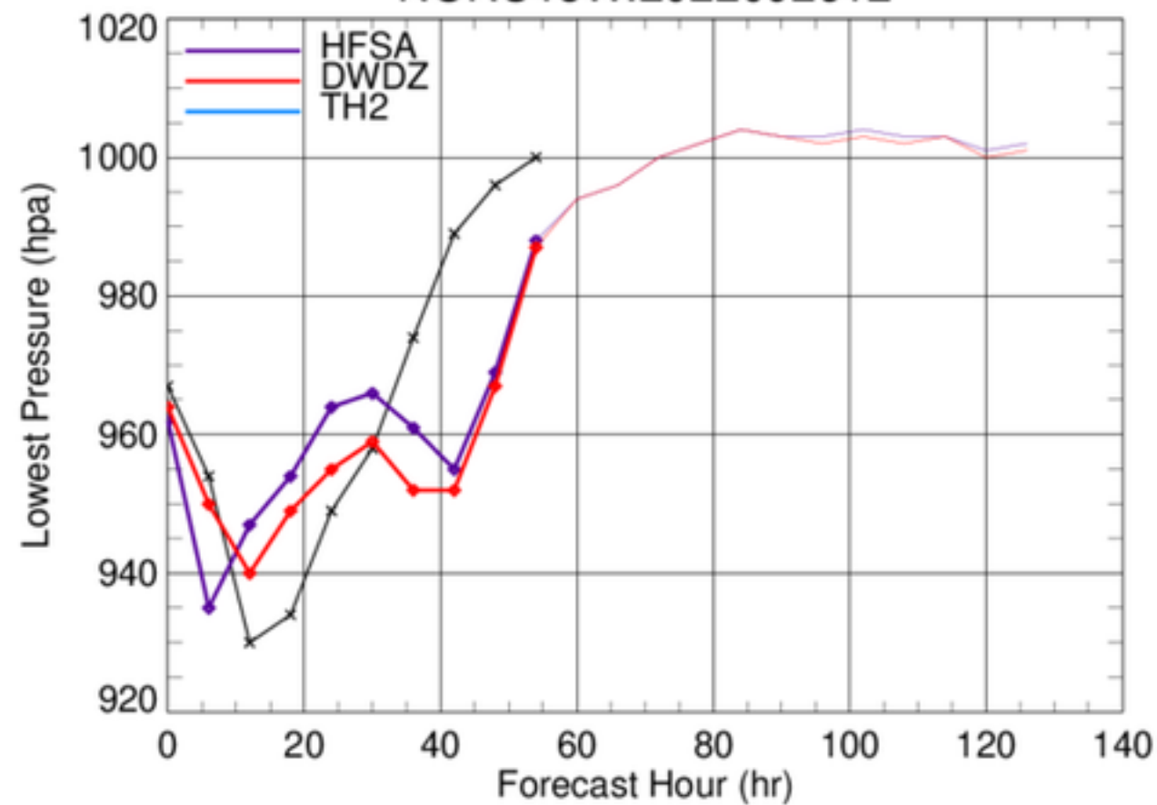
NORU18W.2022092612
