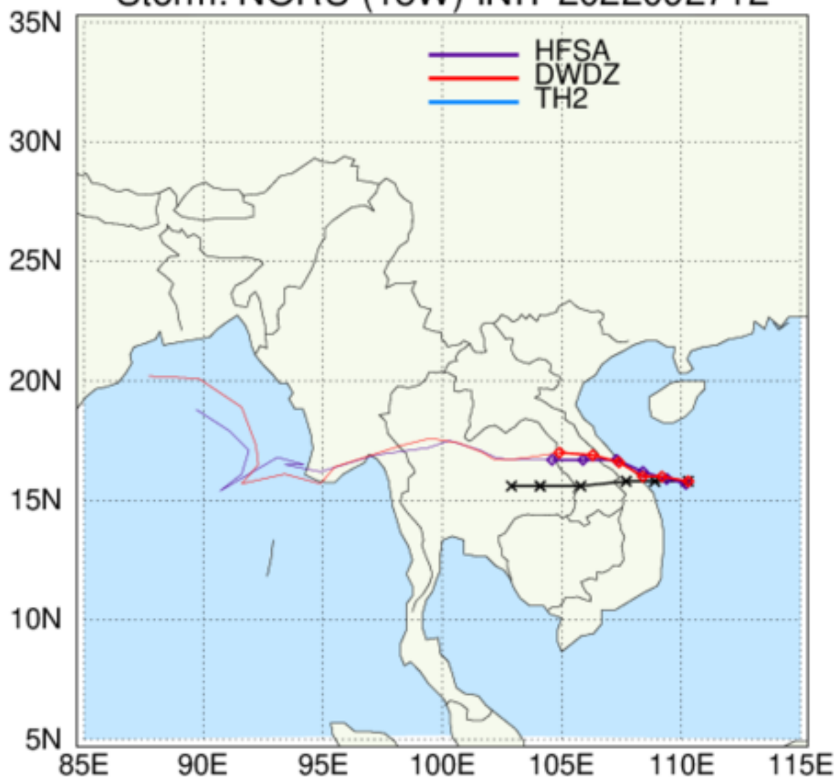
HAFS: TC Tracks Storm: NORU (18W) INIT 2022092712
