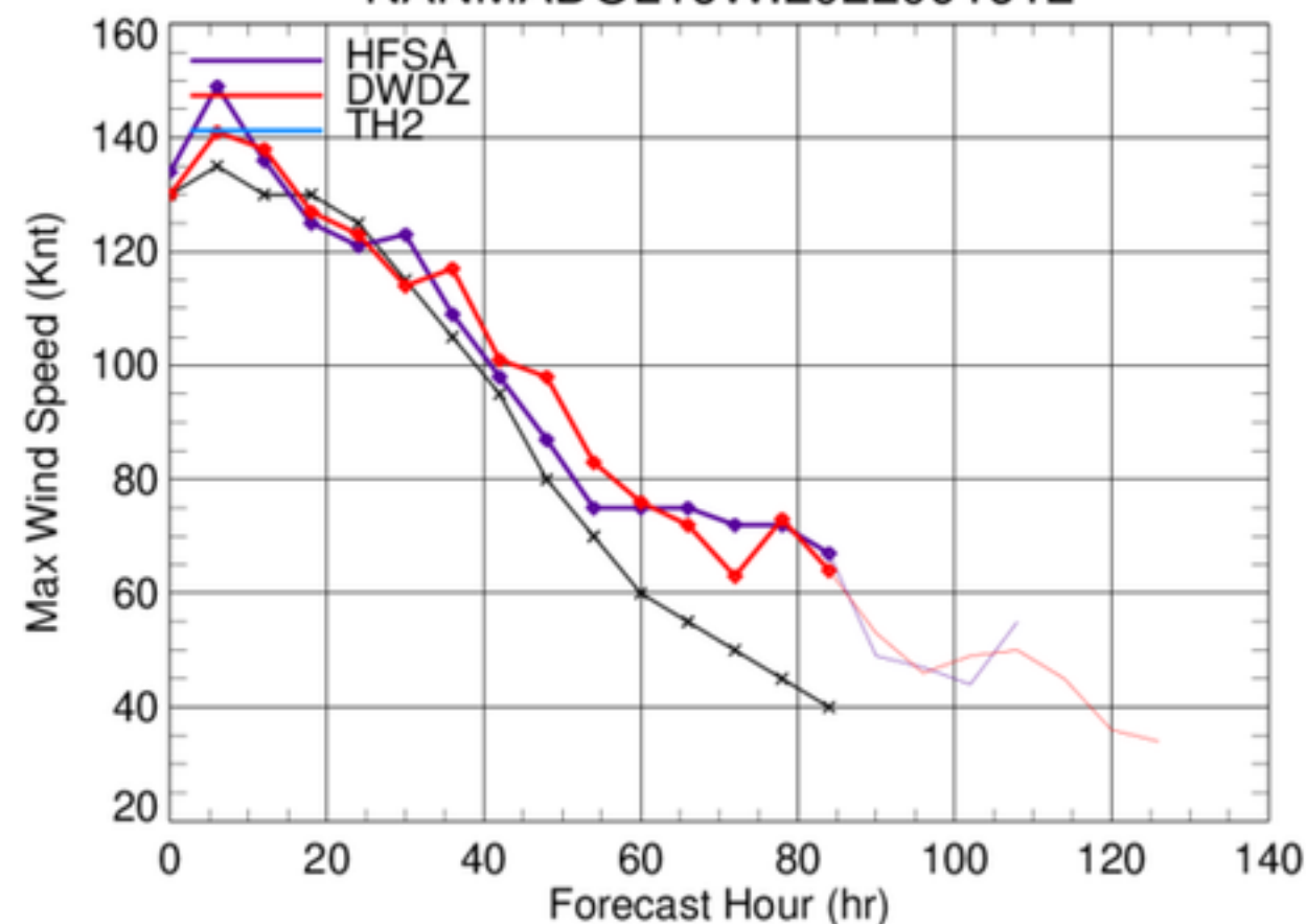
NANMADOL16W.2022091612
