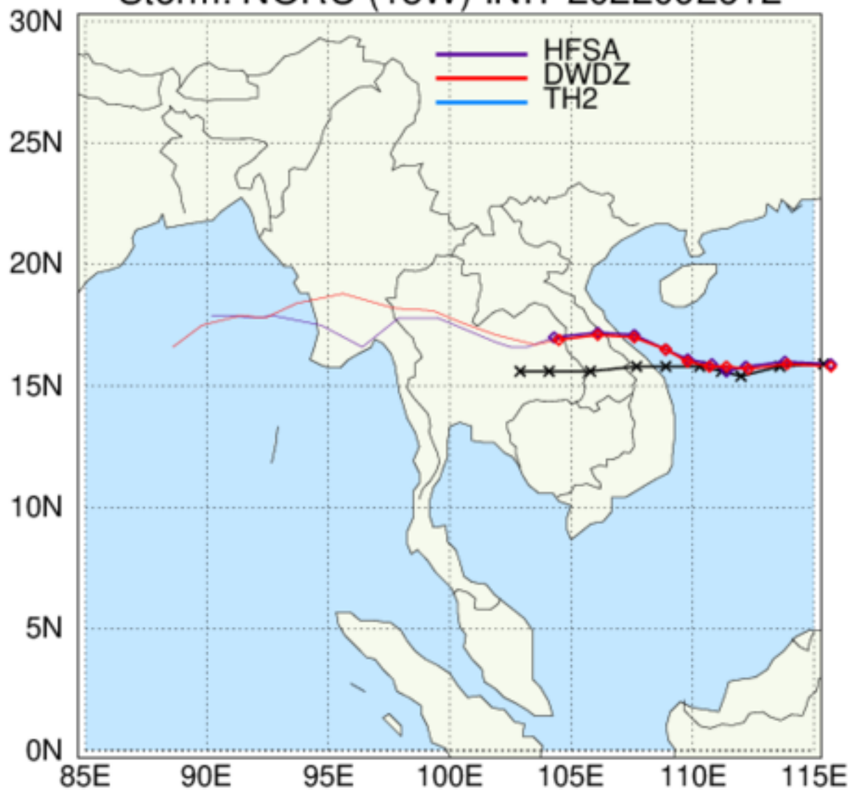
HAFS: TC Tracks Storm: NORU (18W) INIT 2022092612
