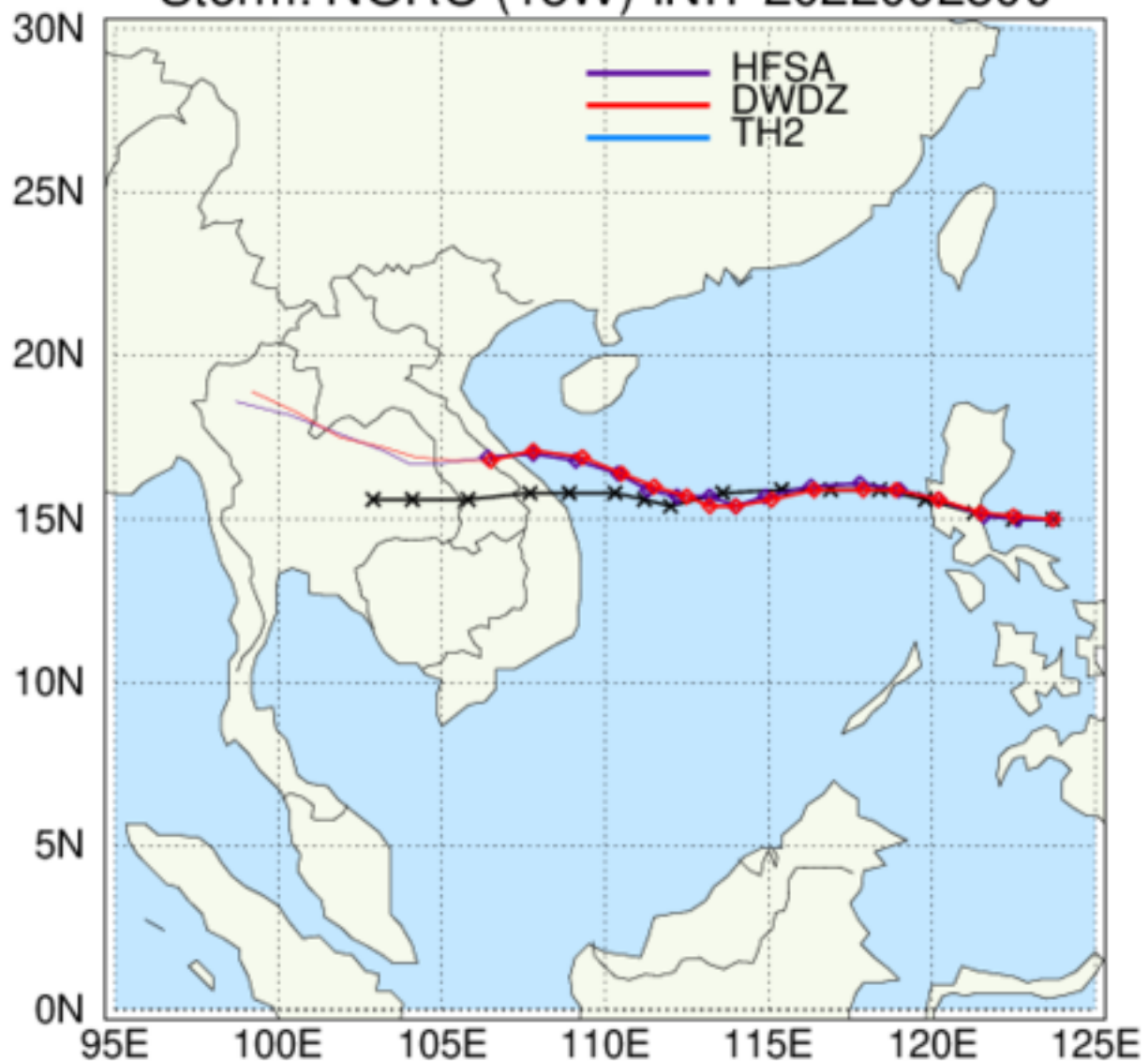
HAFS: TC Tracks Storm: NORU (18W) INIT 2022092500
