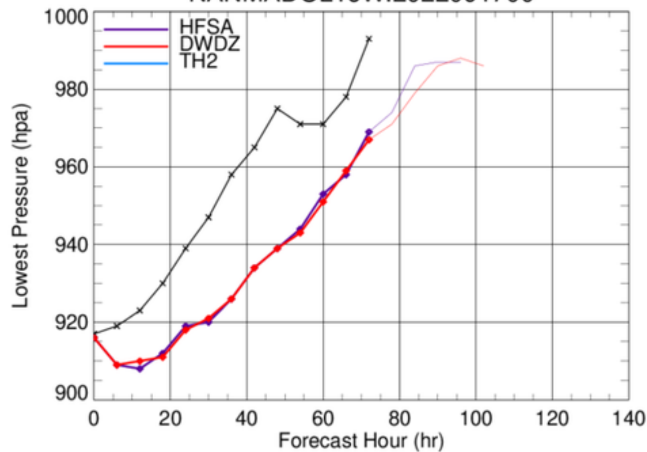
NANMADOL16W.2022091700
