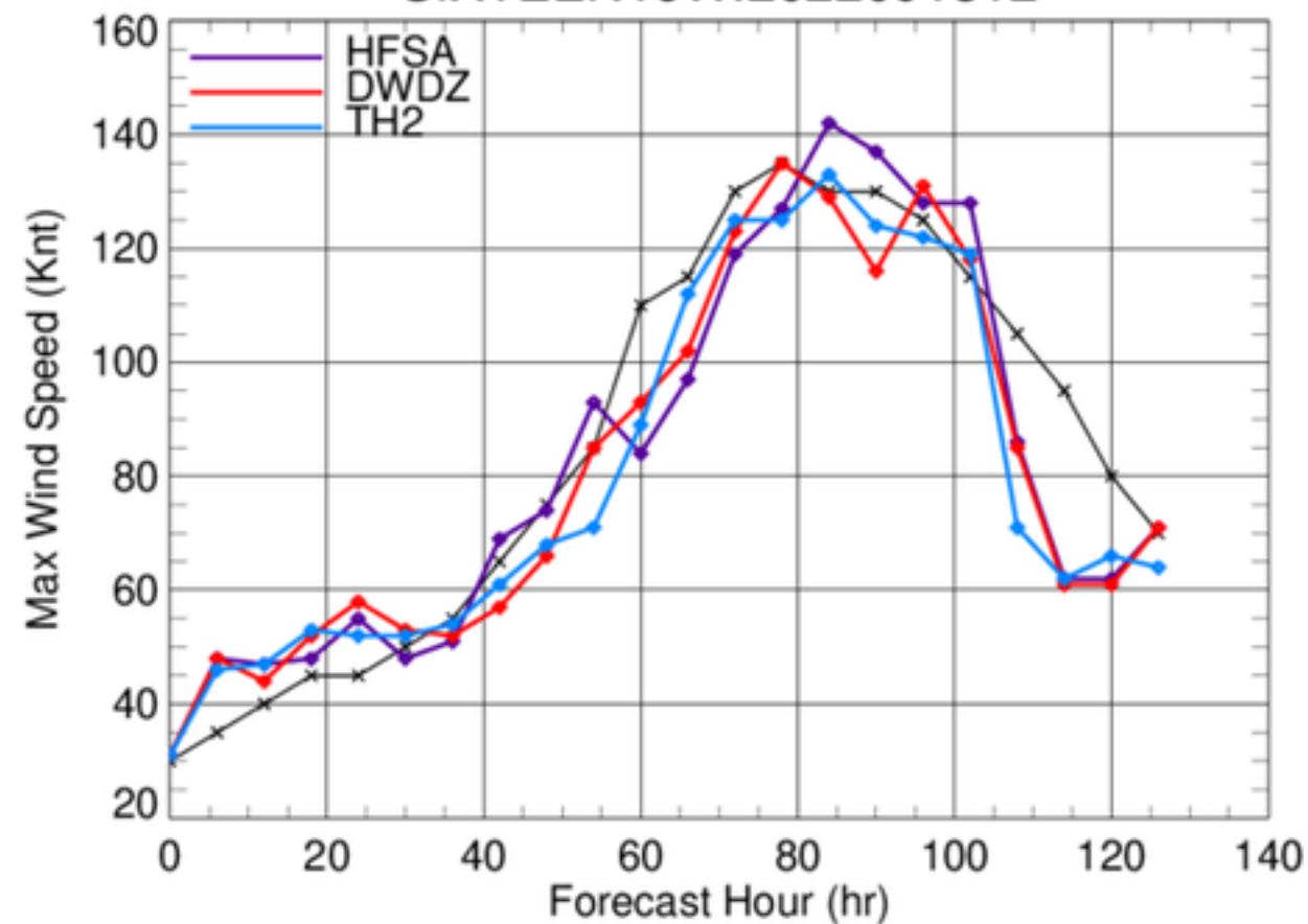
SIXTEEN16W.2022091312
