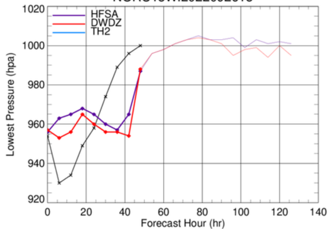
NORU18W.2022092618
