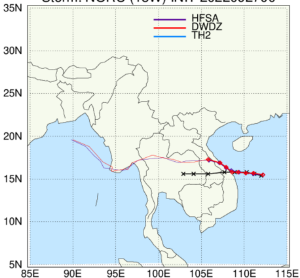
HAFS: TC Tracks Storm: NORU (18W) INIT 2022092700
