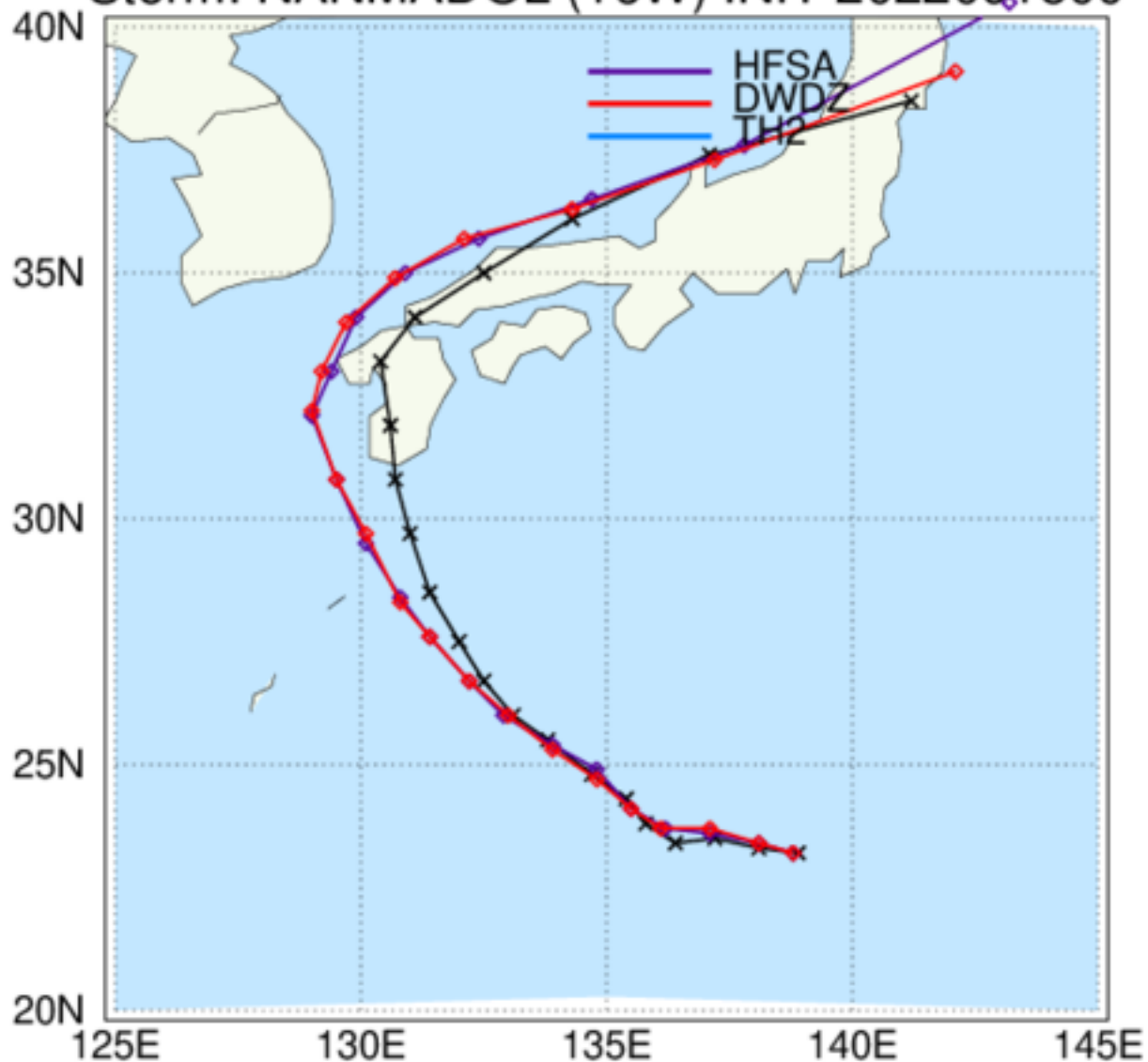
HAFS: TC Tracks Storm: NANMADOL (16W) INIT 2022091500
