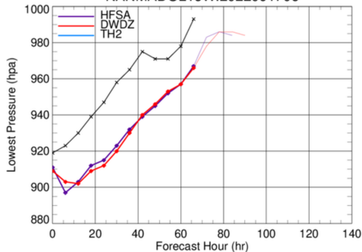
NANMADOL16W.2022091706
