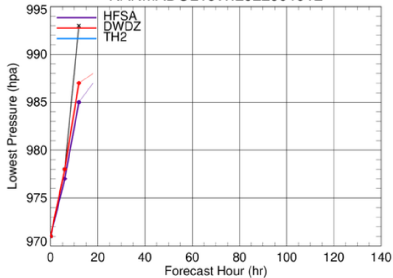
NANMADOL16W.2022091912
