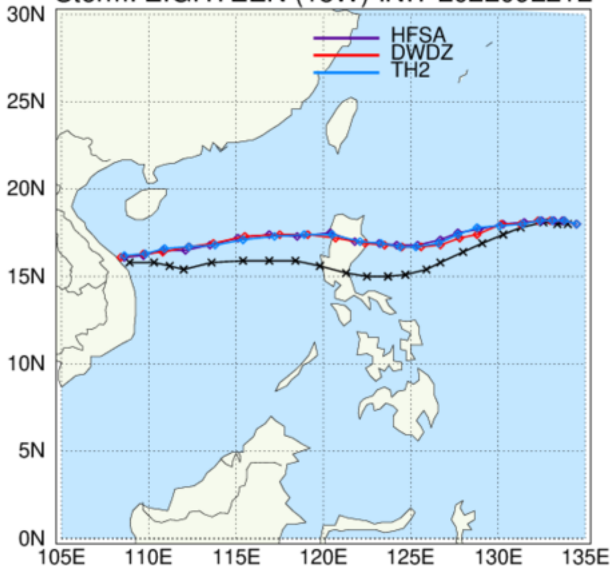
HAFS: TC Tracks Storm: EIGHTEEN (18W) INIT 2022092212
