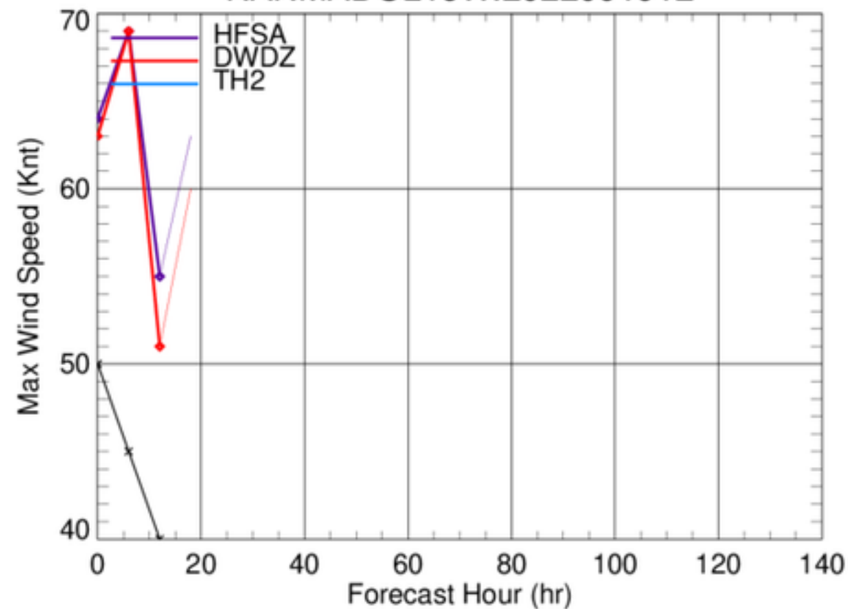
NANMADOL16W.2022091912
