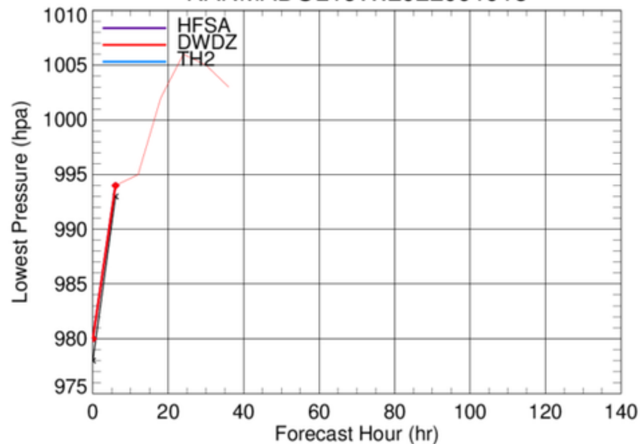
NANMADOL16W.2022091918
