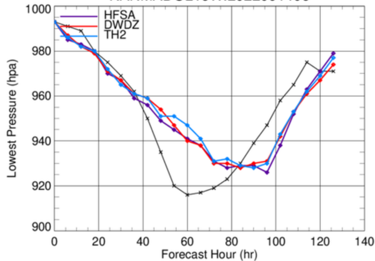
NANMADOL16W.2022091406
