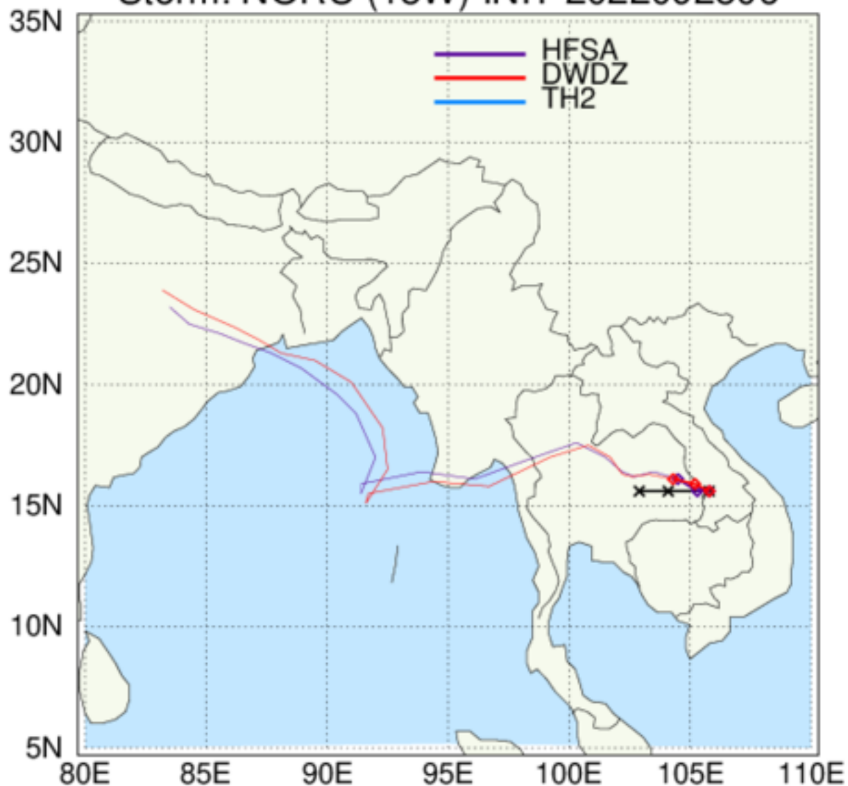
HAFS: TC Tracks Storm: NORU (18W) INIT 2022092806
