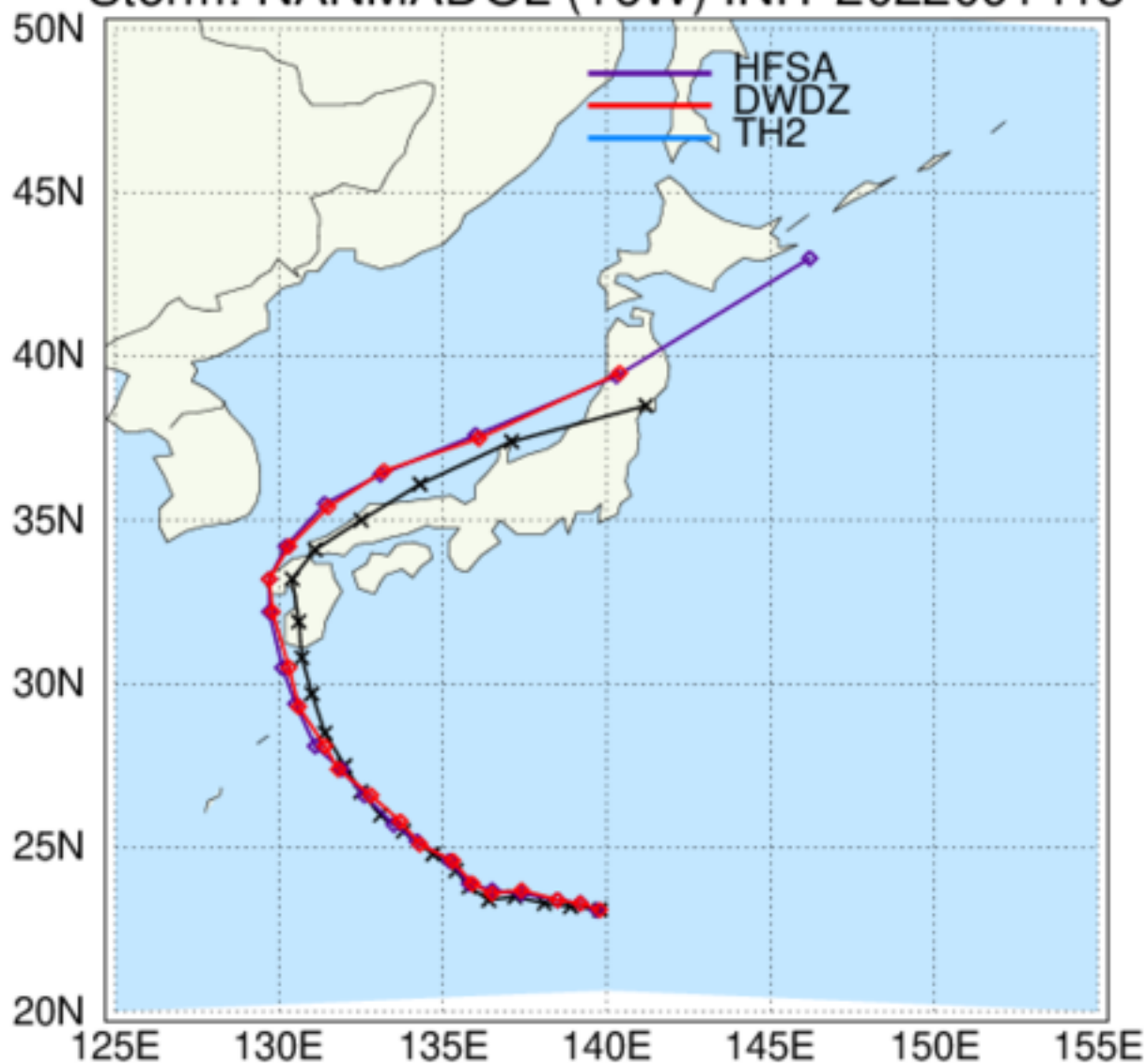
HAFS: TC Tracks Storm: NANMADOL (16W) INIT 2022091418
