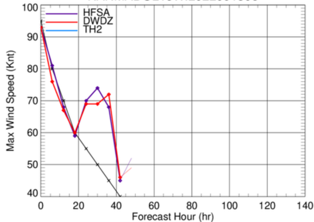
NANMADOL16W.2022091806
