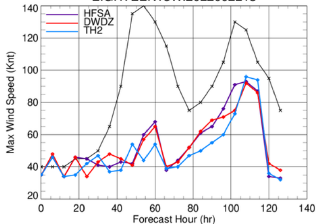
EIGHTEEN18W.2022092218
