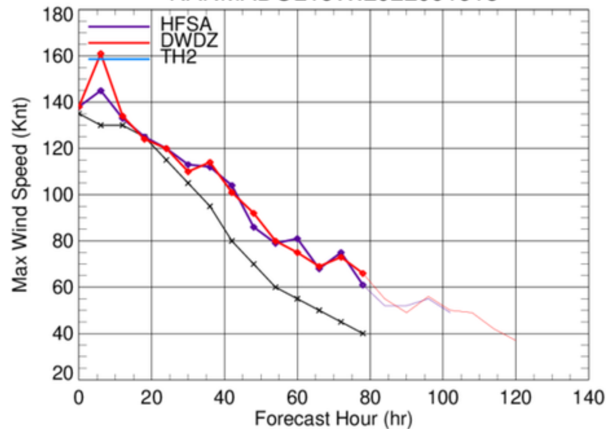
NANMADOL16W.2022091618
