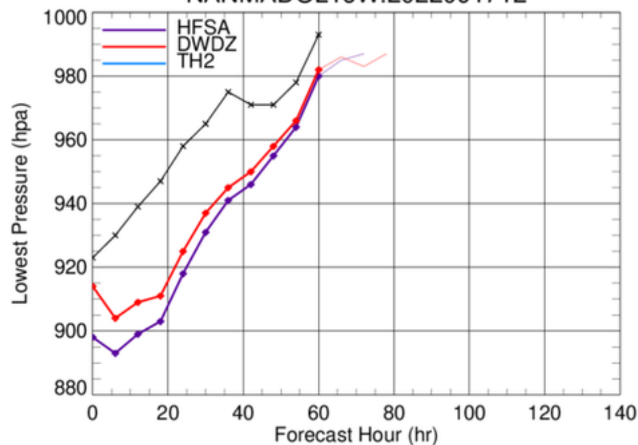
NANMADOL16W.2022091712
