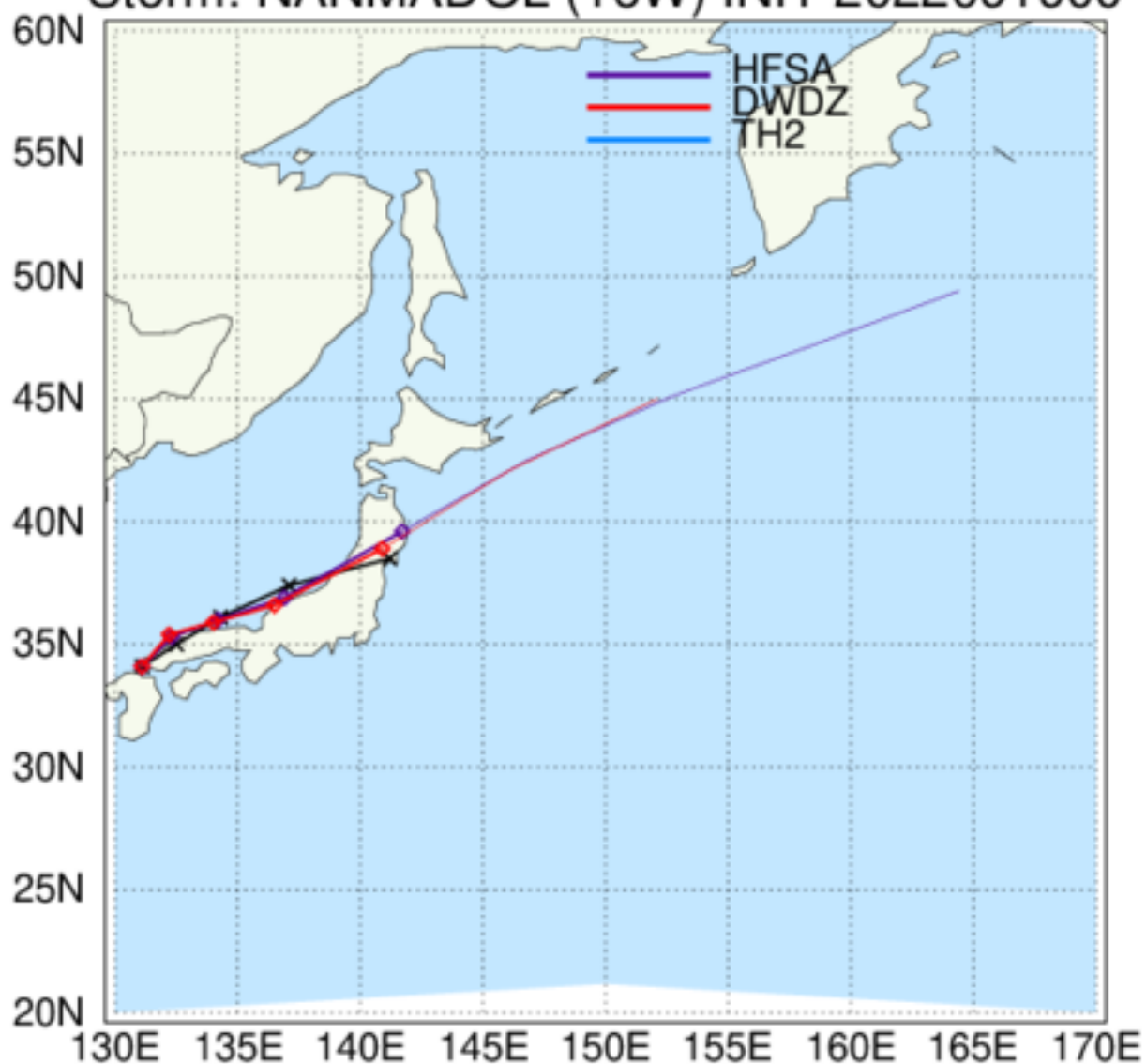
HAFS: TC Tracks Storm: NANMADOL (16W) INIT 2022091900
