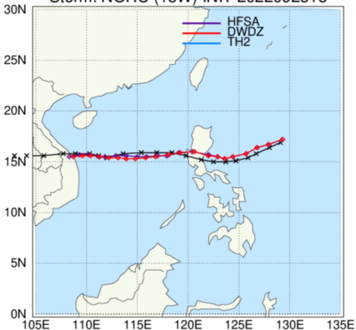
HAFS: TC Tracks Storm: NORU (18W) INIT 2022092318
