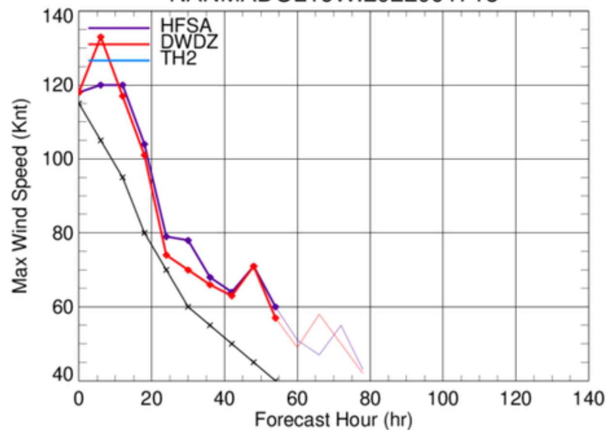
NANMADOL16W.2022091718
