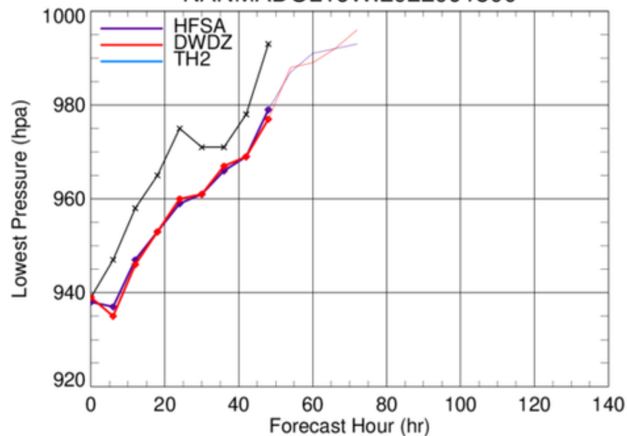
NANMADOL16W.2022091800
