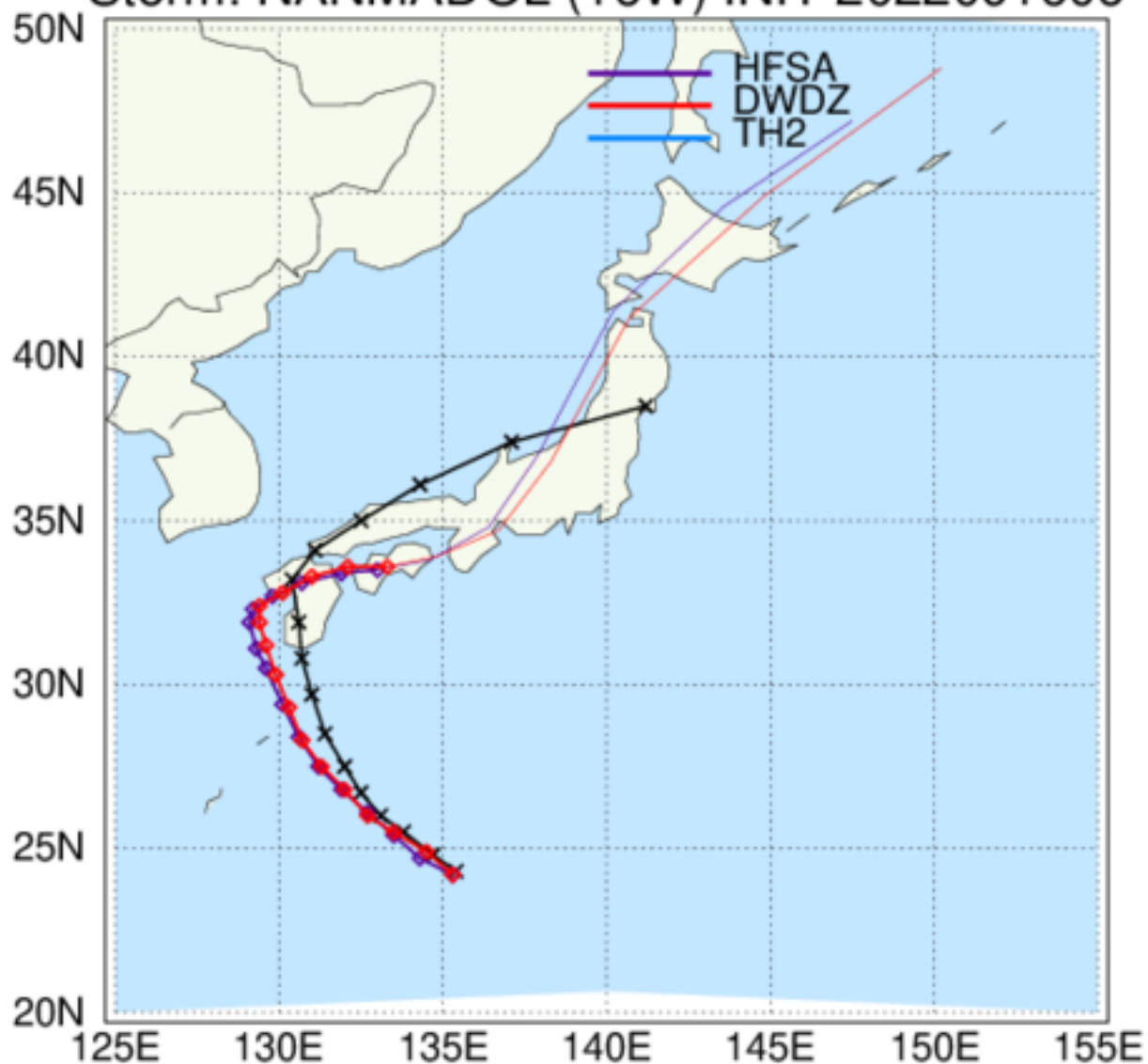
HAFS: TC Tracks Storm: NANMADOL (16W) INIT 2022091606
