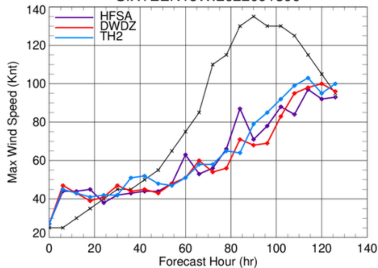
SIXTEEN16W.2022091300
