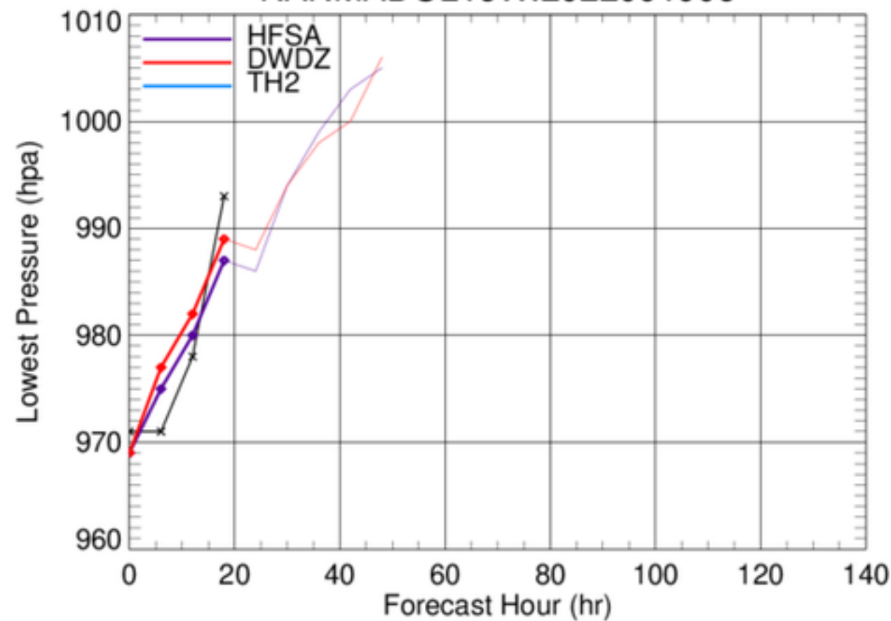
NANMADOL16W.2022091906
