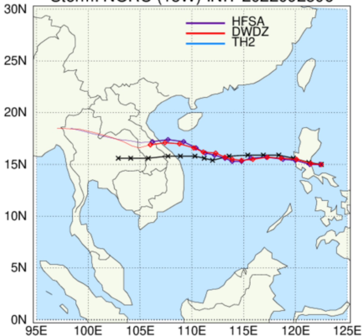
HAFS: TC Tracks Storm: NORU (18W) INIT 2022092506
