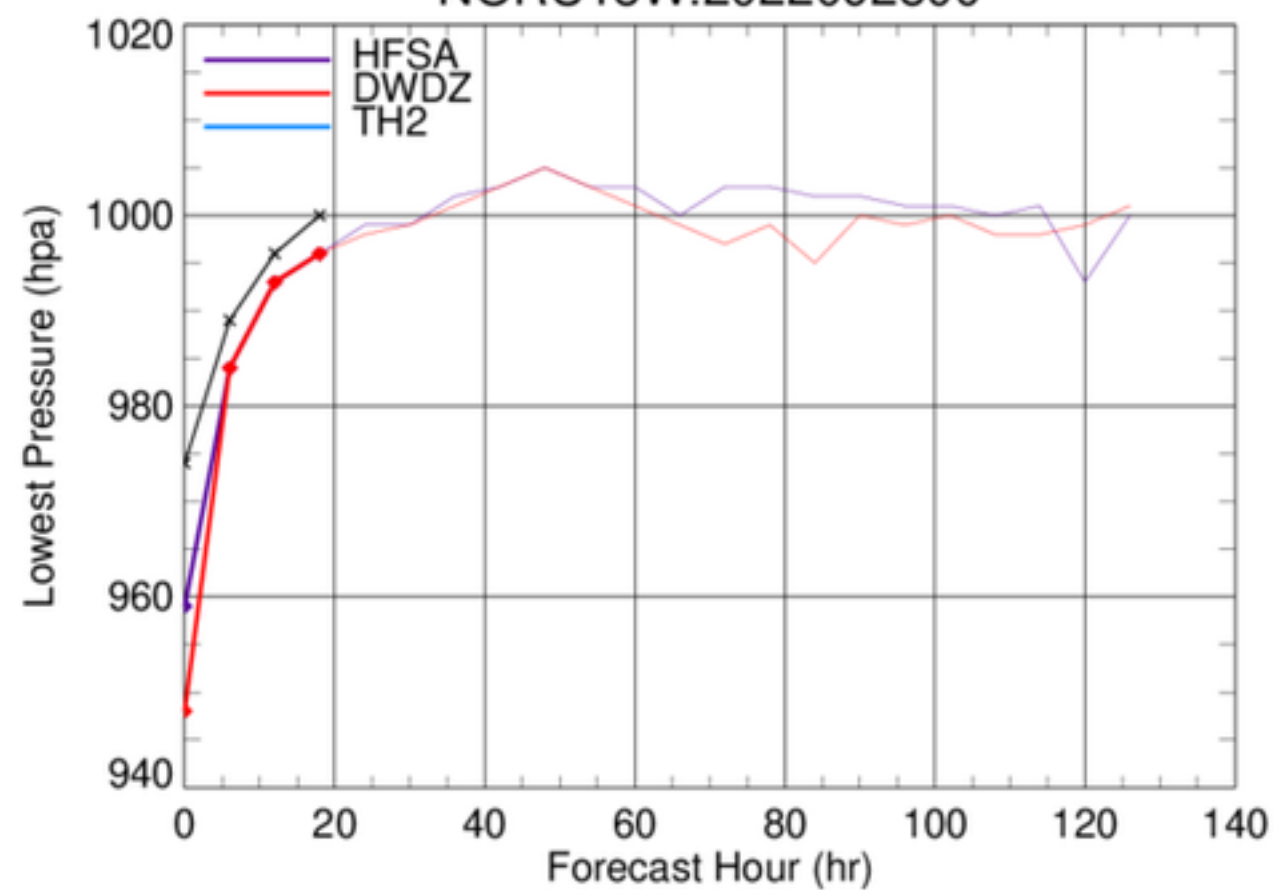
NORU18W.2022092800
