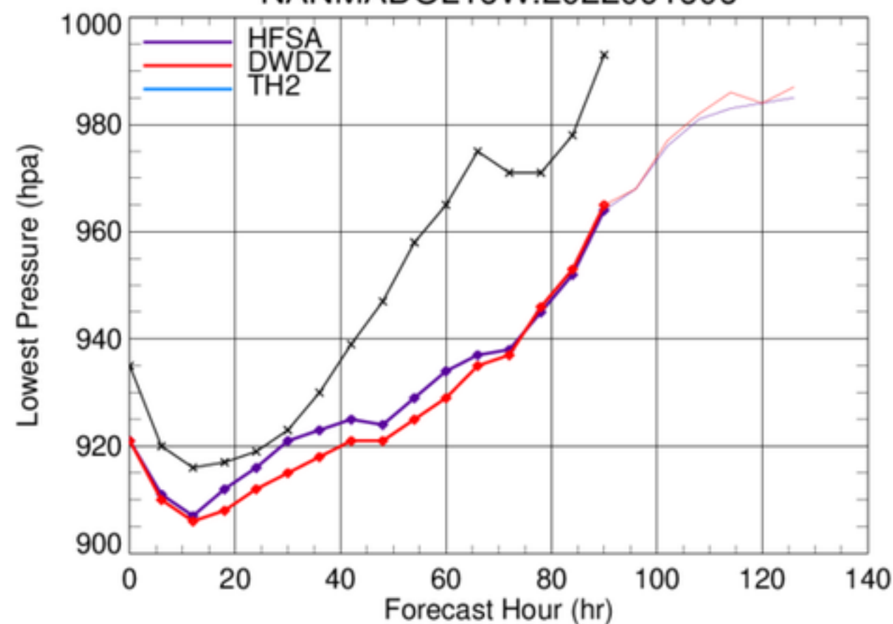
NANMADOL16W.2022091606
