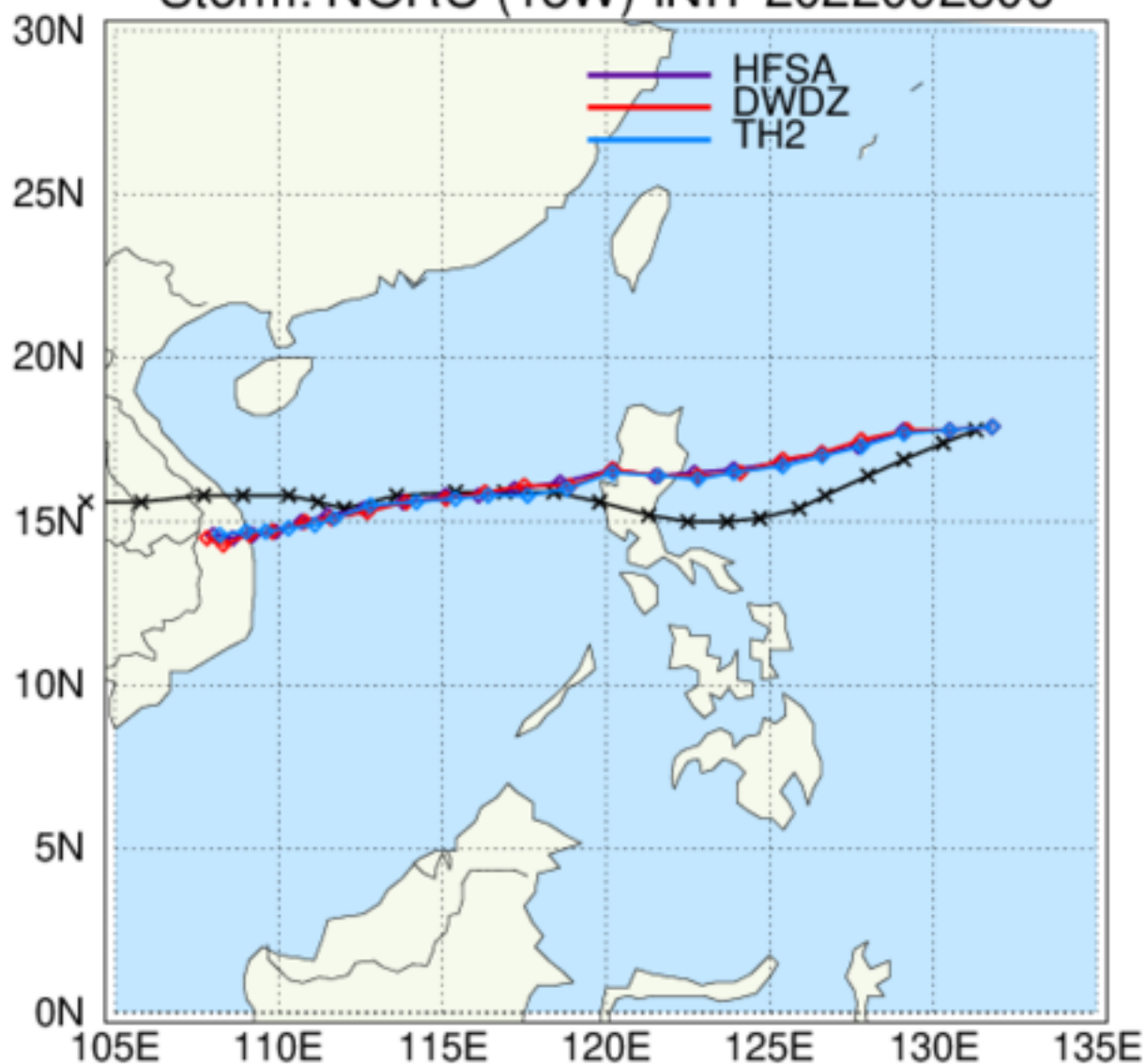
HAFS: TC Tracks Storm: NORU (18W) INIT 2022092306
