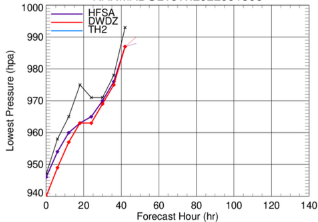
NANMADOL16W.2022091806
