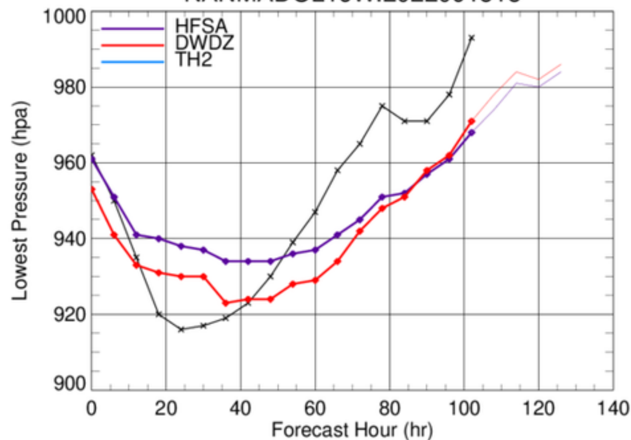
NANMADOL16W.2022091518
