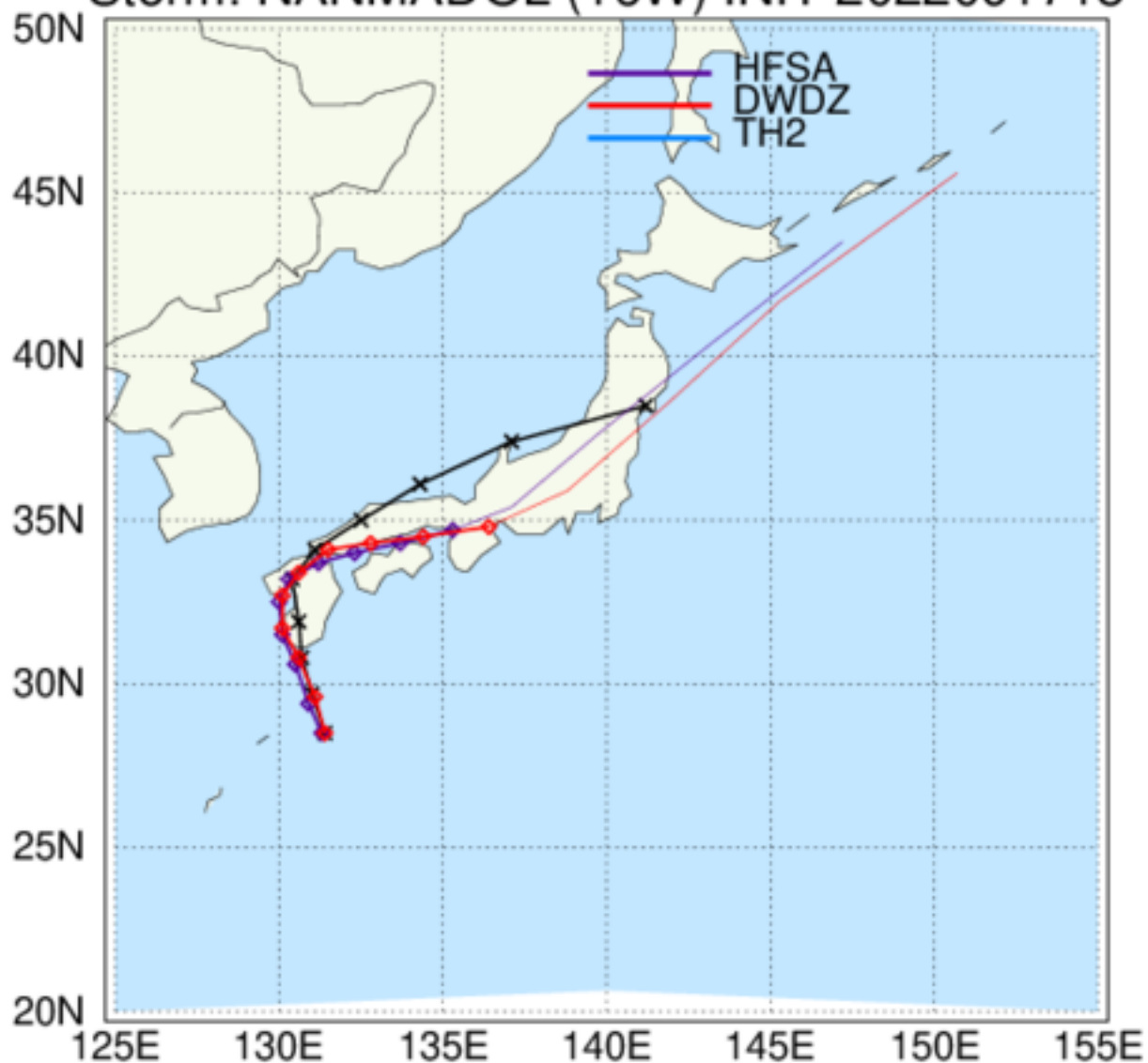
HAFS: TC Tracks Storm: NANMADOL (16W) INIT 2022091718
