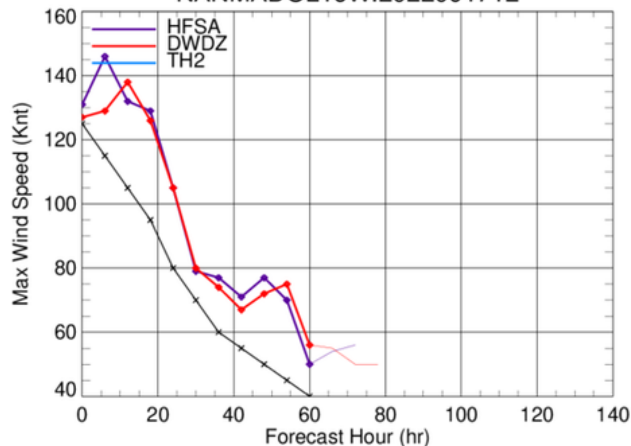
NANMADOL16W.2022091712
