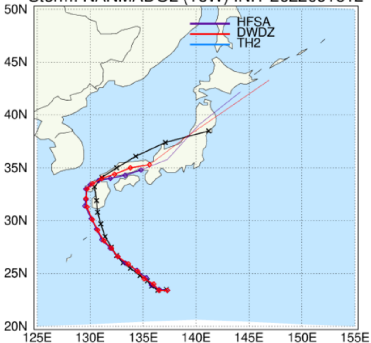
HAFS: TC Tracks Storm: NANMADOL (16W) INIT 2022091512
