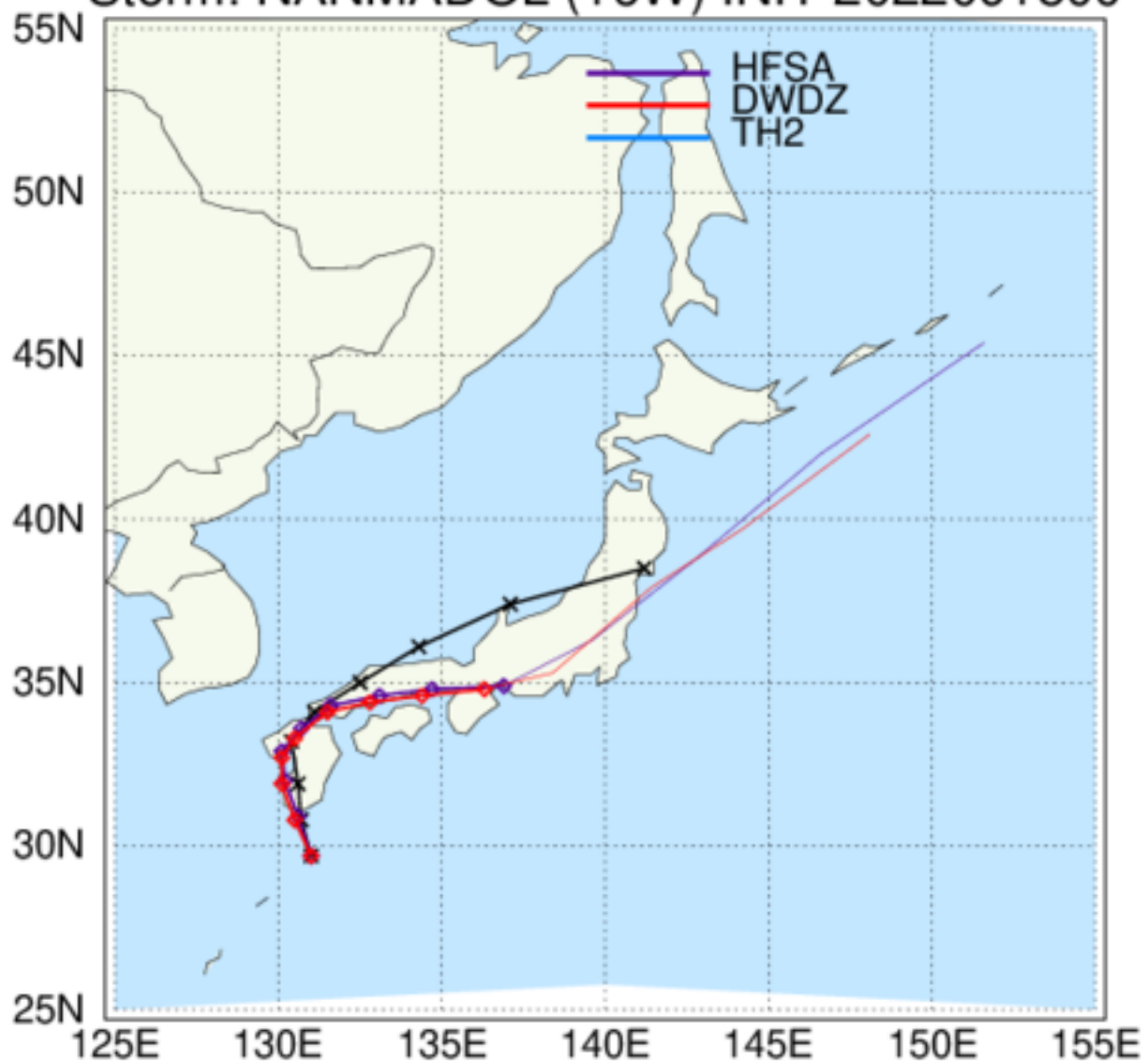
HAFS: TC Tracks Storm: NANMADOL (16W) INIT 2022091800
