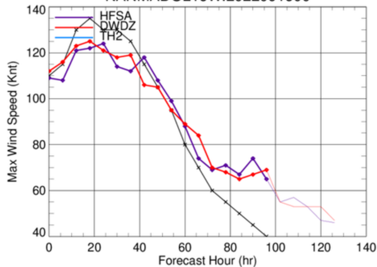
NANMADOL16W.2022091600
