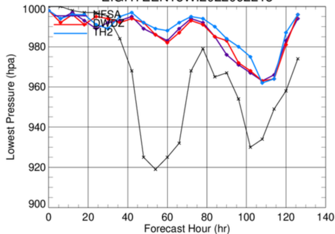
EIGHTEEN18W.2022092218
