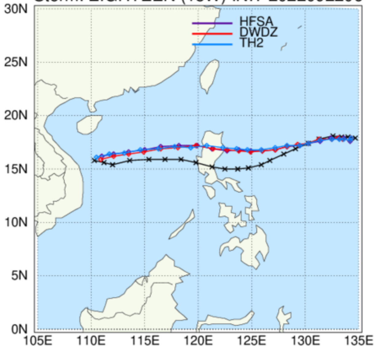
HAFS: TC Tracks Storm: EIGHTEEN (18W) INIT 2022092206
