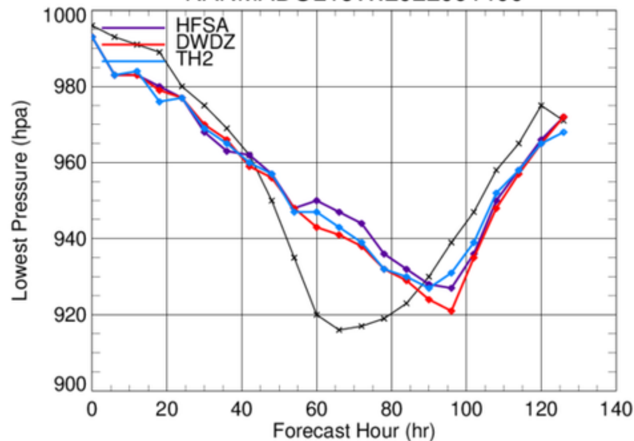
NANMADOL16W.2022091400
