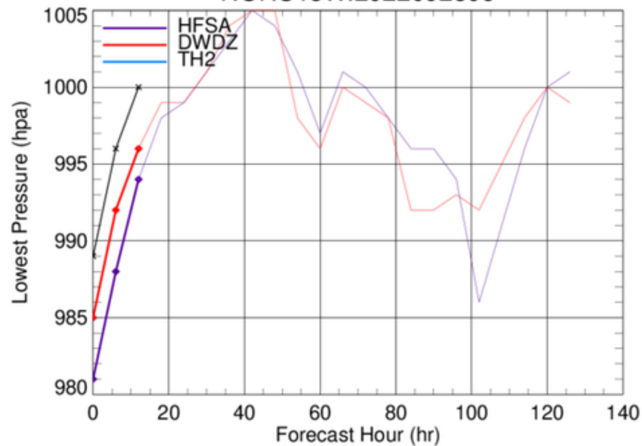
NORU18W.2022092806
