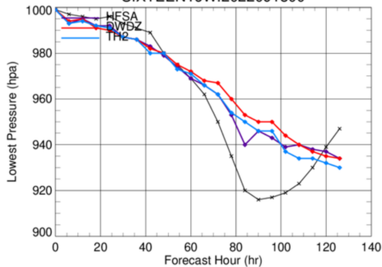
SIXTEEN16W.2022091300
