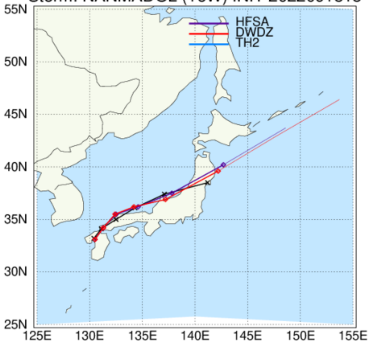
HAFS: TC Tracks Storm: NANMADOL (16W) INIT 2022091818
