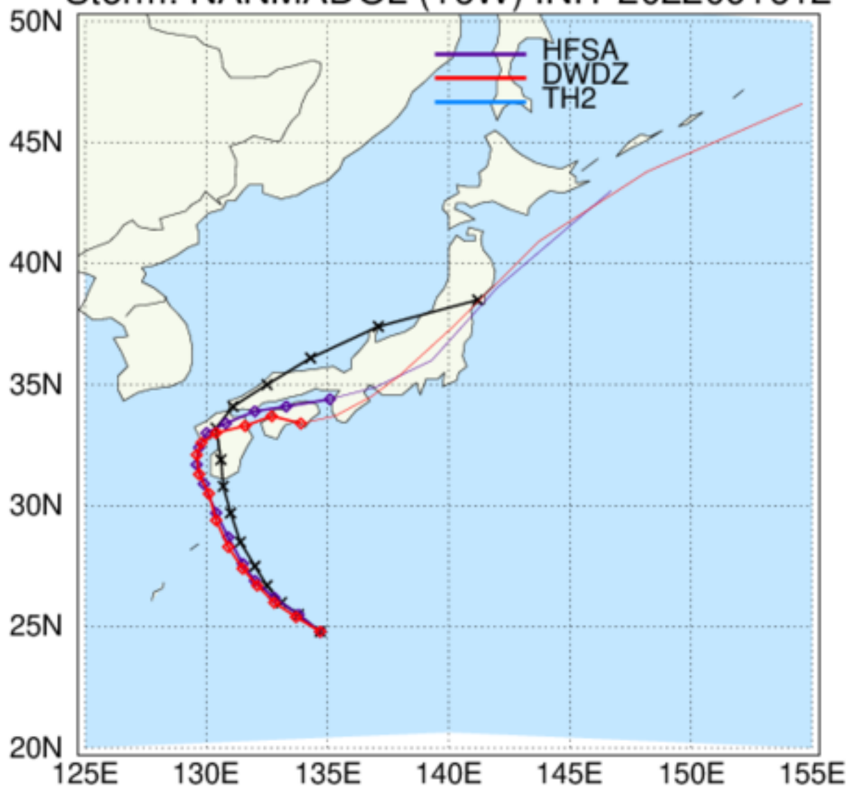
HAFS: TC Tracks Storm: NANMADOL (16W) INIT 2022091612
