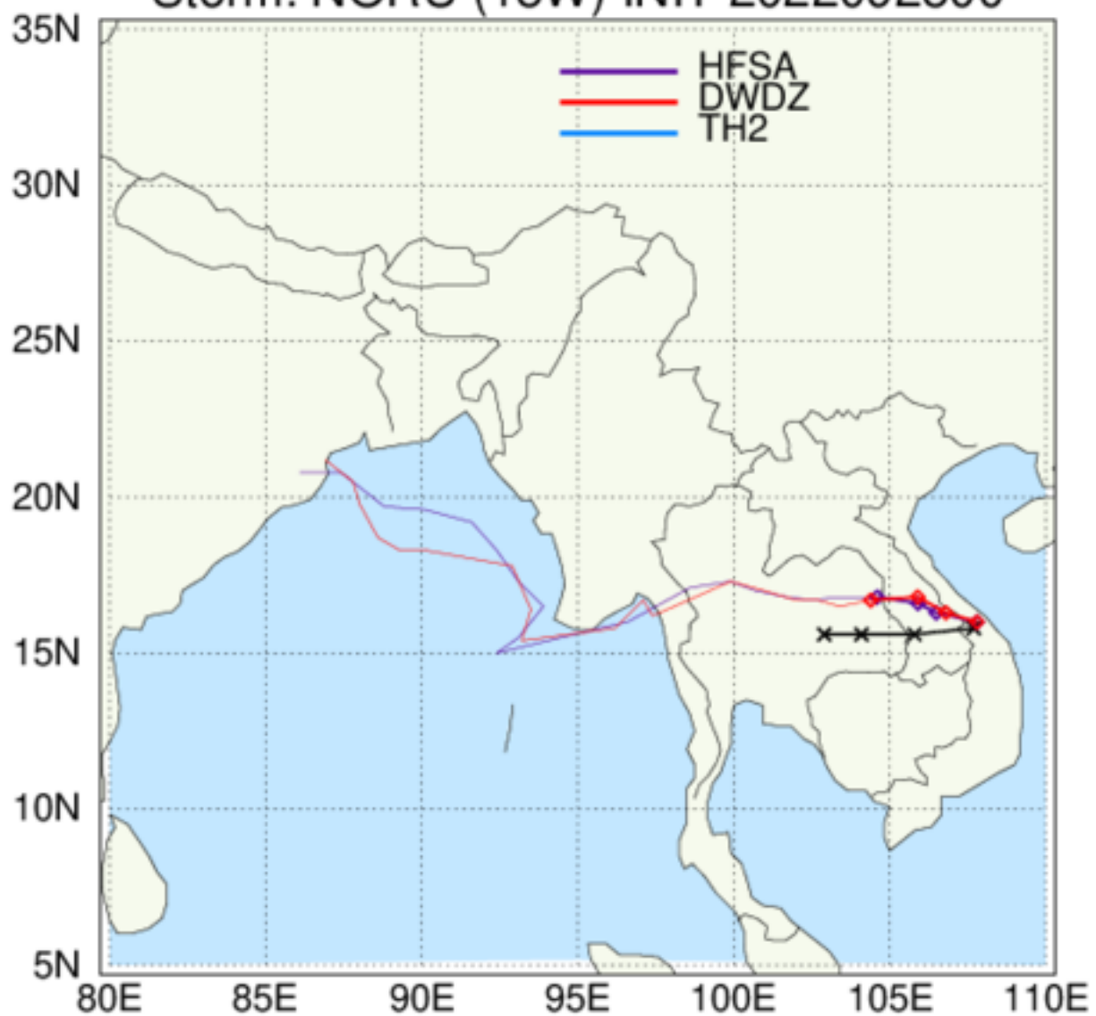
HAFS: TC Tracks Storm: NORU (18W) INIT 2022092800
