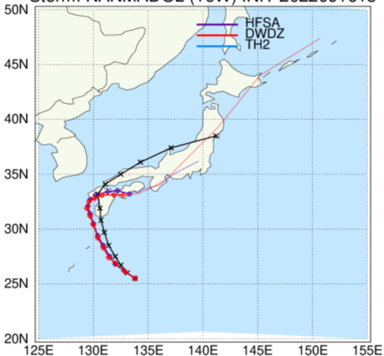
HAFS: TC Tracks Storm: NANMADOL (16W) INIT 2022091618
