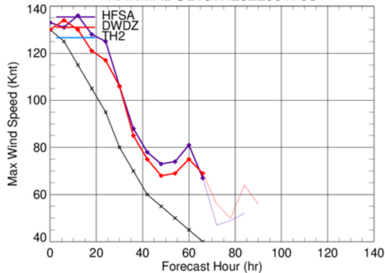
NANMADOL16W.2022091706
