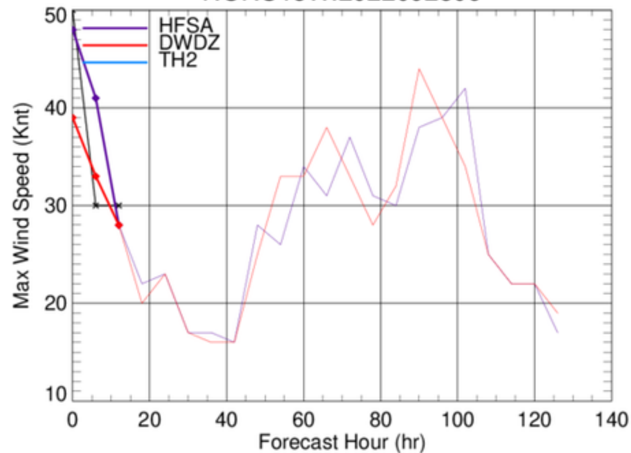
NORU18W.2022092806
