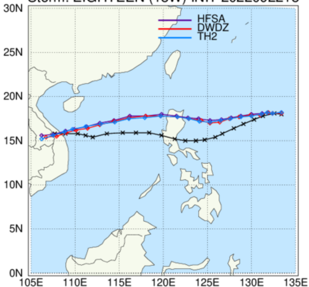
HAFS: TC Tracks Storm: EIGHTEEN (18W) INIT 2022092218
