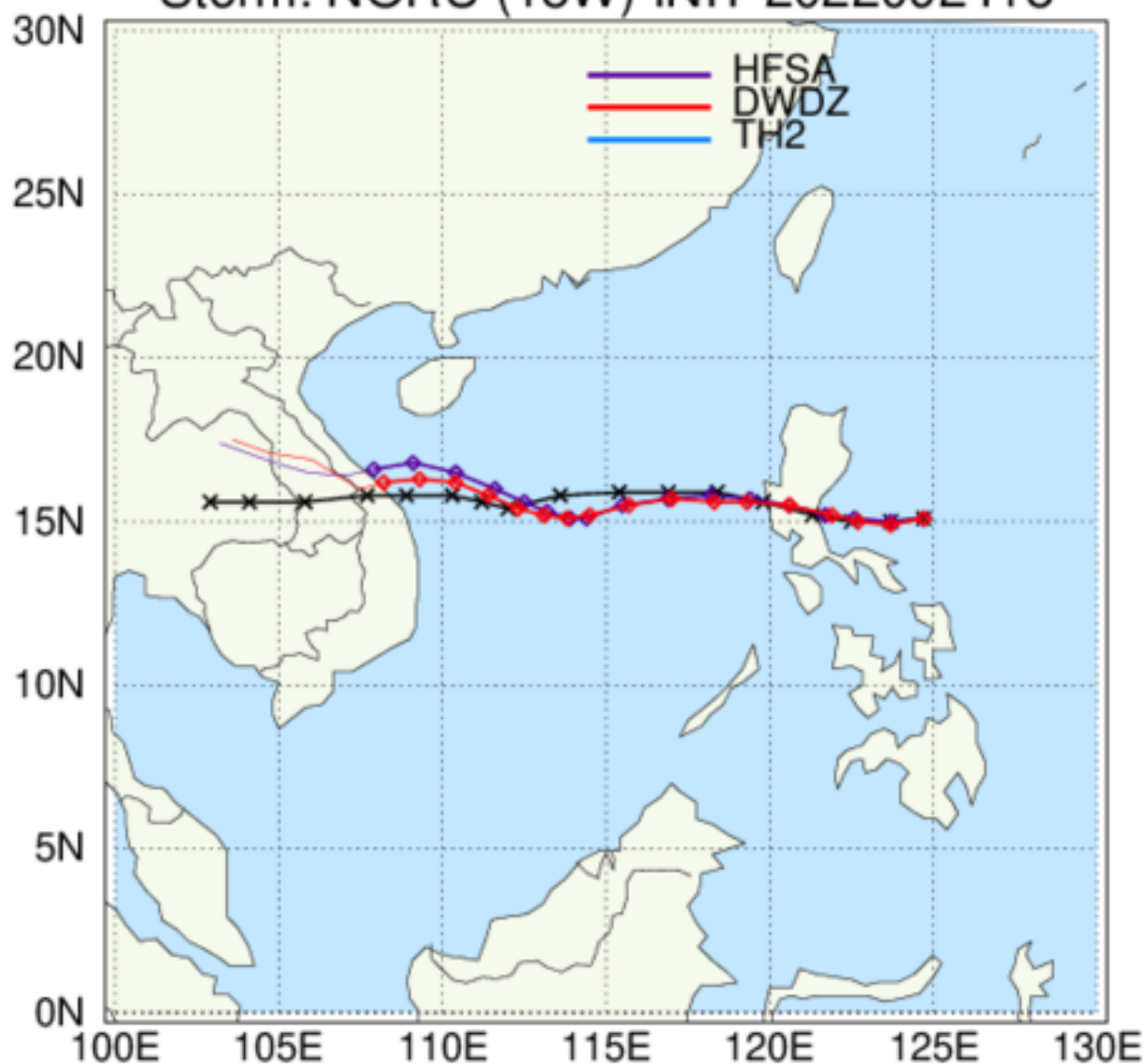
HAFS: TC Tracks Storm: NORU (18W) INIT 2022092418
