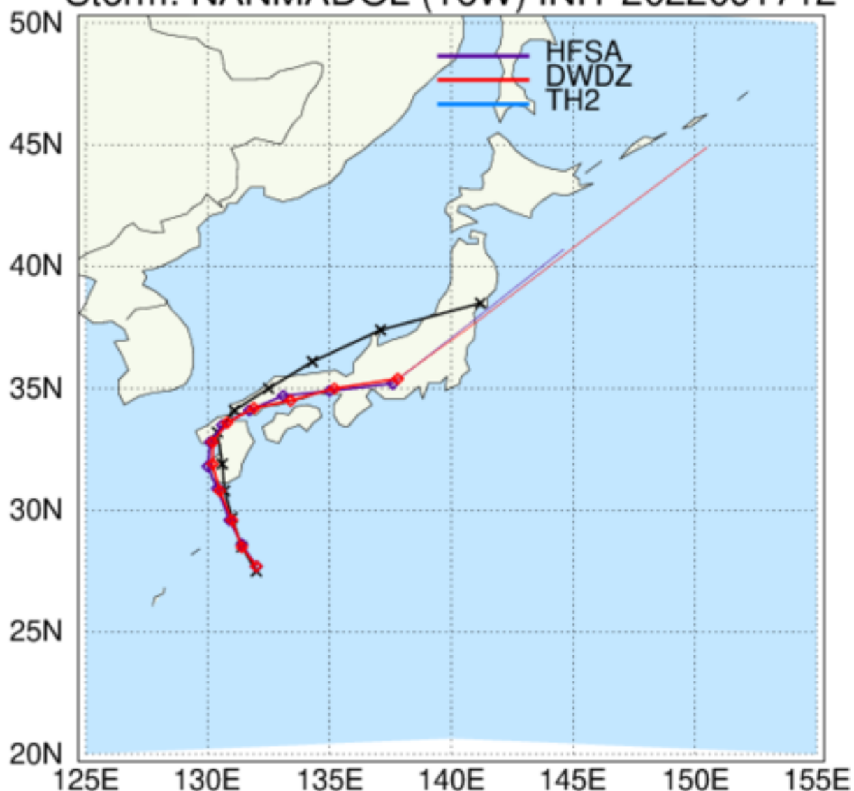
HAFS: TC Tracks Storm: NANMADOL (16W) INIT 2022091712
