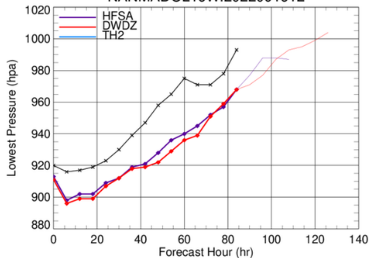
NANMADOL16W.2022091612
