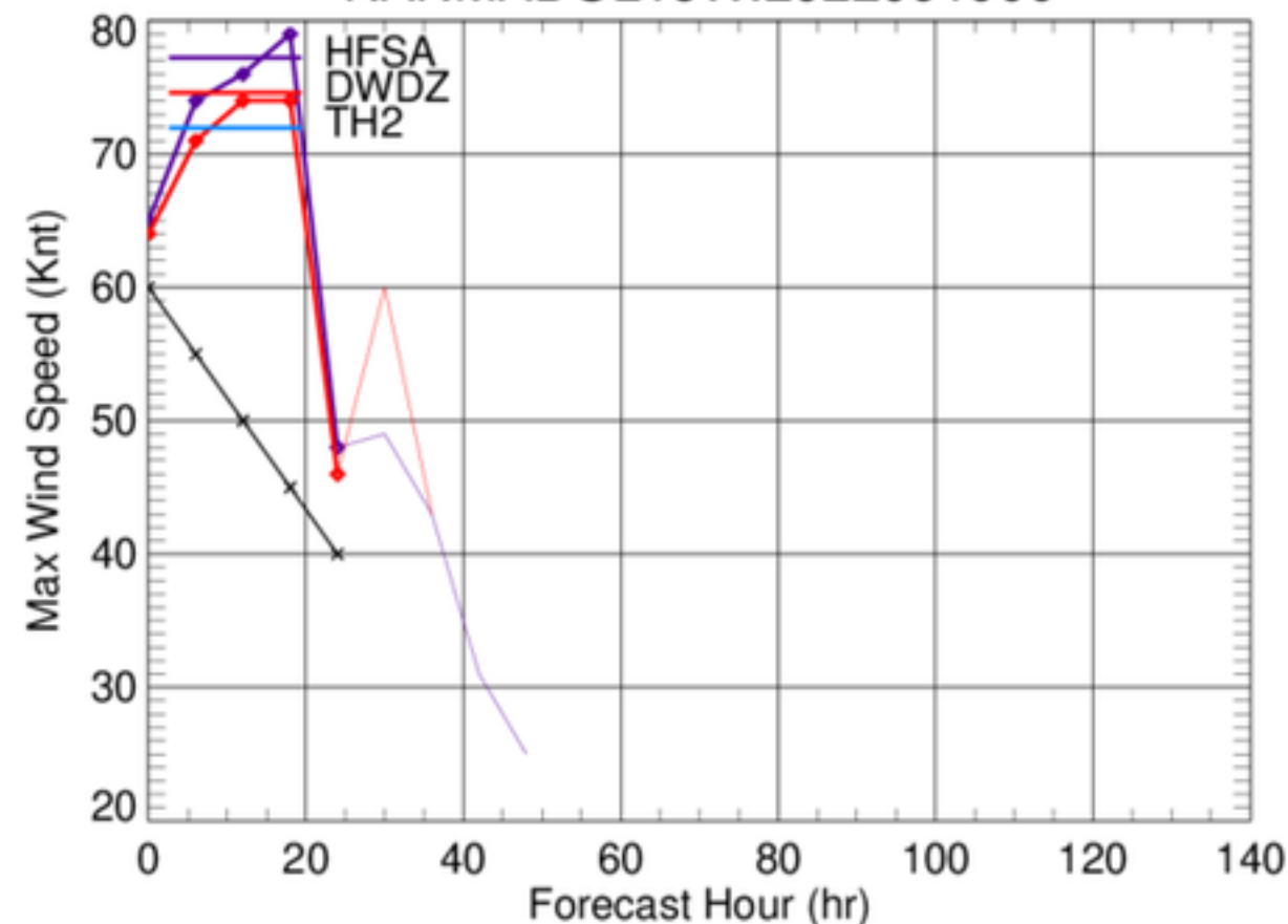
NANMADOL16W.2022091900
