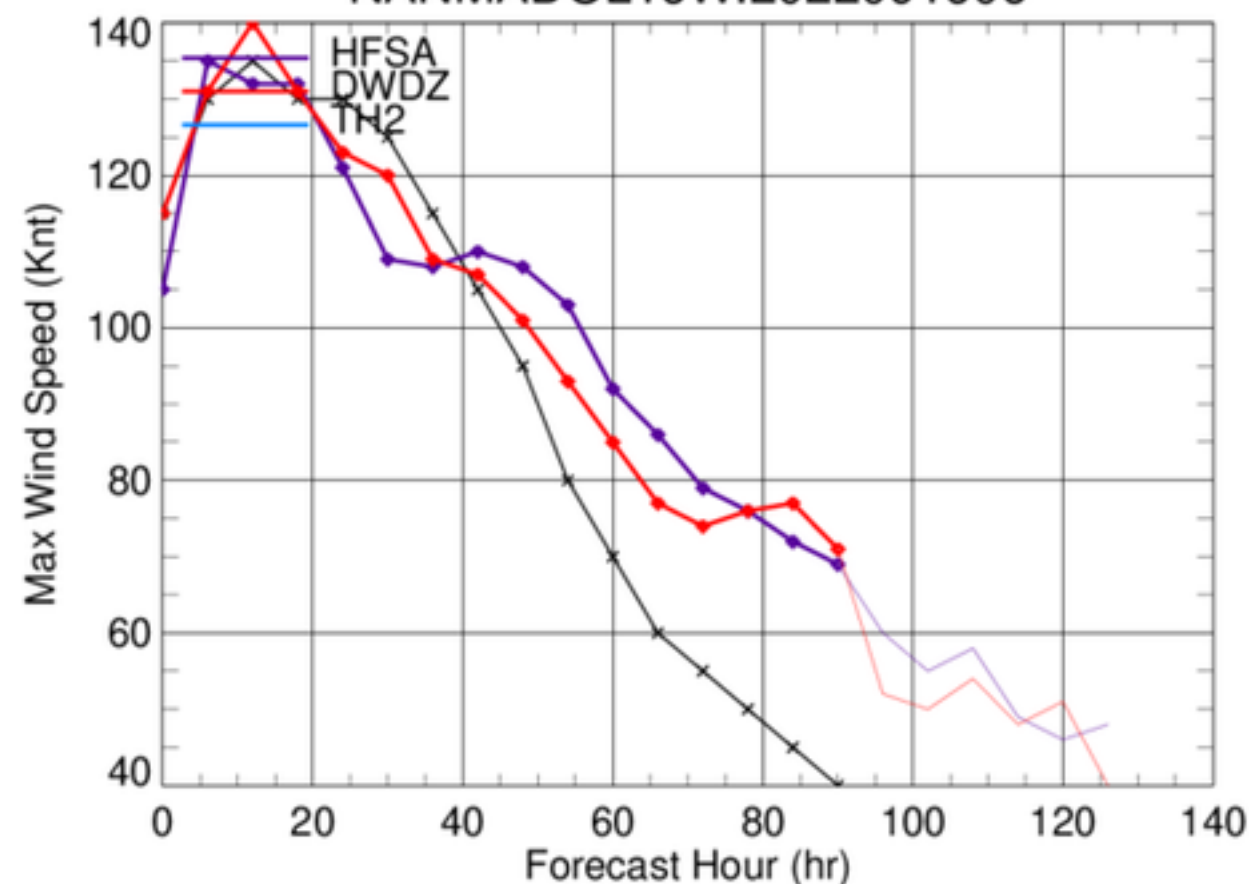
NANMADOL16W.2022091606
