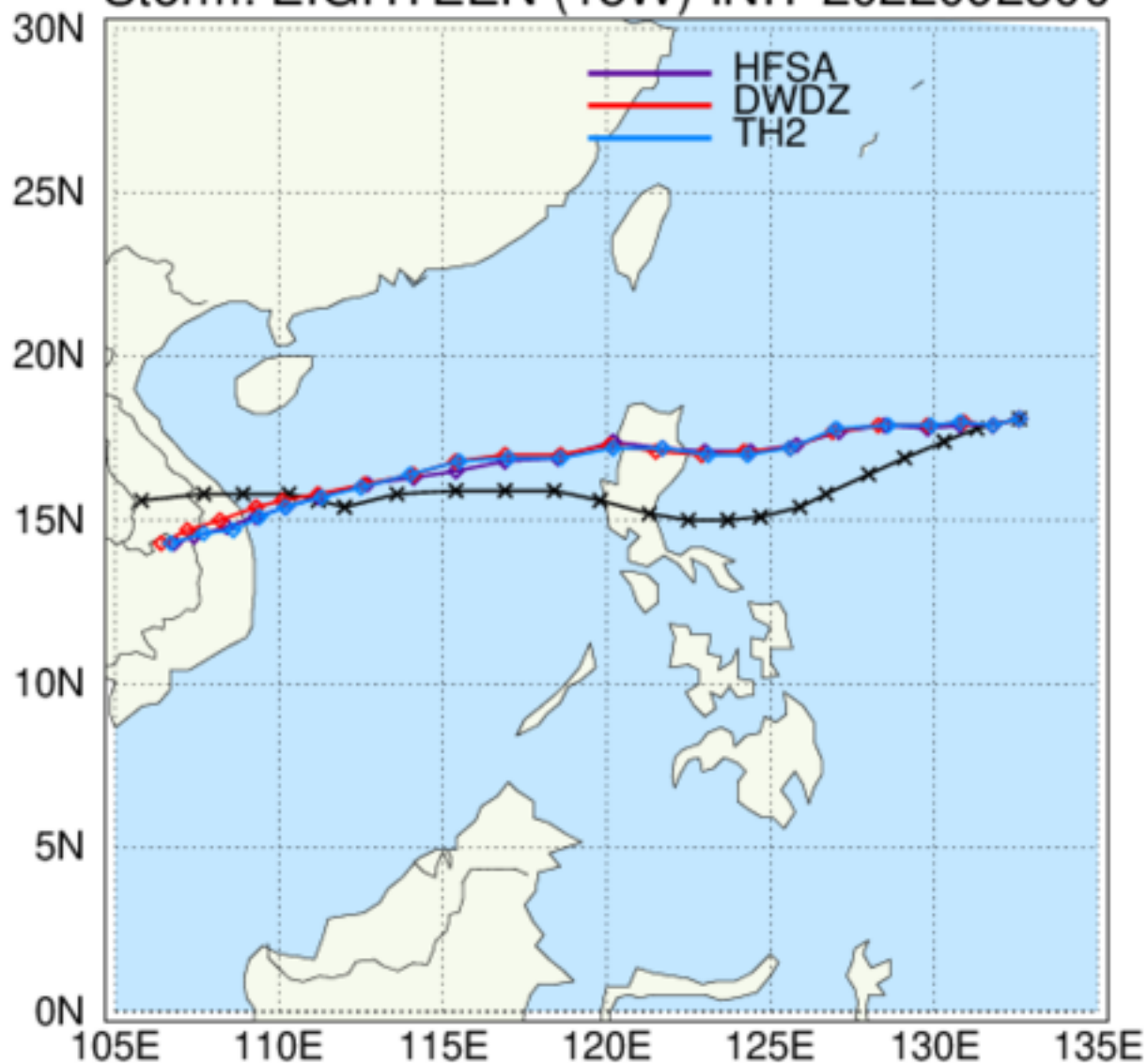
HAFS: TC Tracks Storm: EIGHTEEN (18W) INIT 2022092300
