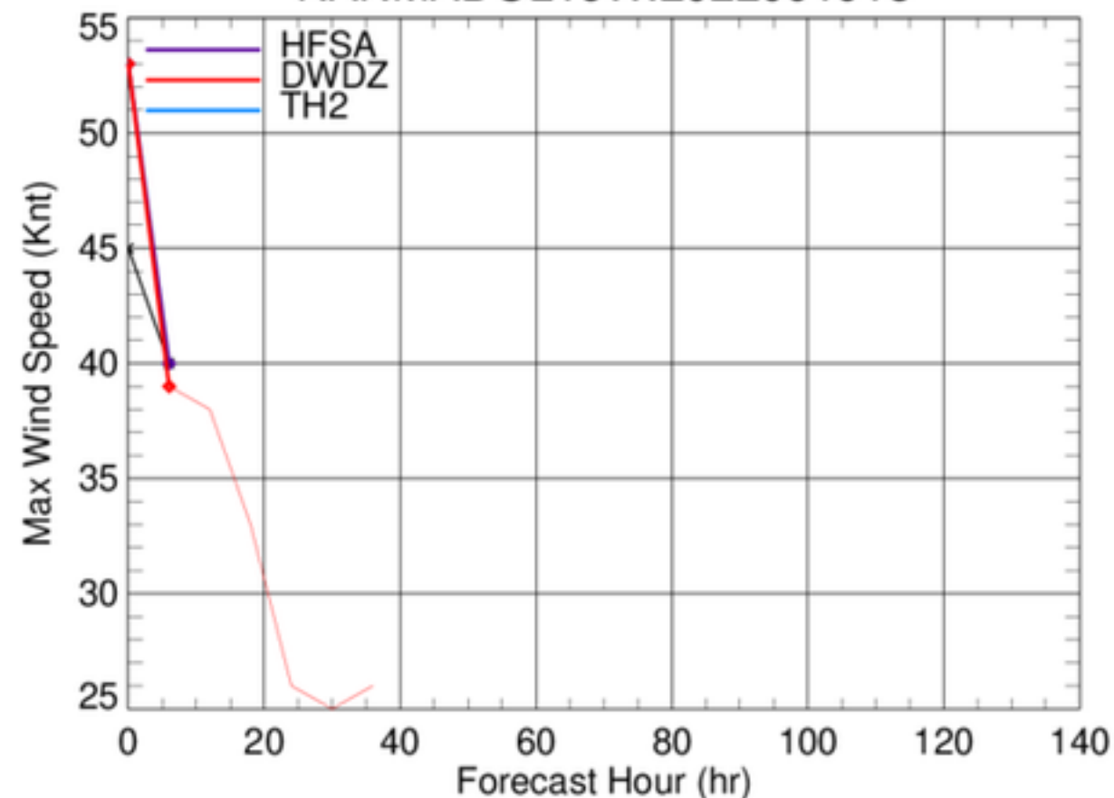
NANMADOL16W.2022091918
