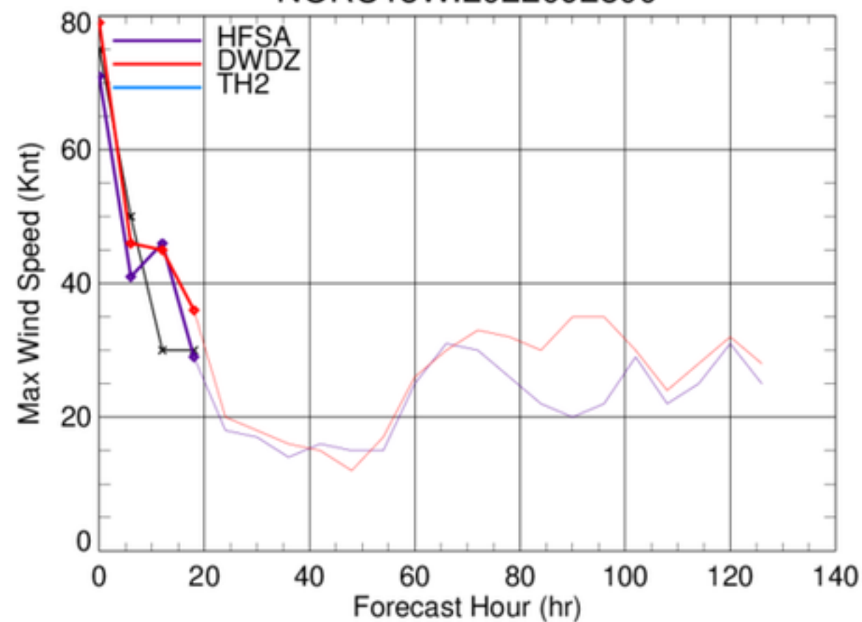
NORU18W.2022092800
