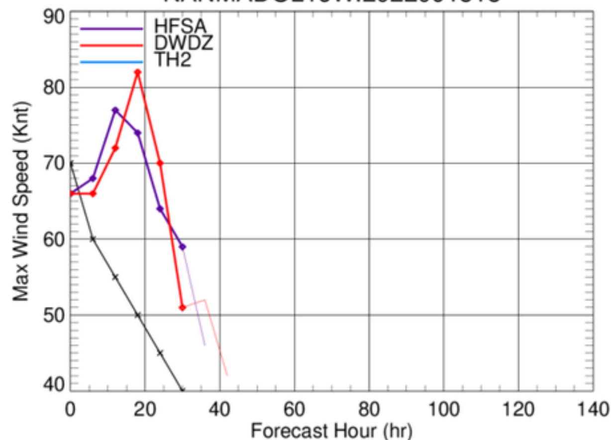
NANMADOL16W.2022091818
