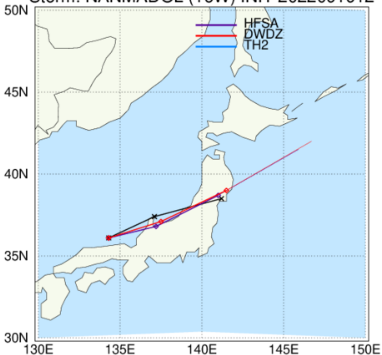
HAFS: TC Tracks Storm: NANMADOL (16W) INIT 2022091912
