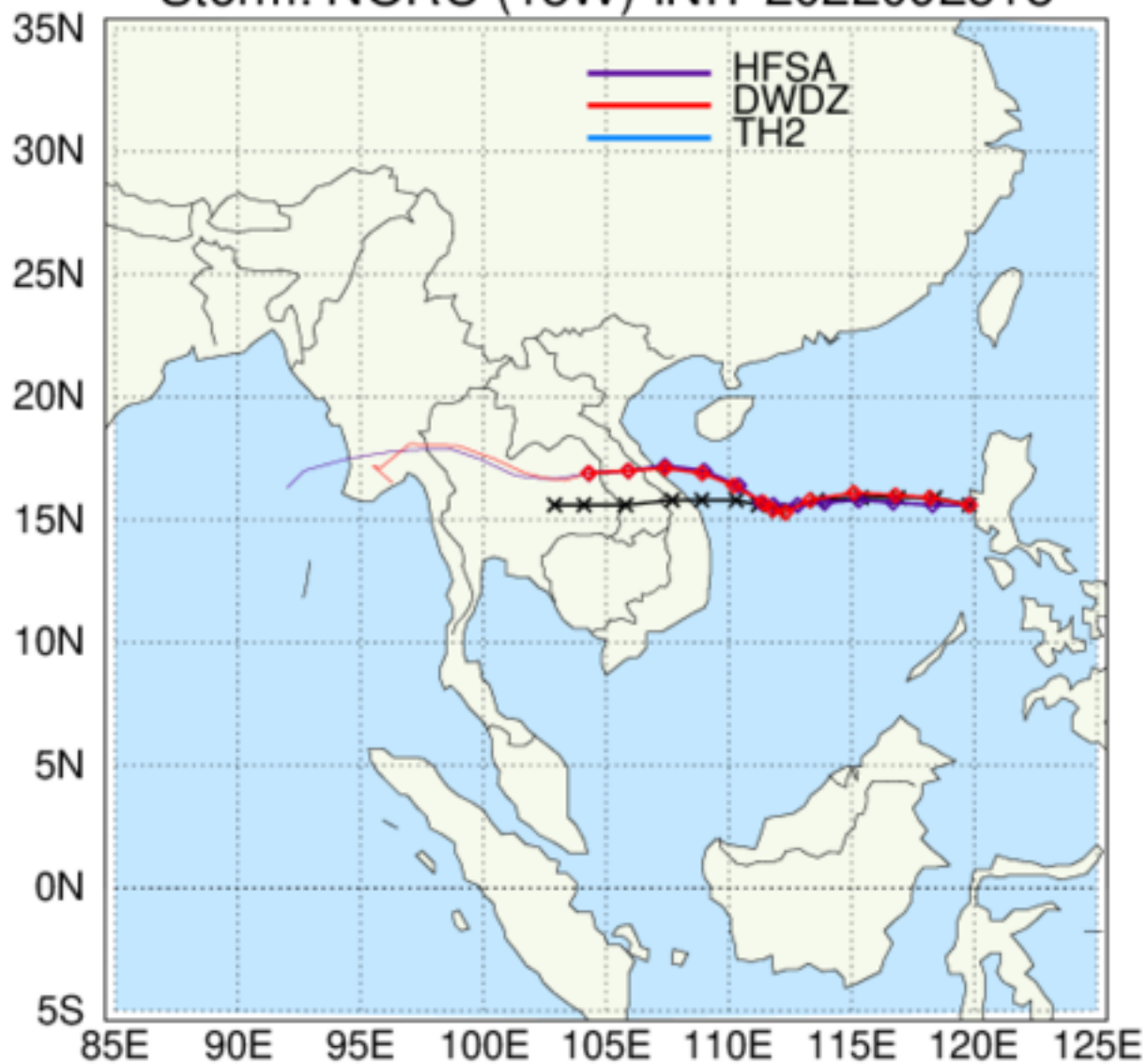
HAFS: TC Tracks Storm: NORU (18W) INIT 2022092518
