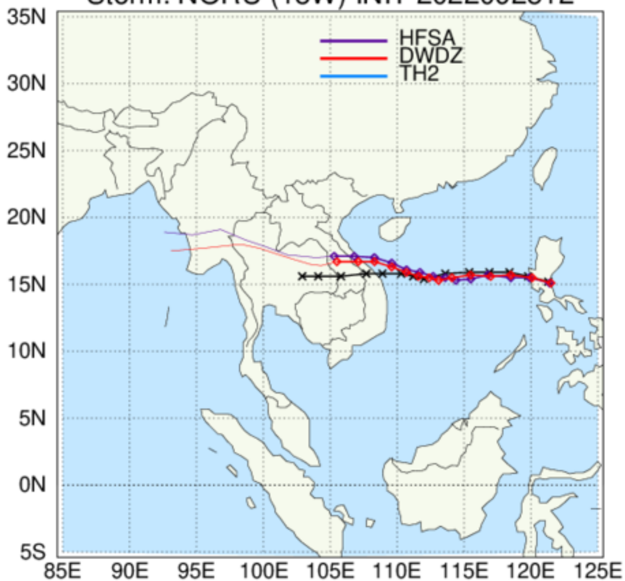
HAFS: TC Tracks Storm: NORU (18W) INIT 2022092512
