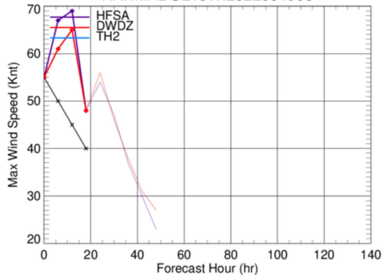
NANMADOL16W.2022091906
