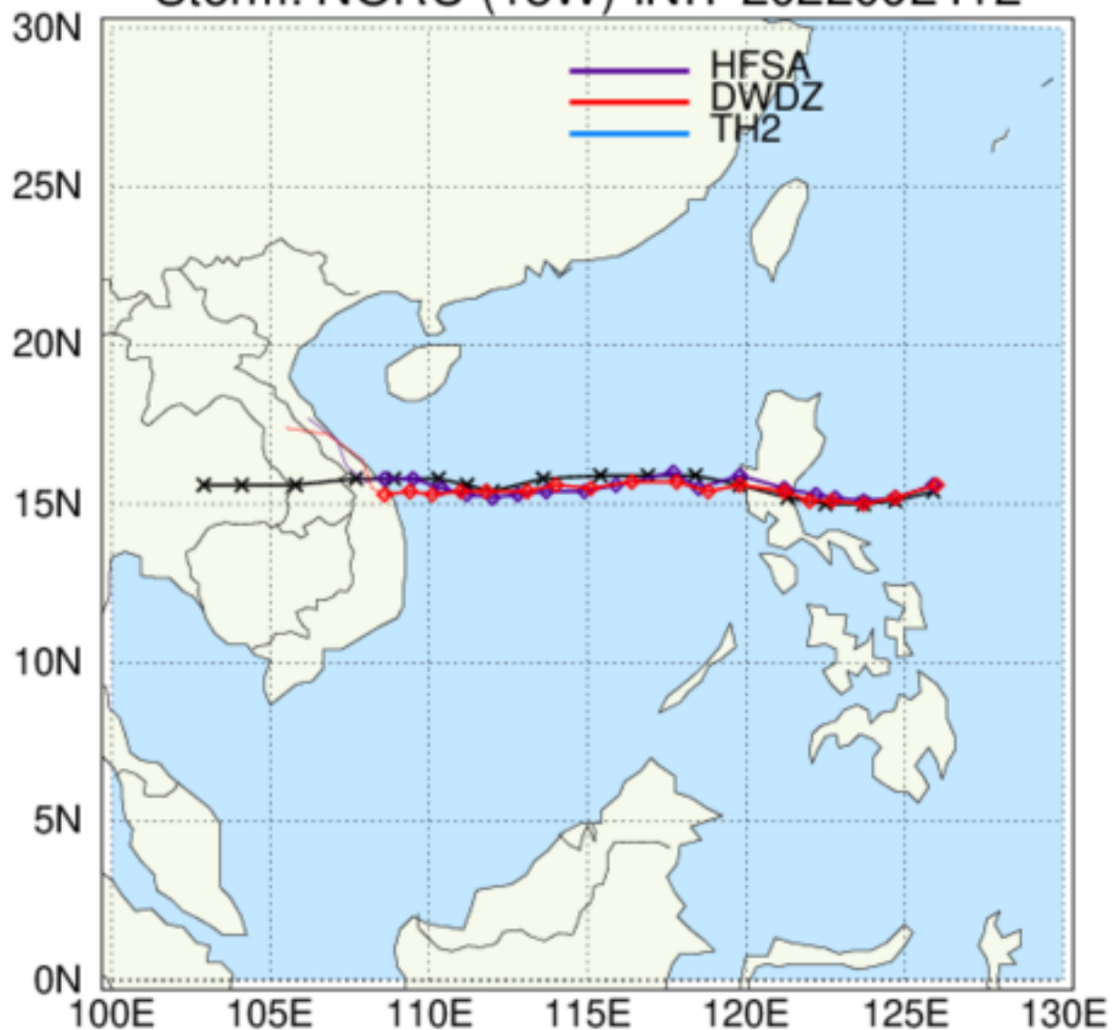
HAFS: TC Tracks Storm: NORU (18W) INIT 2022092412
