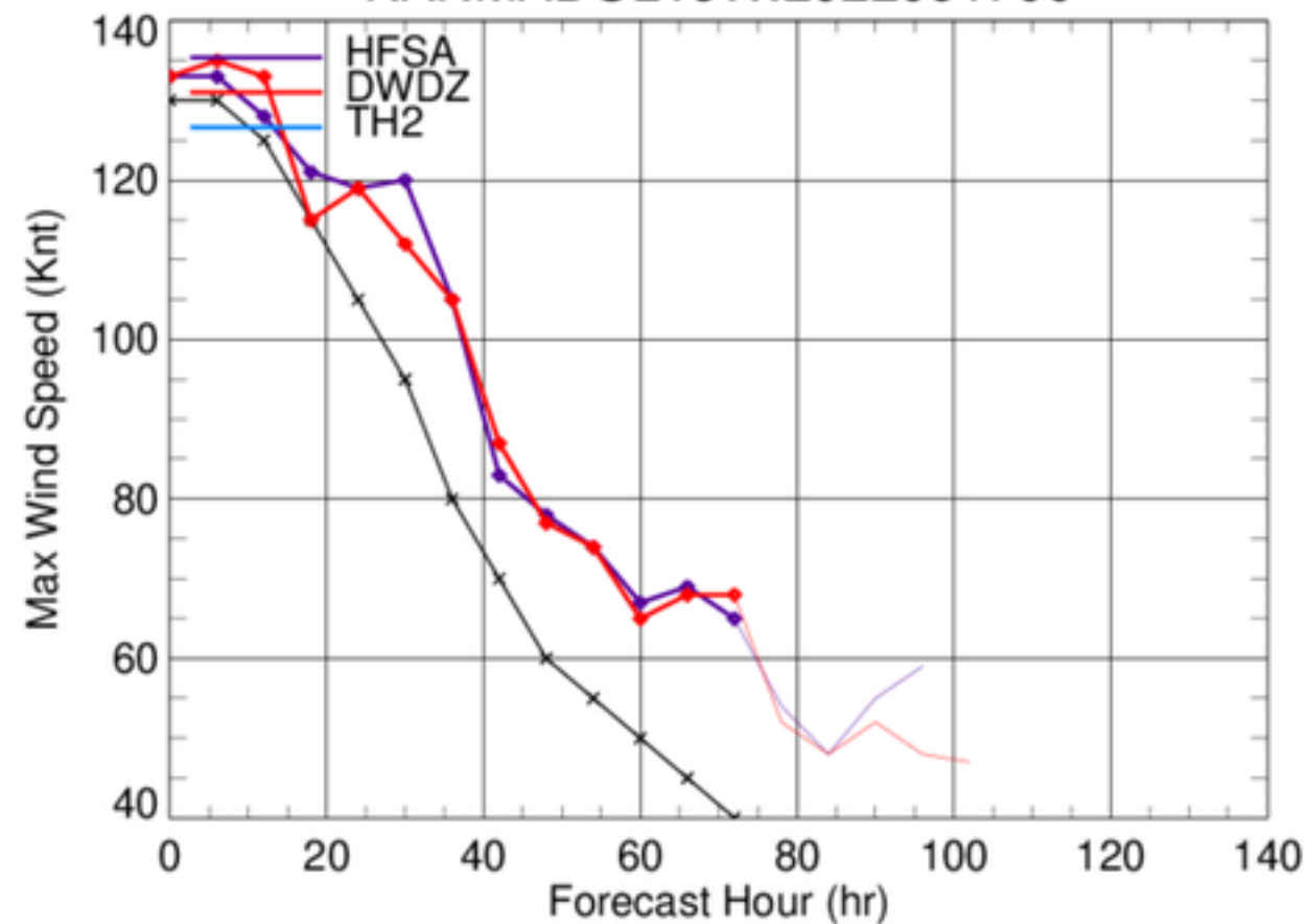
NANMADOL16W.2022091700
