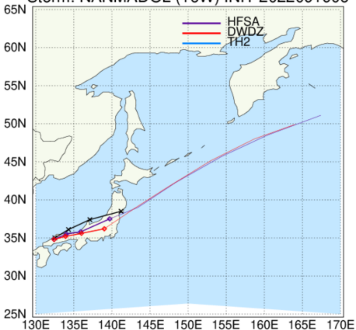
HAFS: TC Tracks Storm: NANMADOL (16W) INIT 2022091906
