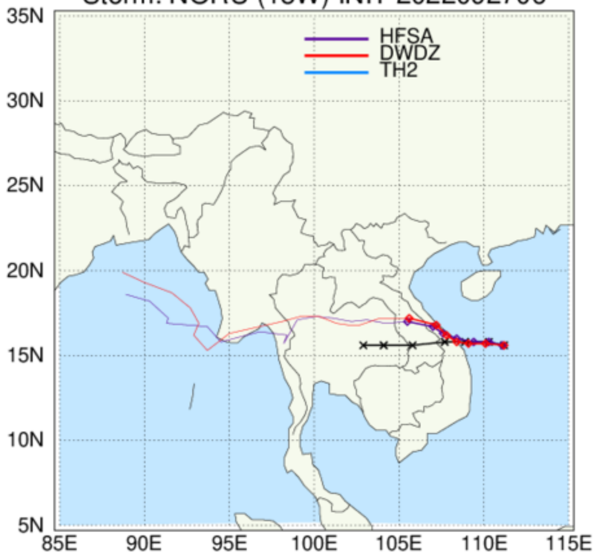
HAFS: TC Tracks Storm: NORU (18W) INIT 2022092706
