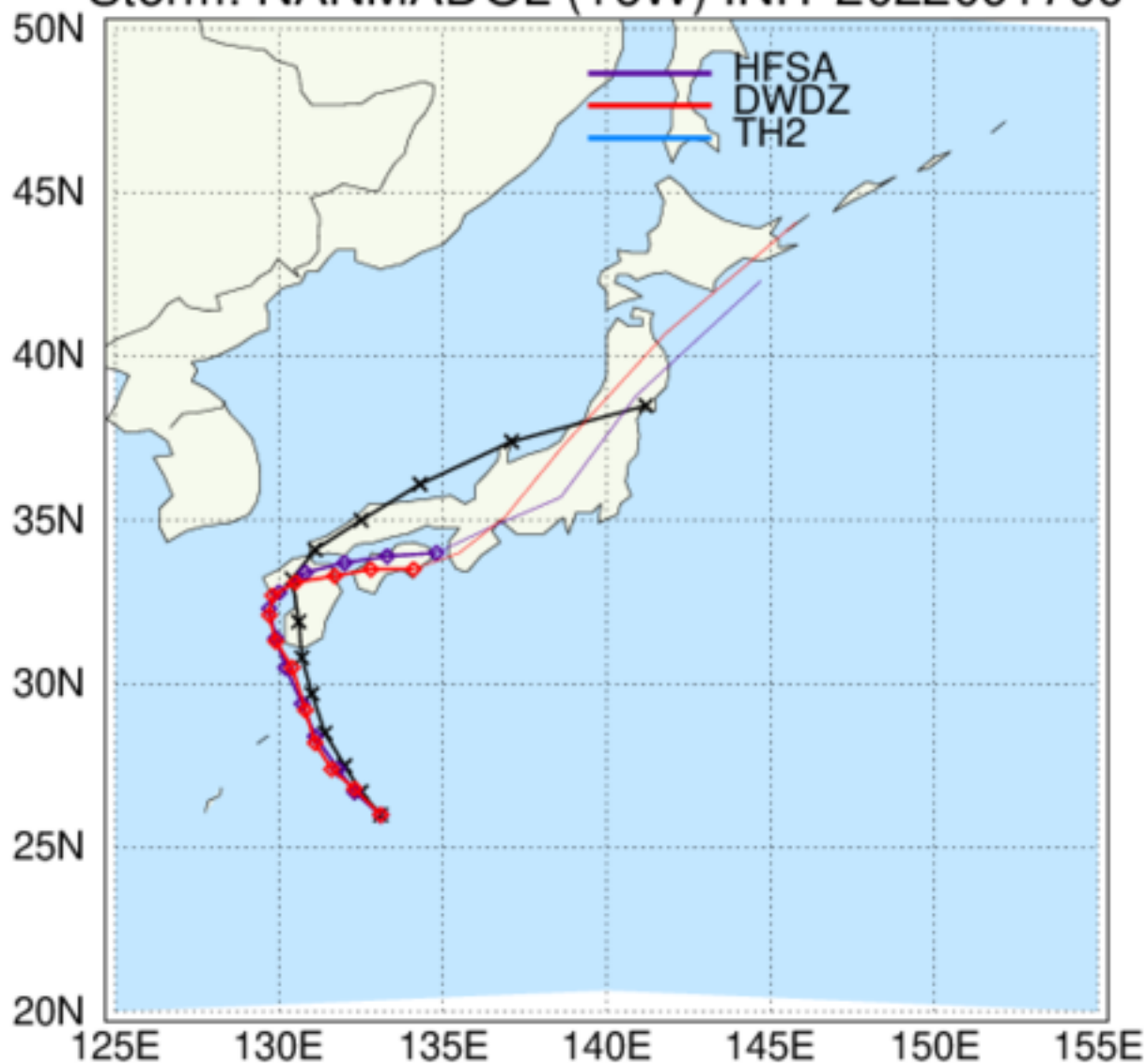
HAFS: TC Tracks Storm: NANMADOL (16W) INIT 2022091700
