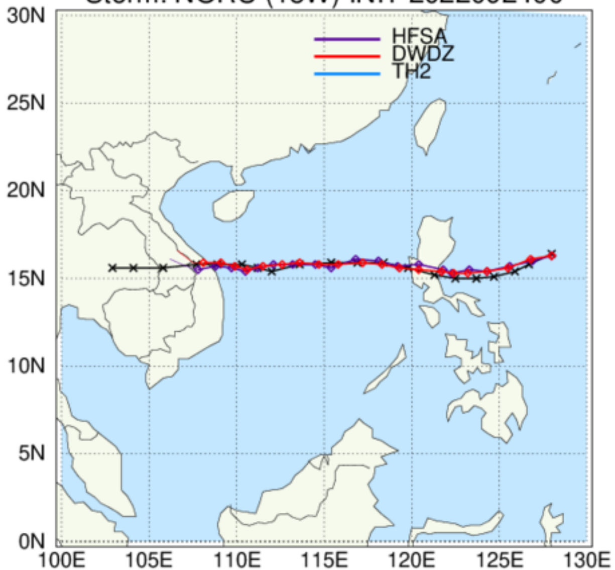
HAFS: TC Tracks Storm: NORU (18W) INIT 2022092400
