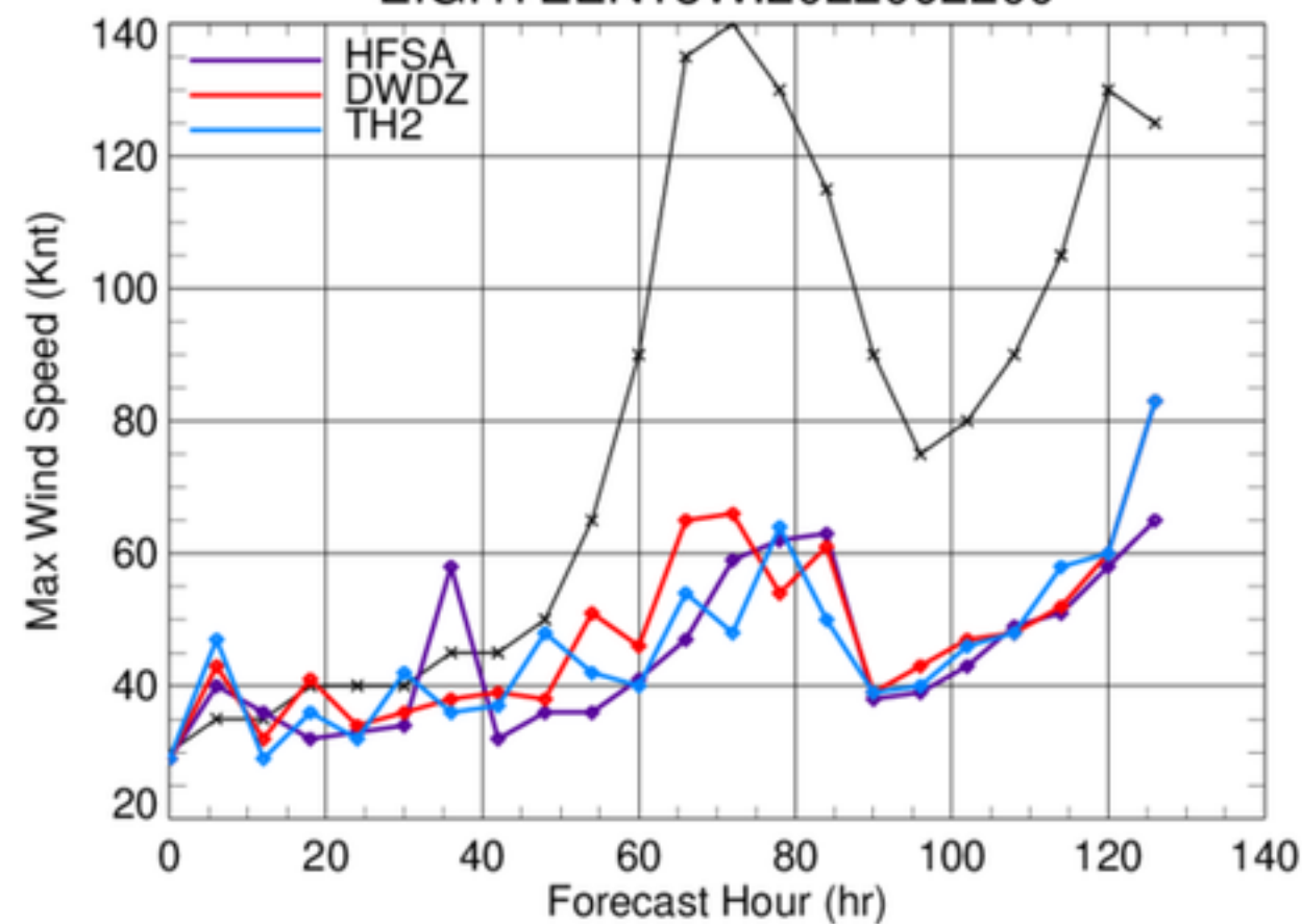
EIGHTEEN18W.2022092200
