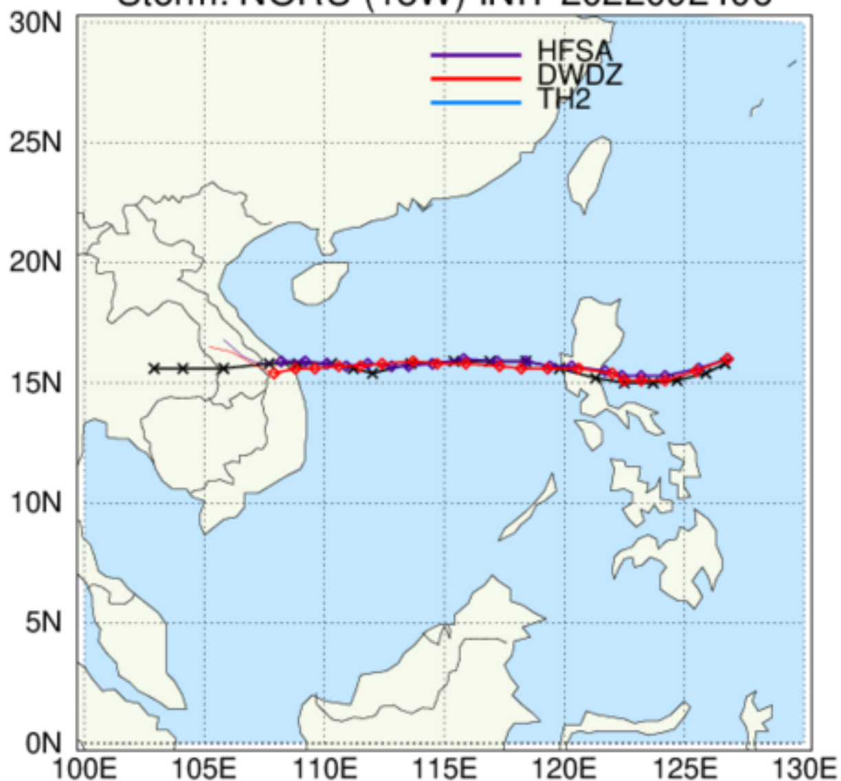
HAFS: TC Tracks Storm: NORU (18W) INIT 2022092406
