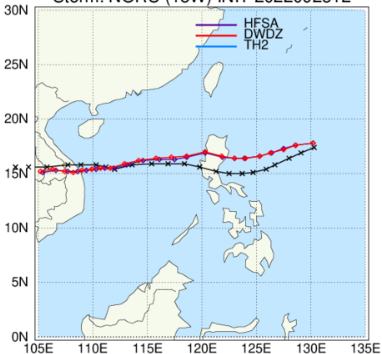
HAFS: TC Tracks Storm: NORU (18W) INIT 2022092312
