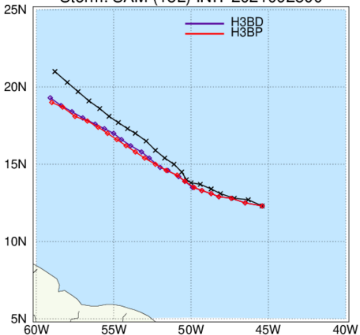
HAFS: TC Tracks Storm: SAM (18L) INIT 2021092500
