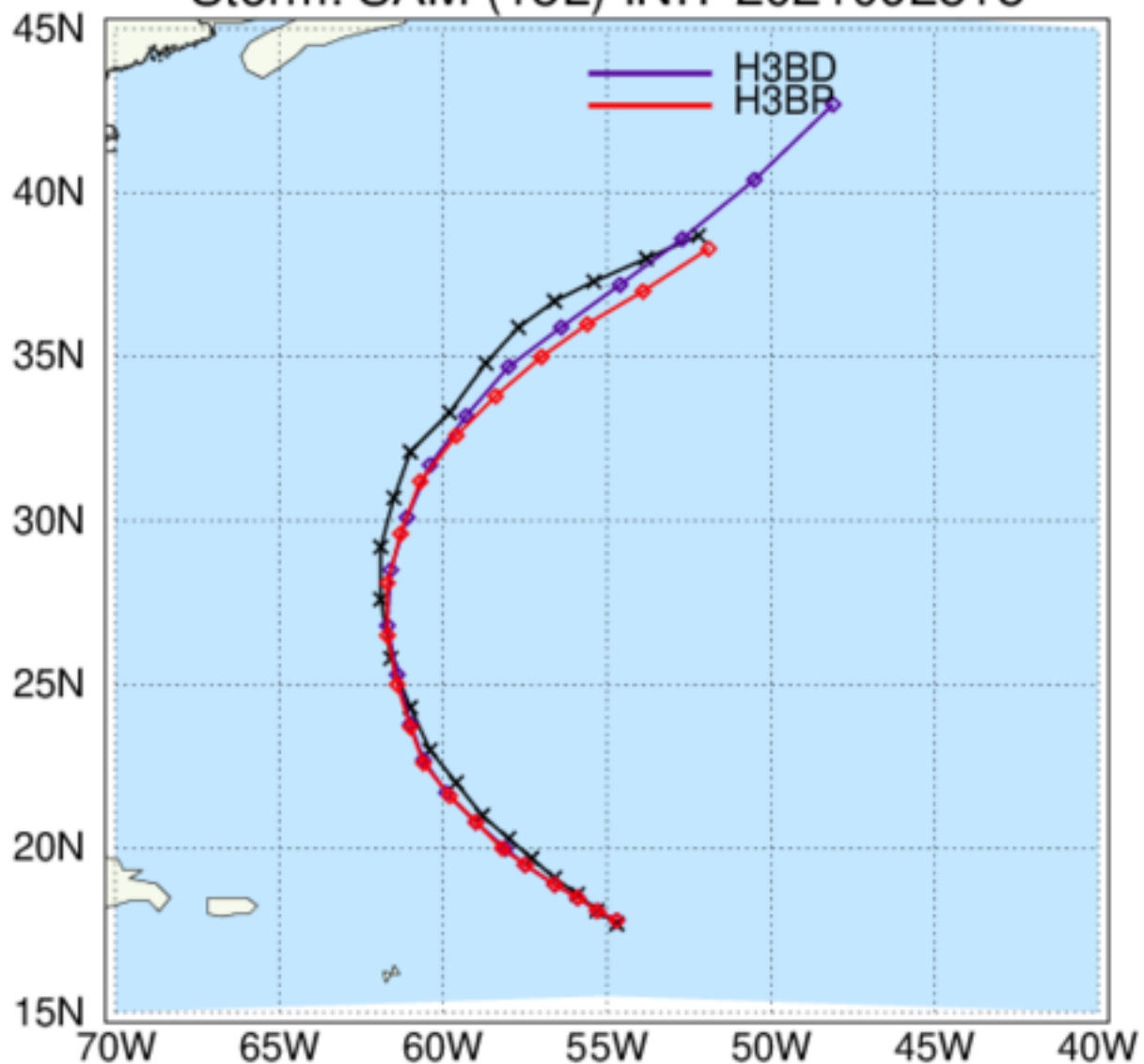
HAFS: TC Tracks Storm: SAM (18L) INIT 2021092818
