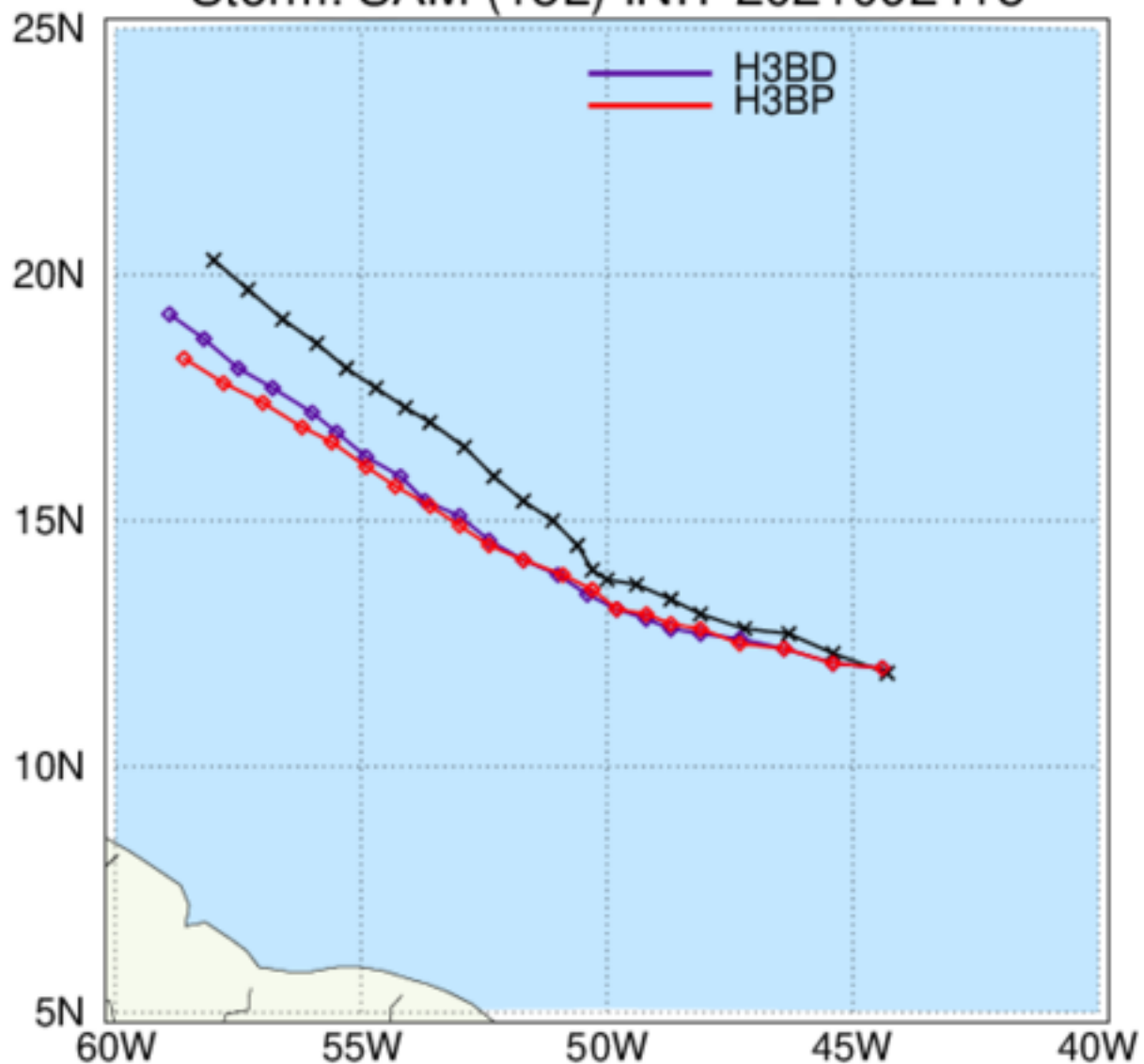
HAFS: TC Tracks Storm: SAM (18L) INIT 2021092418
