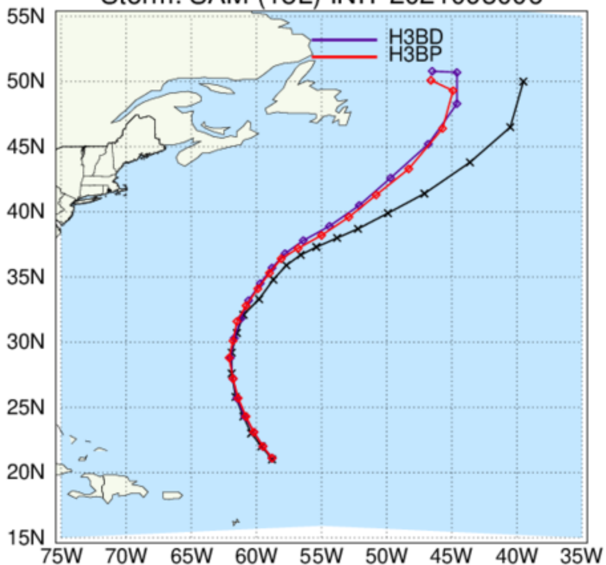
HAFS: TC Tracks Storm: SAM (18L) INIT 2021093006
