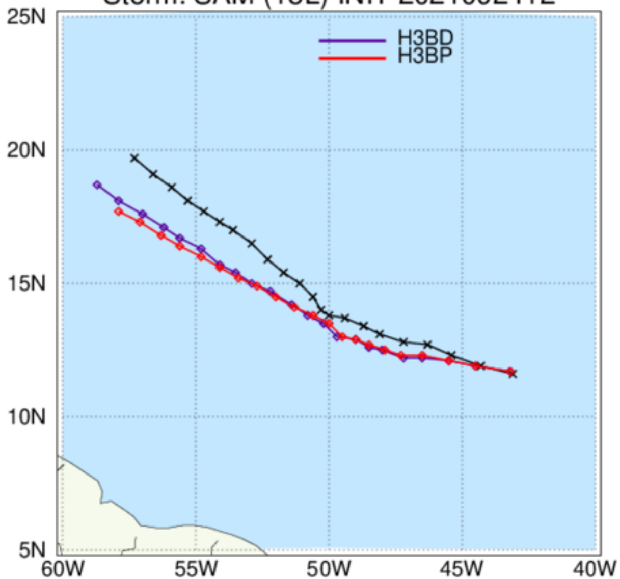
HAFS: TC Tracks Storm: SAM (18L) INIT 2021092412
