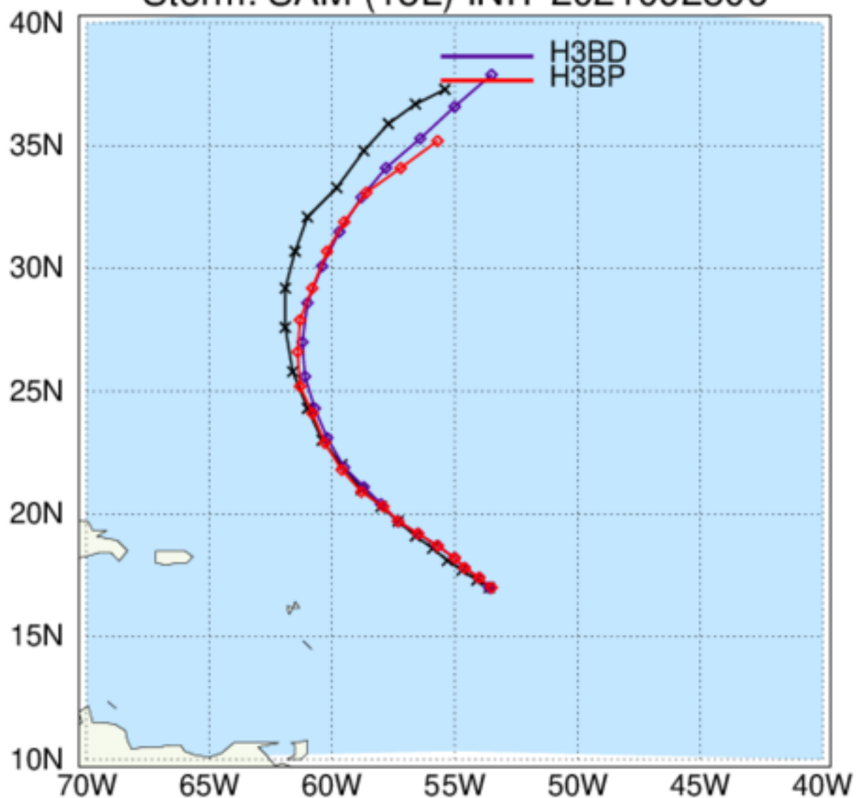
HAFS: TC Tracks Storm: SAM (18L) INIT 2021092806
