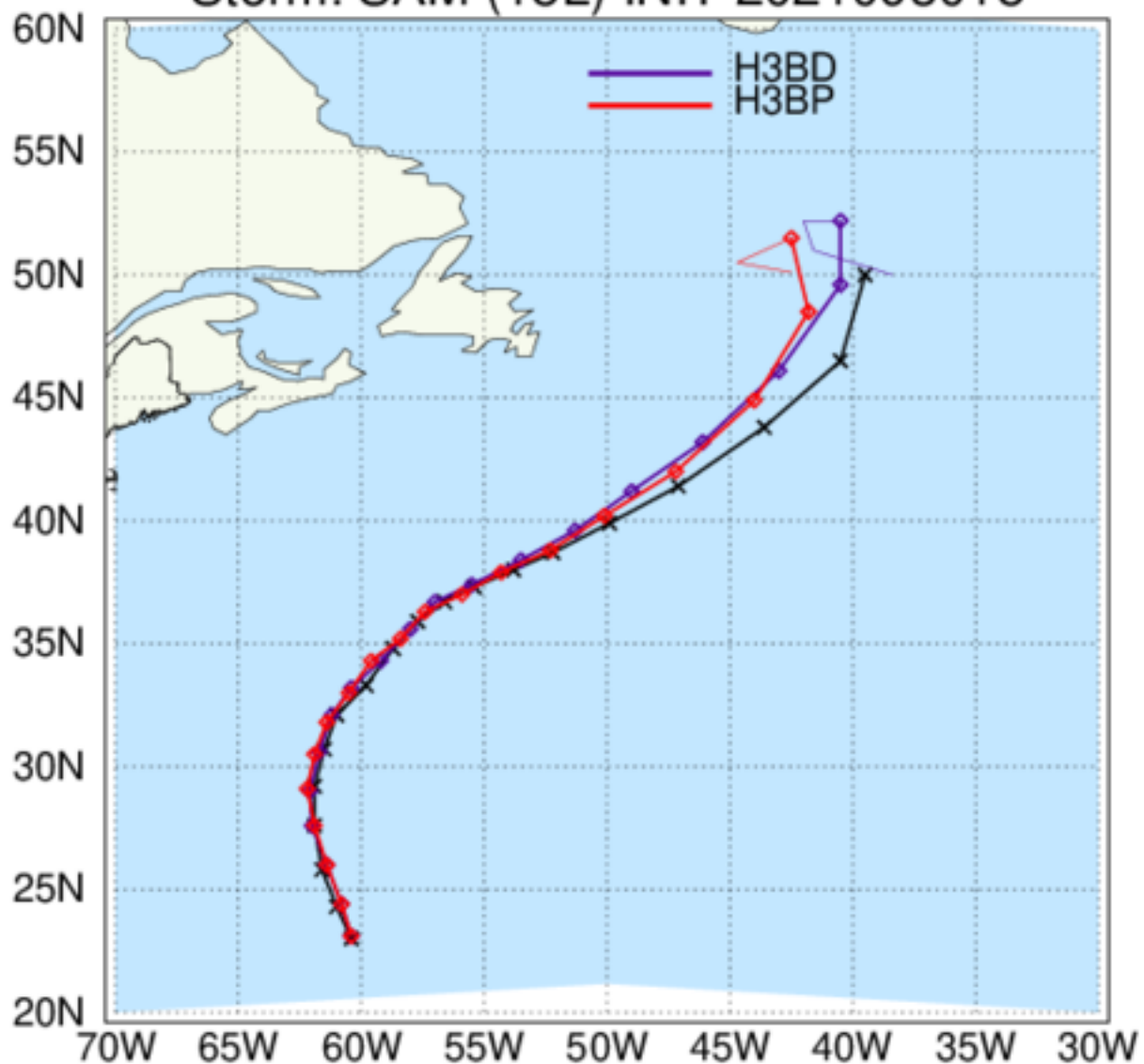
HAFS: TC Tracks Storm: SAM (18L) INIT 2021093018
