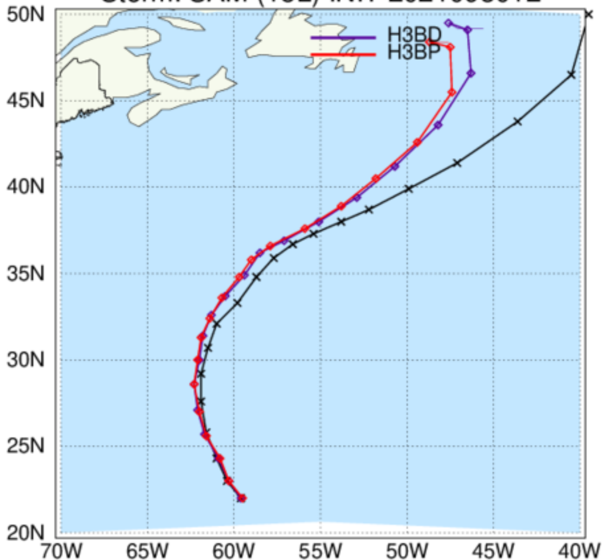
HAFS: TC Tracks Storm: SAM (18L) INIT 2021093012
