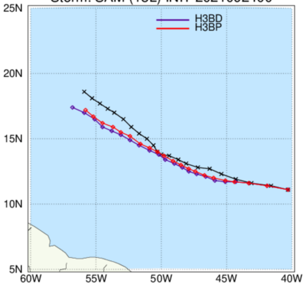
HAFS: TC Tracks Storm: SAM (18L) INIT 2021092400
