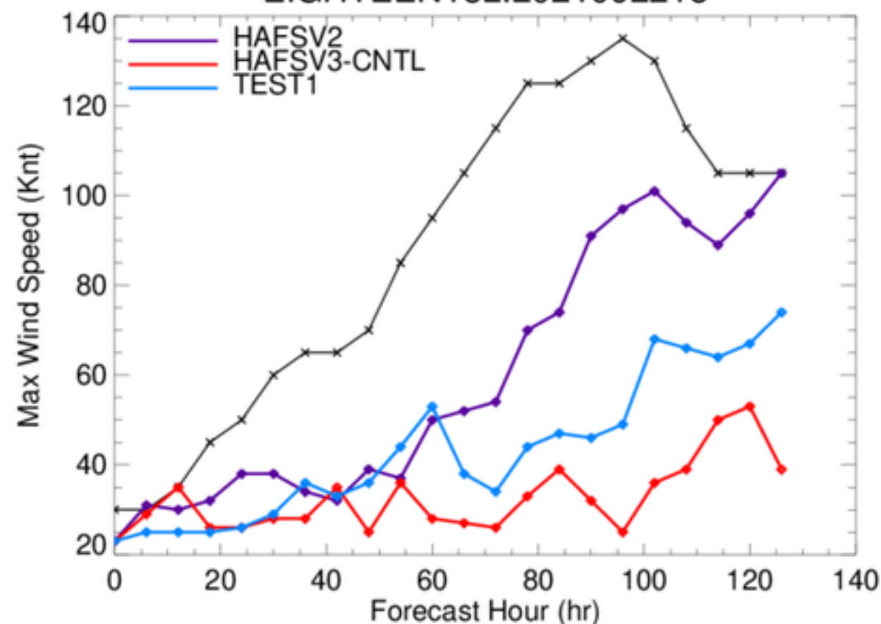
EIGHTEEN18L.2021092218
