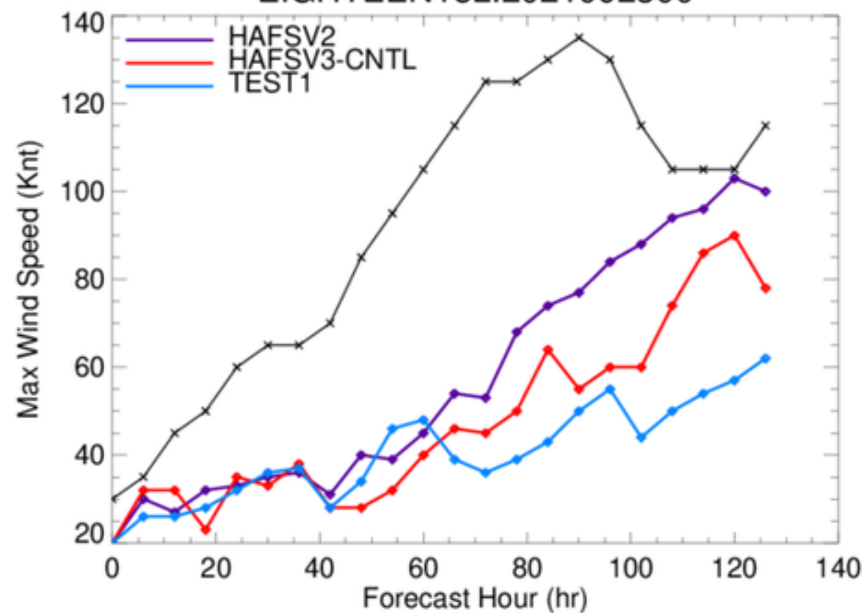
EIGHTEEN18L.2021092300
