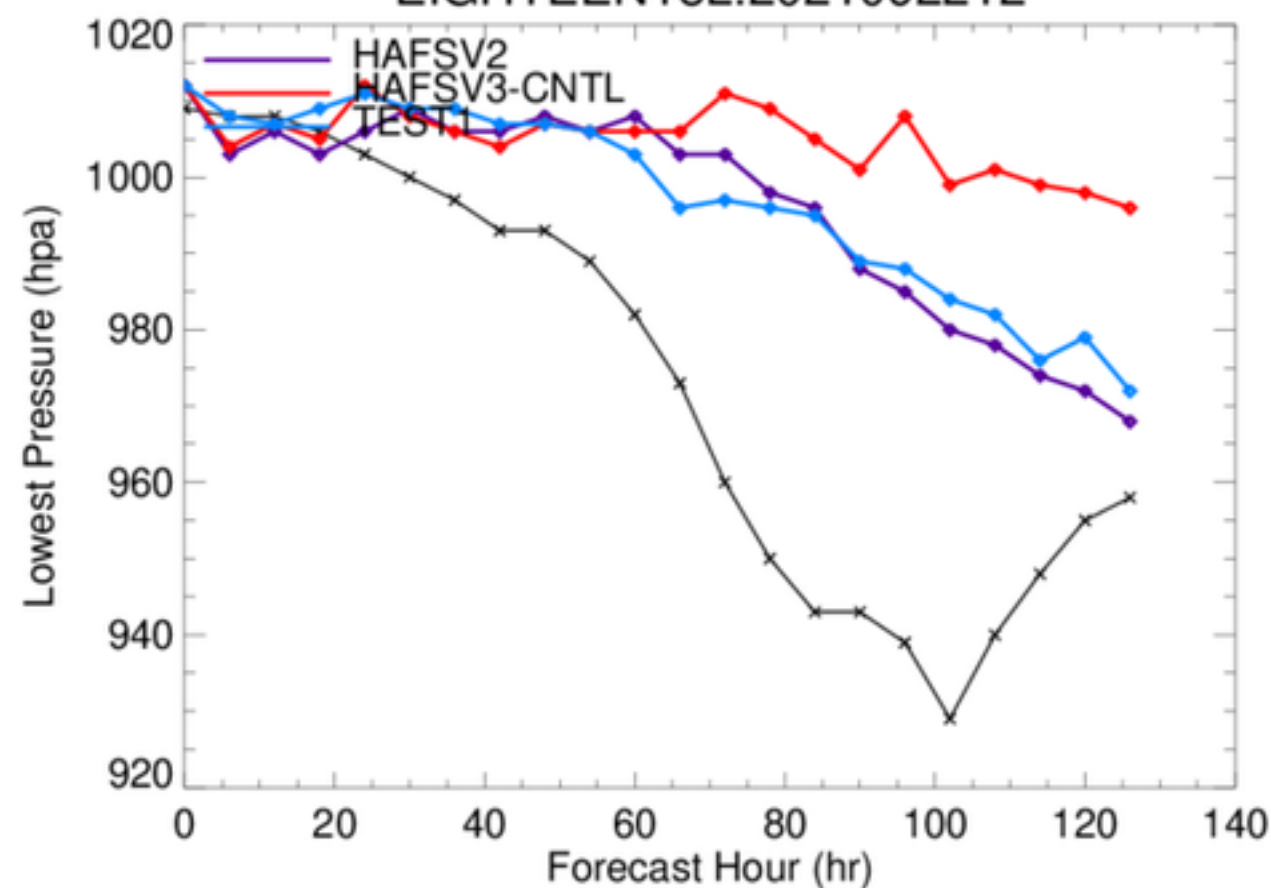
EIGHTEEN18L.2021092212
