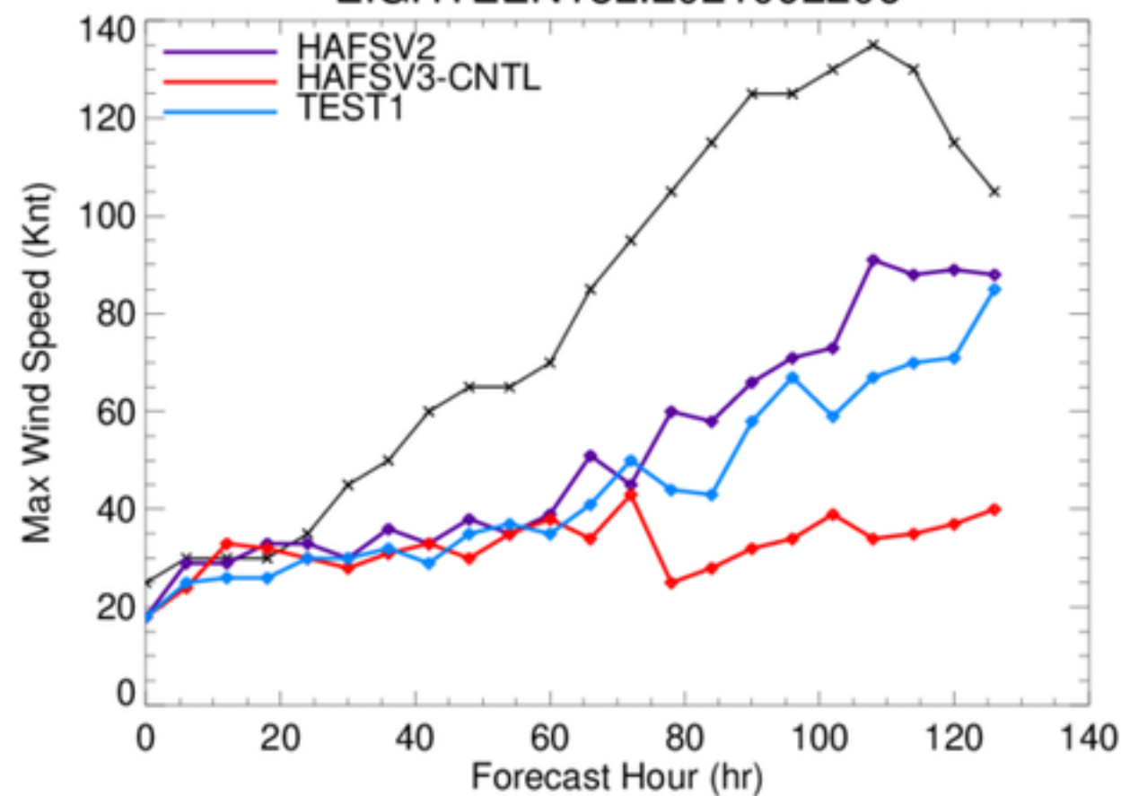
EIGHTEEN18L.2021092206
