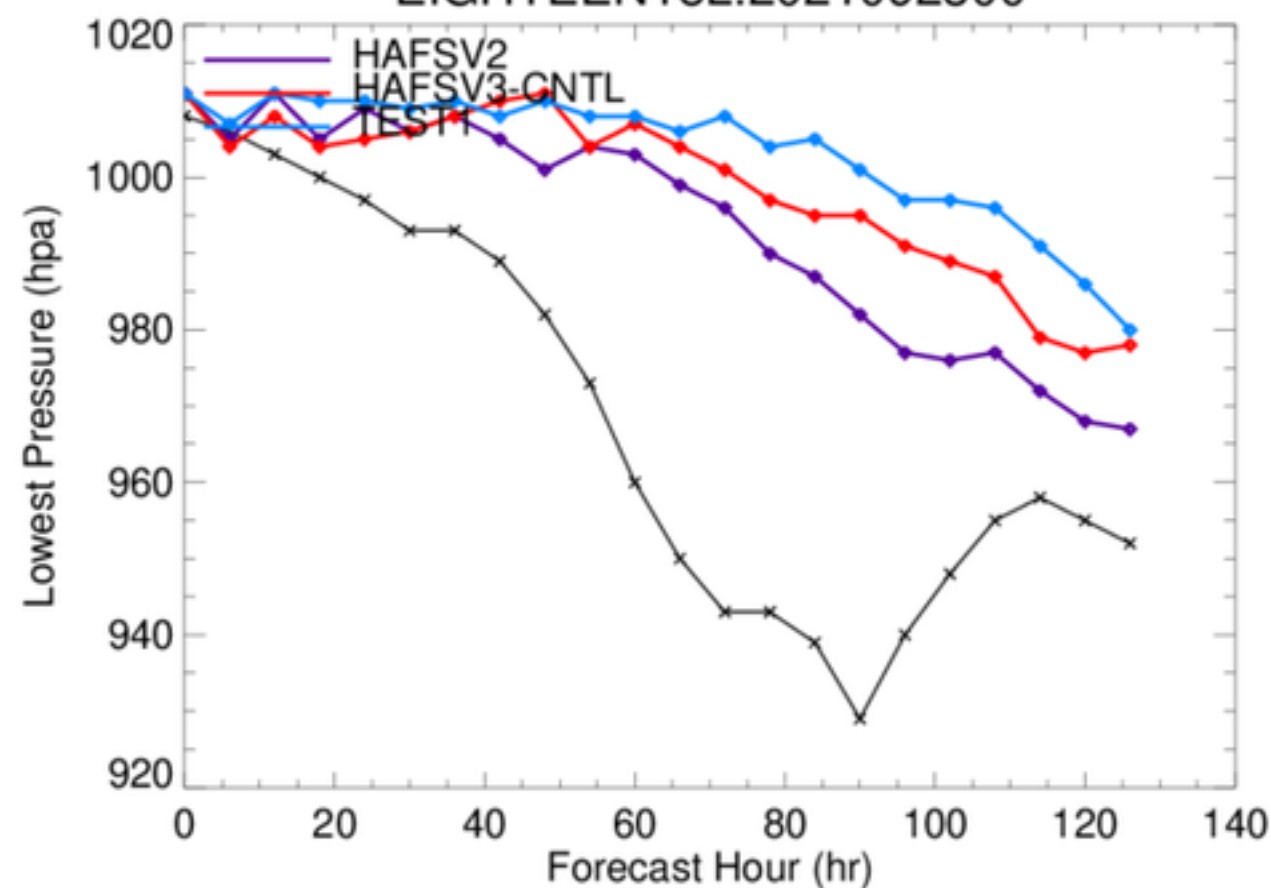
EIGHTEEN18L.2021092300
