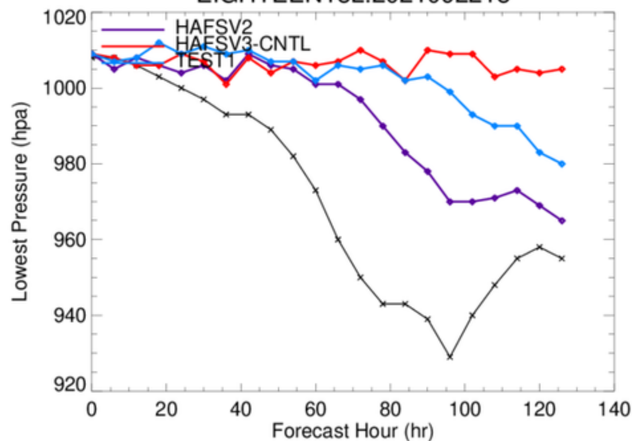
EIGHTEEN18L.2021092218
