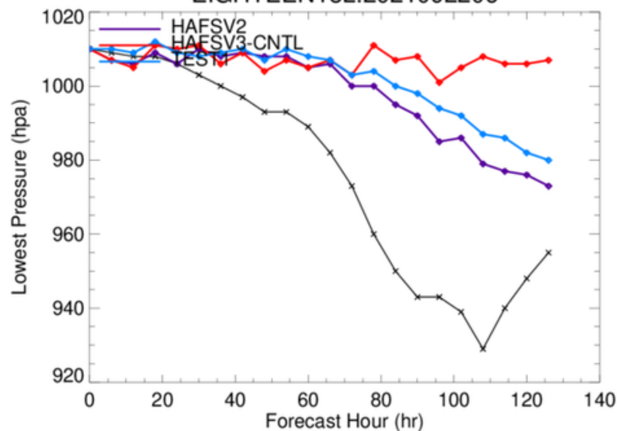
EIGHTEEN18L.2021092206
