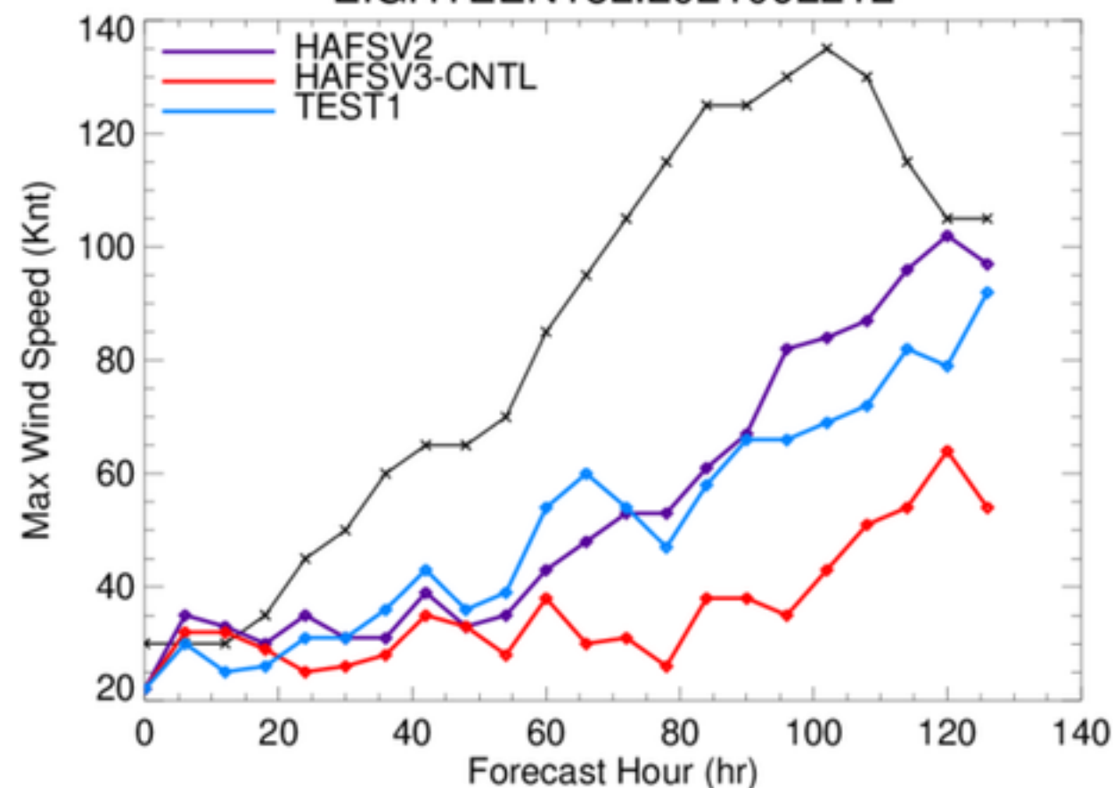
EIGHTEEN18L.2021092212
