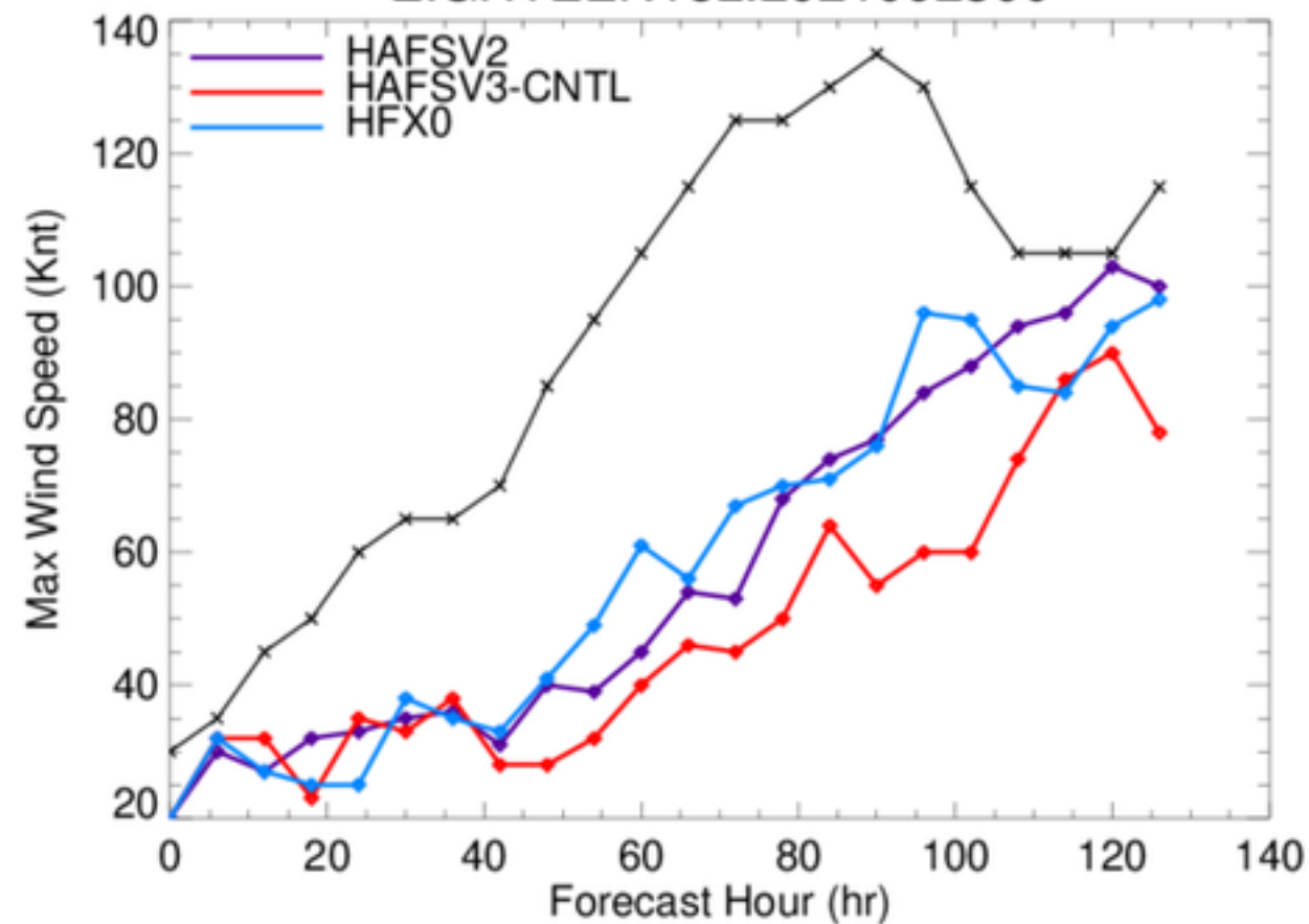
EIGHTEEN18L.2021092300
