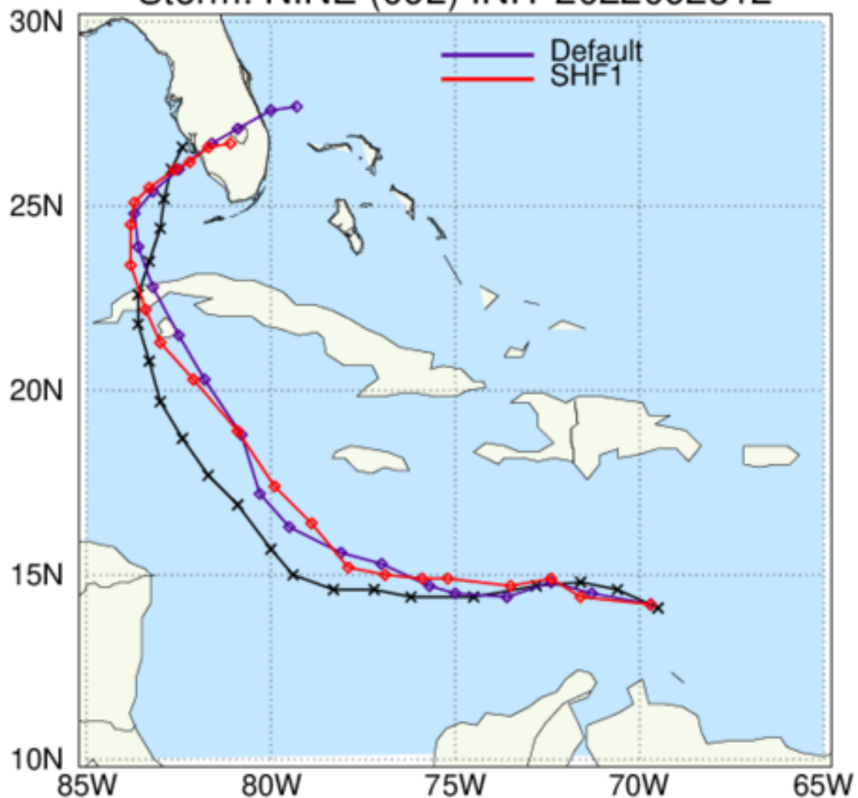
HAFS: TC Tracks Storm: NINE (09L) INIT 2022092312
