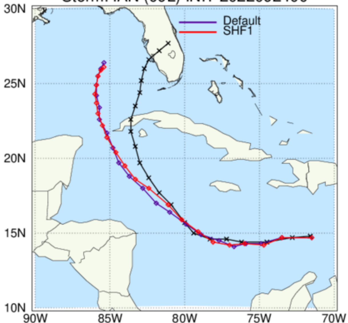
HAFS: TC Tracks Storm: IAN (09L) INIT 2022092400
