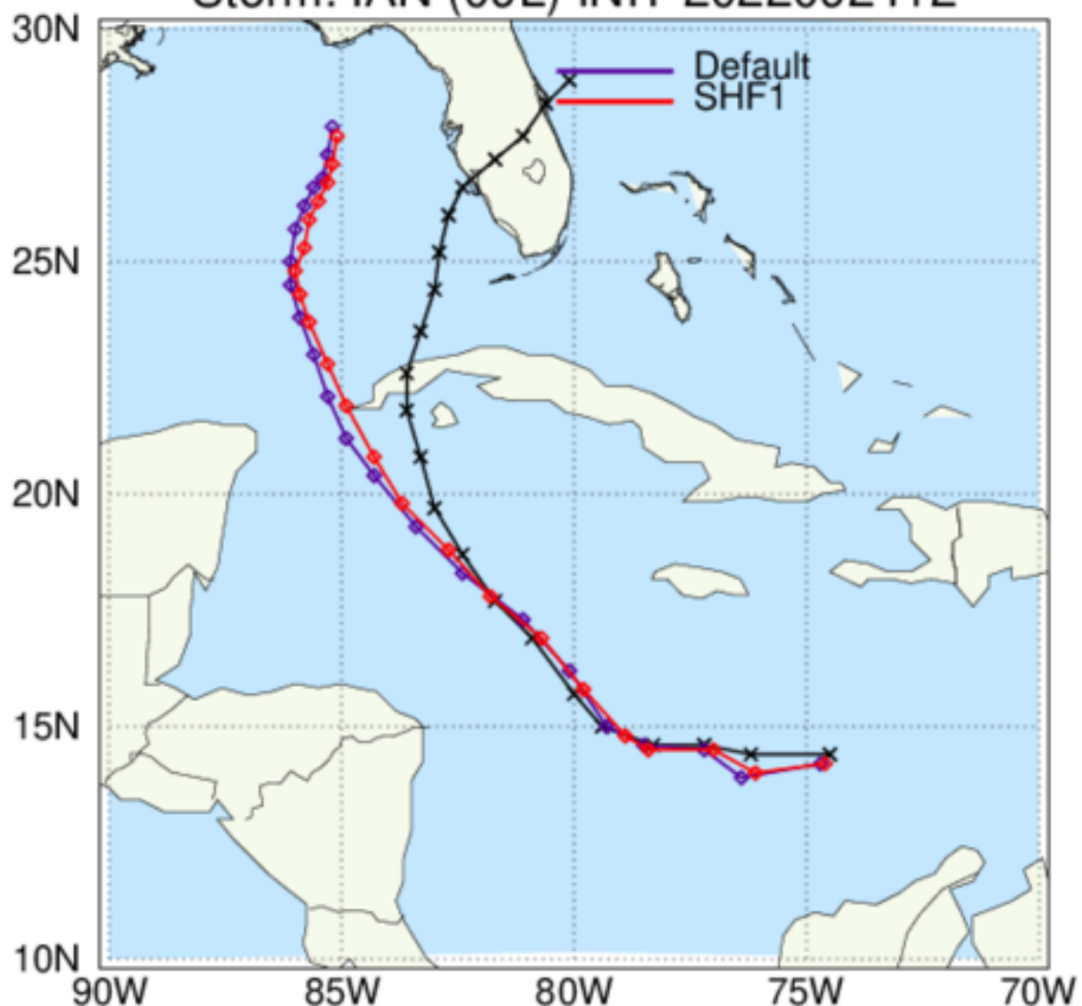
HAFS: TC Tracks Storm: IAN (09L) INIT 2022092412
