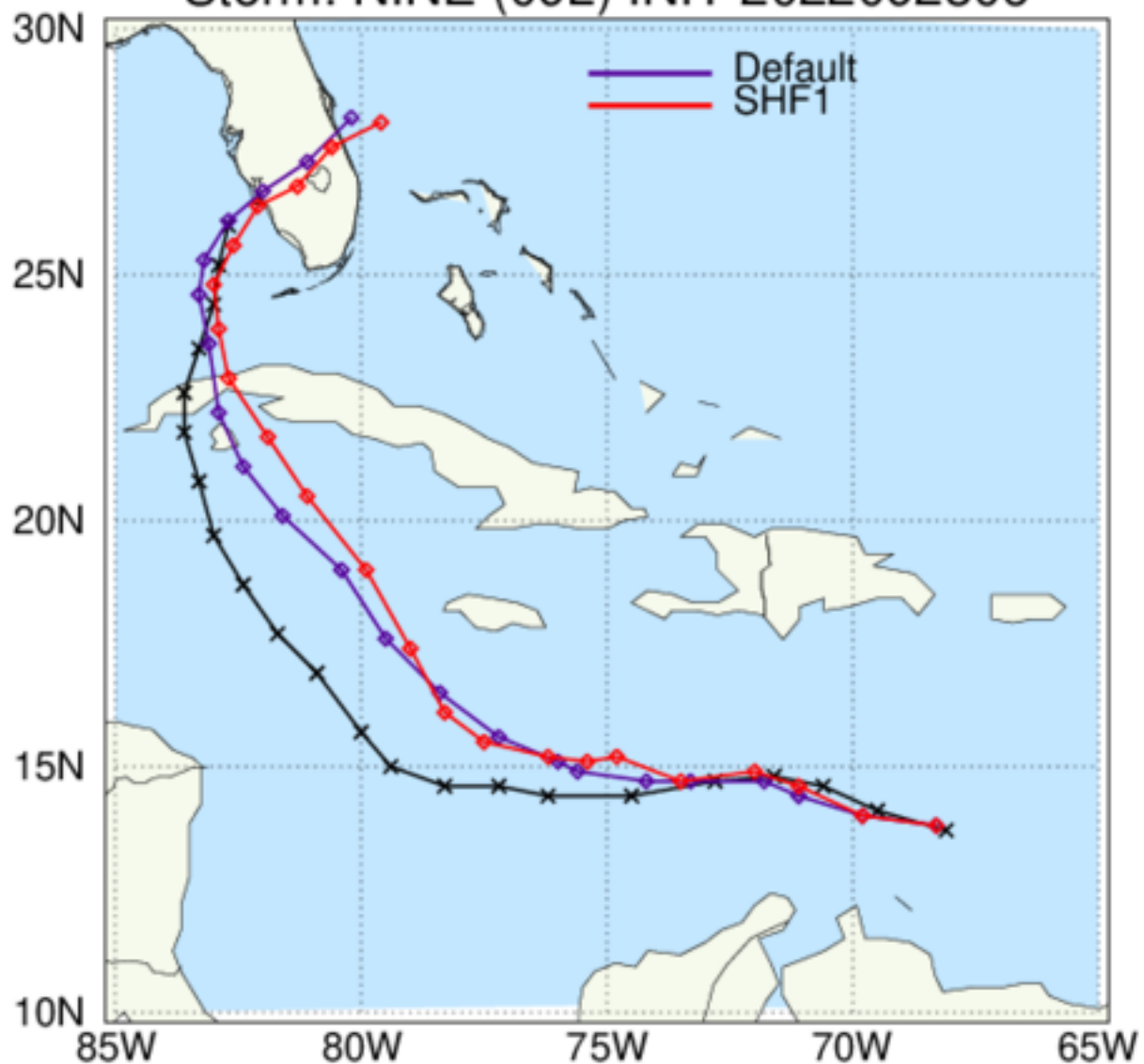
HAFS: TC Tracks Storm: NINE (09L) INIT 2022092306
