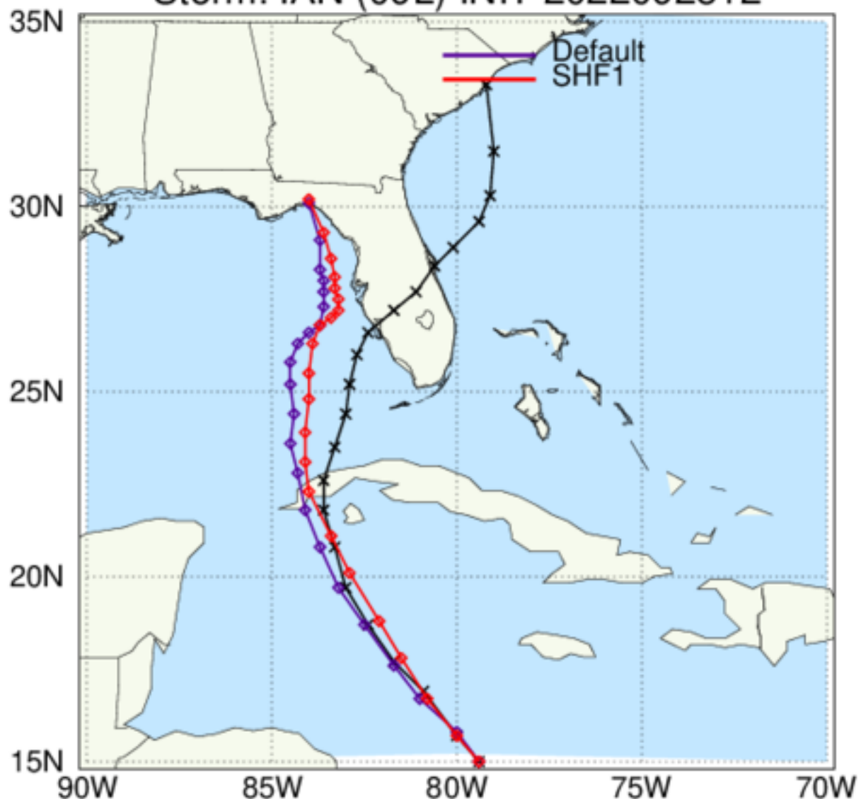
HAFS: TC Tracks Storm: IAN (09L) INIT 2022092512
