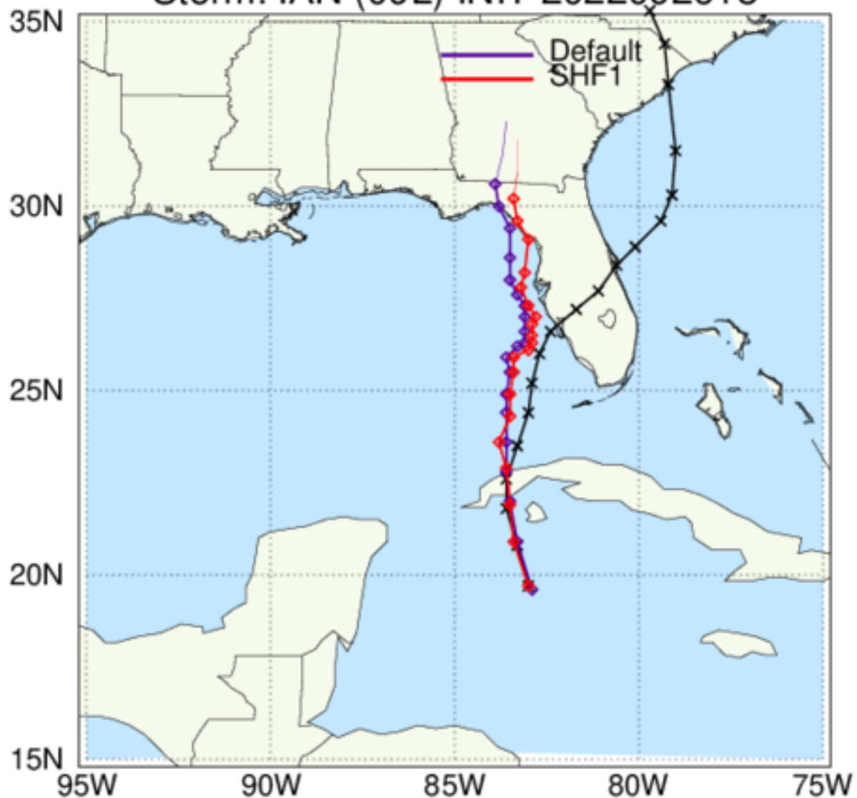
HAFS: TC Tracks Storm: IAN (09L) INIT 2022092618
