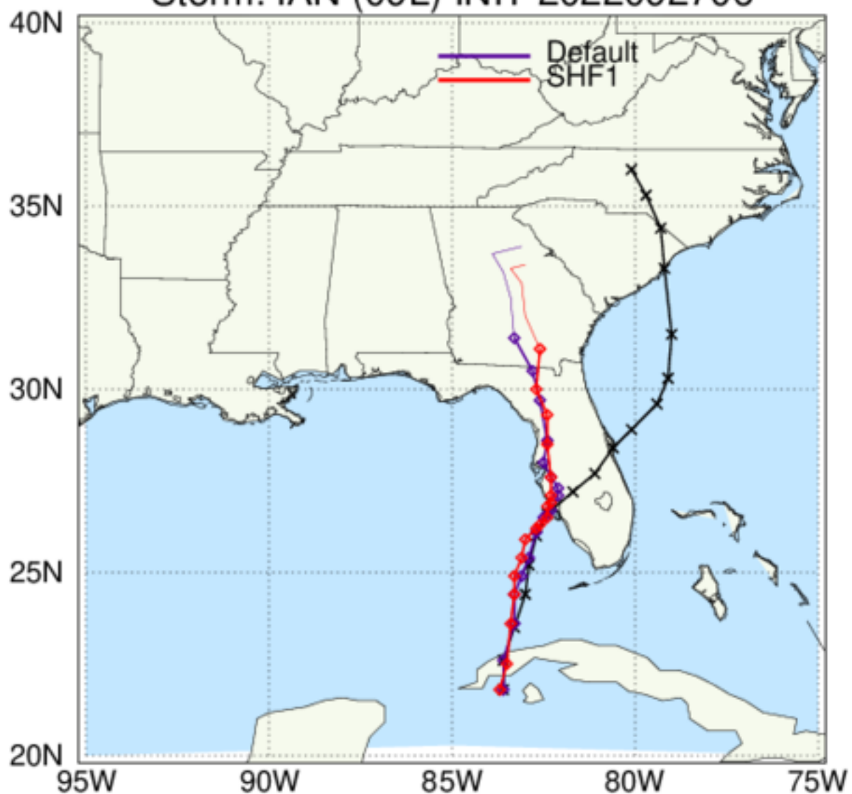
HAFS: TC Tracks Storm: IAN (09L) INIT 2022092706
