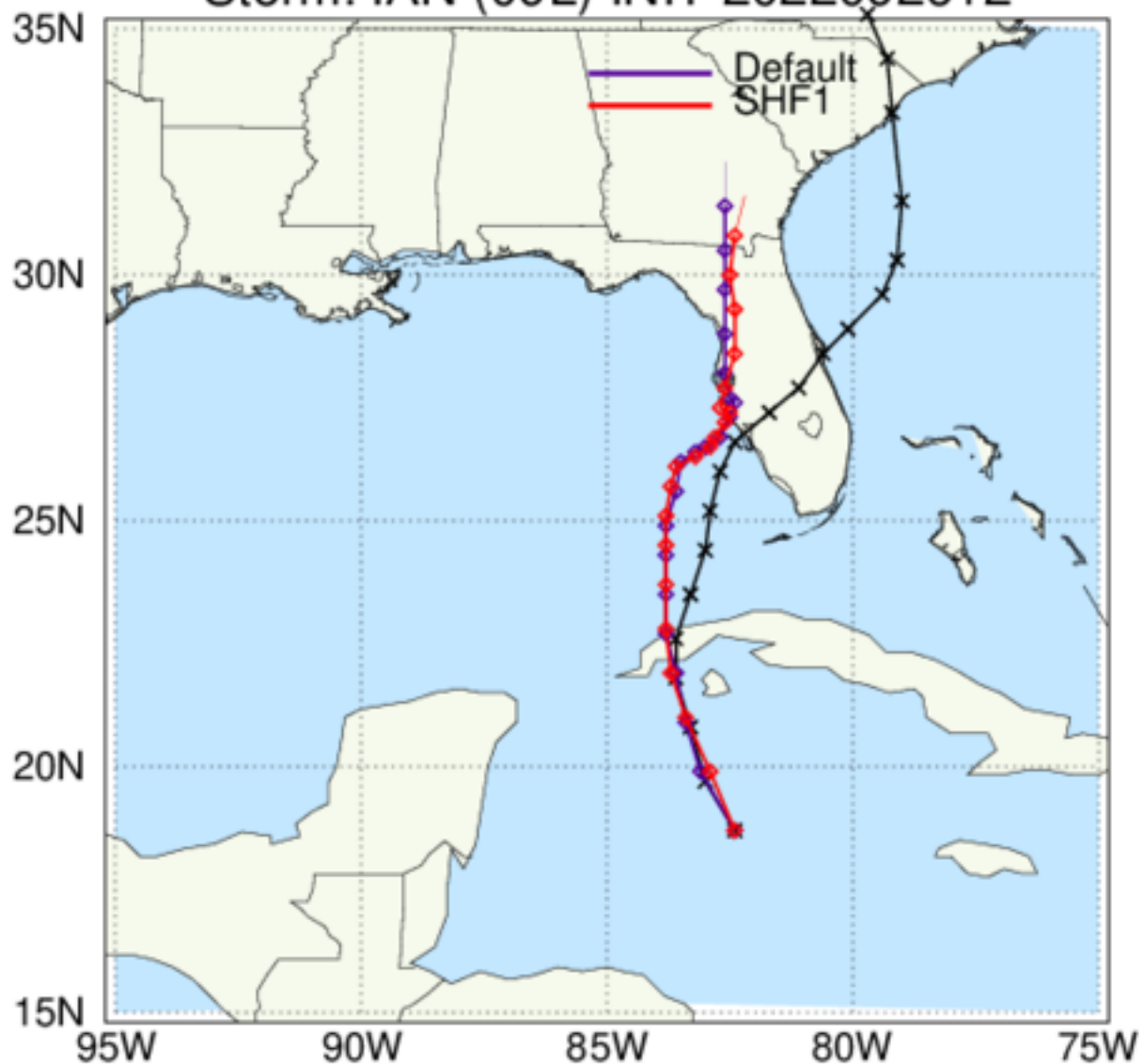
HAFS: TC Tracks Storm: IAN (09L) INIT 2022092612
