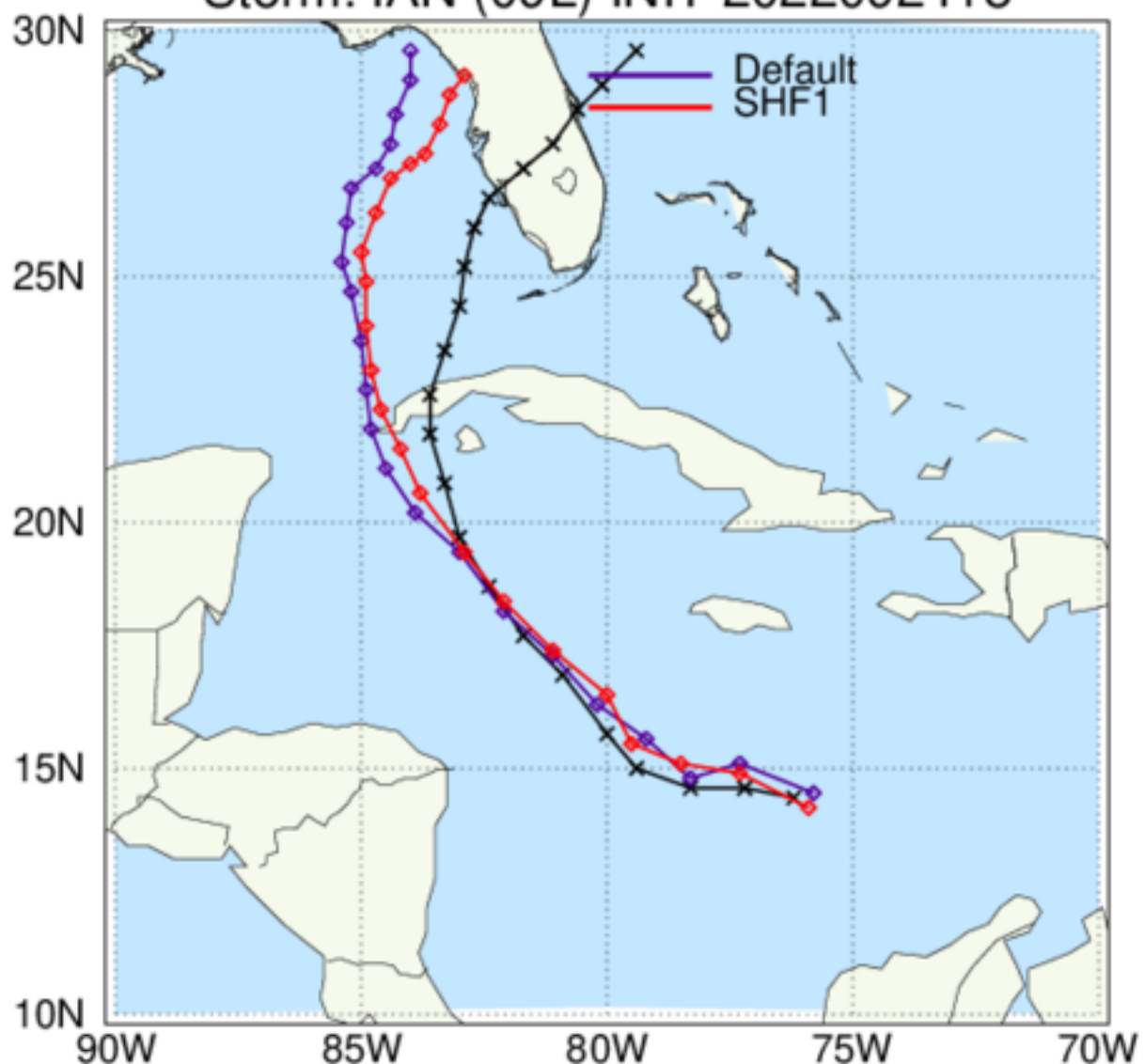
HAFS: TC Tracks Storm: IAN (09L) INIT 2022092418
