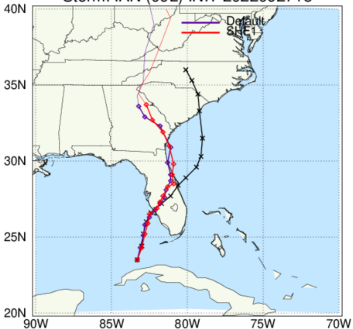
HAFS: TC Tracks Storm: IAN (09L) INIT 2022092718
