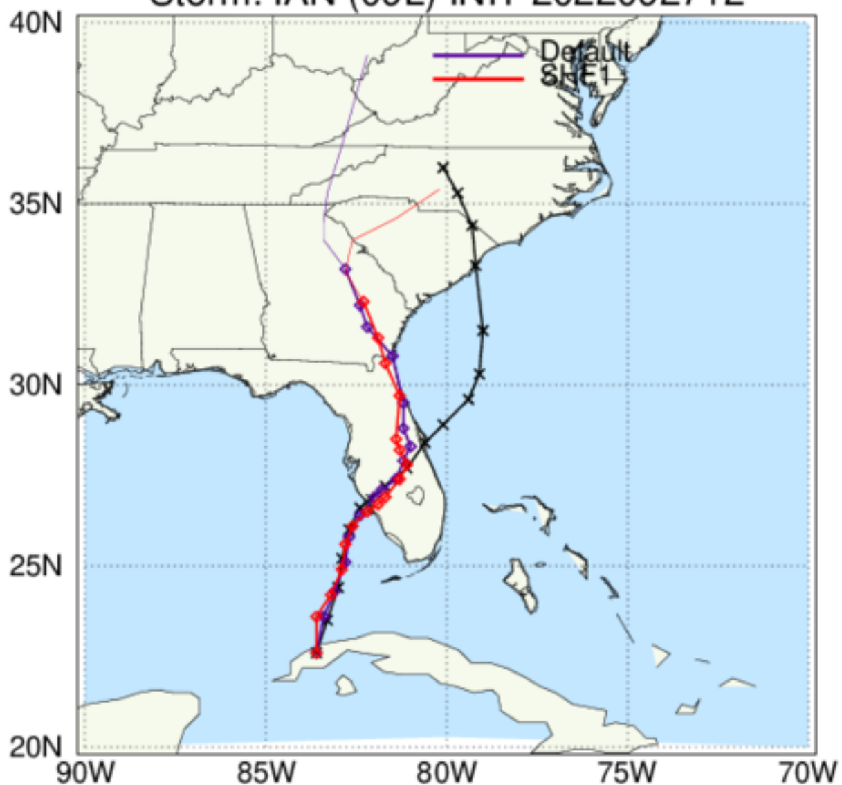
HAFS: TC Tracks Storm: IAN (09L) INIT 2022092712
