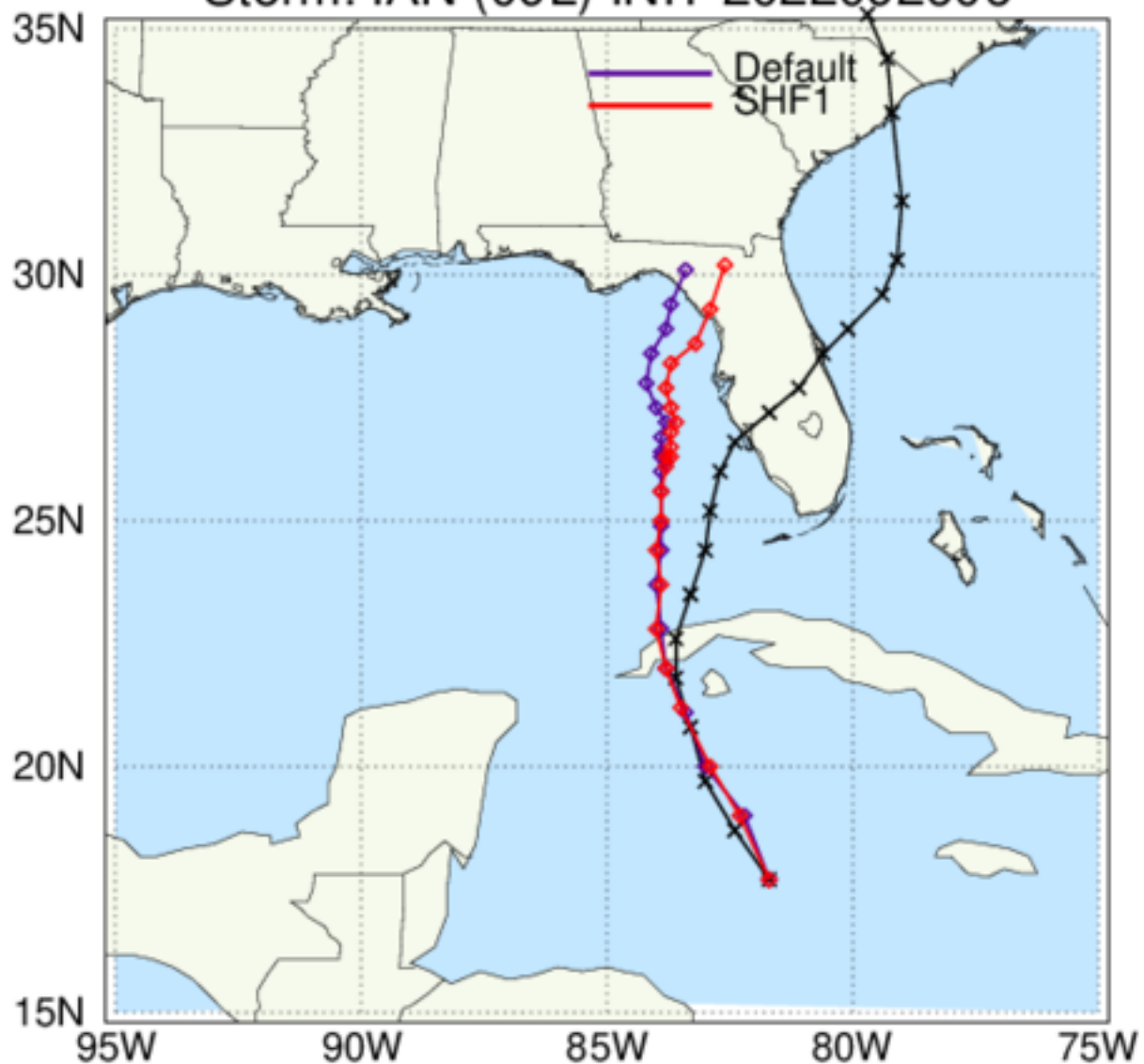
HAFS: TC Tracks Storm: IAN (09L) INIT 2022092606
