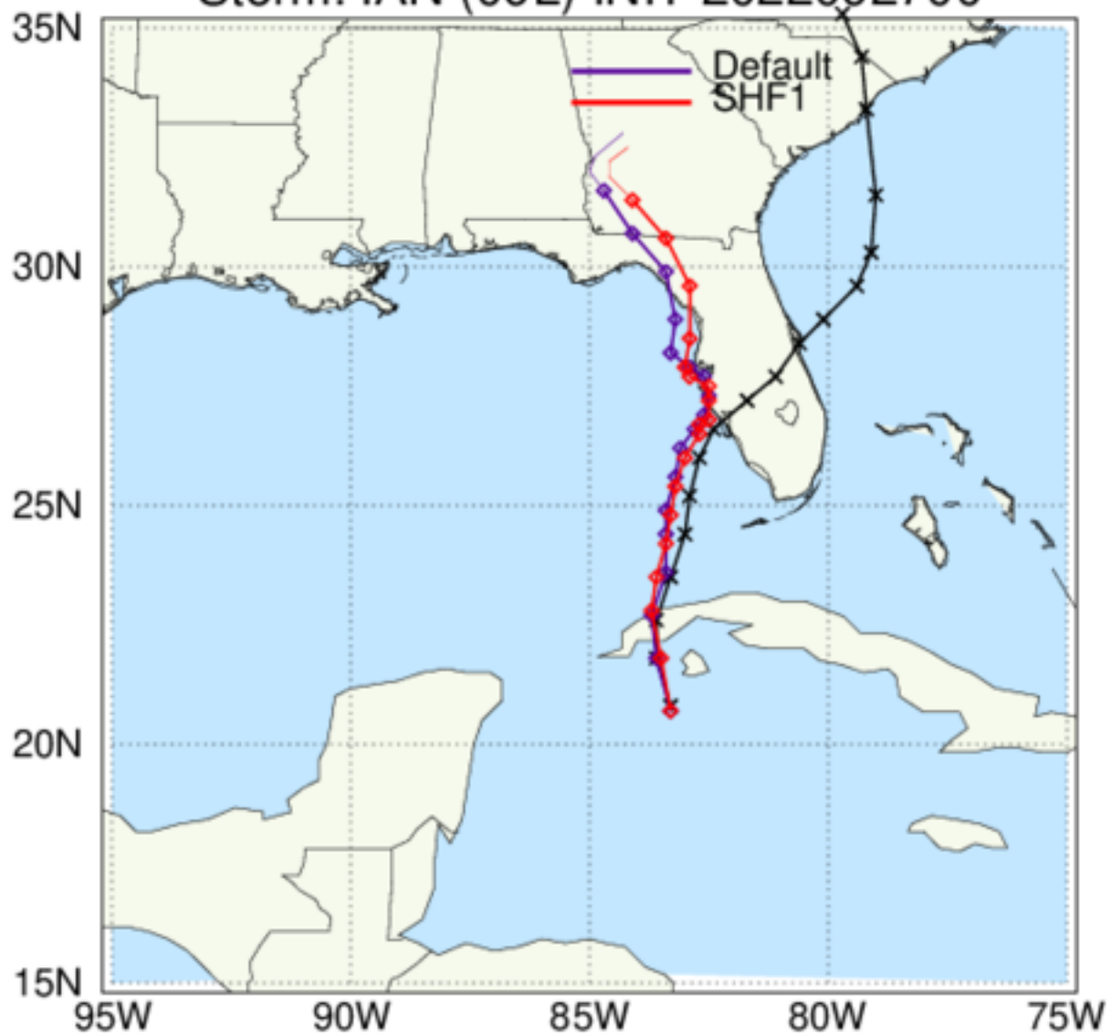
HAFS: TC Tracks Storm: IAN (09L) INIT 2022092700
