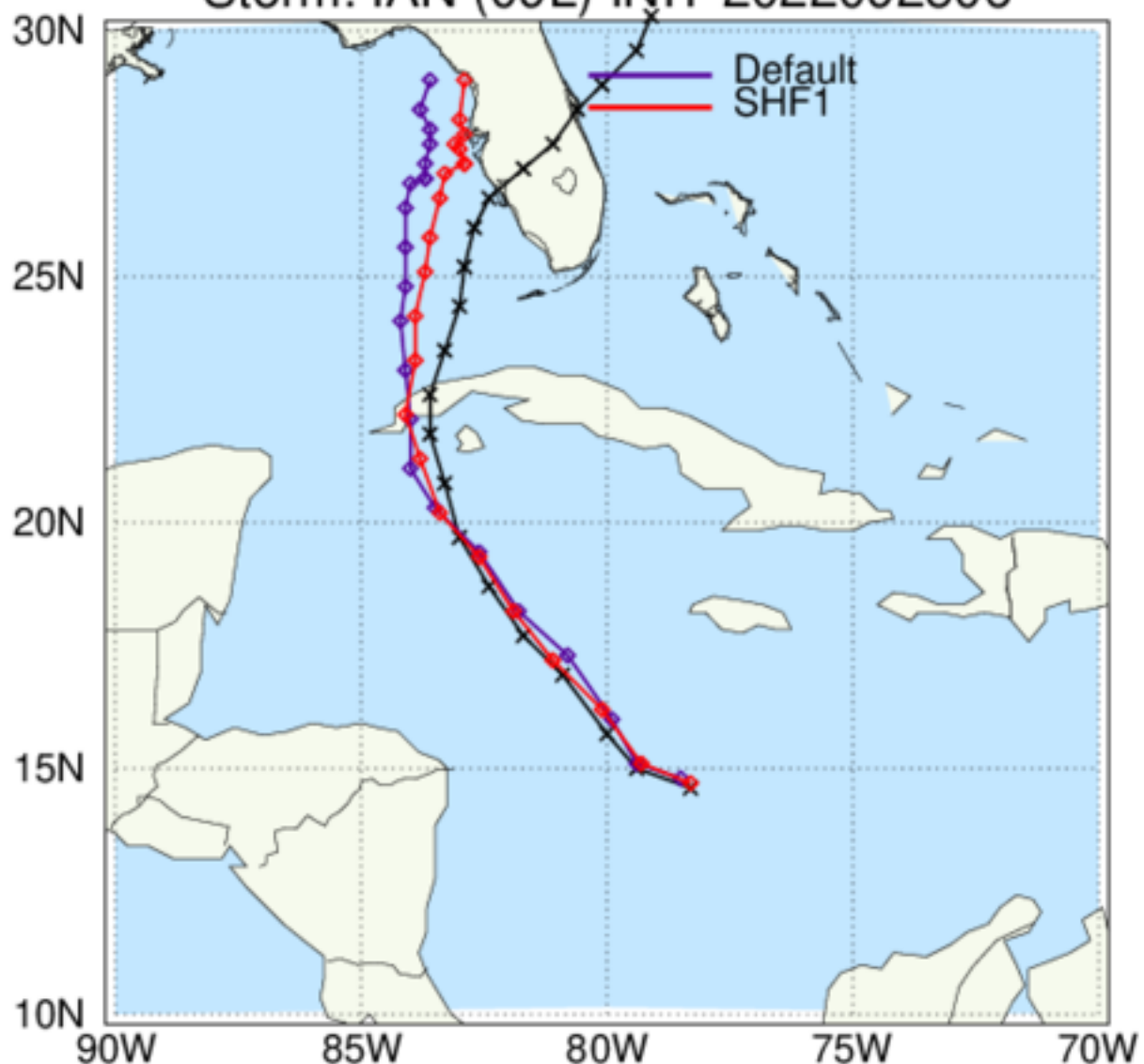
HAFS: TC Tracks Storm: IAN (09L) INIT 2022092506
