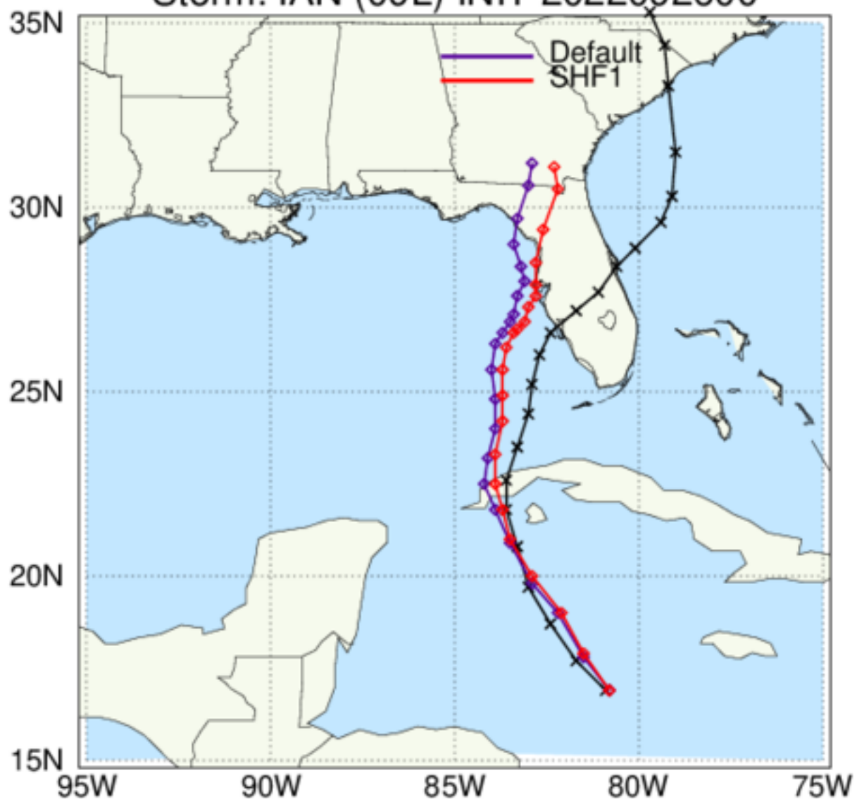
HAFS: TC Tracks Storm: IAN (09L) INIT 2022092600
