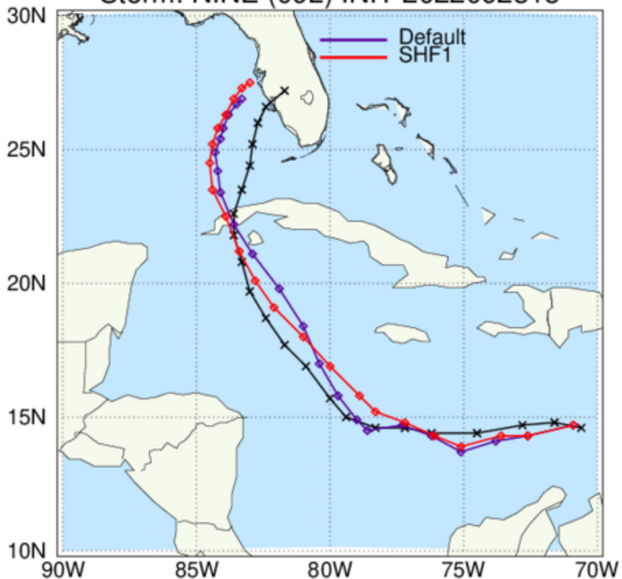
HAFS: TC Tracks Storm: NINE (09L) INIT 2022092318
