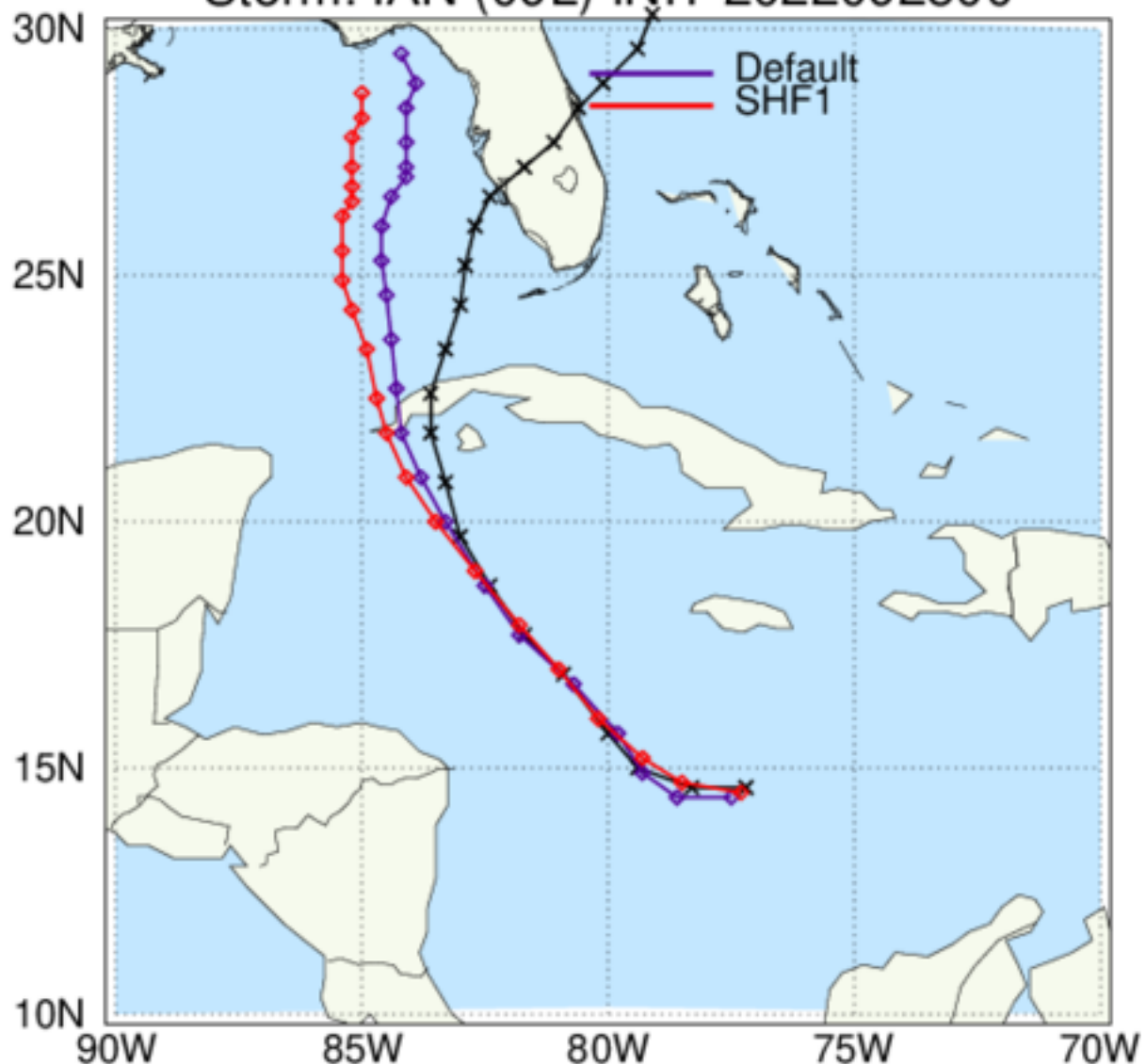
HAFS: TC Tracks Storm: IAN (09L) INIT 2022092500
