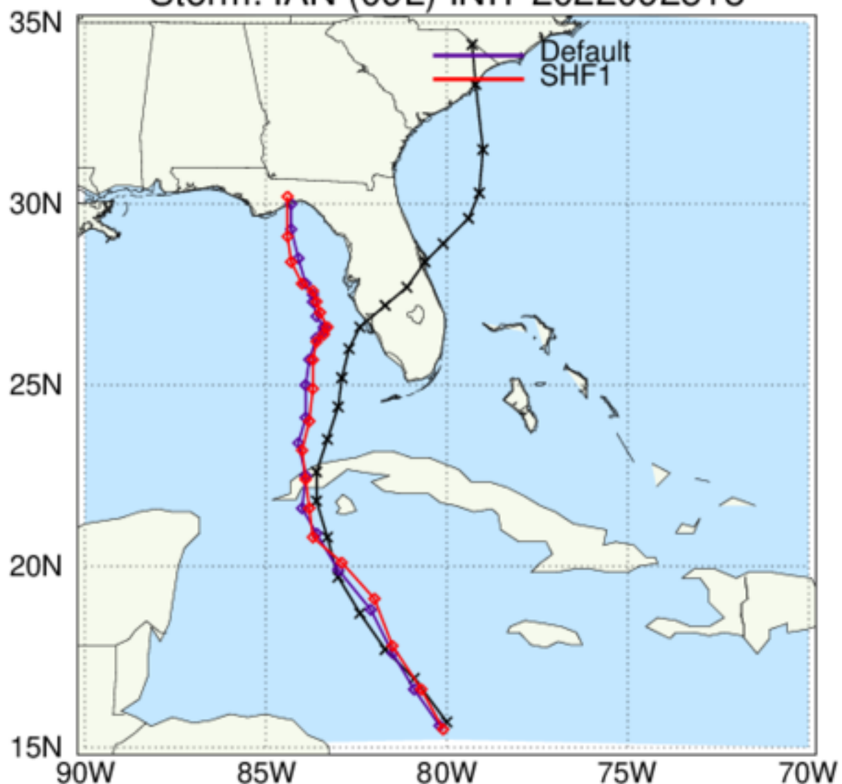
HAFS: TC Tracks Storm: IAN (09L) INIT 2022092518
