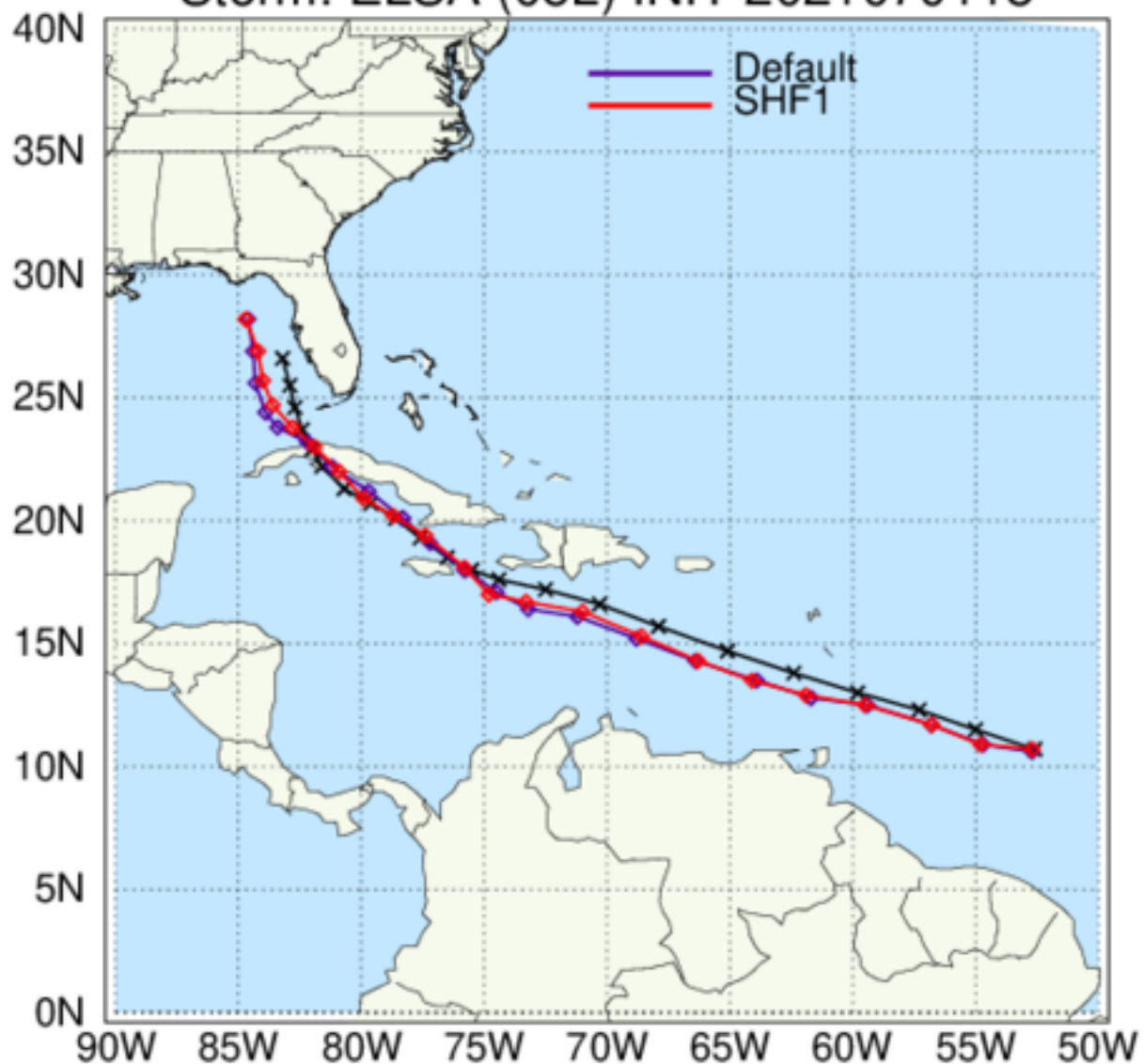
HAFS: TC Tracks Storm: ELSA (05L) INIT 2021070118
