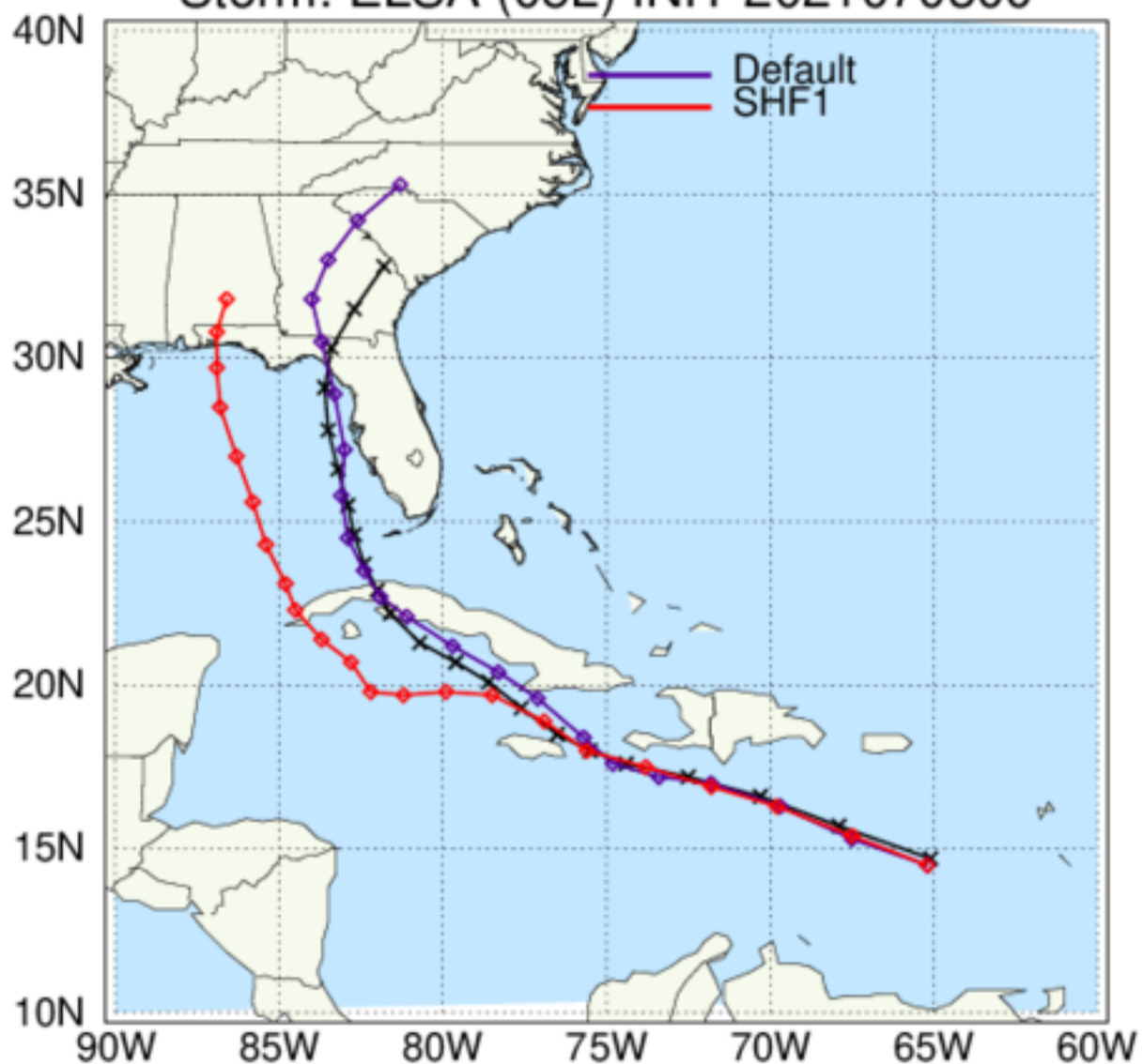
HAFS: TC Tracks Storm: ELSA (05L) INIT 2021070300
