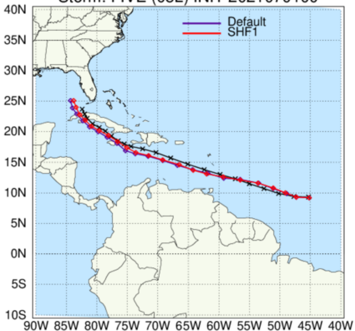
HAFS: TC Tracks Storm: FIVE (05L) INIT 2021070100
