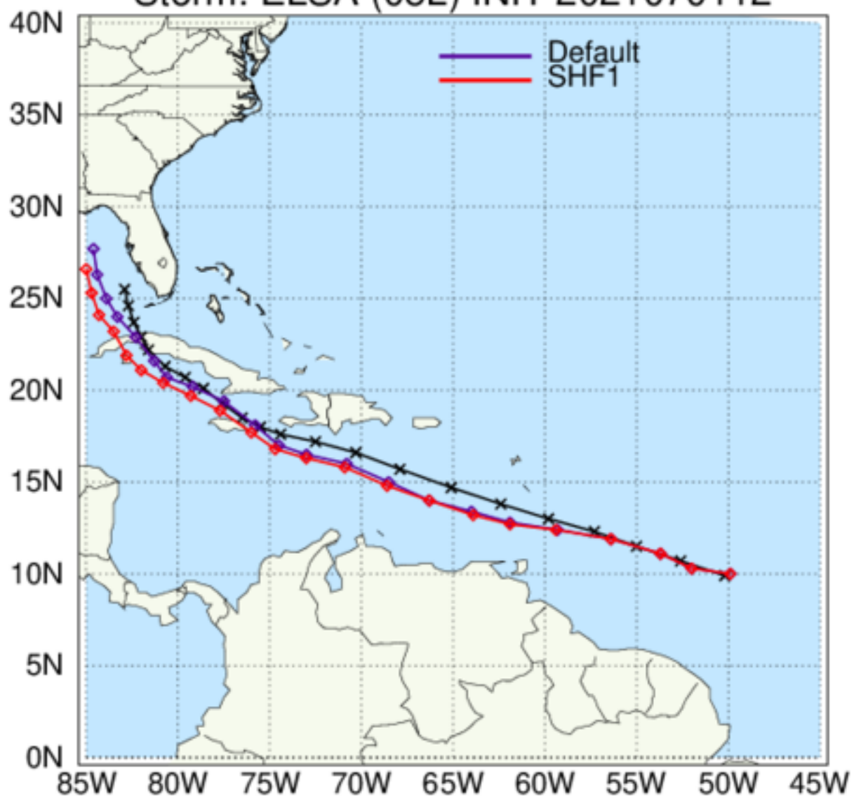
HAFS: TC Tracks Storm: ELSA (05L) INIT 2021070112
