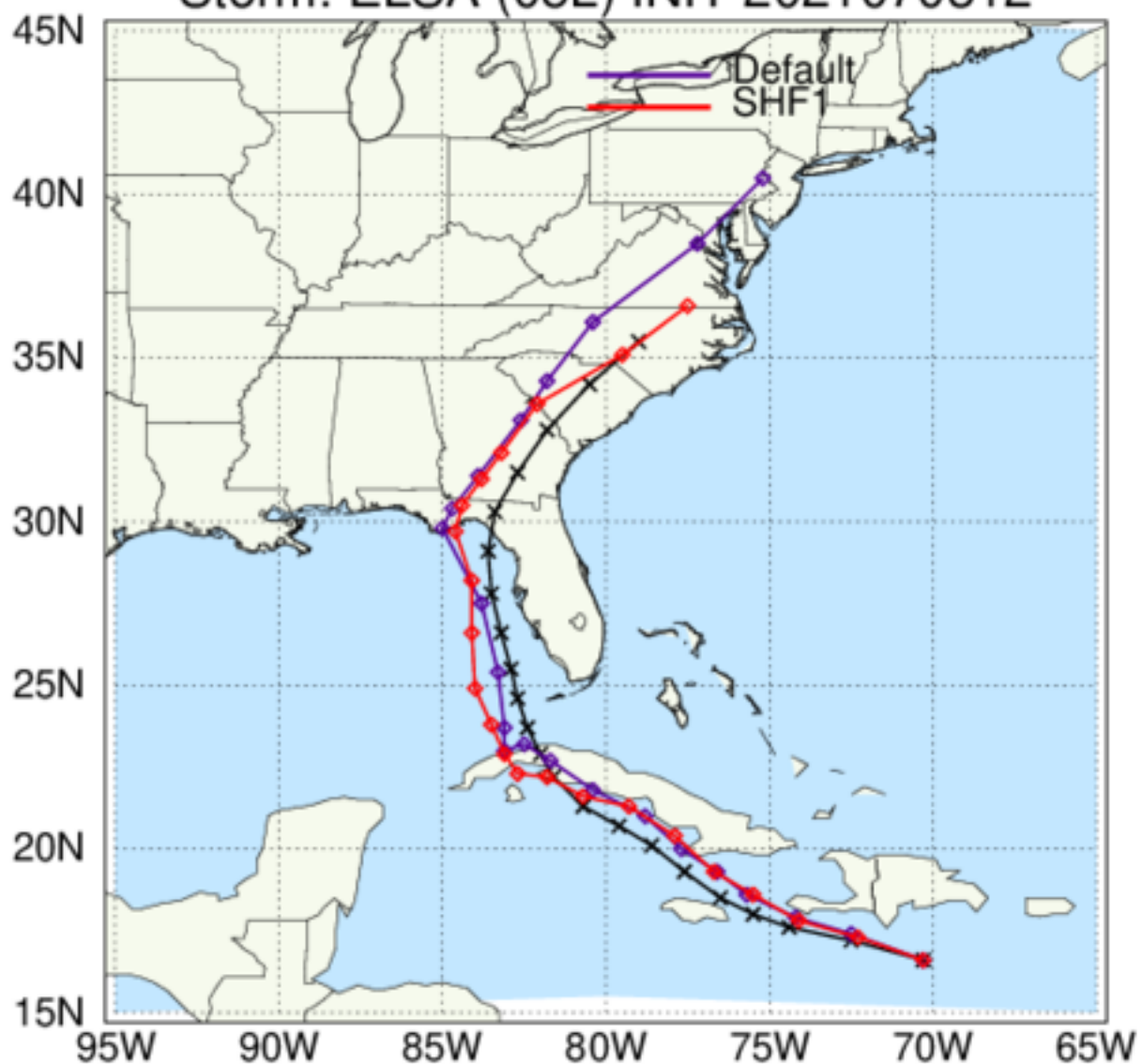
HAFS: TC Tracks Storm: ELSA (05L) INIT 2021070312
