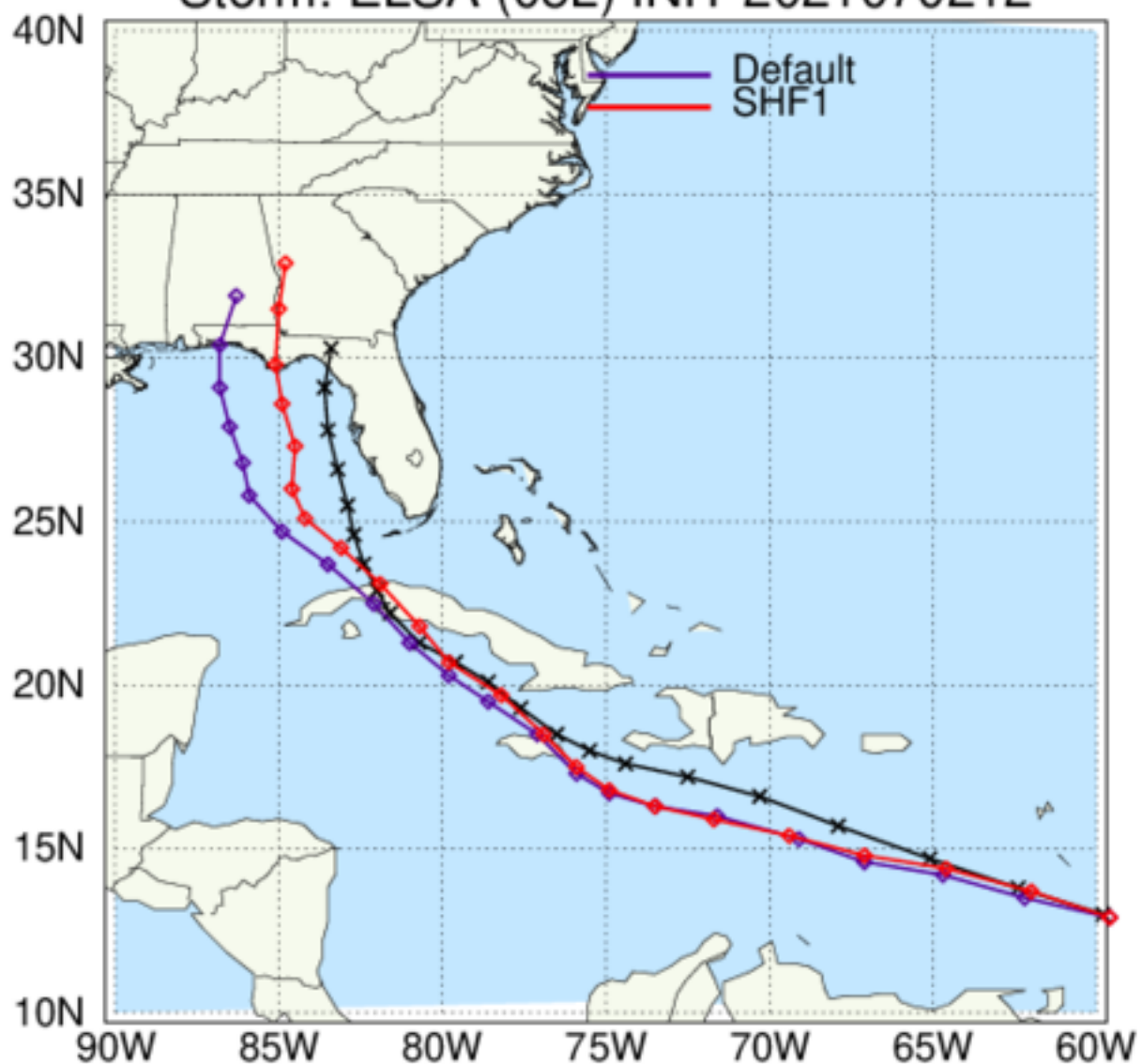
HAFS: TC Tracks Storm: ELSA (05L) INIT 2021070212
