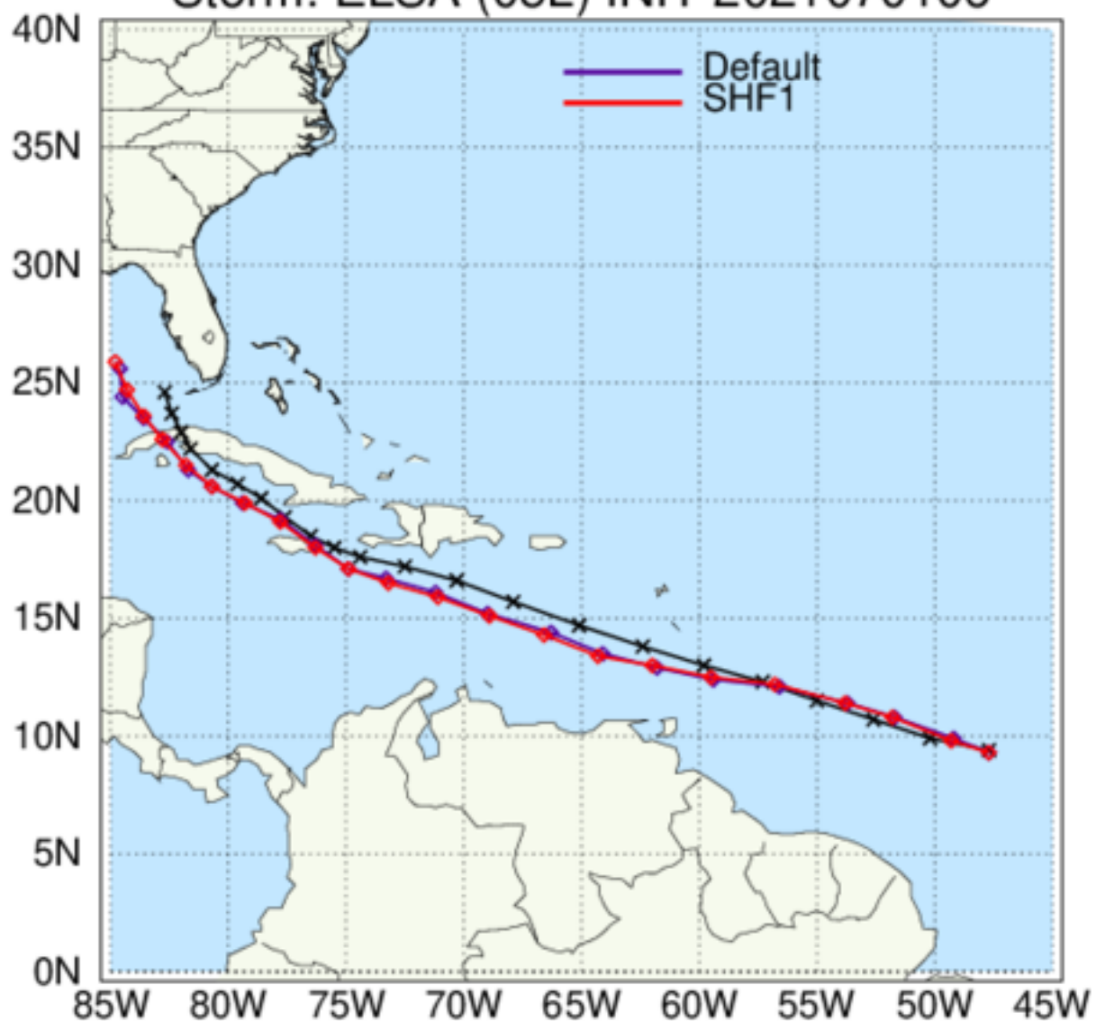
HAFS: TC Tracks Storm: ELSA (05L) INIT 2021070106
