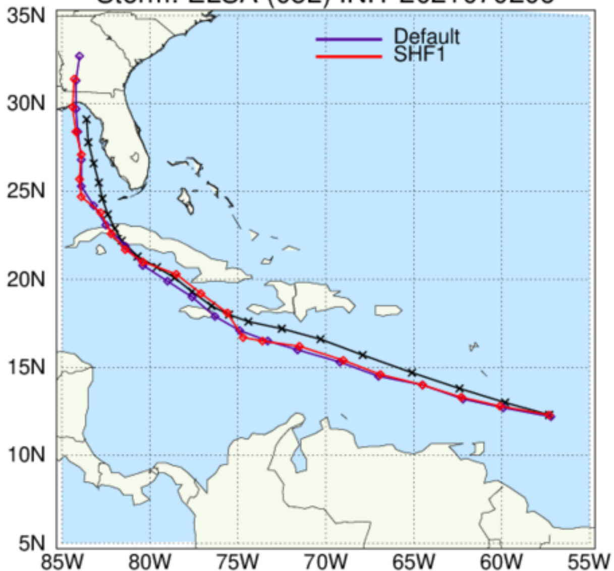
HAFS: TC Tracks Storm: ELSA (05L) INIT 2021070206
