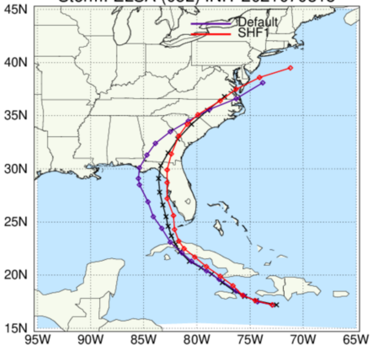
HAFS: TC Tracks Storm: ELSA (05L) INIT 2021070318
