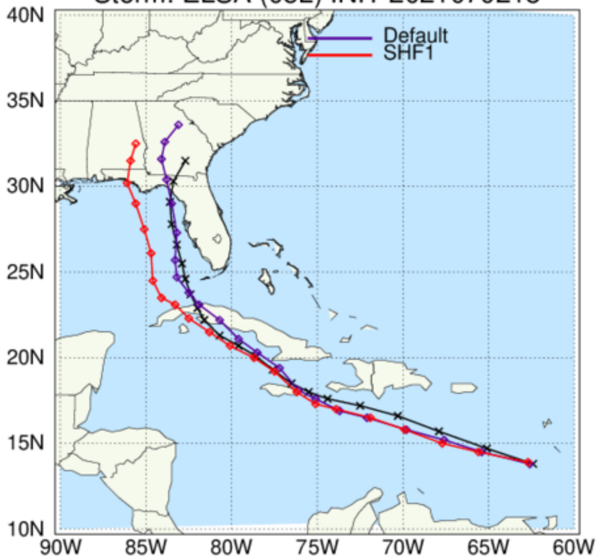
HAFS: TC Tracks Storm: ELSA (05L) INIT 2021070218
