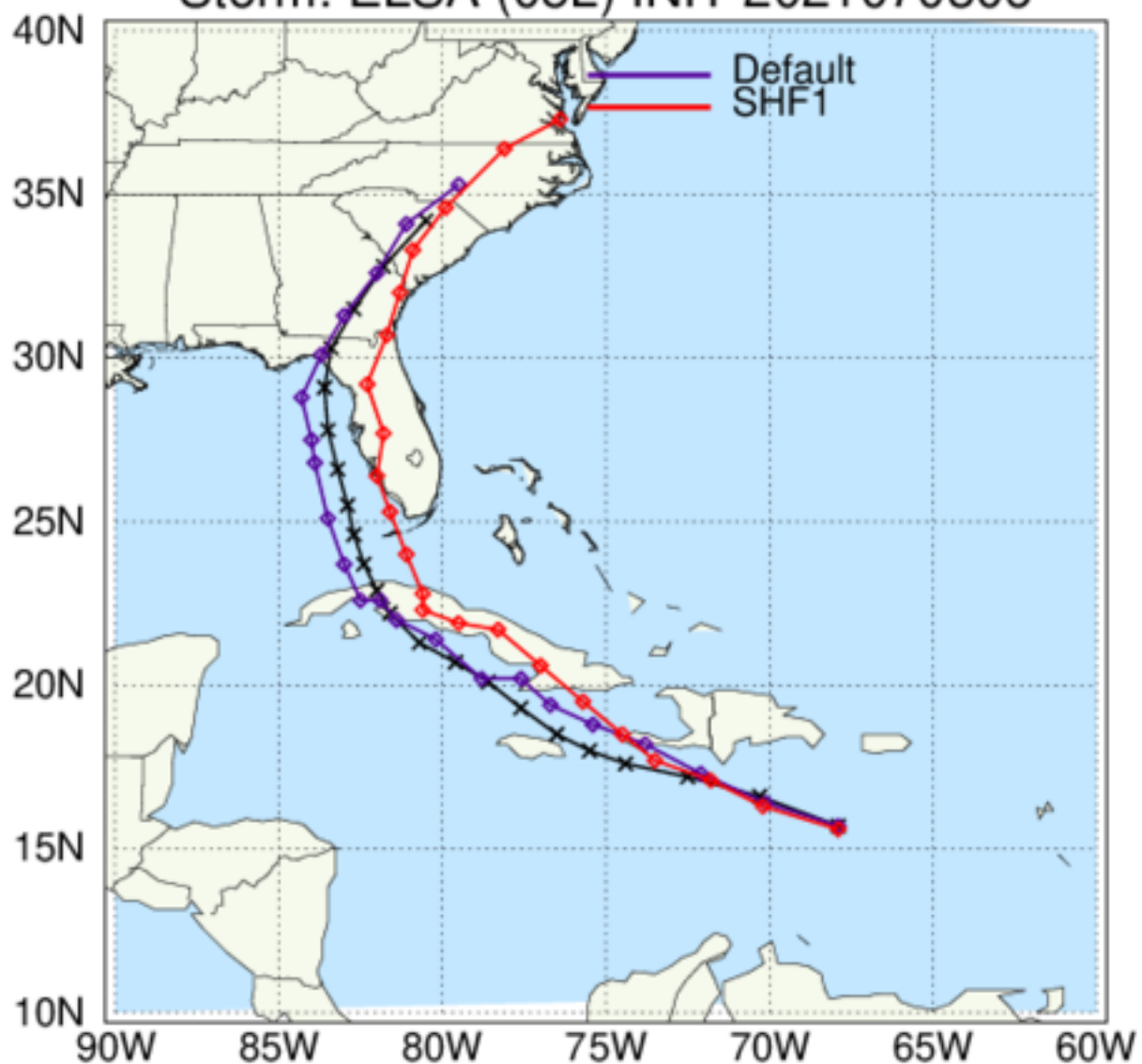
HAFS: TC Tracks Storm: ELSA (05L) INIT 2021070306
