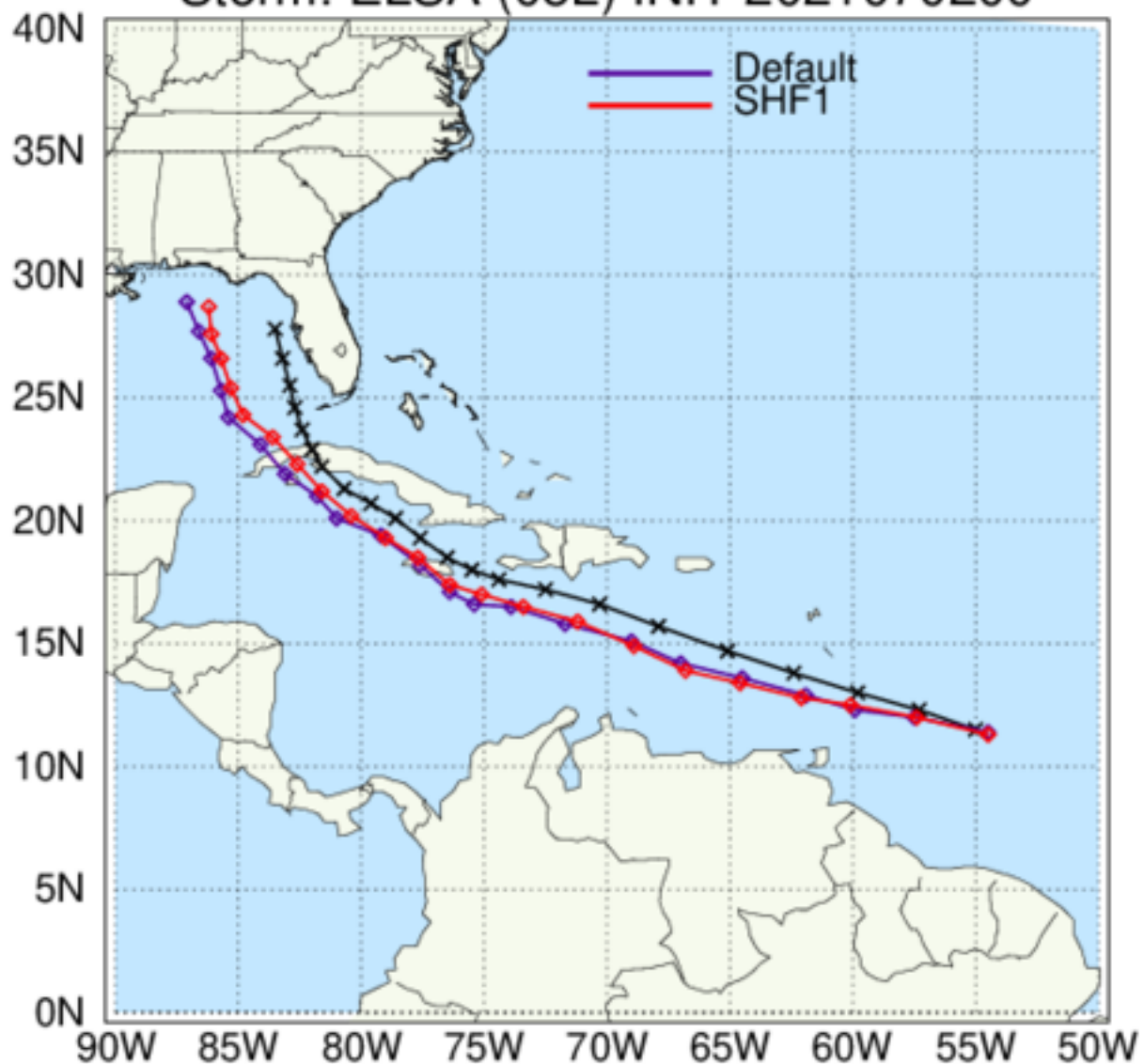
HAFS: TC Tracks Storm: ELSA (05L) INIT 2021070200
