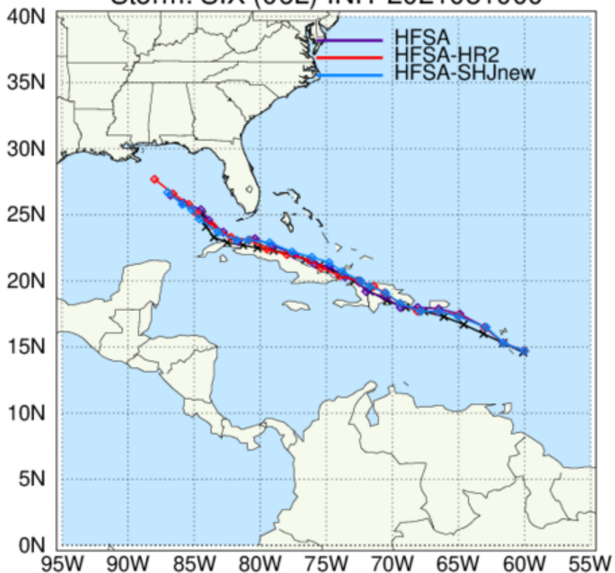
HAFS: TC Tracks Storm: SIX (06L) INIT 2021081000
