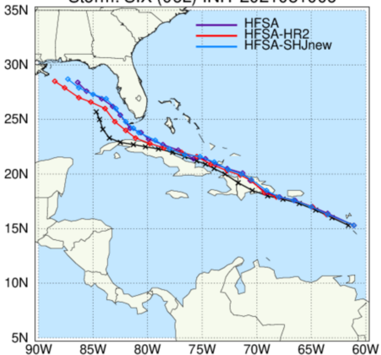
HAFS: TC Tracks Storm: SIX (06L) INIT 2021081006
