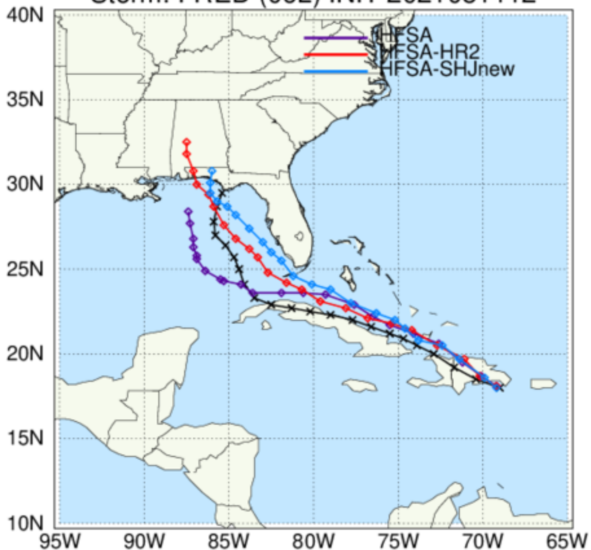
HAFS: TC Tracks Storm: FRED (06L) INIT 2021081112
