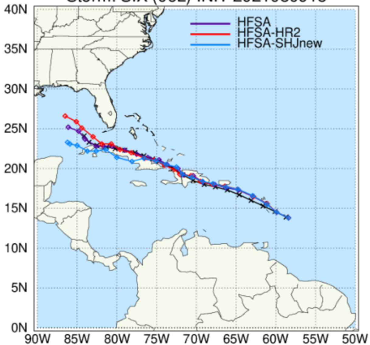
HAFS: TC Tracks Storm: SIX (06L) INIT 2021080918
