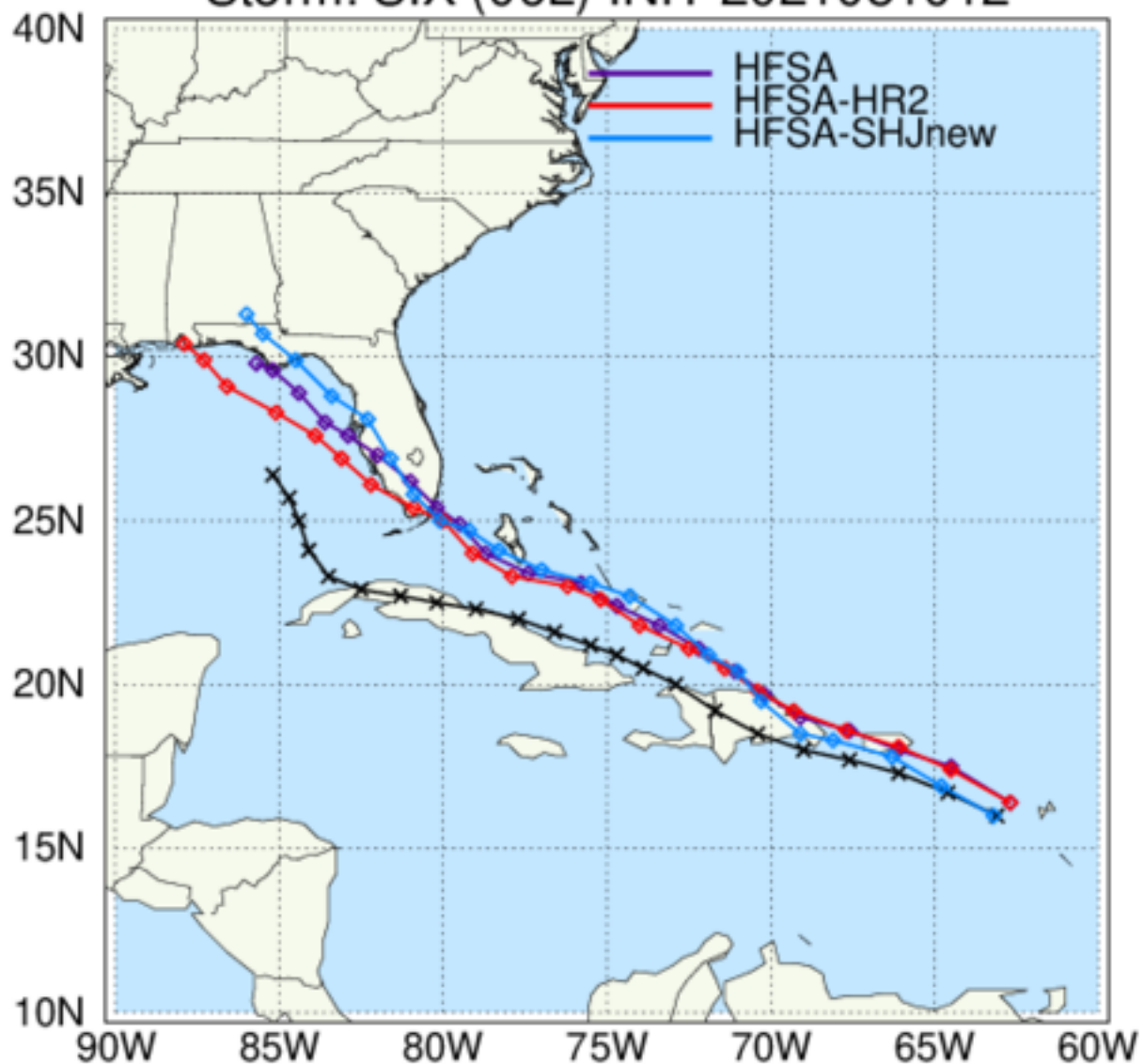
HAFS: TC Tracks Storm: SIX (06L) INIT 2021081012
