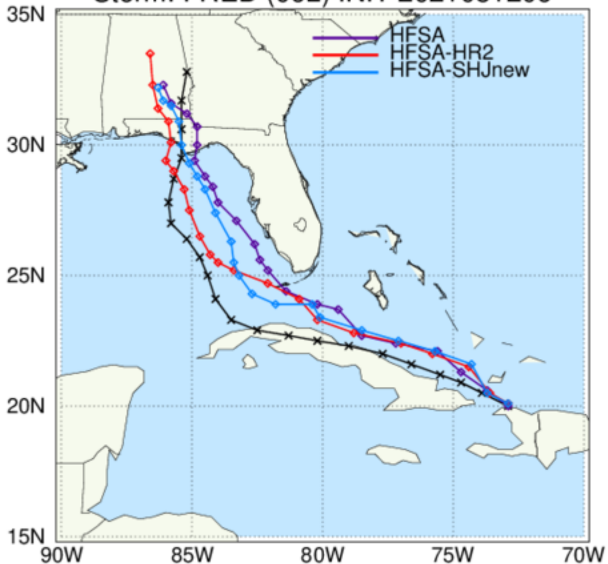
HAFS: TC Tracks Storm: FRED (06L) INIT 2021081206
