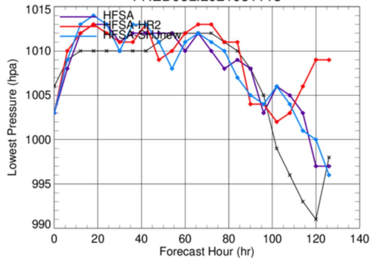
FRED06L.2021081118
