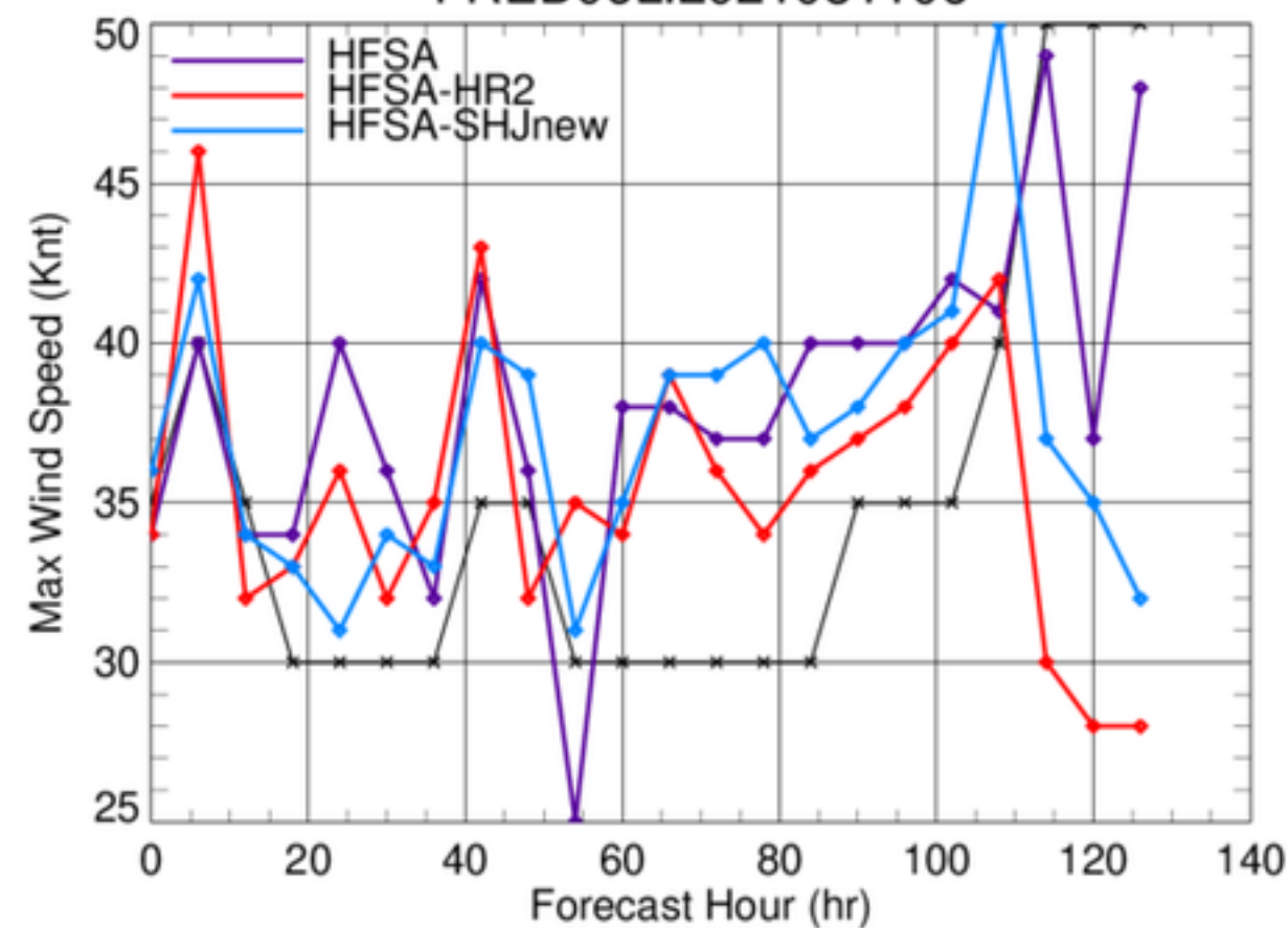
FRED06L.2021081106
