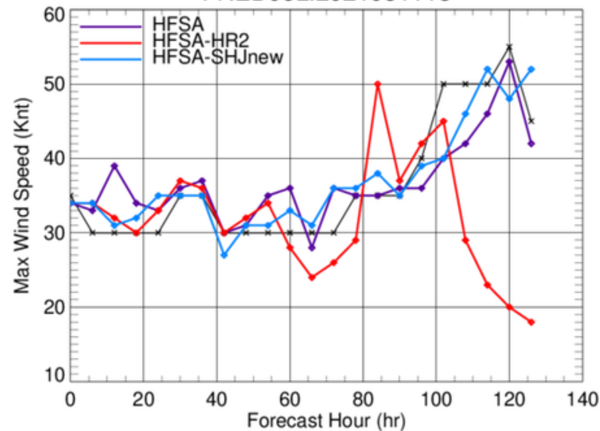
FRED06L.2021081118
