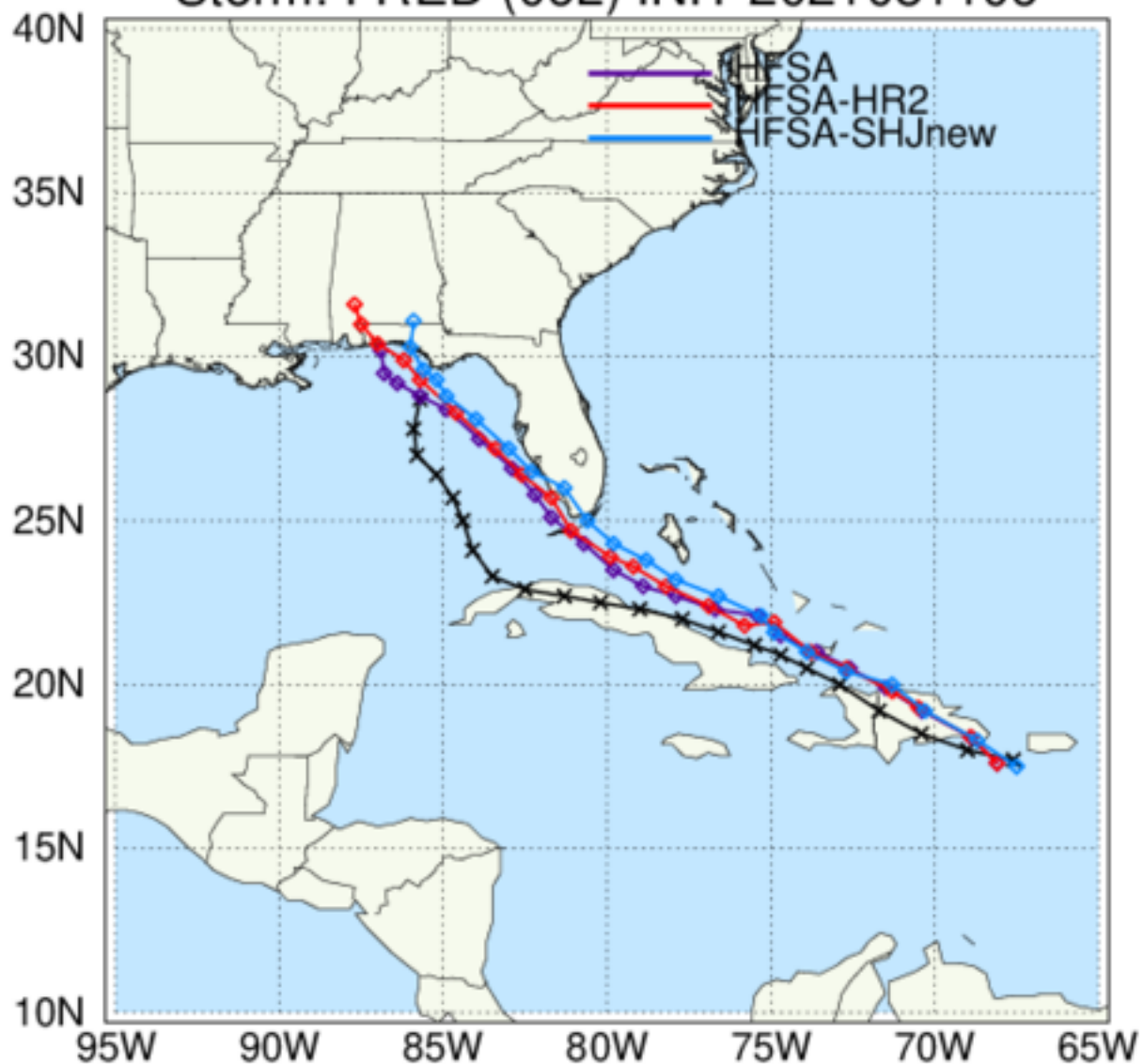
HAFS: TC Tracks Storm: FRED (06L) INIT 2021081106
