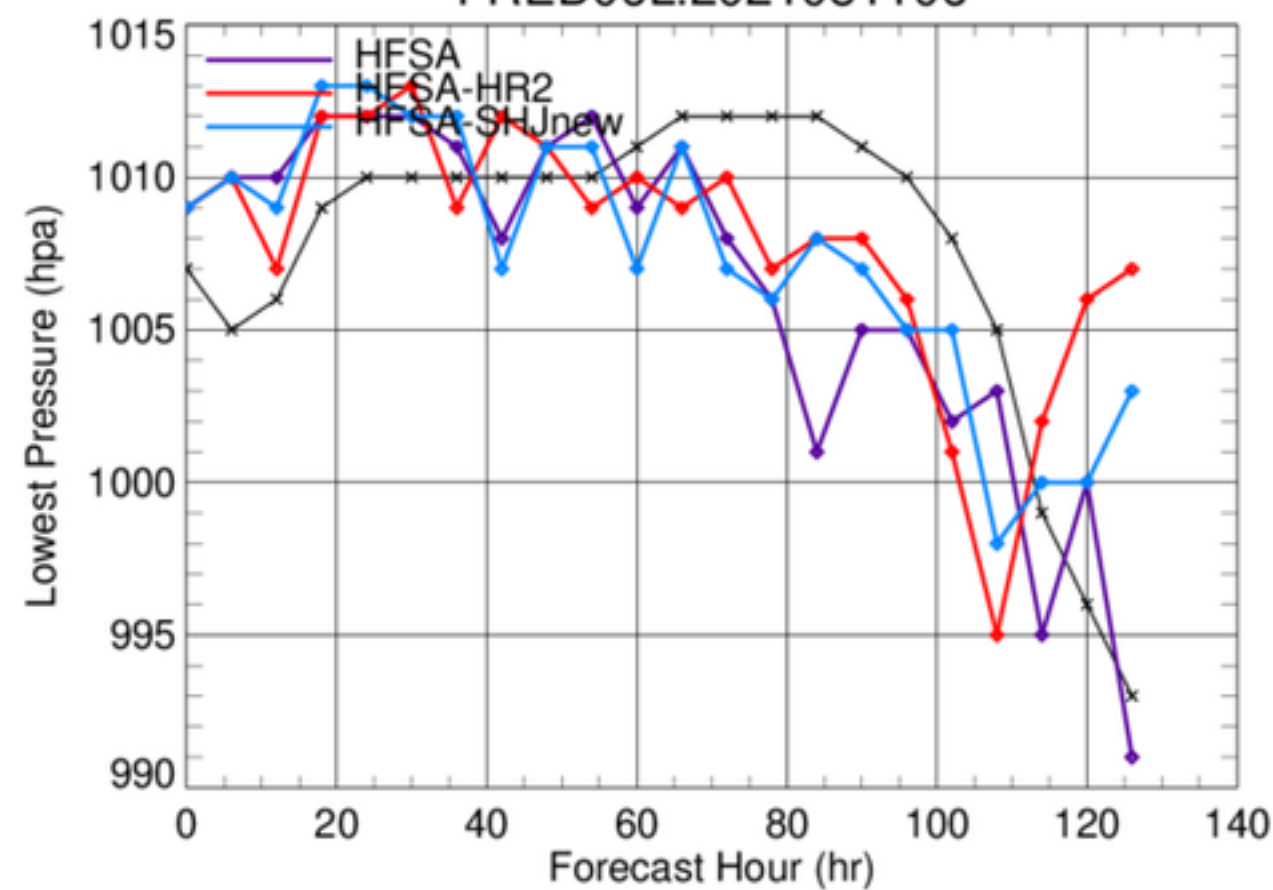
FRED06L.2021081106
