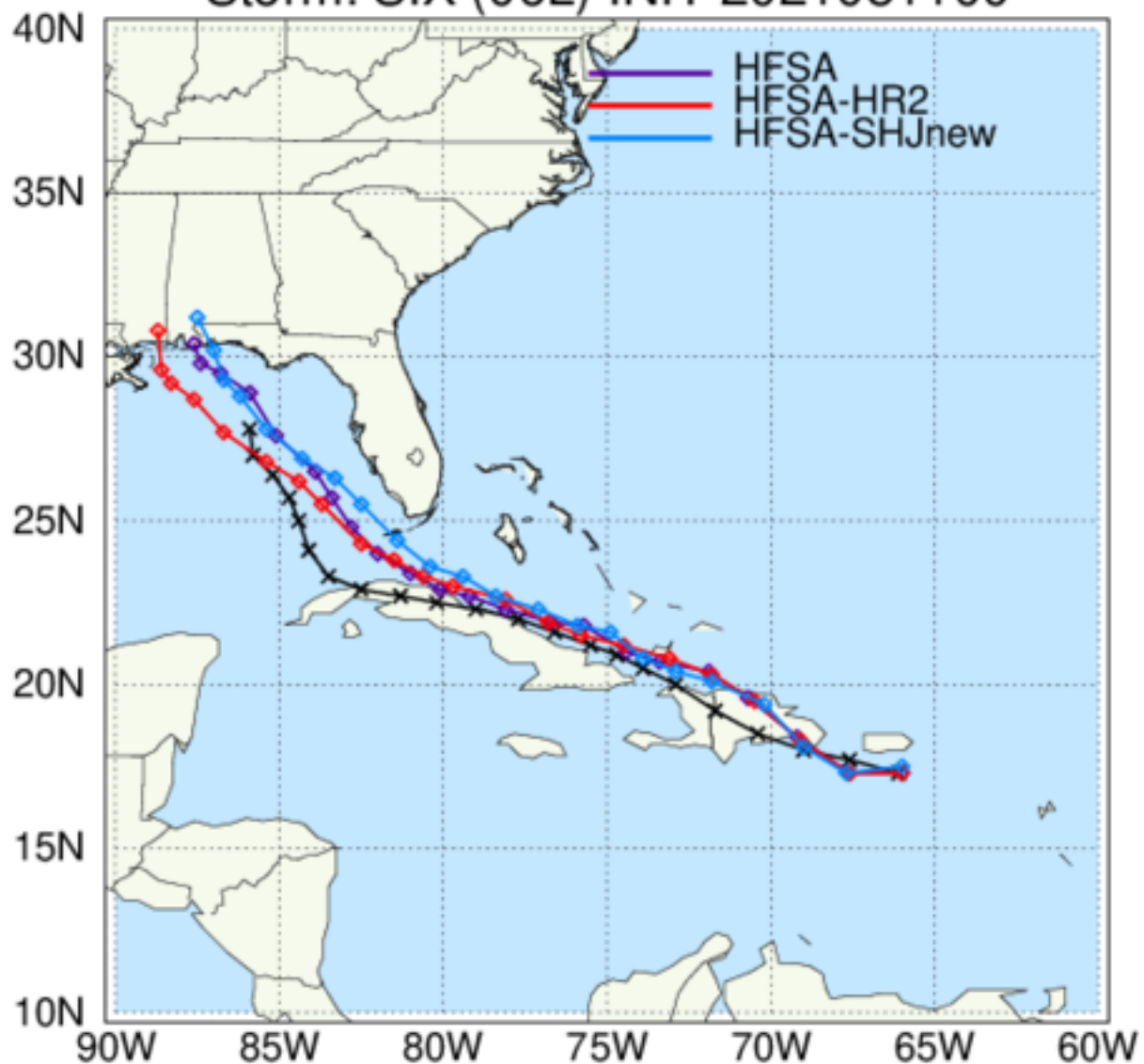
HAFS: TC Tracks Storm: SIX (06L) INIT 2021081100
