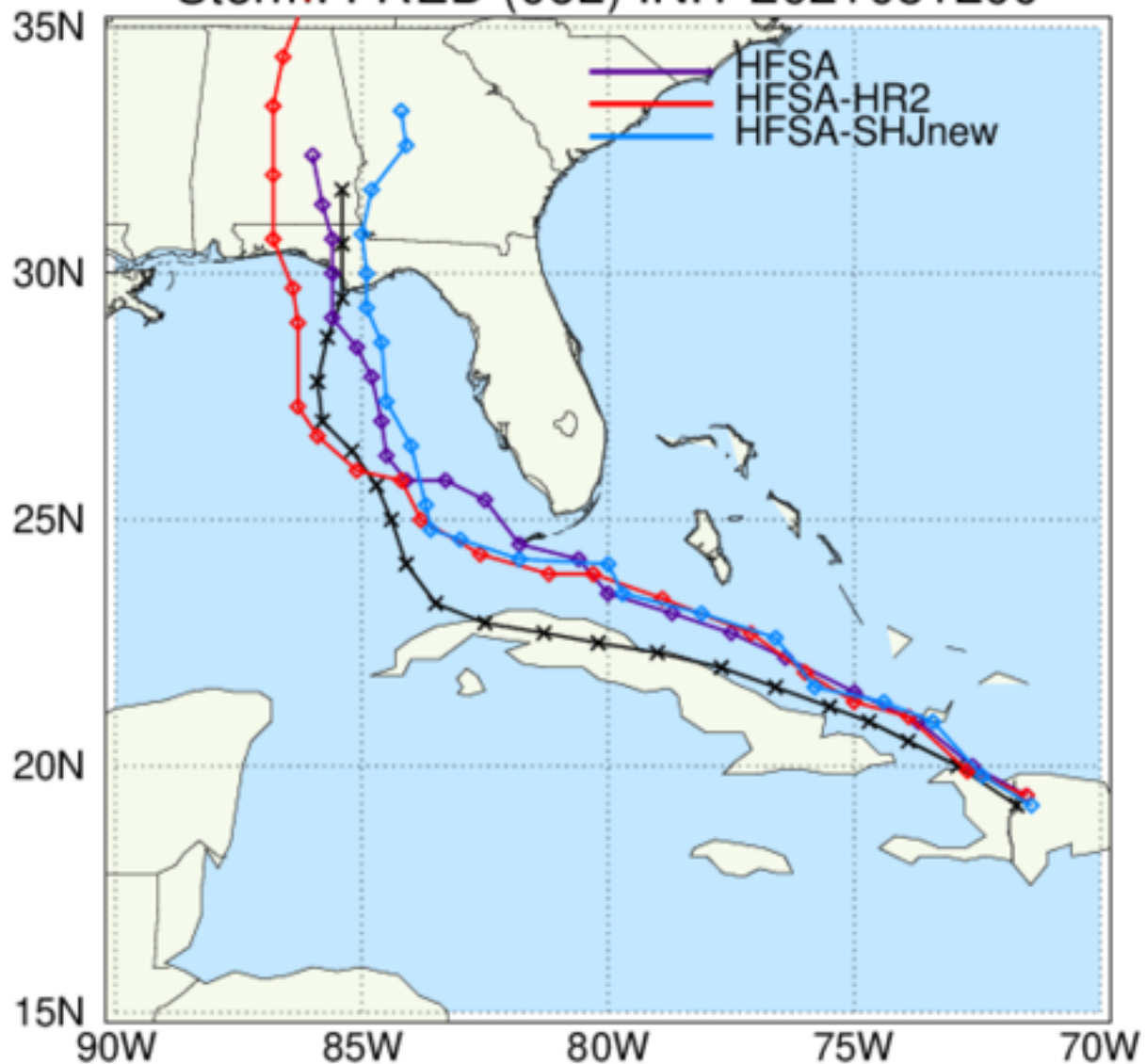
HAFS: TC Tracks Storm: FRED (06L) INIT 2021081200
