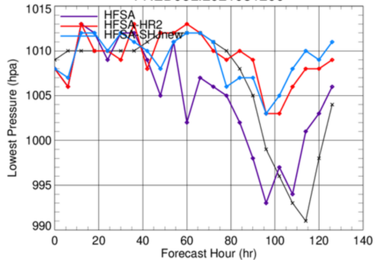
FRED06L.2021081200
