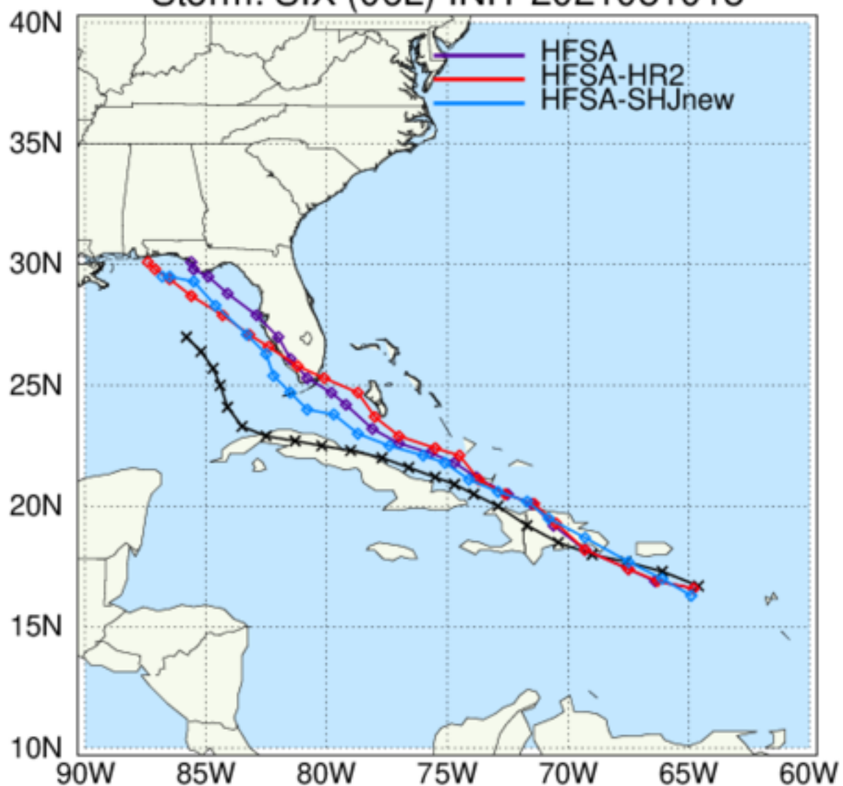
HAFS: TC Tracks Storm: SIX (06L) INIT 2021081018
