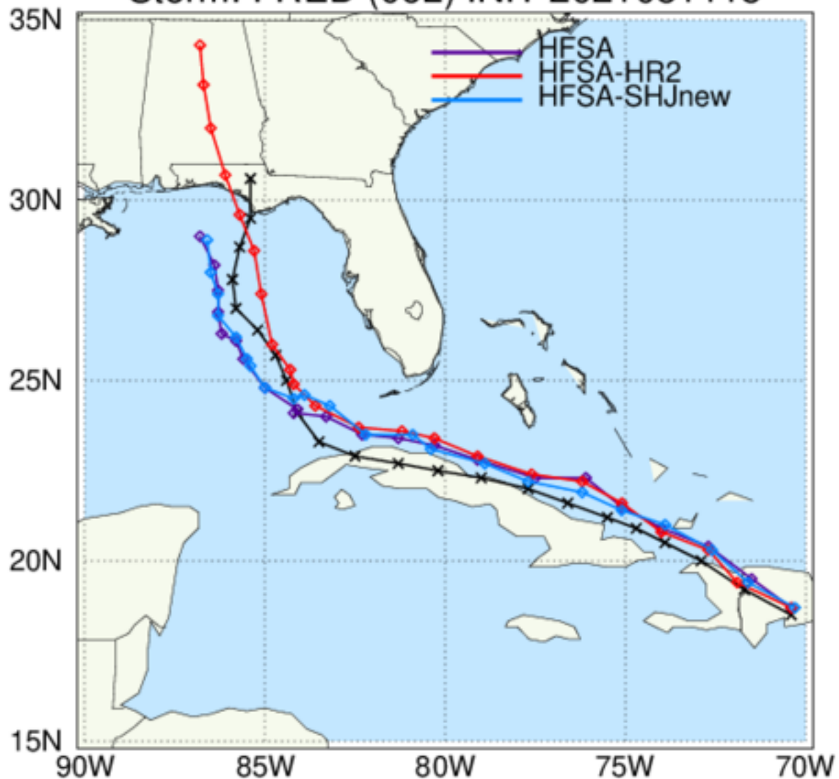
HAFS: TC Tracks Storm: FRED (06L) INIT 2021081118
