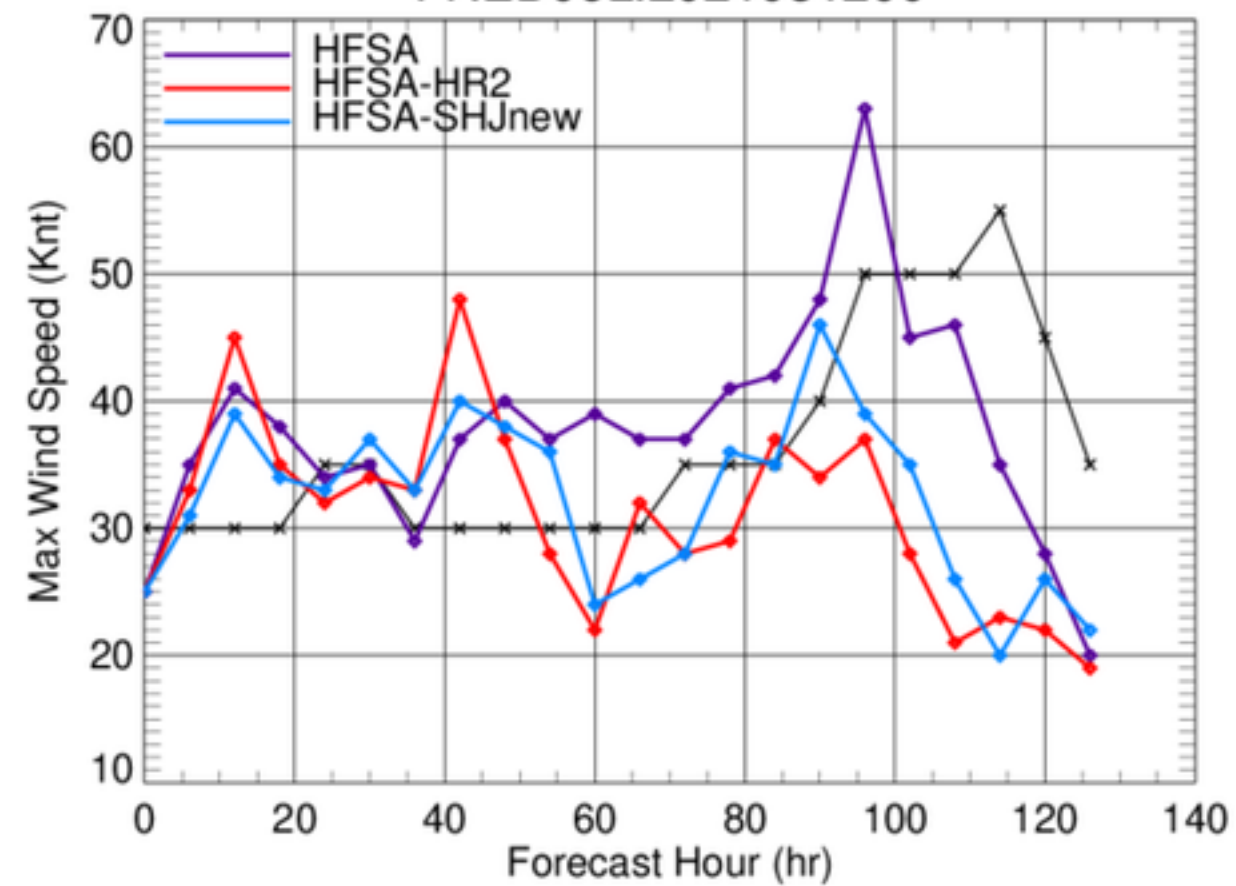
FRED06L.2021081200
