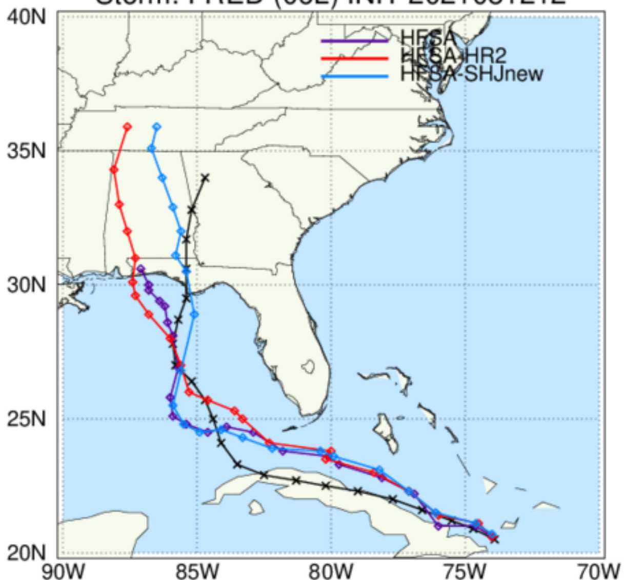
HAFS: TC Tracks Storm: FRED (06L) INIT 2021081212
