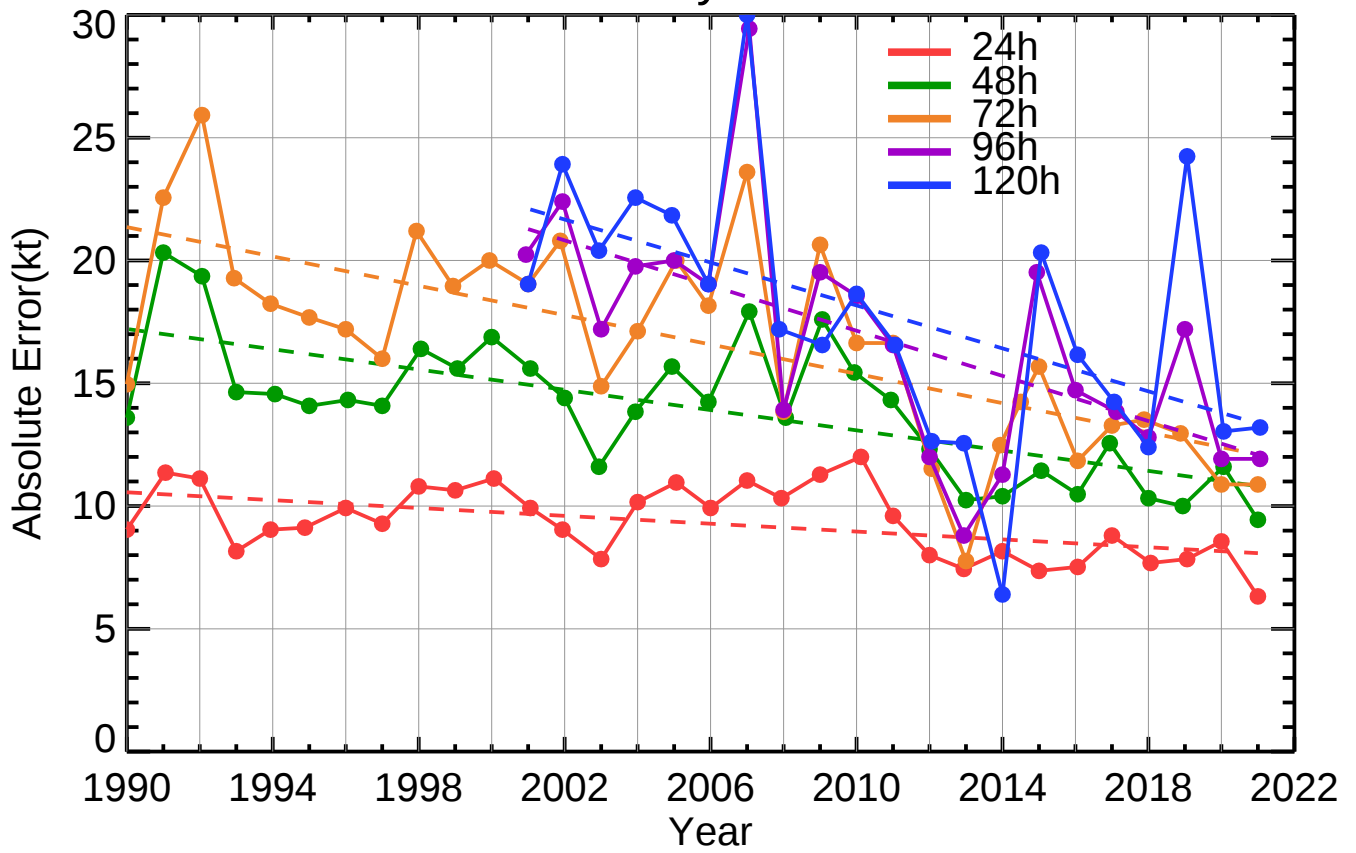
NHC official intensity forecast error trend
