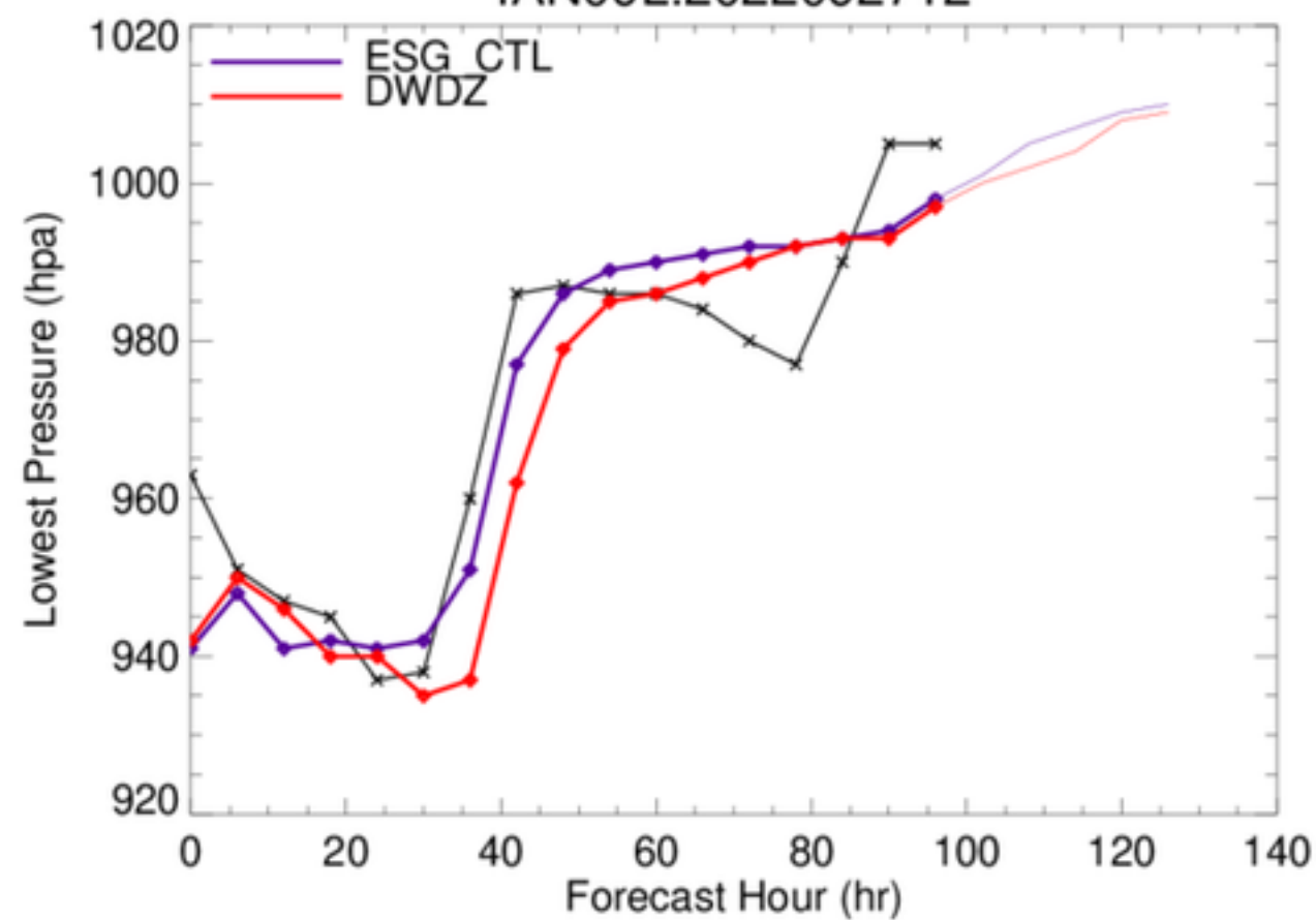
IAN09L.2022092712
