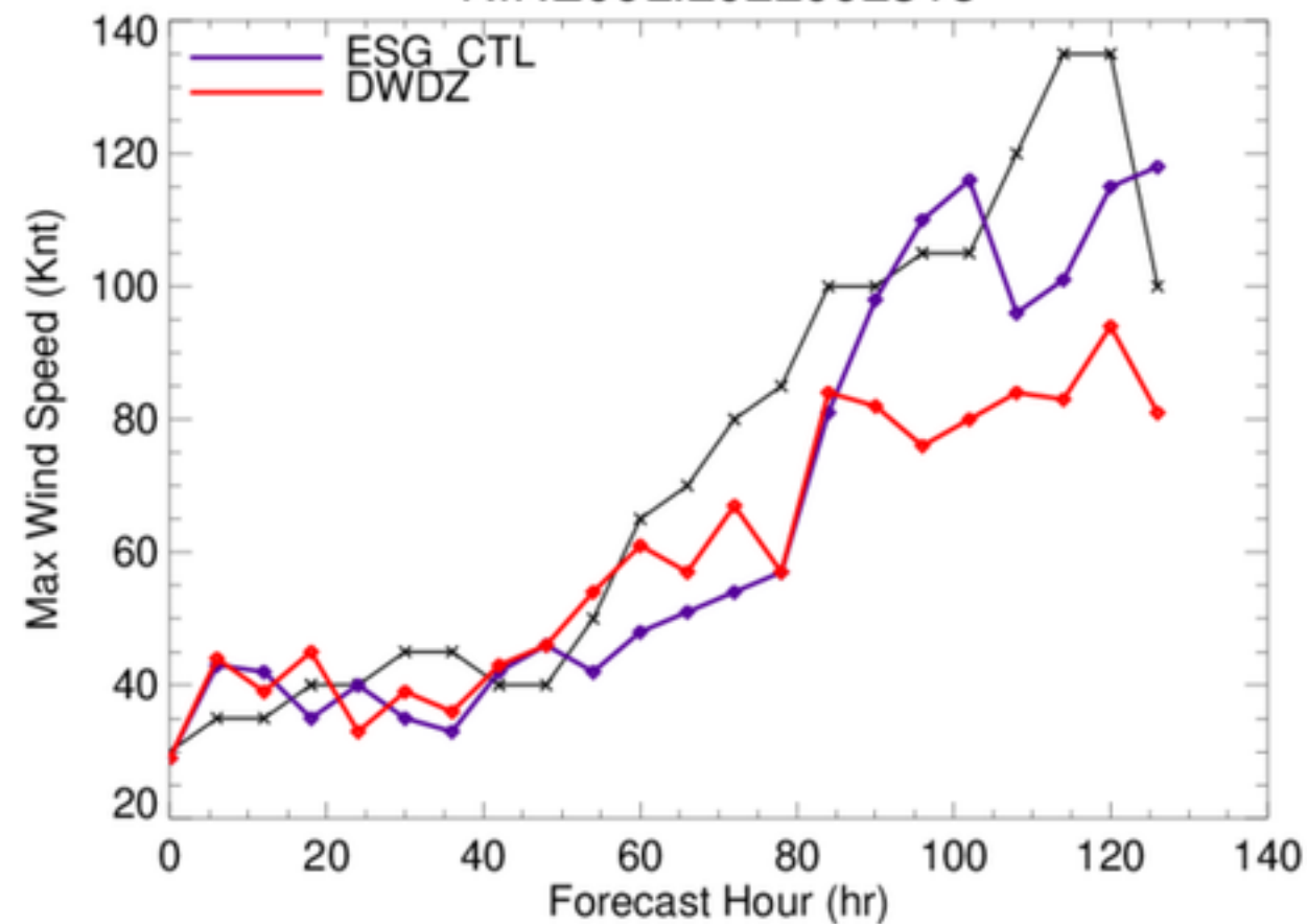
NINE09L.2022092318
