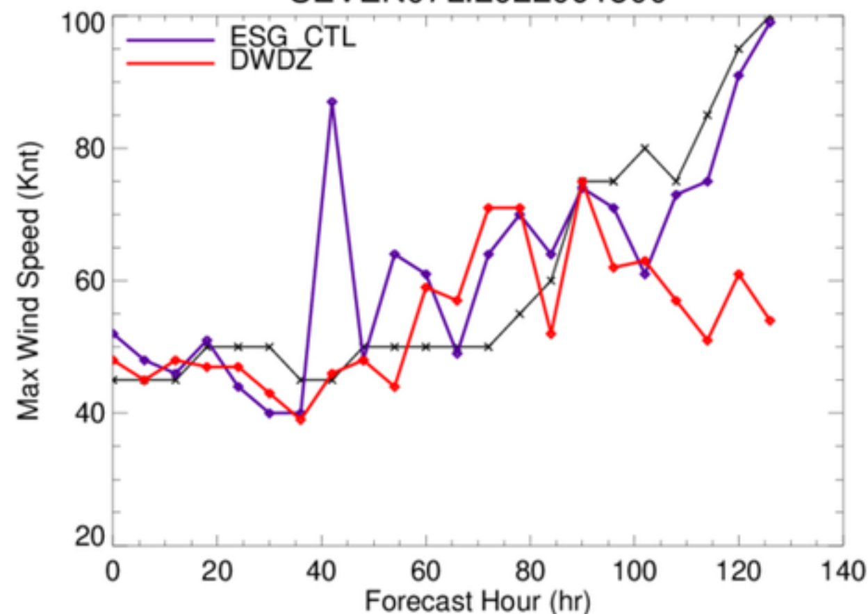
SEVEN07L.2022091500
