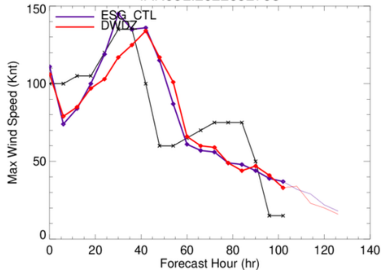
IAN09L.2022092706
