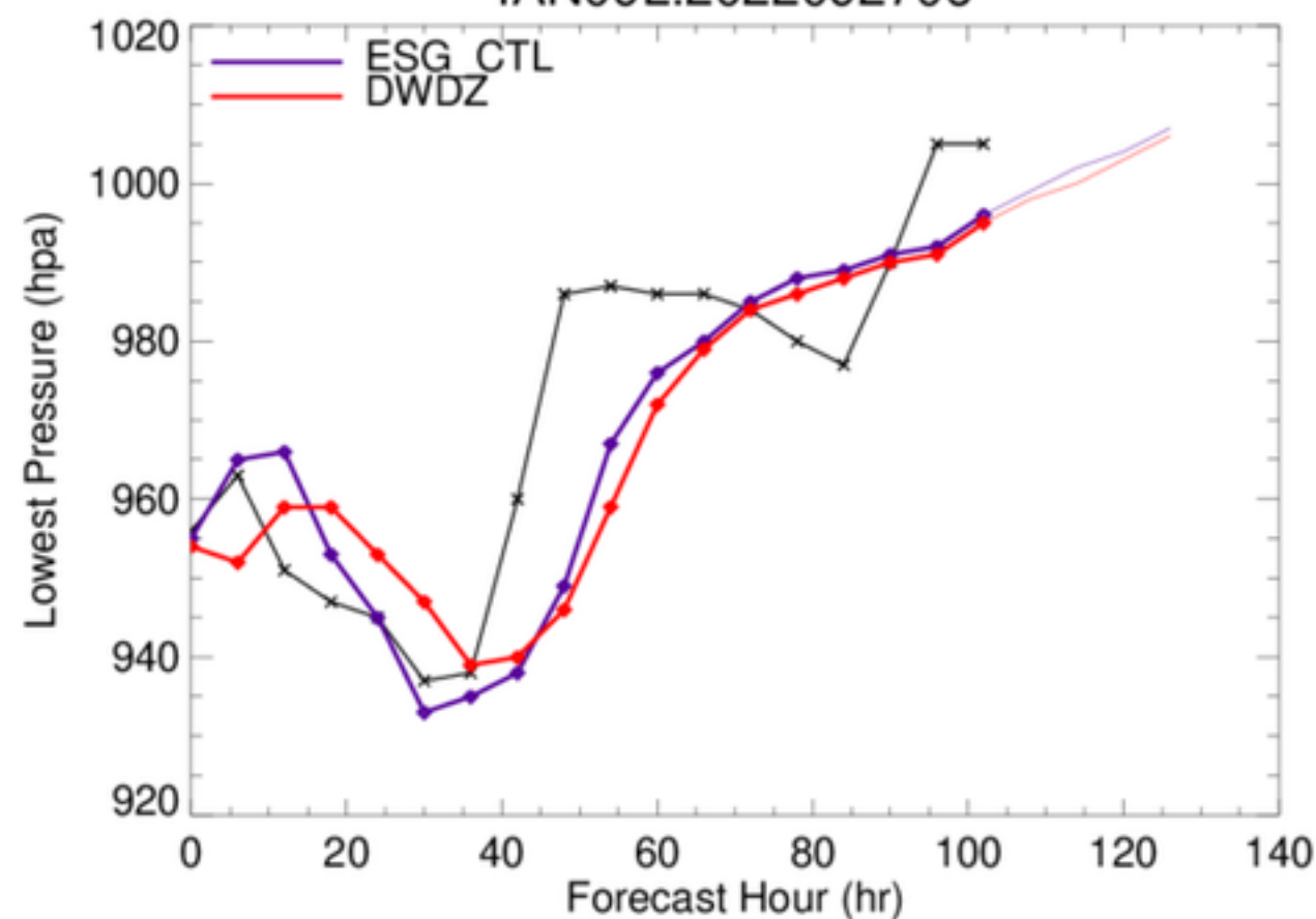
IAN09L.2022092706
