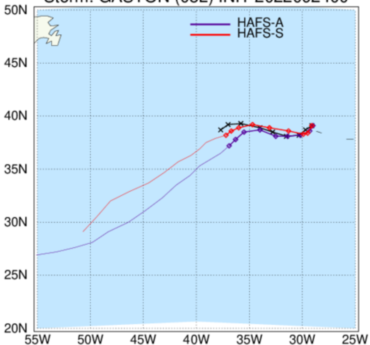
HAFS: TC Tracks Storm: GASTON (08L) INIT 2022092400
