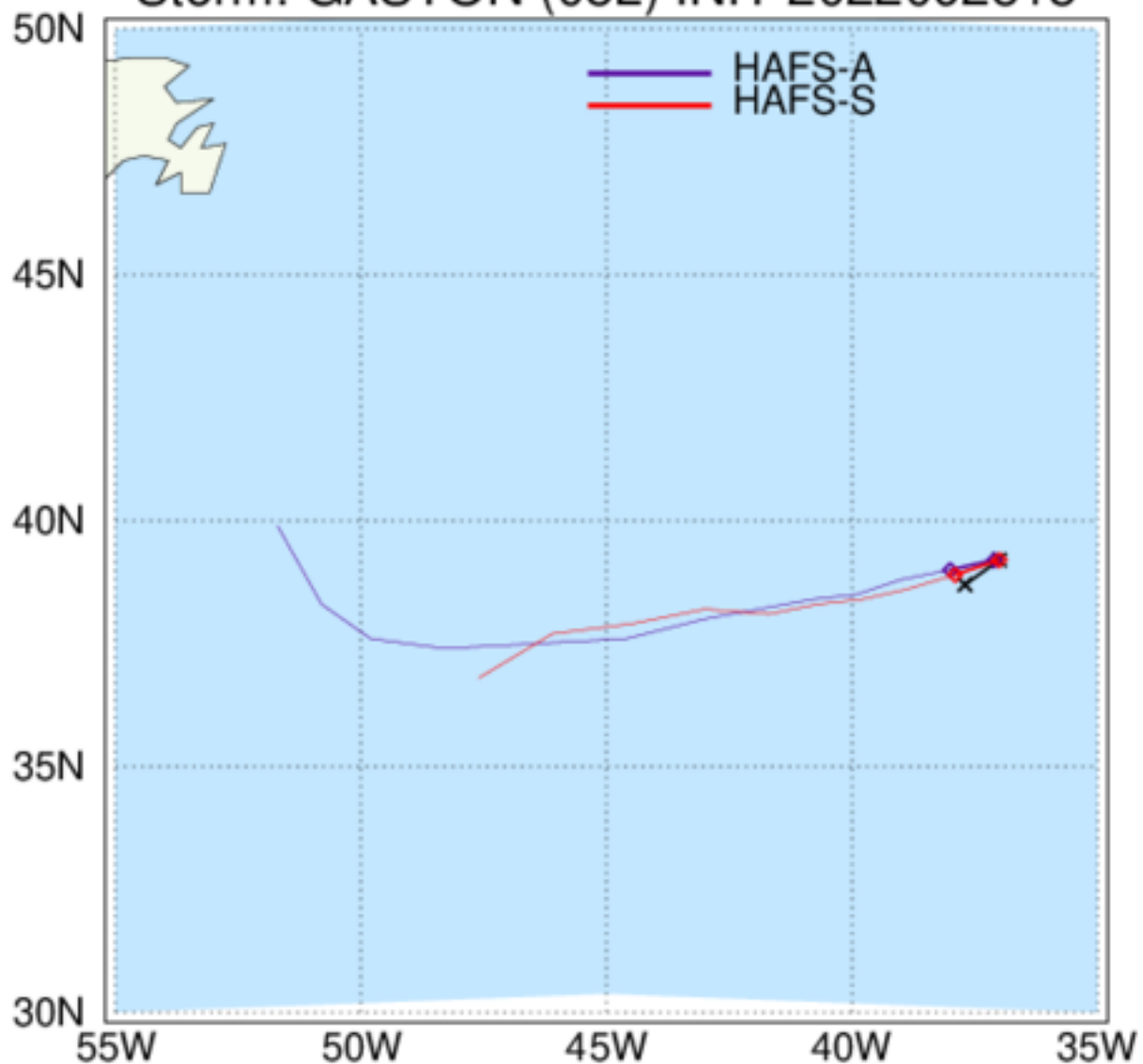
HAFS: TC Tracks Storm: GASTON (08L) INIT 2022092518
