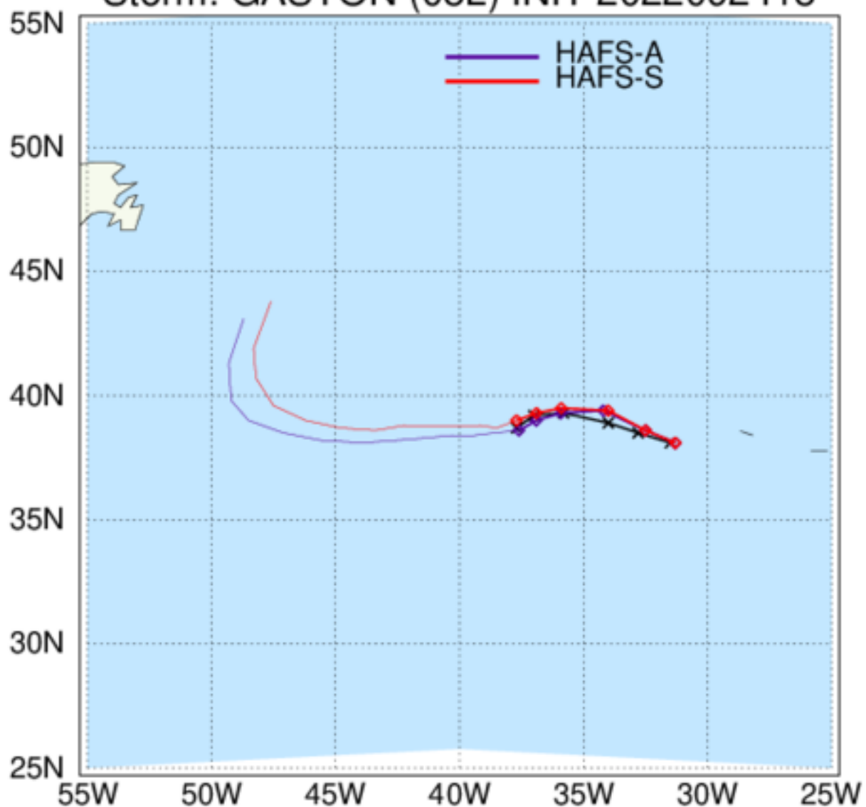
HAFS: TC Tracks Storm: GASTON (08L) INIT 2022092418
