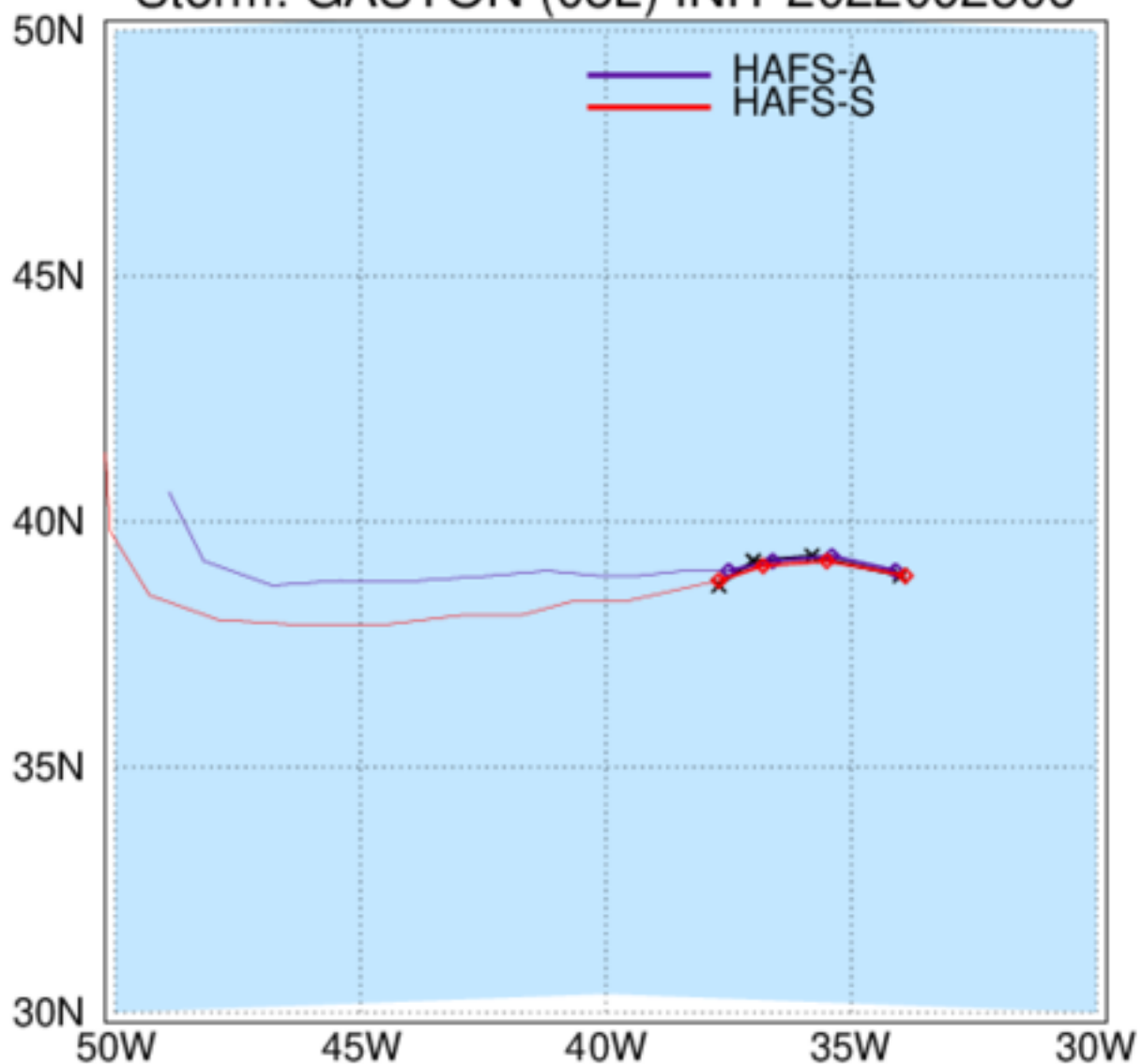
HAFS: TC Tracks Storm: GASTON (08L) INIT 2022092506
