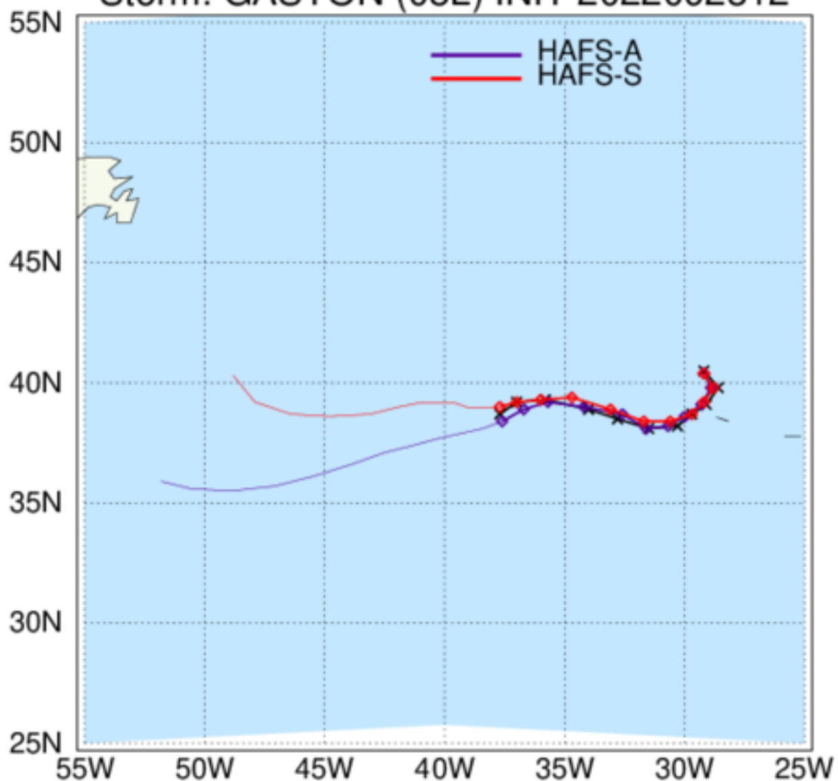
HAFS: TC Tracks Storm: GASTON (08L) INIT 2022092312
