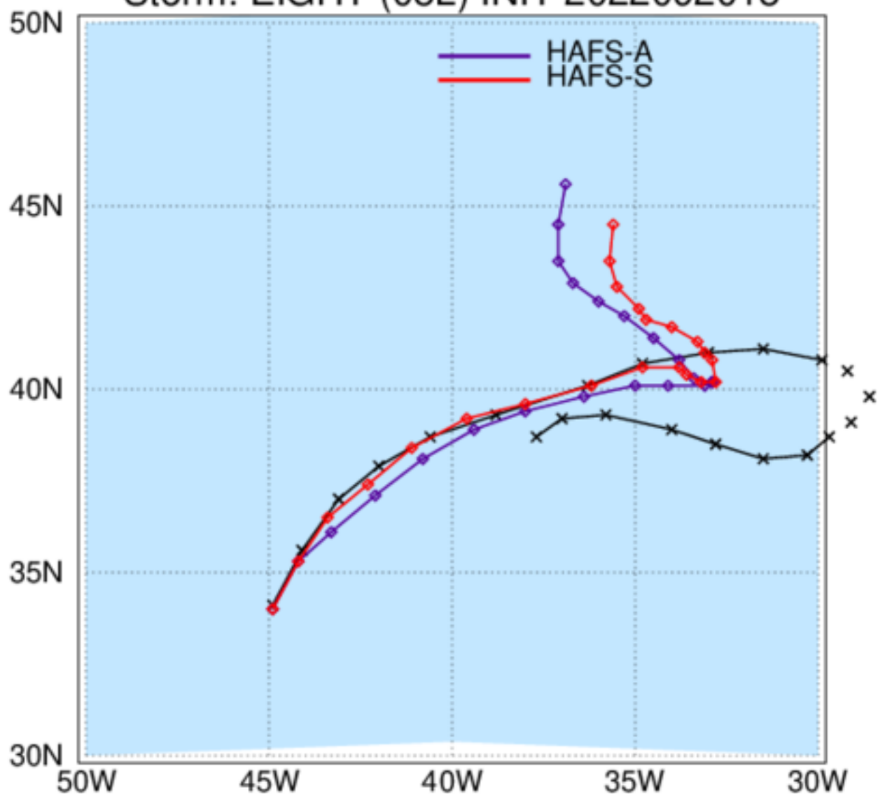
HAFS: TC Tracks Storm: EIGHT (08L) INIT 2022092018
