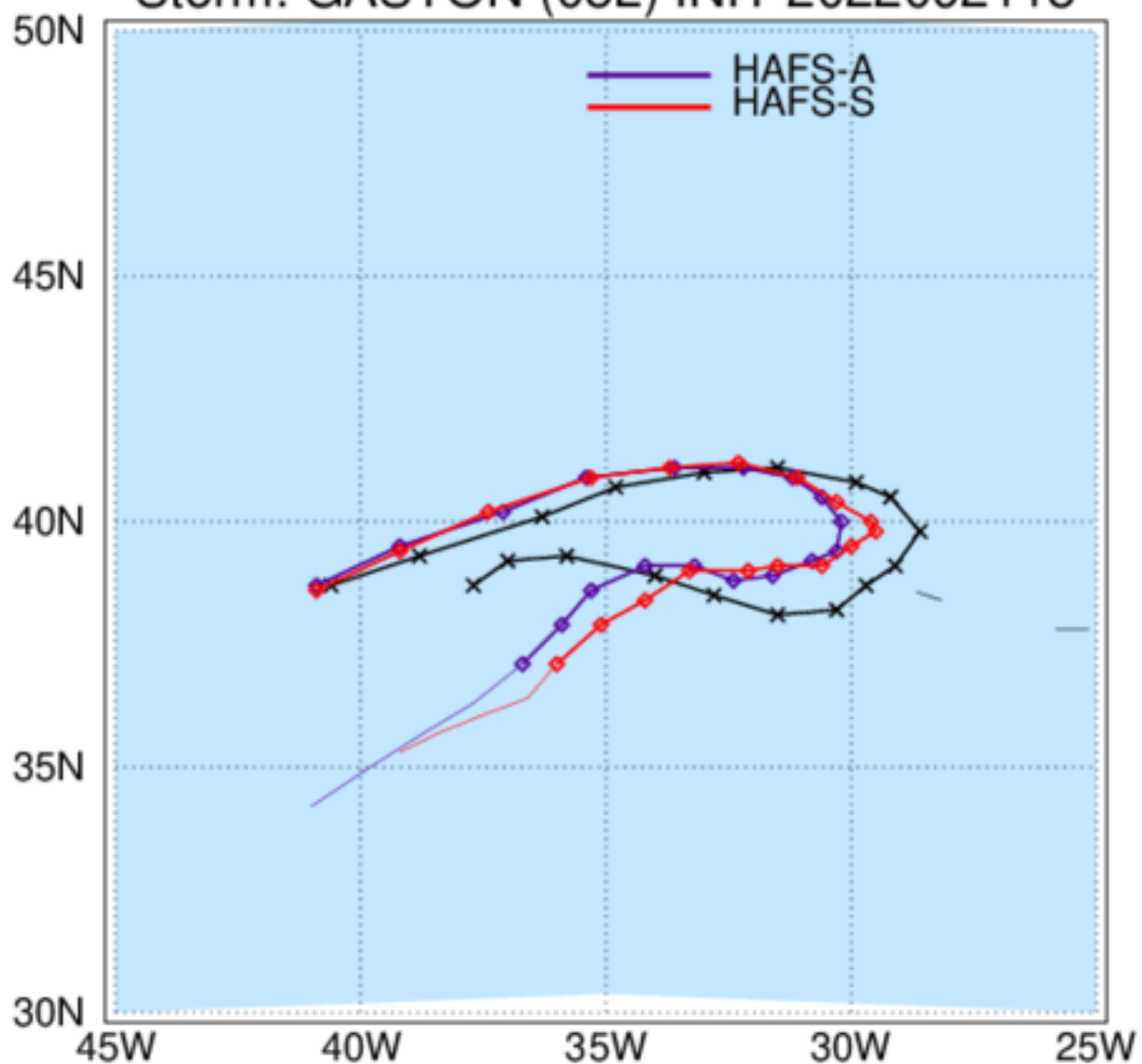
HAFS: TC Tracks Storm: GASTON (08L) INIT 2022092118
