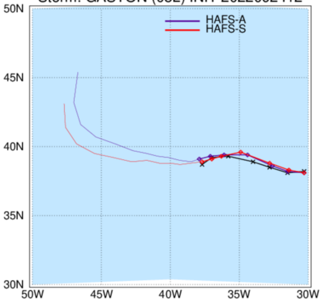
HAFS: TC Tracks Storm: GASTON (08L) INIT 2022092412
