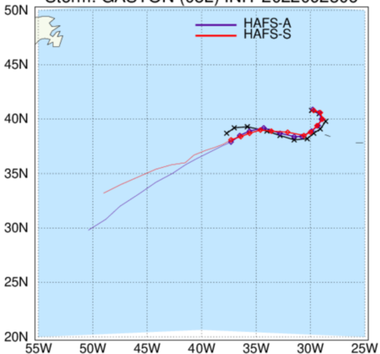
HAFS: TC Tracks Storm: GASTON (08L) INIT 2022092306
