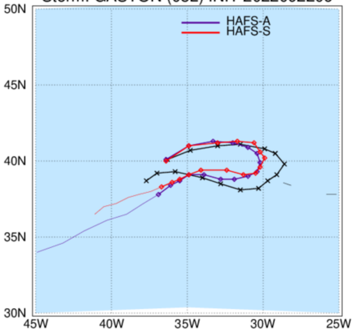
HAFS: TC Tracks Storm: GASTON (08L) INIT 2022092206
