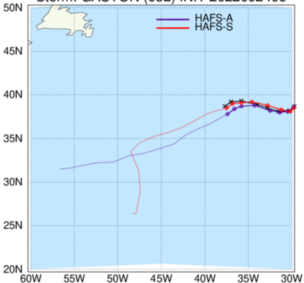
HAFS: TC Tracks Storm: GASTON (08L) INIT 2022092406
