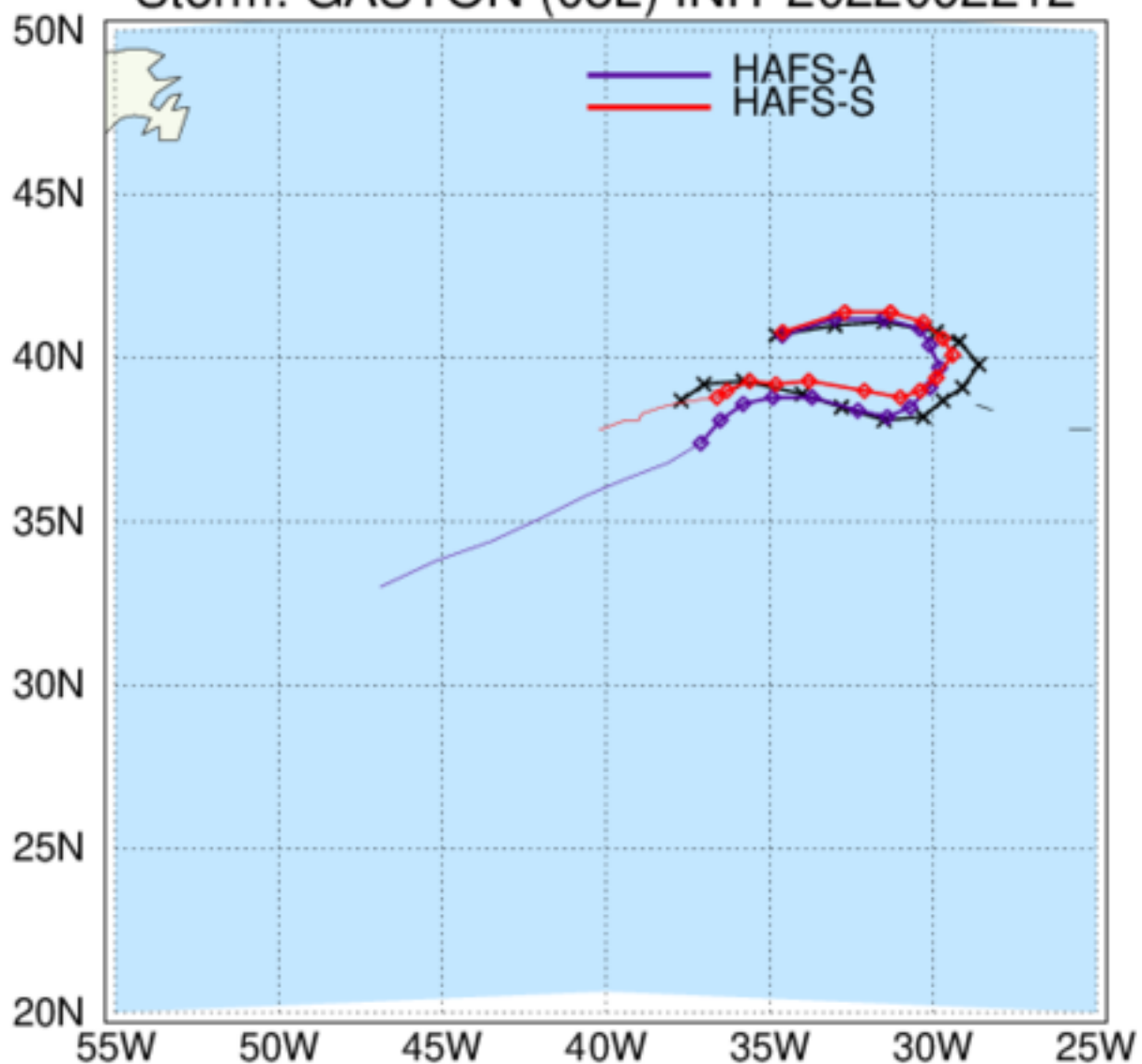
HAFS: TC Tracks Storm: GASTON (08L) INIT 2022092212
