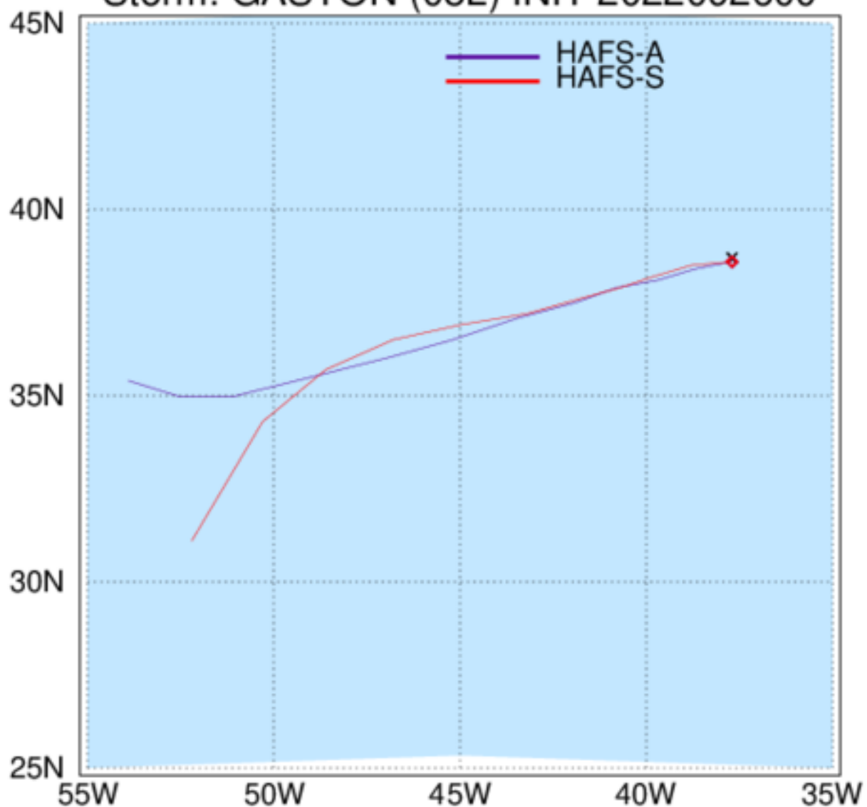
HAFS: TC Tracks Storm: GASTON (08L) INIT 2022092600
