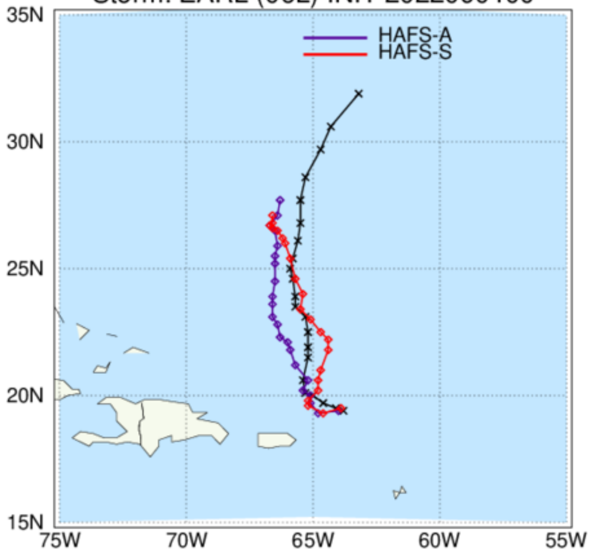
HAFS: TC Tracks Storm: EARL (06L) INIT 2022090400
