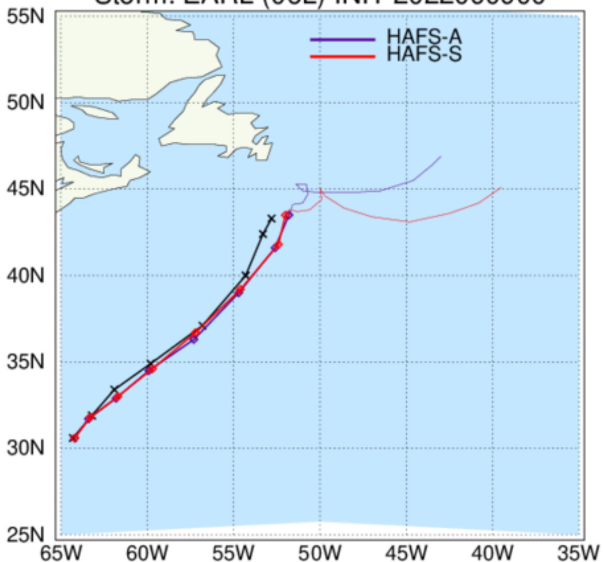
HAFS: TC Tracks Storm: EARL (06L) INIT 2022090900
