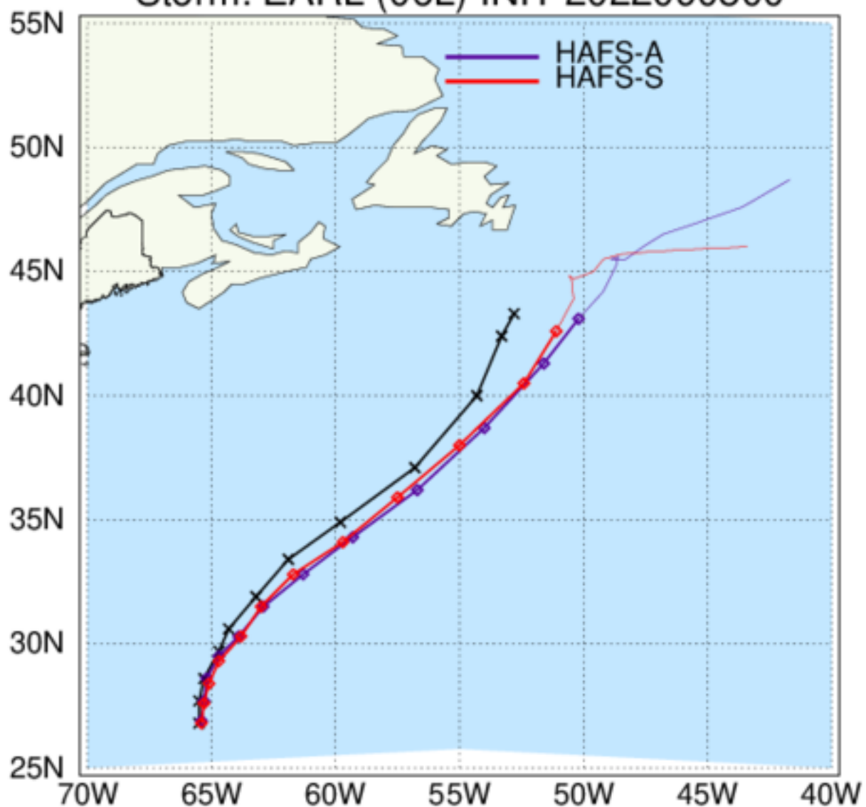
HAFS: TC Tracks Storm: EARL (06L) INIT 2022090800
