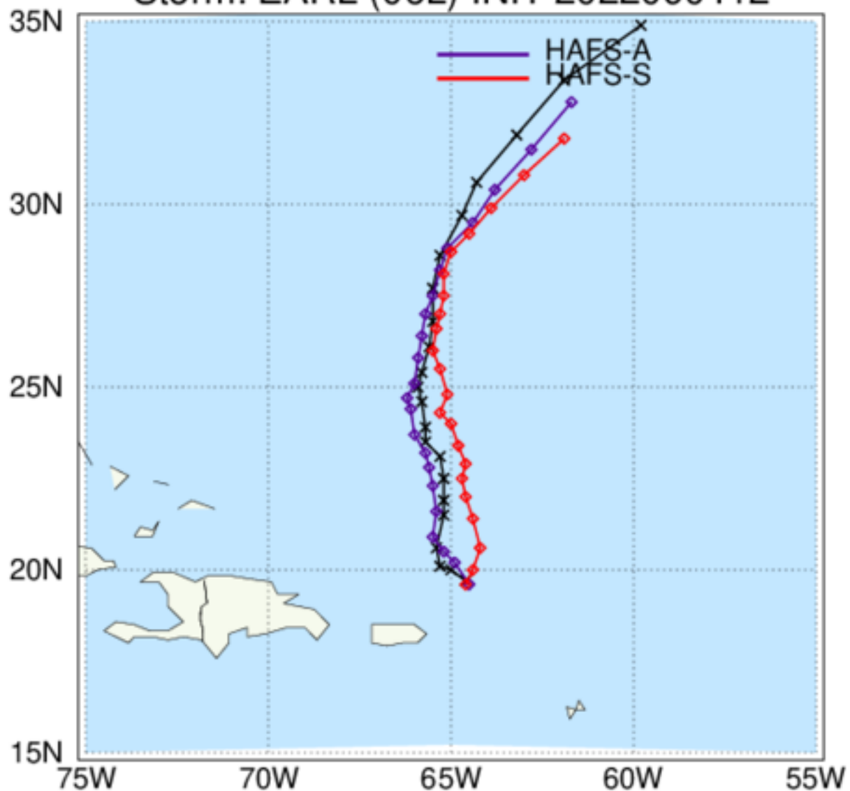
HAFS: TC Tracks Storm: EARL (06L) INIT 2022090412
