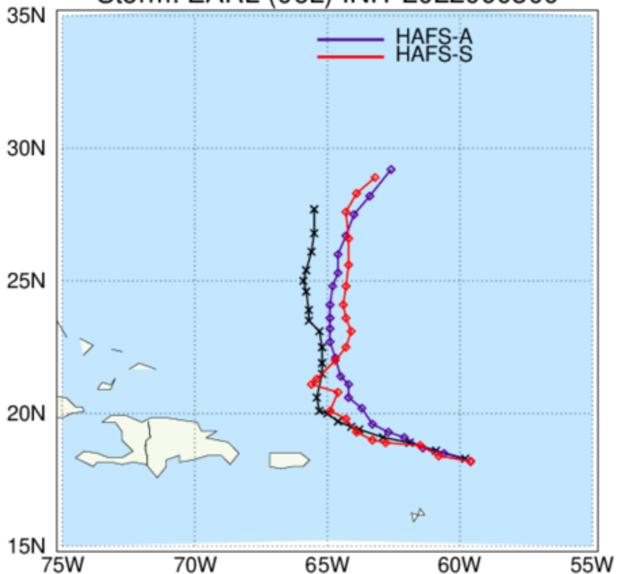
HAFS: TC Tracks Storm: EARL (06L) INIT 2022090300
