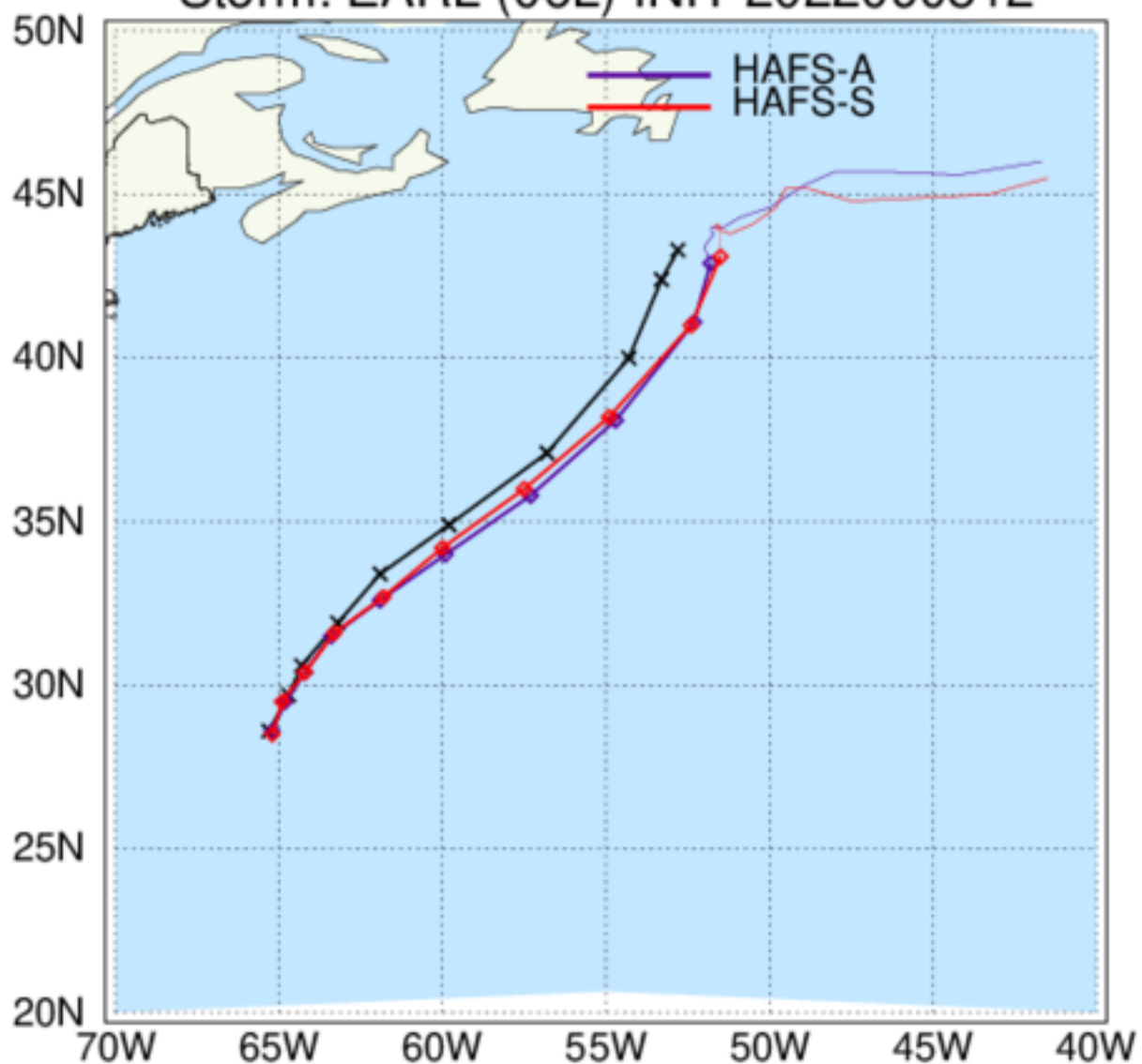
HAFS: TC Tracks Storm: EARL (06L) INIT 2022090812
