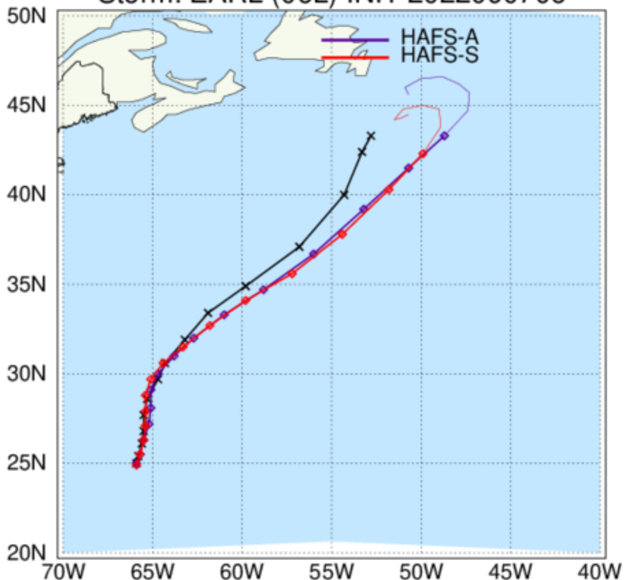
HAFS: TC Tracks Storm: EARL (06L) INIT 2022090706
