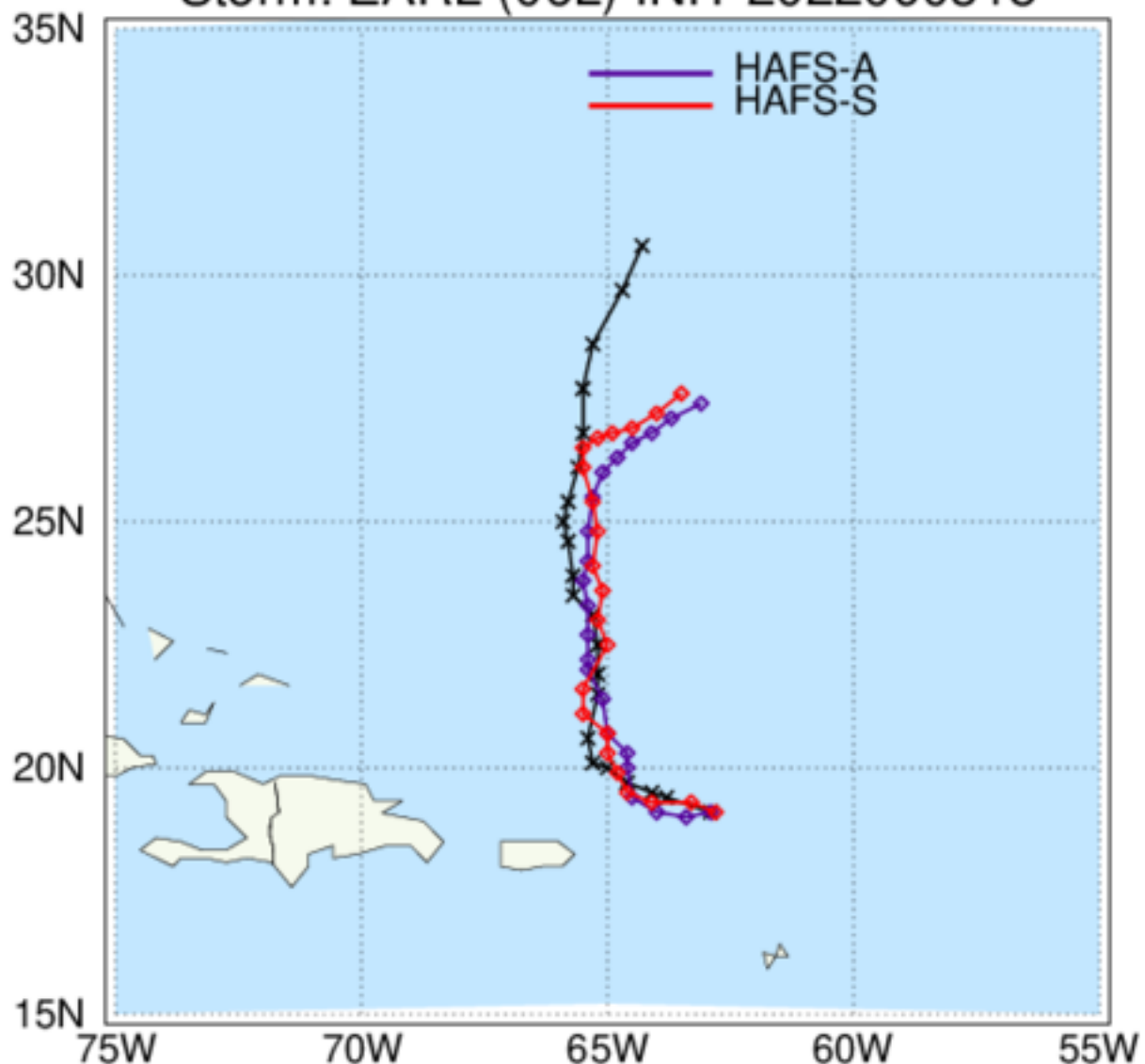
HAFS: TC Tracks Storm: EARL (06L) INIT 2022090318
