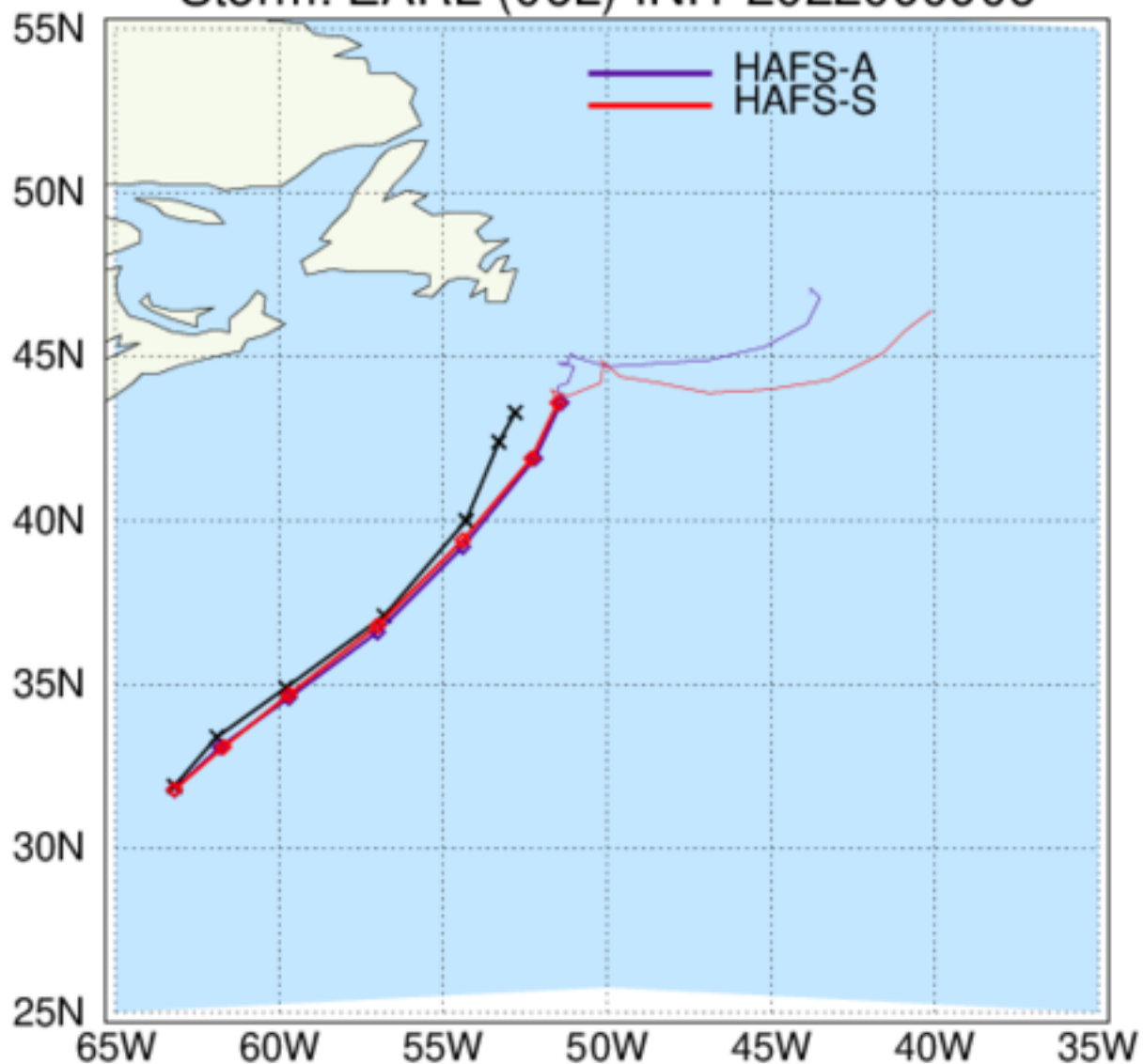
HAFS: TC Tracks Storm: EARL (06L) INIT 2022090906
