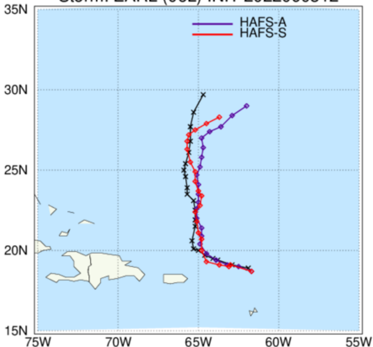
HAFS: TC Tracks Storm: EARL (06L) INIT 2022090312
