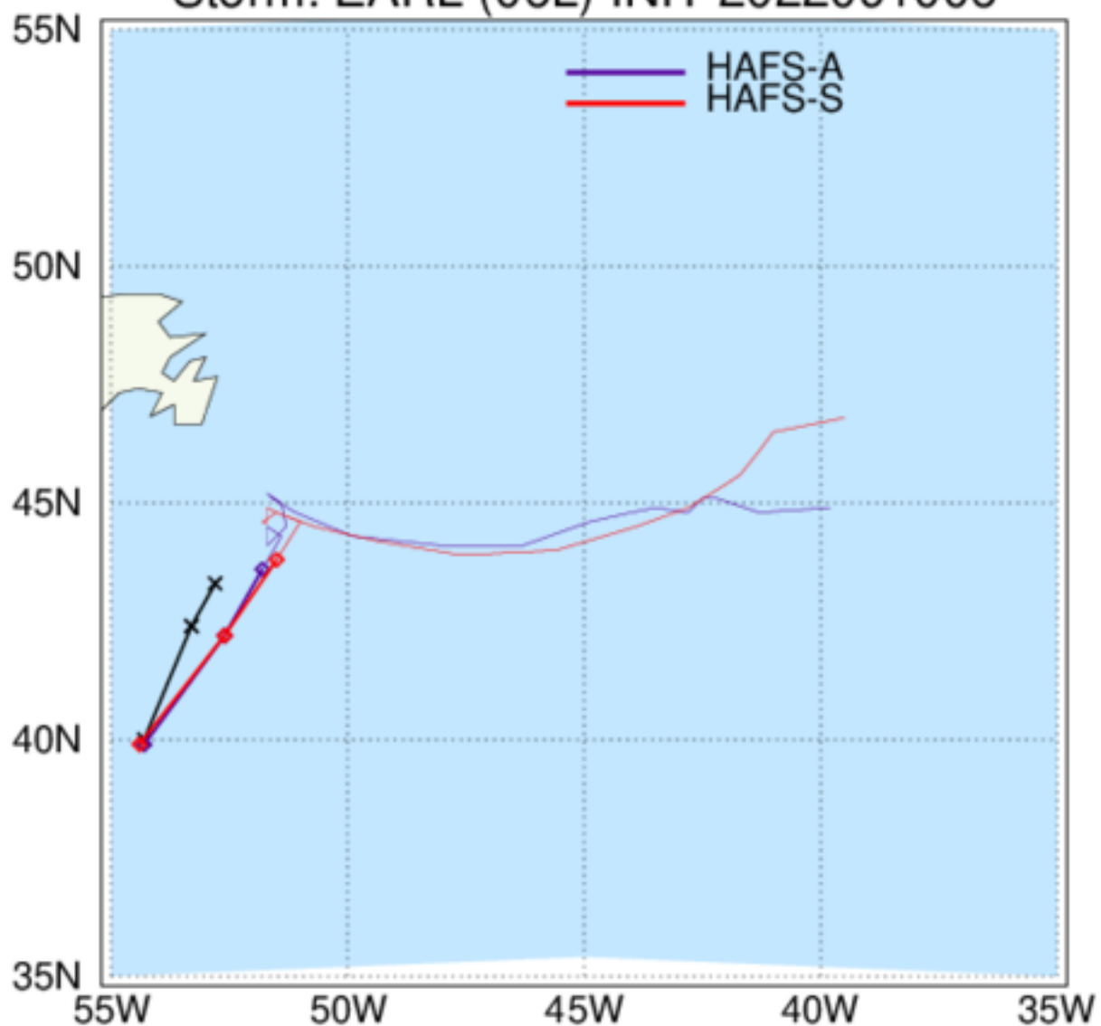
HAFS: TC Tracks Storm: EARL (06L) INIT 2022091006
