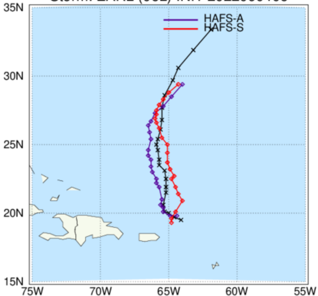
HAFS: TC Tracks Storm: EARL (06L) INIT 2022090406
