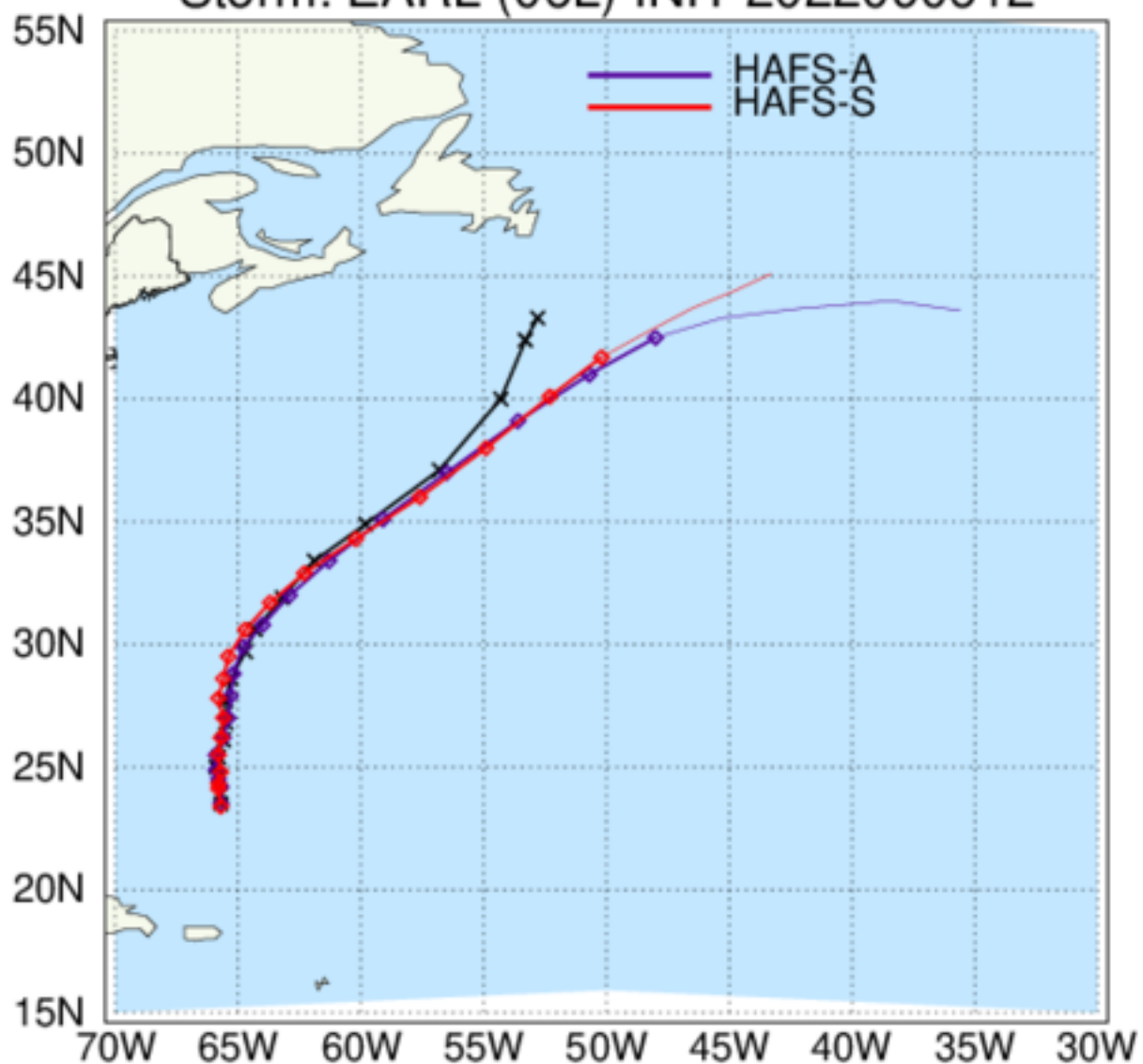
HAFS: TC Tracks Storm: EARL (06L) INIT 2022090612
