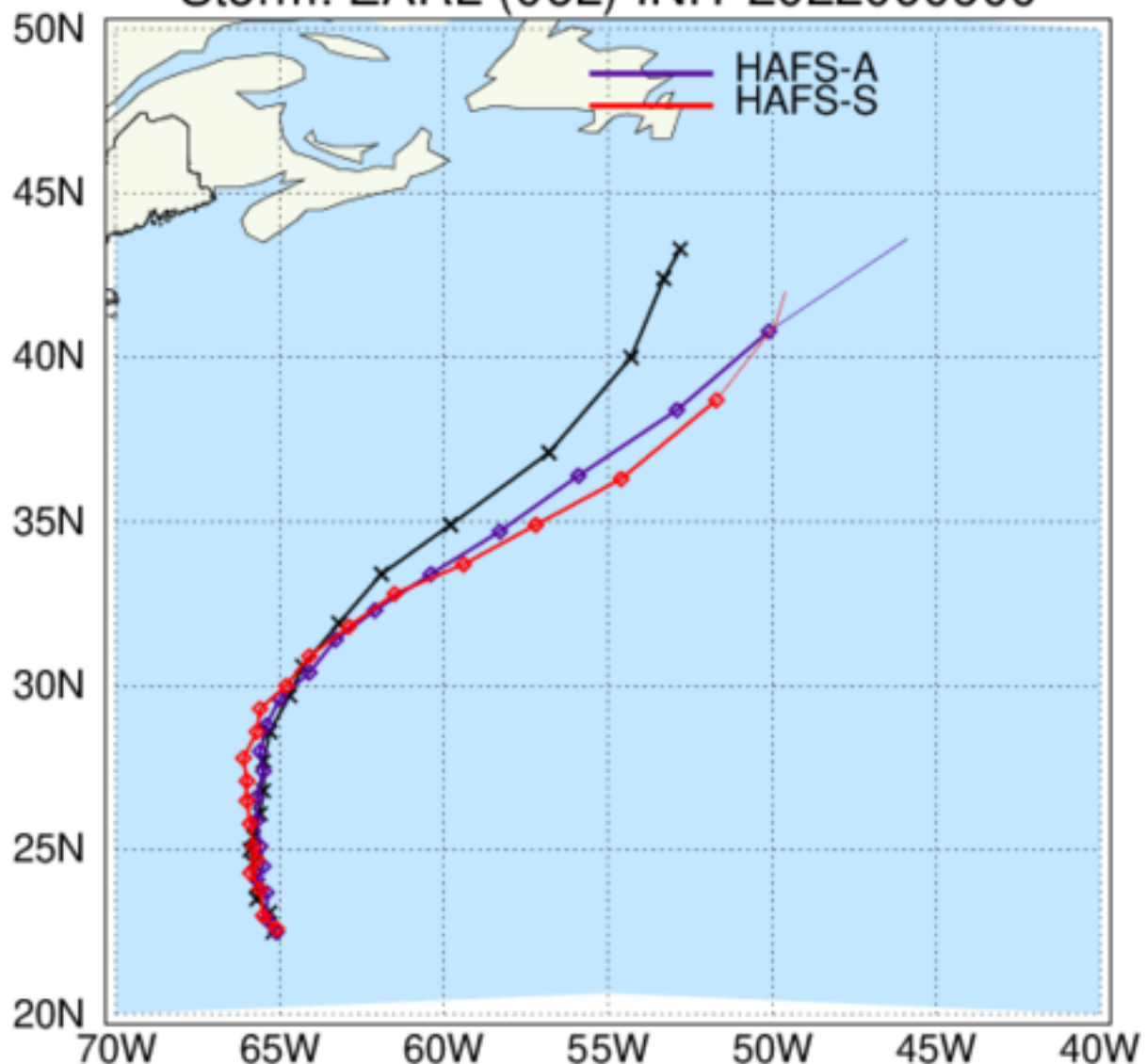
HAFS: TC Tracks Storm: EARL (06L) INIT 2022090600
