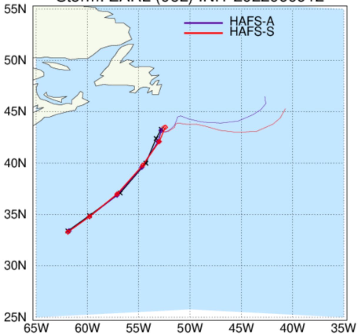
HAFS: TC Tracks Storm: EARL (06L) INIT 2022090912
