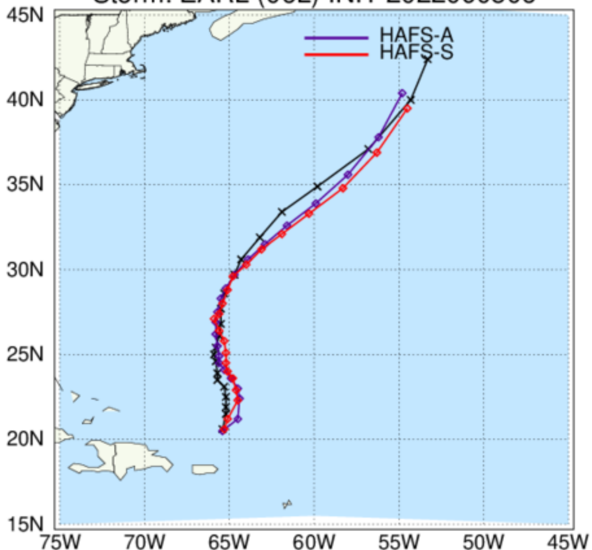
HAFS: TC Tracks Storm: EARL (06L) INIT 2022090506
