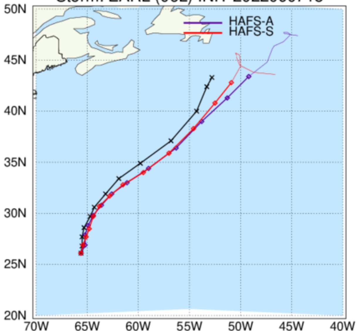
HAFS: TC Tracks Storm: EARL (06L) INIT 2022090718
