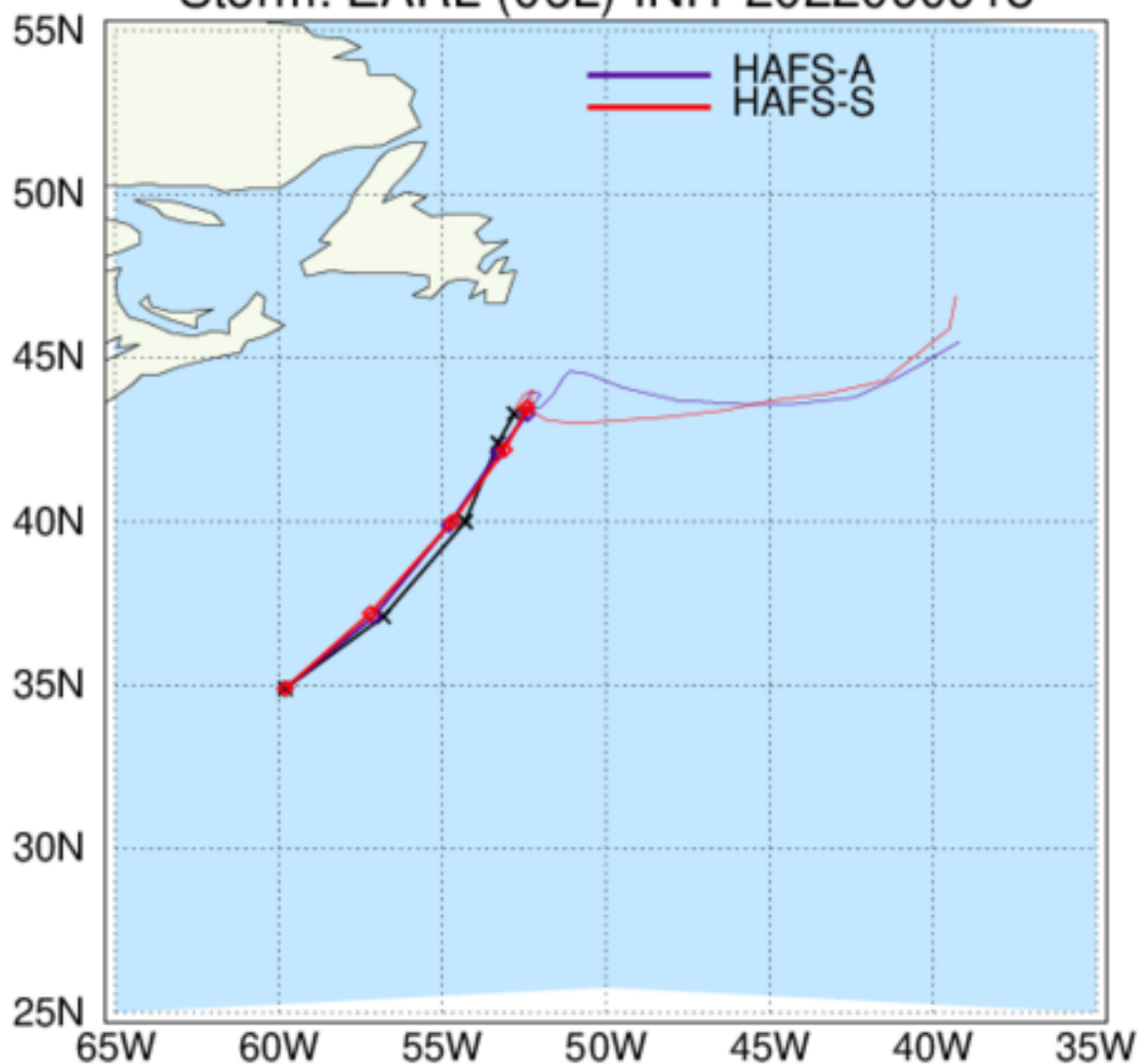
HAFS: TC Tracks Storm: EARL (06L) INIT 2022090918
