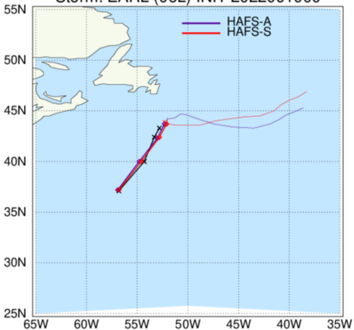
HAFS: TC Tracks Storm: EARL (06L) INIT 2022091000
