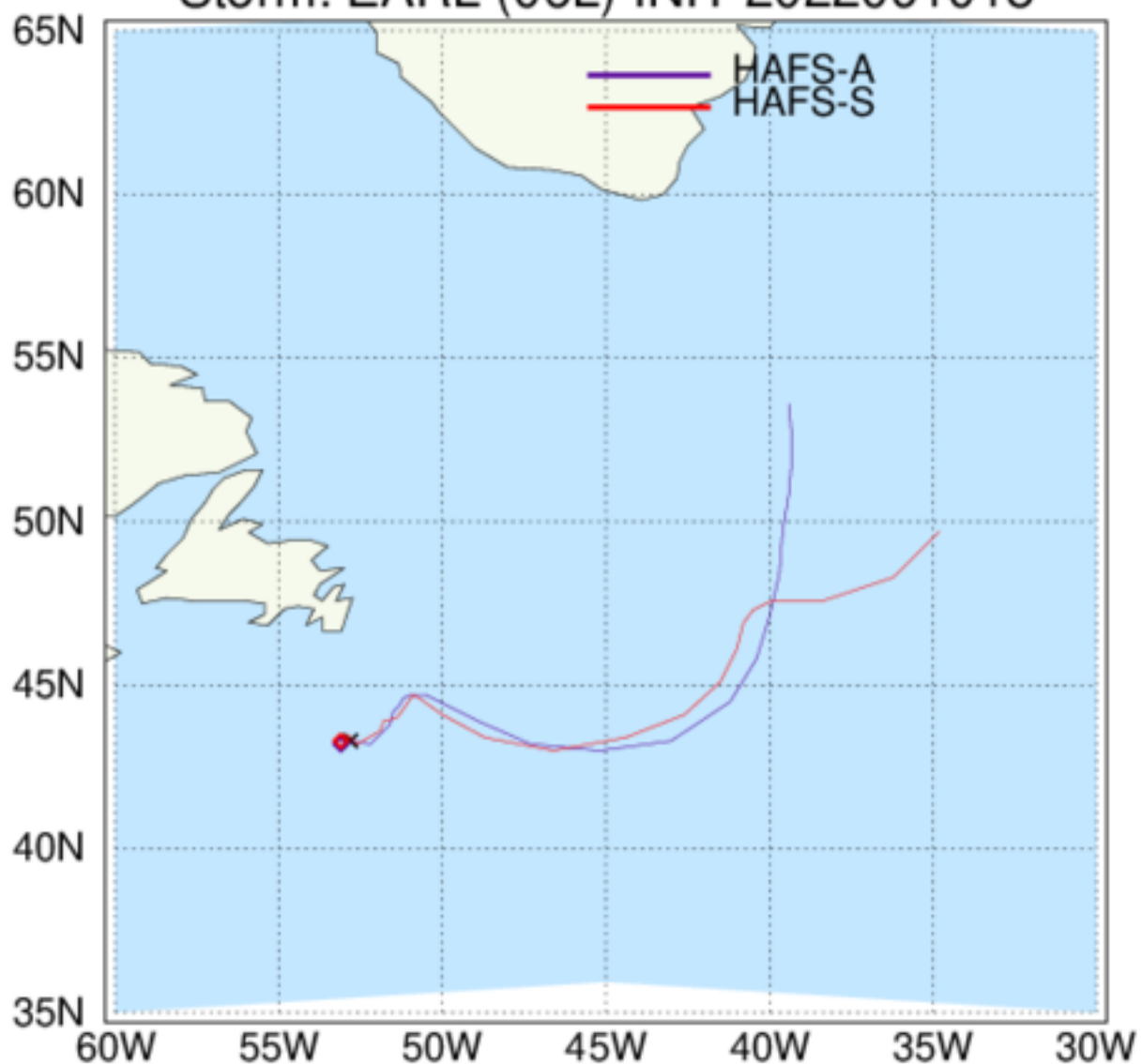
HAFS: TC Tracks Storm: EARL (06L) INIT 2022091018
