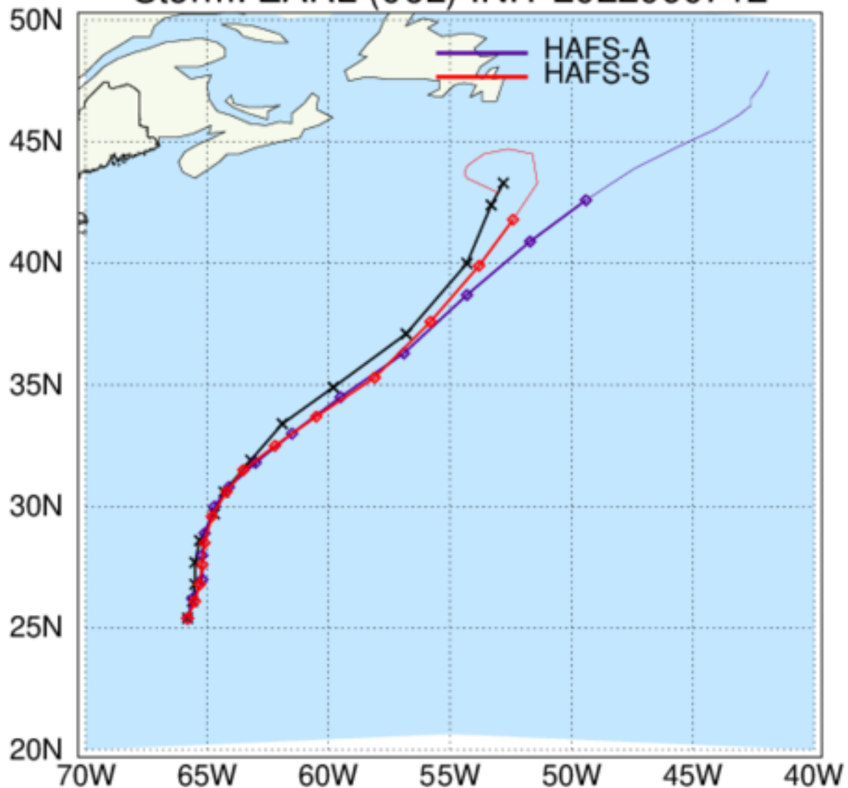
HAFS: TC Tracks Storm: EARL (06L) INIT 2022090712
