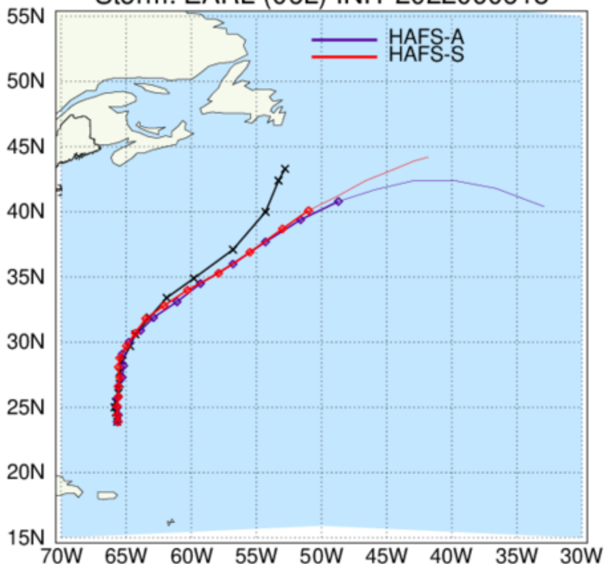
HAFS: TC Tracks Storm: EARL (06L) INIT 2022090618
