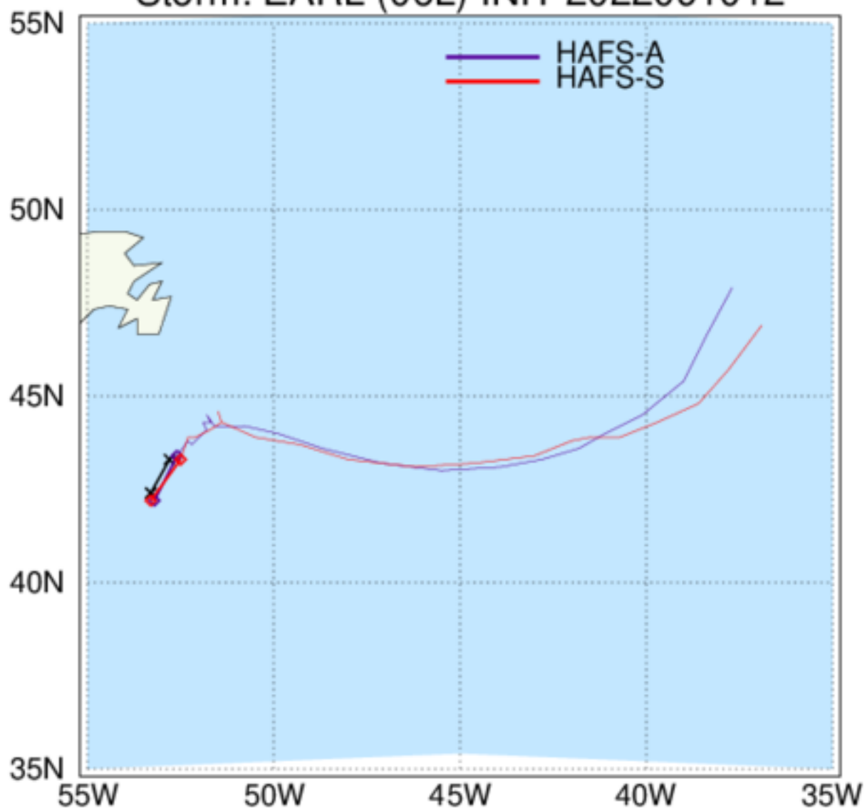
HAFS: TC Tracks Storm: EARL (06L) INIT 2022091012
