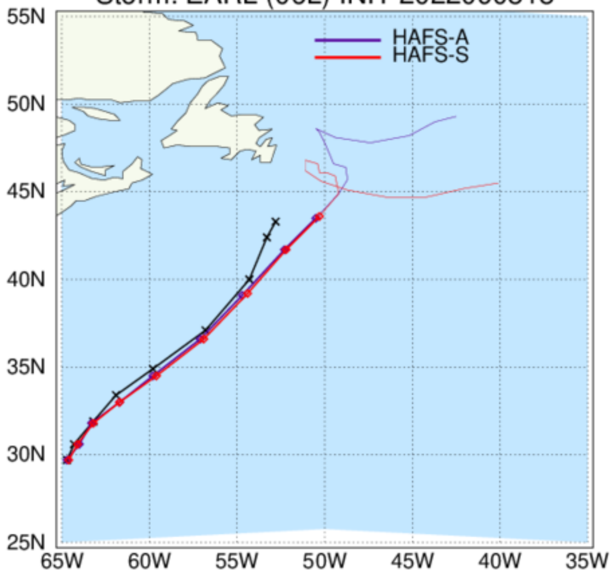
HAFS: TC Tracks Storm: EARL (06L) INIT 2022090818
