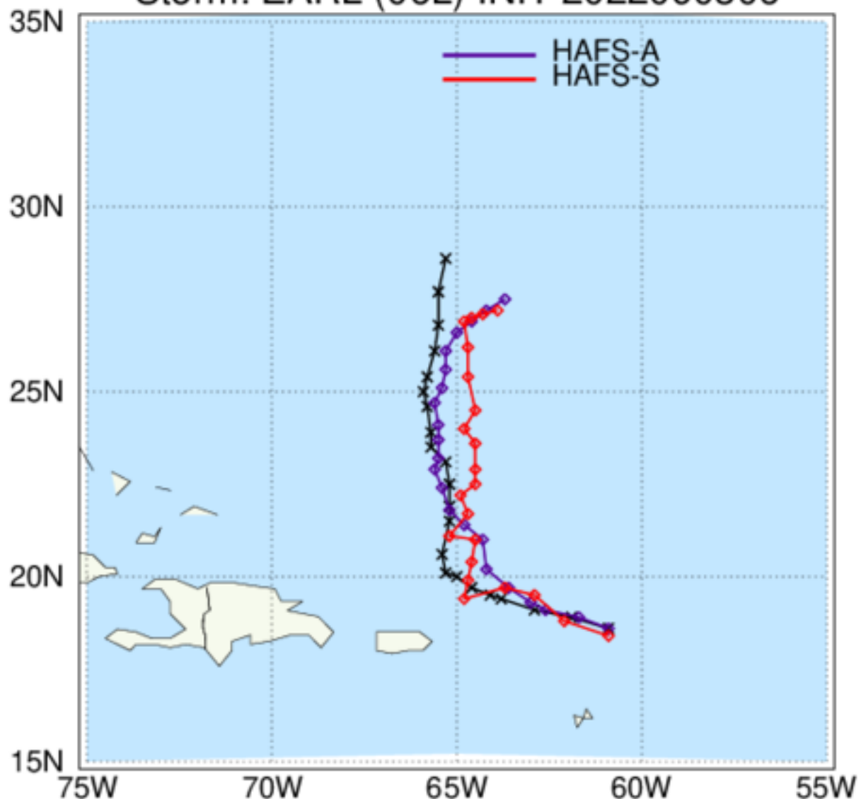
HAFS: TC Tracks Storm: EARL (06L) INIT 2022090306
