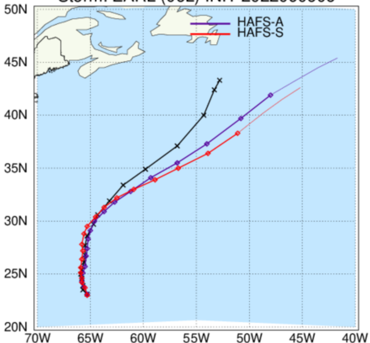
HAFS: TC Tracks Storm: EARL (06L) INIT 2022090606
