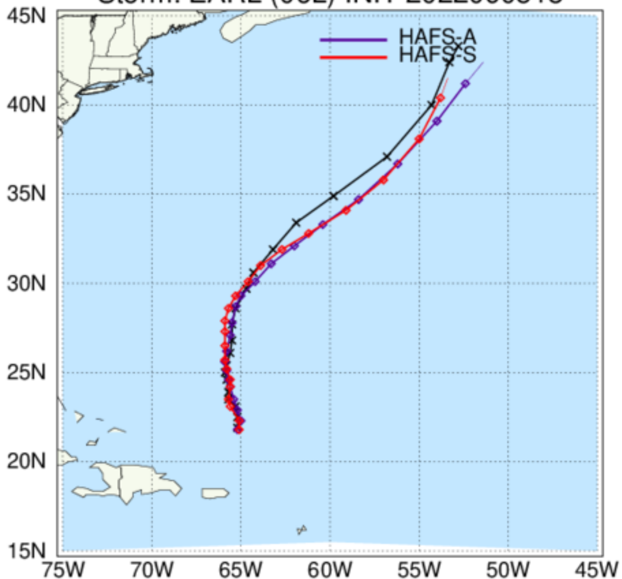
HAFS: TC Tracks Storm: EARL (06L) INIT 2022090518
