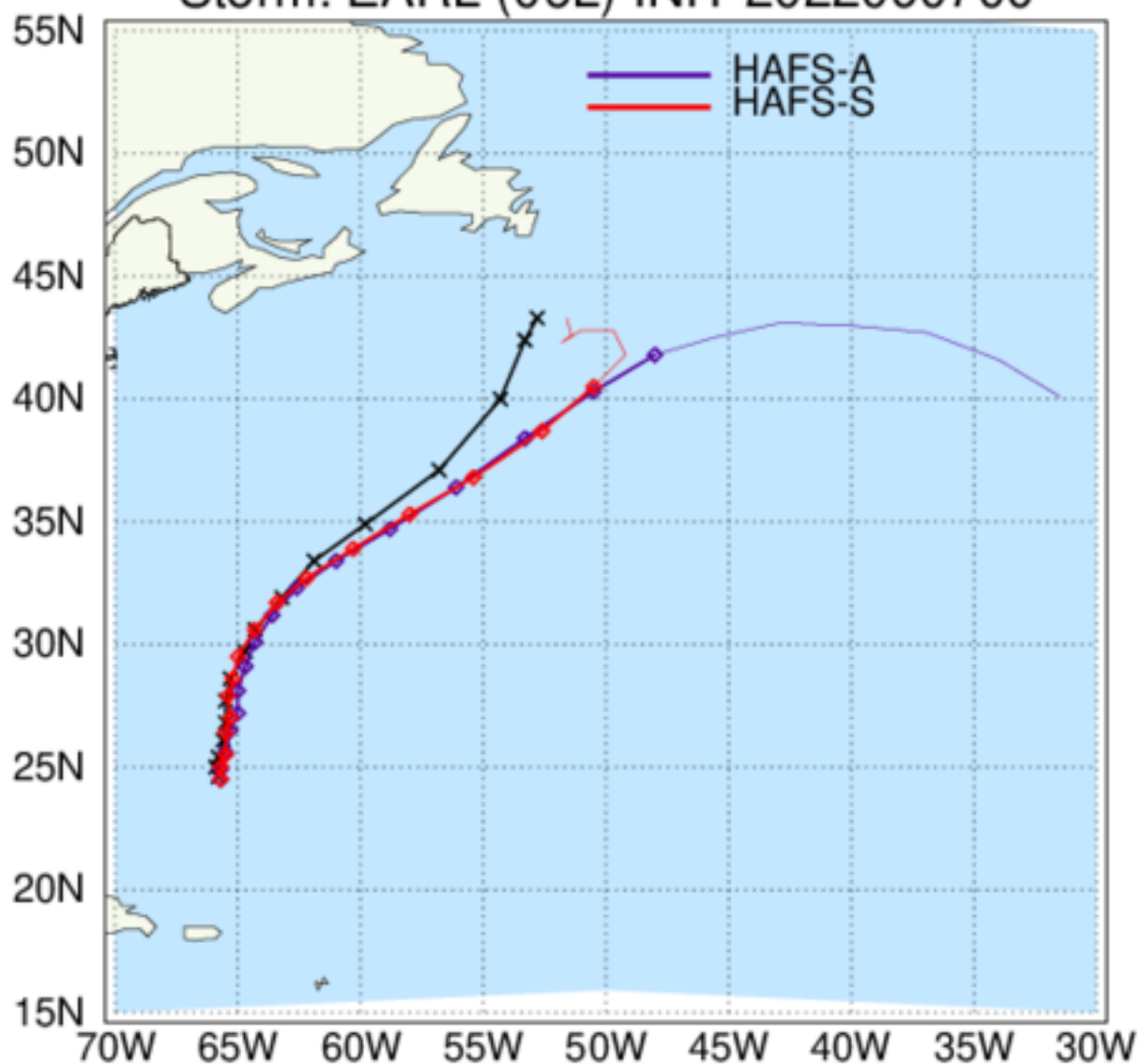
HAFS: TC Tracks Storm: EARL (06L) INIT 2022090700
