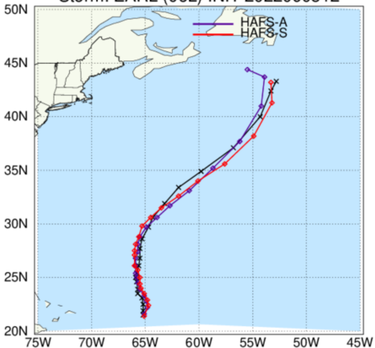
HAFS: TC Tracks Storm: EARL (06L) INIT 2022090512
