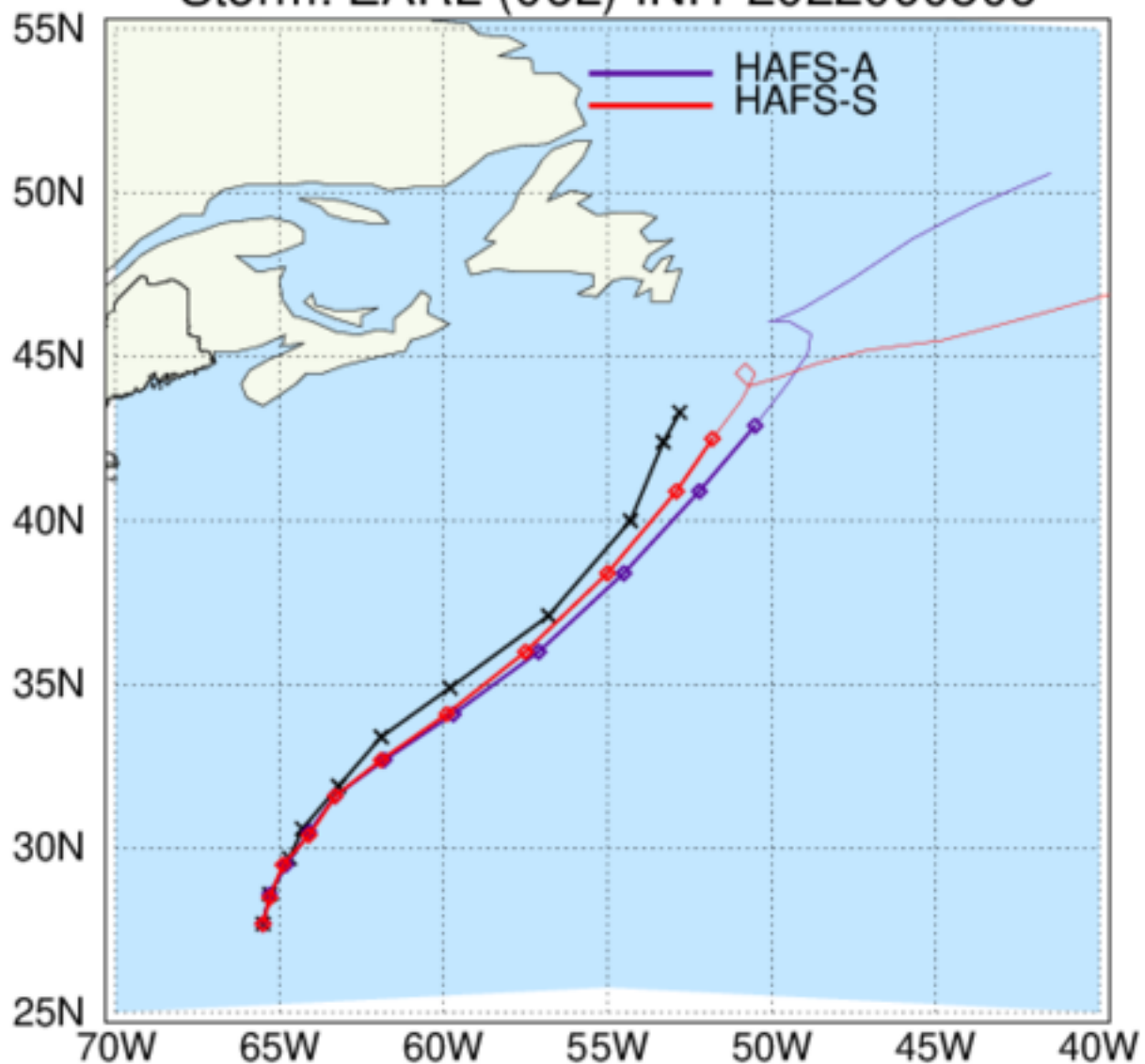
HAFS: TC Tracks Storm: EARL (06L) INIT 2022090806
