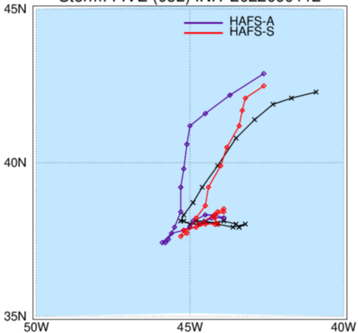
HAFS: TC Tracks Storm: FIVE (05L) INIT 2022090112
