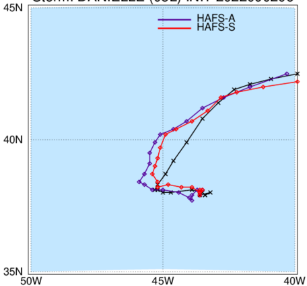
HAFS: TC Tracks Storm: DANIELLE (05L) INIT 2022090206
