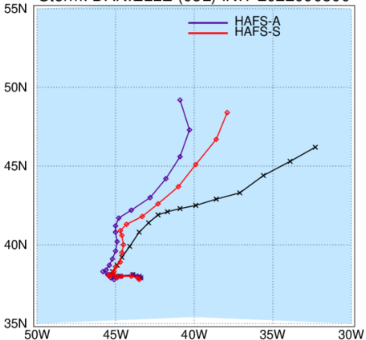
HAFS: TC Tracks Storm: DANIELLE (05L) INIT 2022090300
