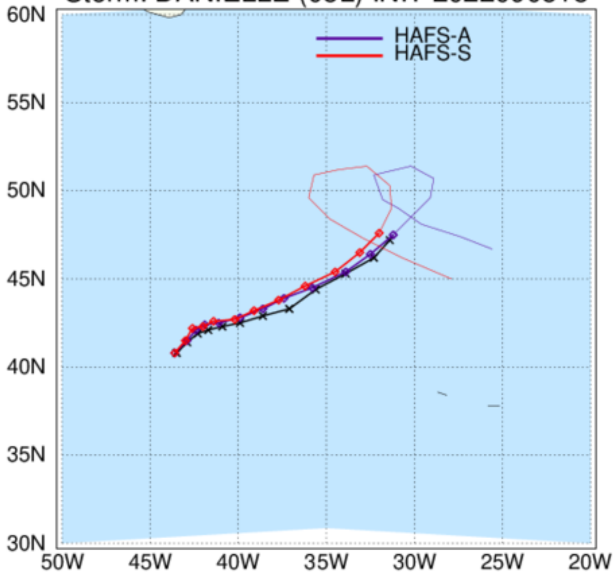
HAFS: TC Tracks Storm: DANIELLE (05L) INIT 2022090518
