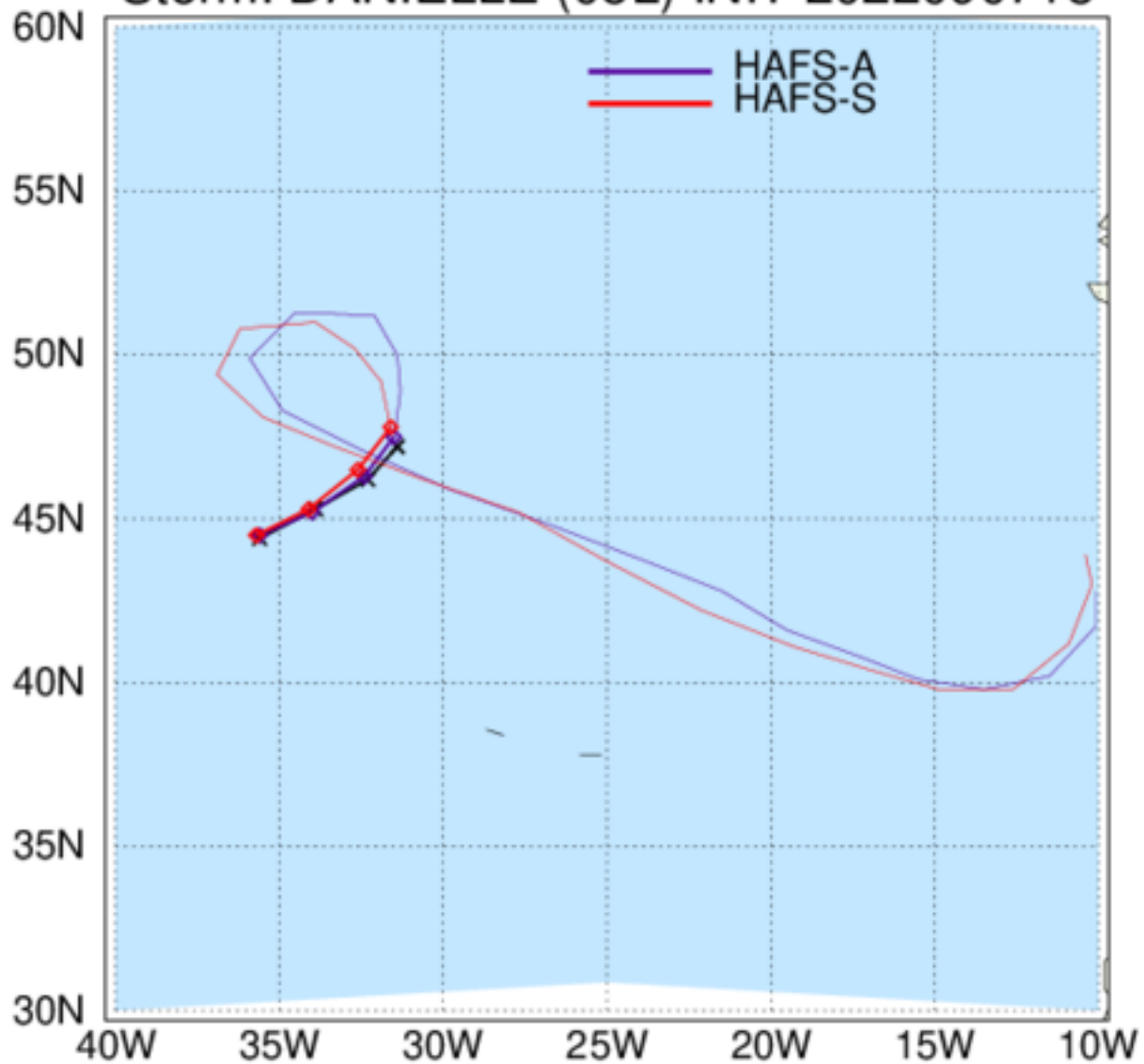
HAFS: TC Tracks Storm: DANIELLE (05L) INIT 2022090718
