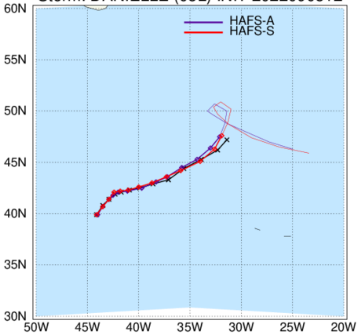
HAFS: TC Tracks Storm: DANIELLE (05L) INIT 2022090512
