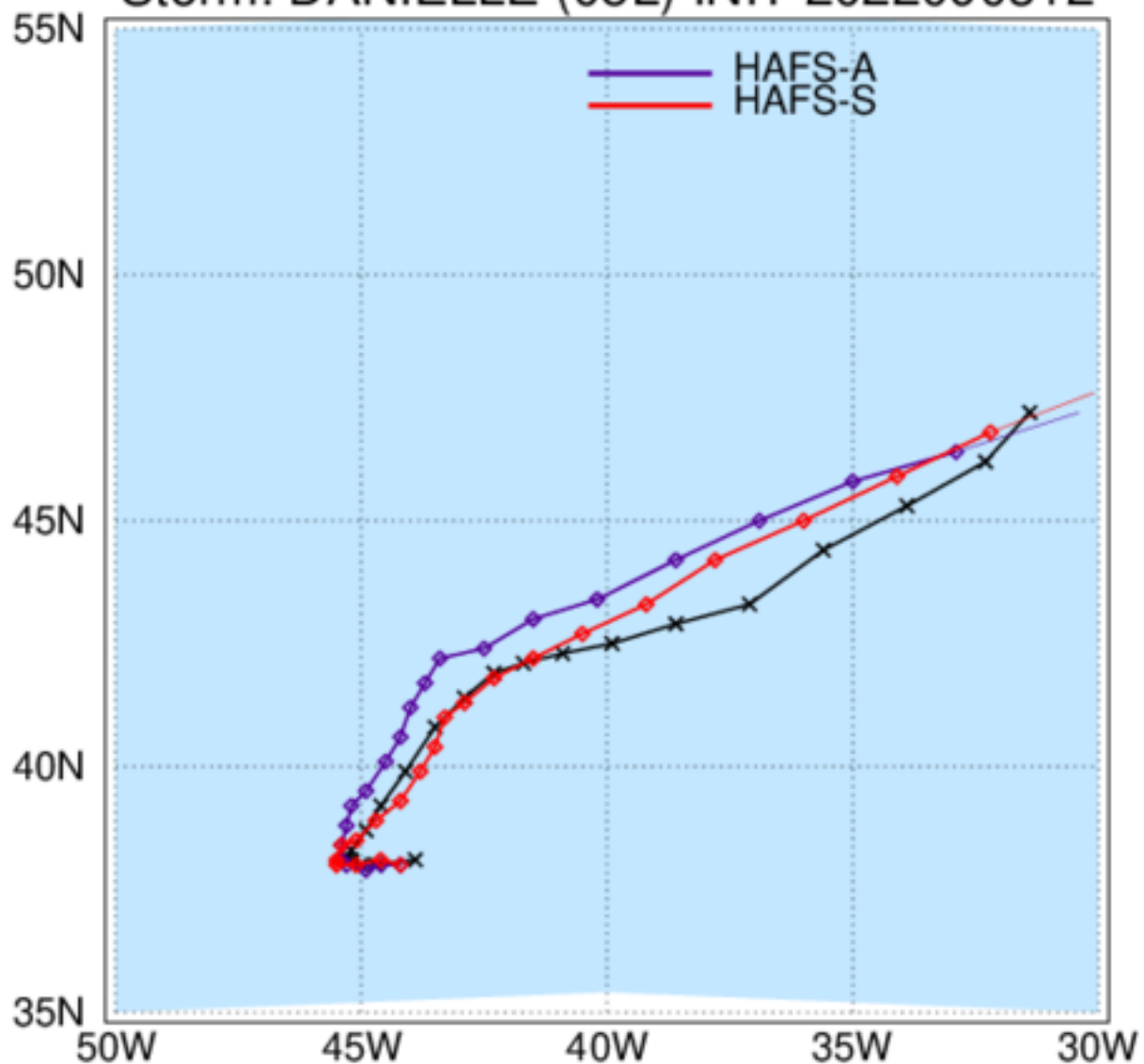
HAFS: TC Tracks Storm: DANIELLE (05L) INIT 2022090312
