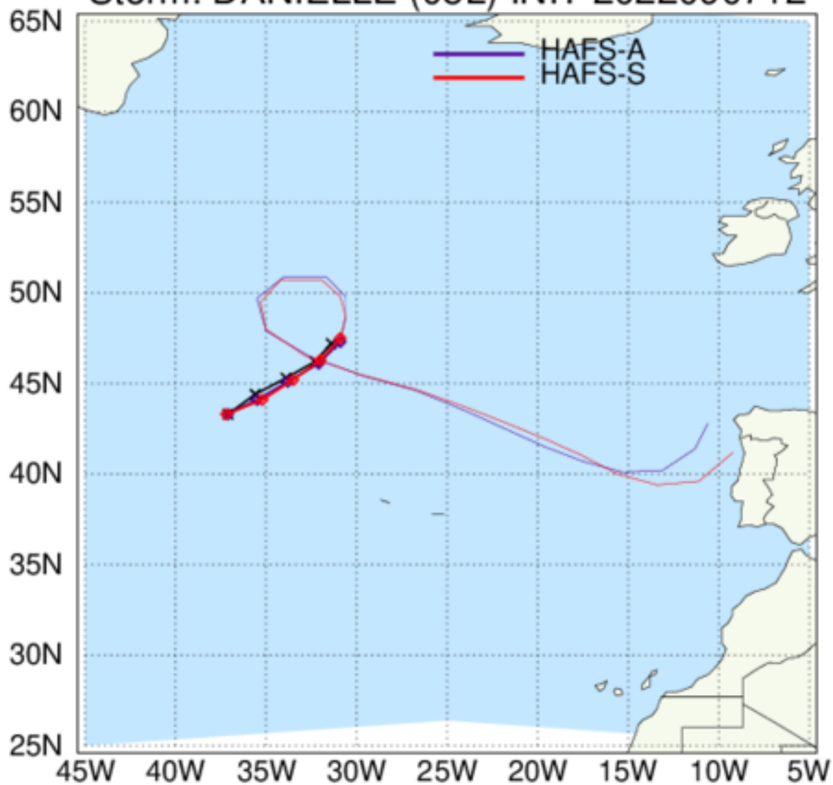
HAFS: TC Tracks Storm: DANIELLE (05L) INIT 2022090712
