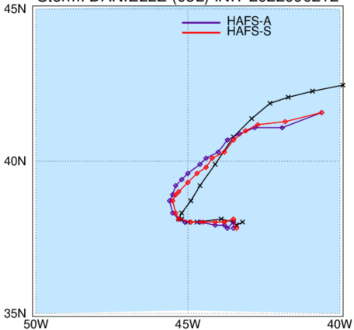
HAFS: TC Tracks Storm: DANIELLE (05L) INIT 2022090212
