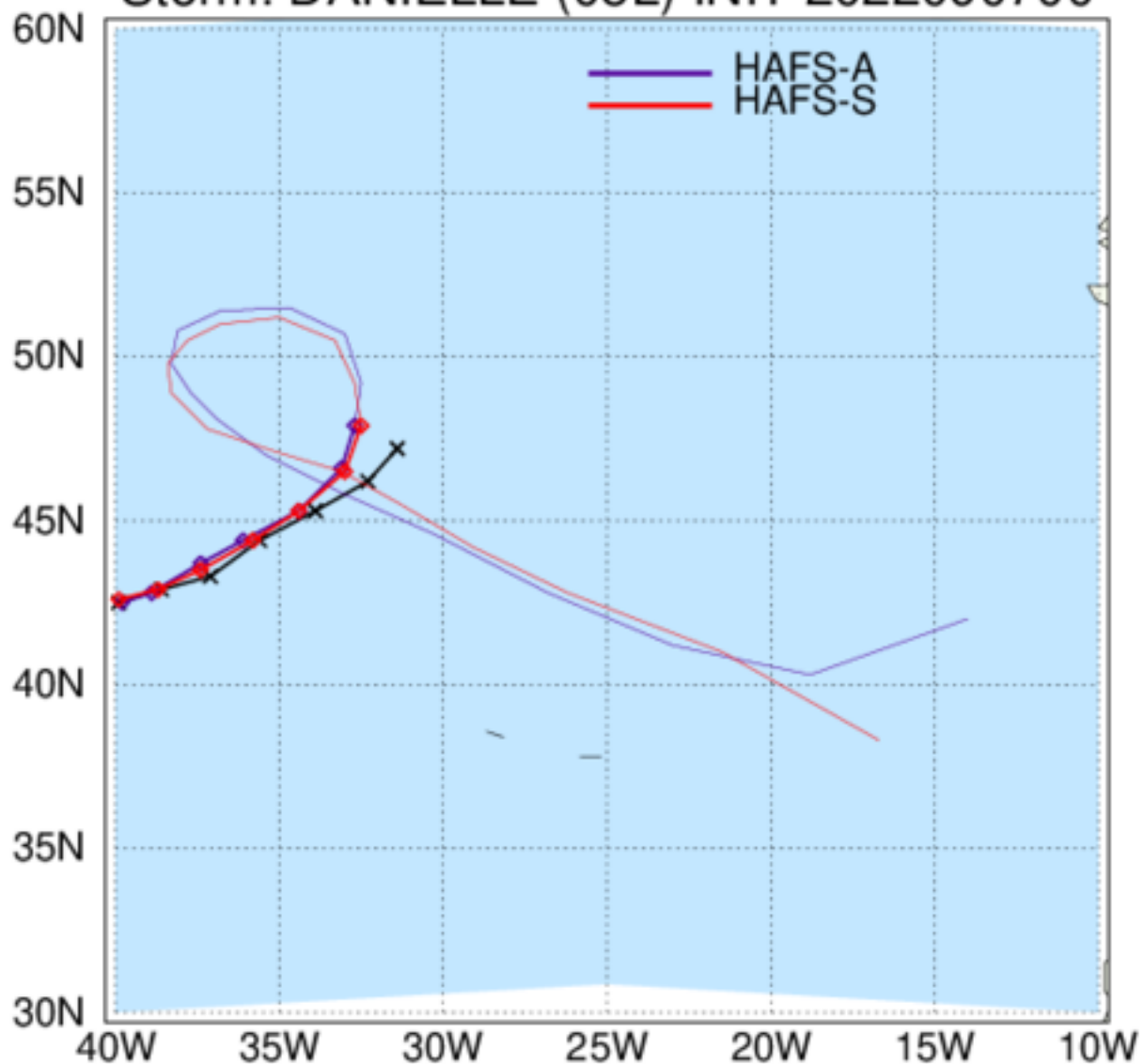
HAFS: TC Tracks Storm: DANIELLE (05L) INIT 2022090700
