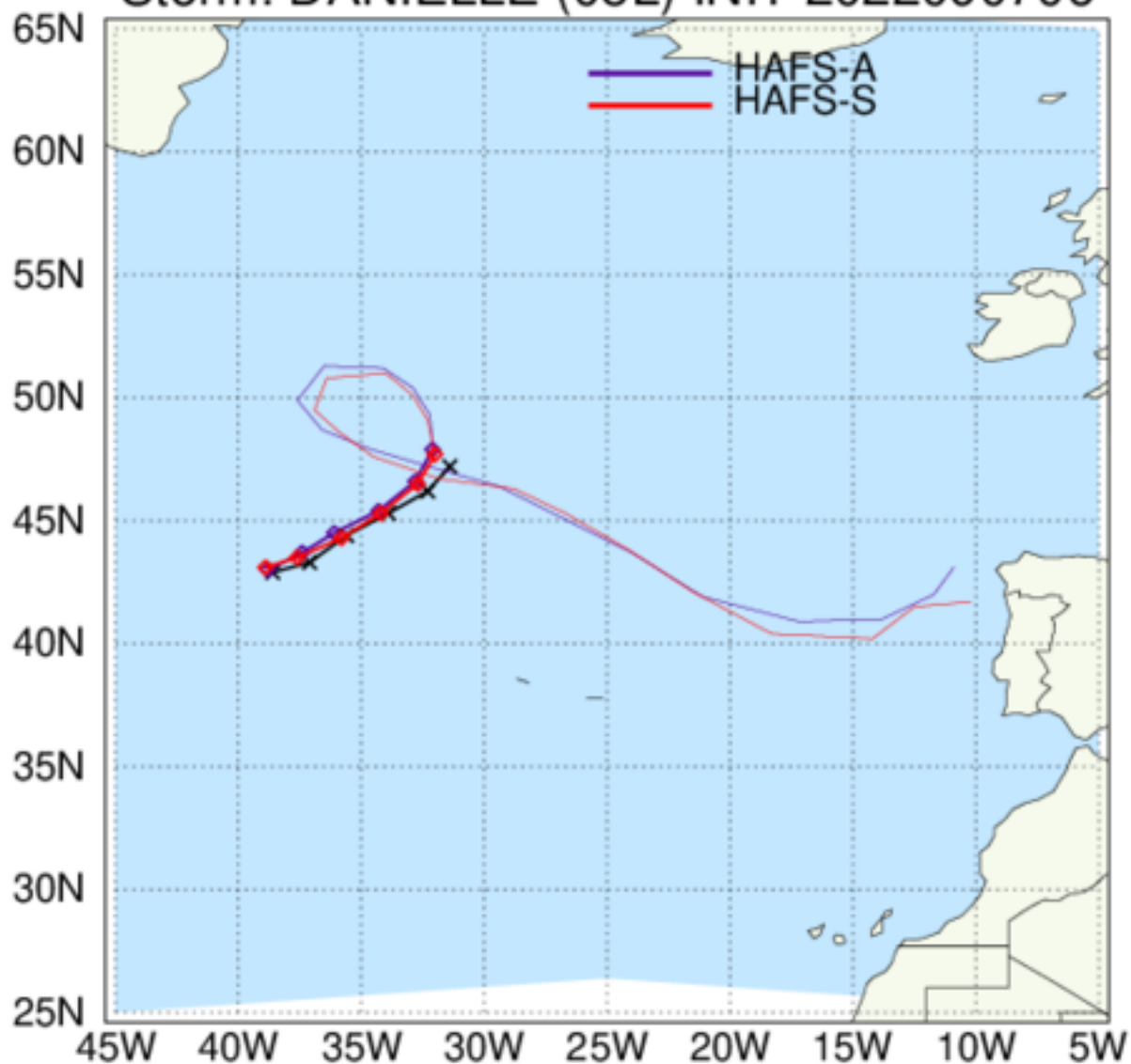
HAFS: TC Tracks Storm: DANIELLE (05L) INIT 2022090706
