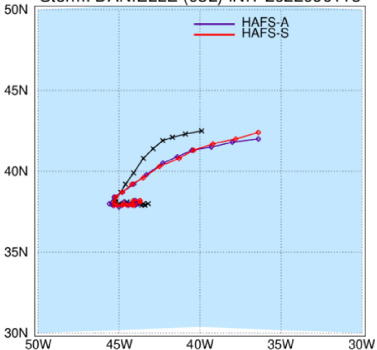
HAFS: TC Tracks Storm: DANIELLE (05L) INIT 2022090118
