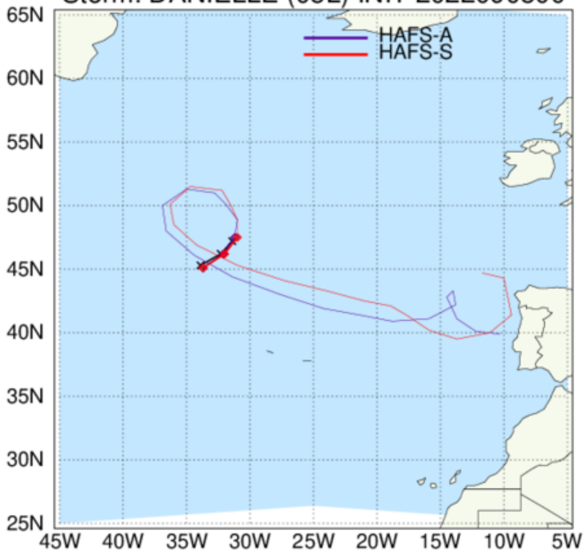
HAFS: TC Tracks Storm: DANIELLE (05L) INIT 2022090800
