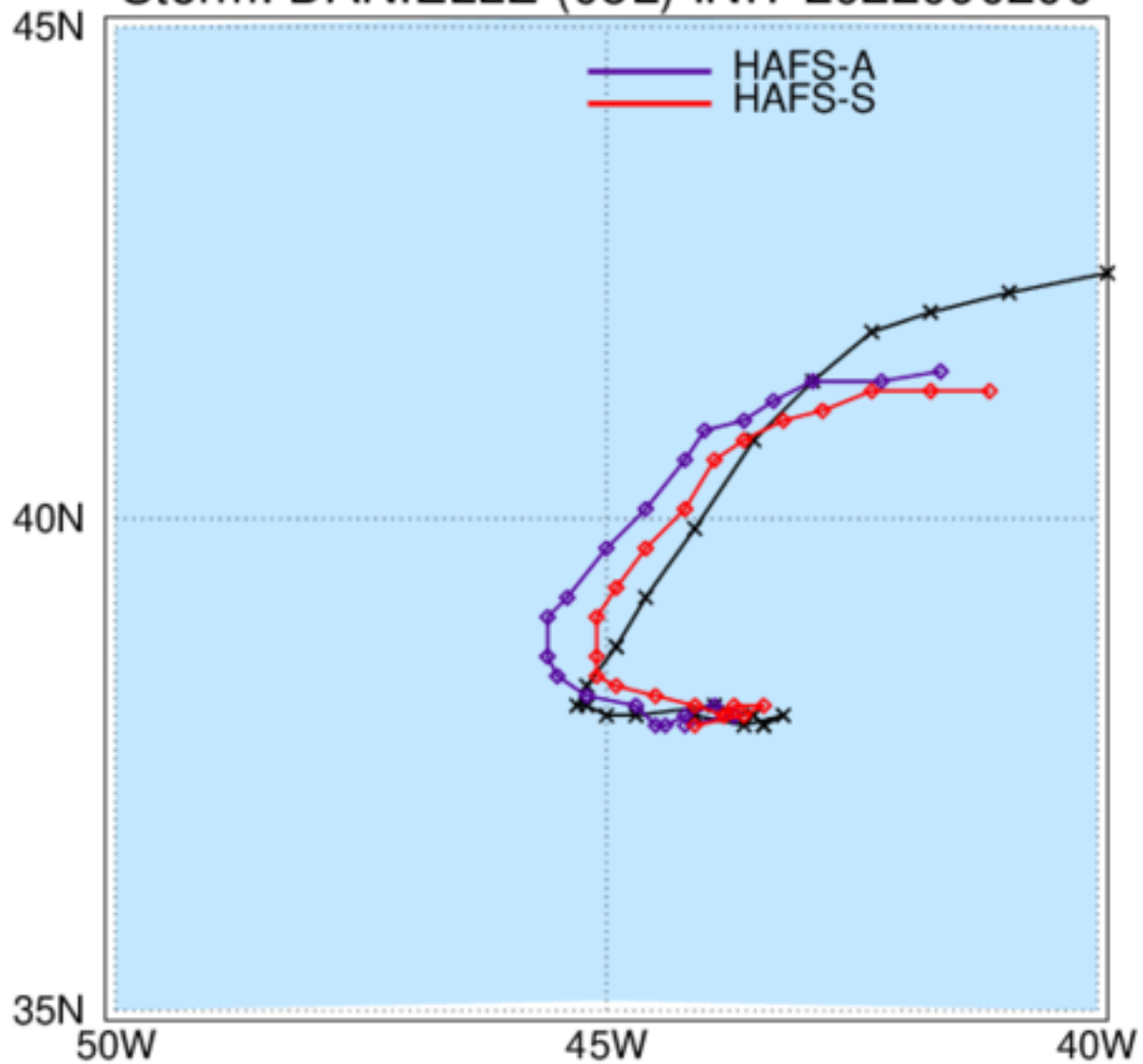
HAFS: TC Tracks Storm: DANIELLE (05L) INIT 2022090200
