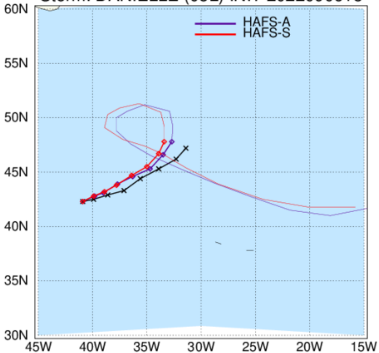
HAFS: TC Tracks Storm: DANIELLE (05L) INIT 2022090618
