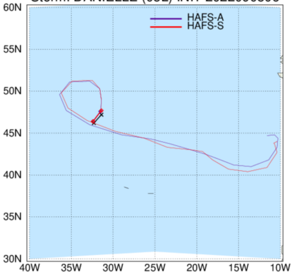
HAFS: TC Tracks Storm: DANIELLE (05L) INIT 2022090806
