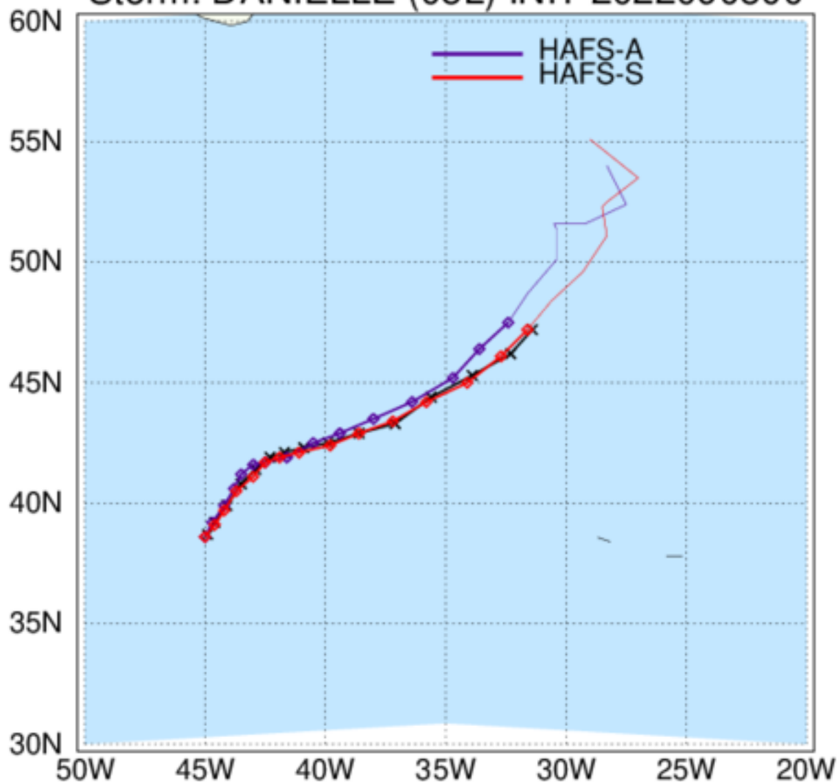
HAFS: TC Tracks Storm: DANIELLE (05L) INIT 2022090500
