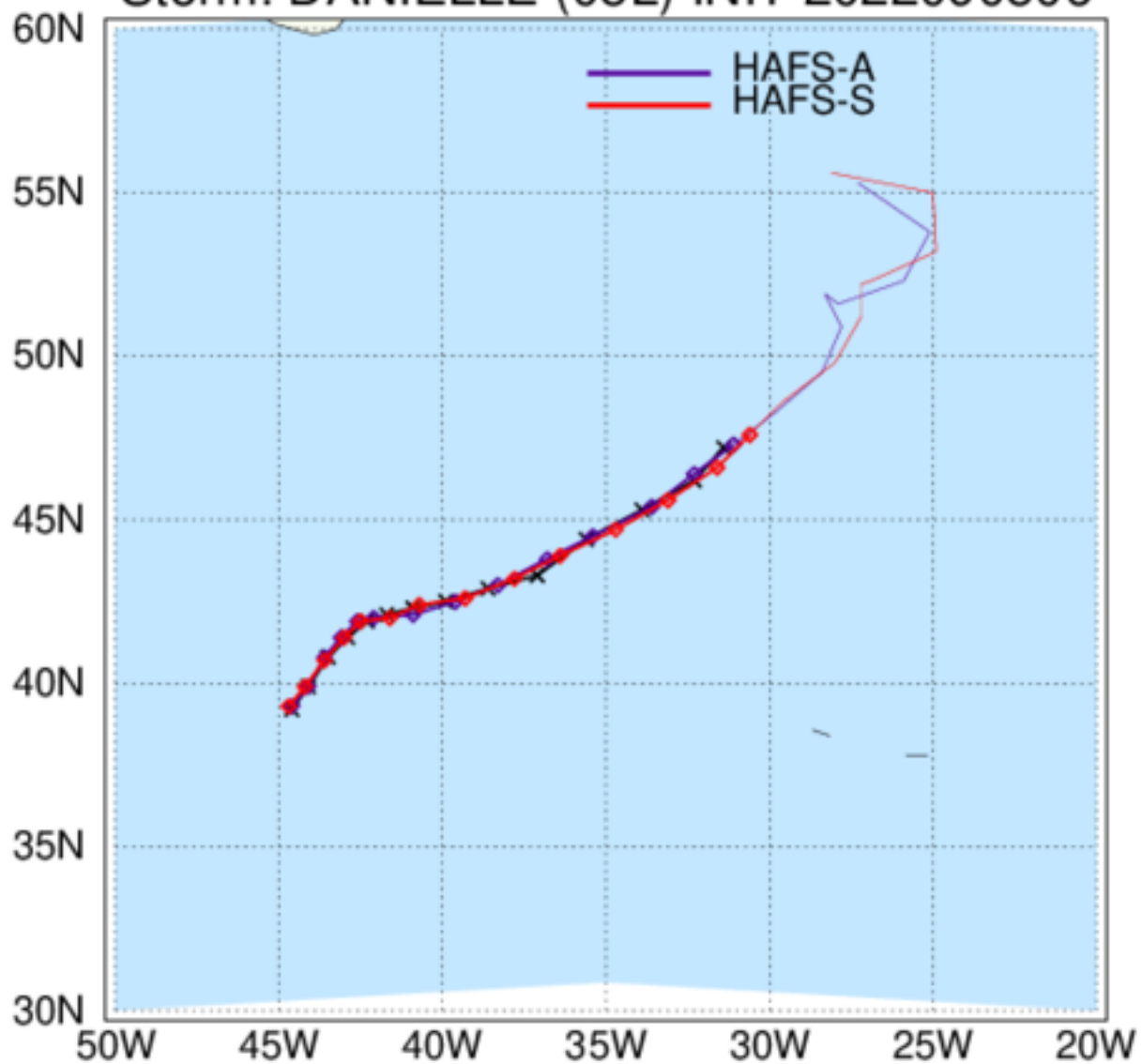
HAFS: TC Tracks Storm: DANIELLE (05L) INIT 2022090506
