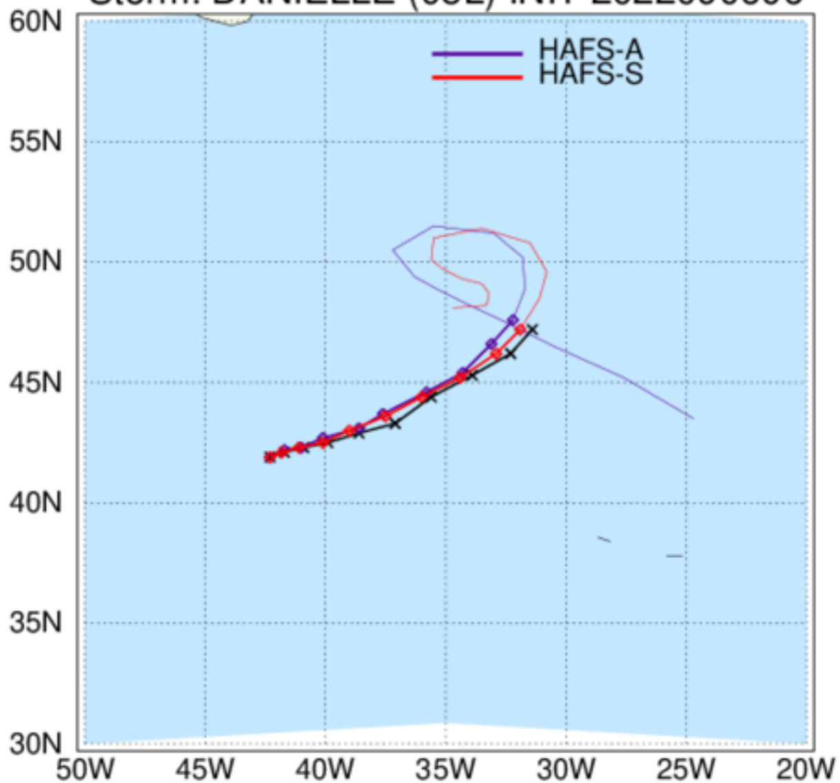
HAFS: TC Tracks Storm: DANIELLE (05L) INIT 2022090606
