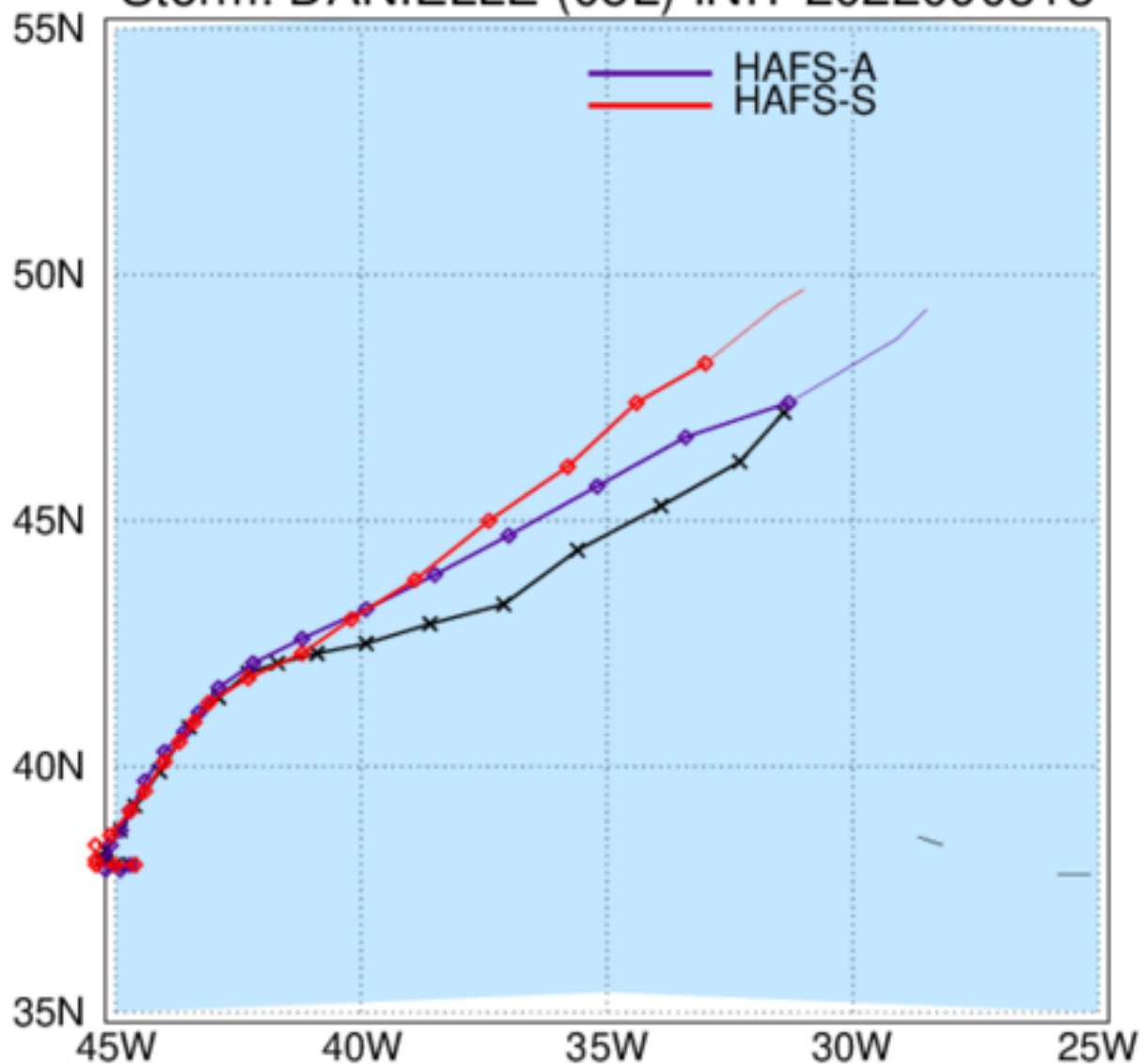
HAFS: TC Tracks Storm: DANIELLE (05L) INIT 2022090318
