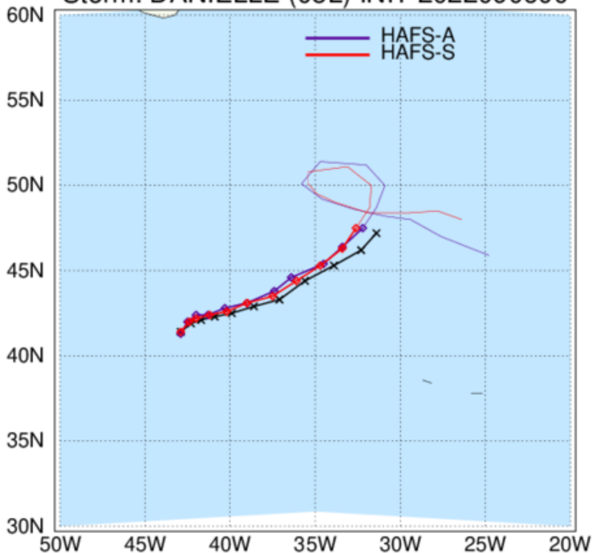
HAFS: TC Tracks Storm: DANIELLE (05L) INIT 2022090600
