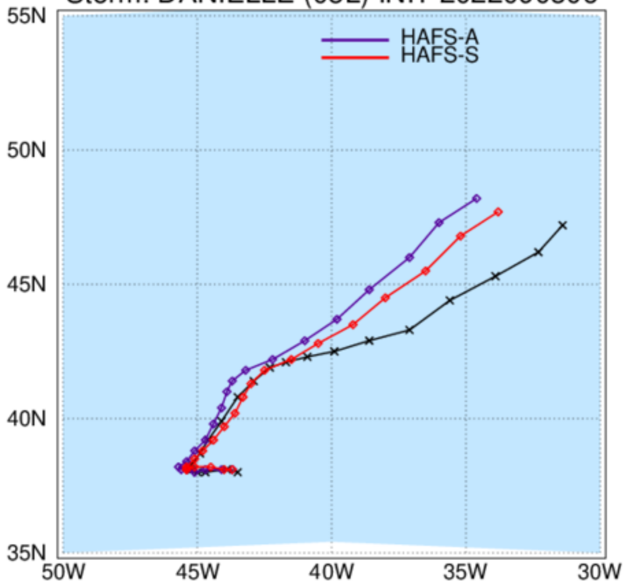
HAFS: TC Tracks Storm: DANIELLE (05L) INIT 2022090306
