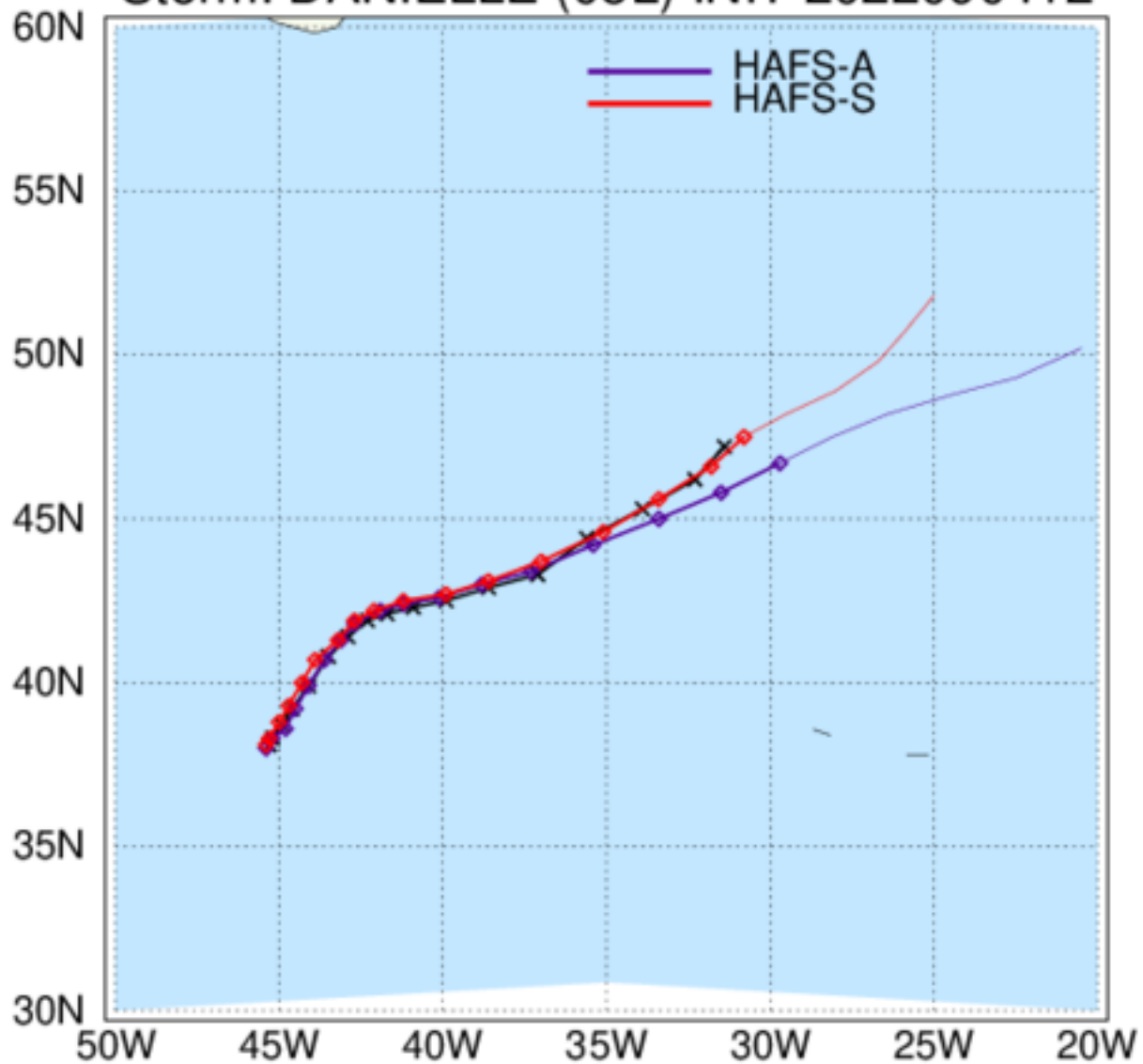
HAFS: TC Tracks Storm: DANIELLE (05L) INIT 2022090412
