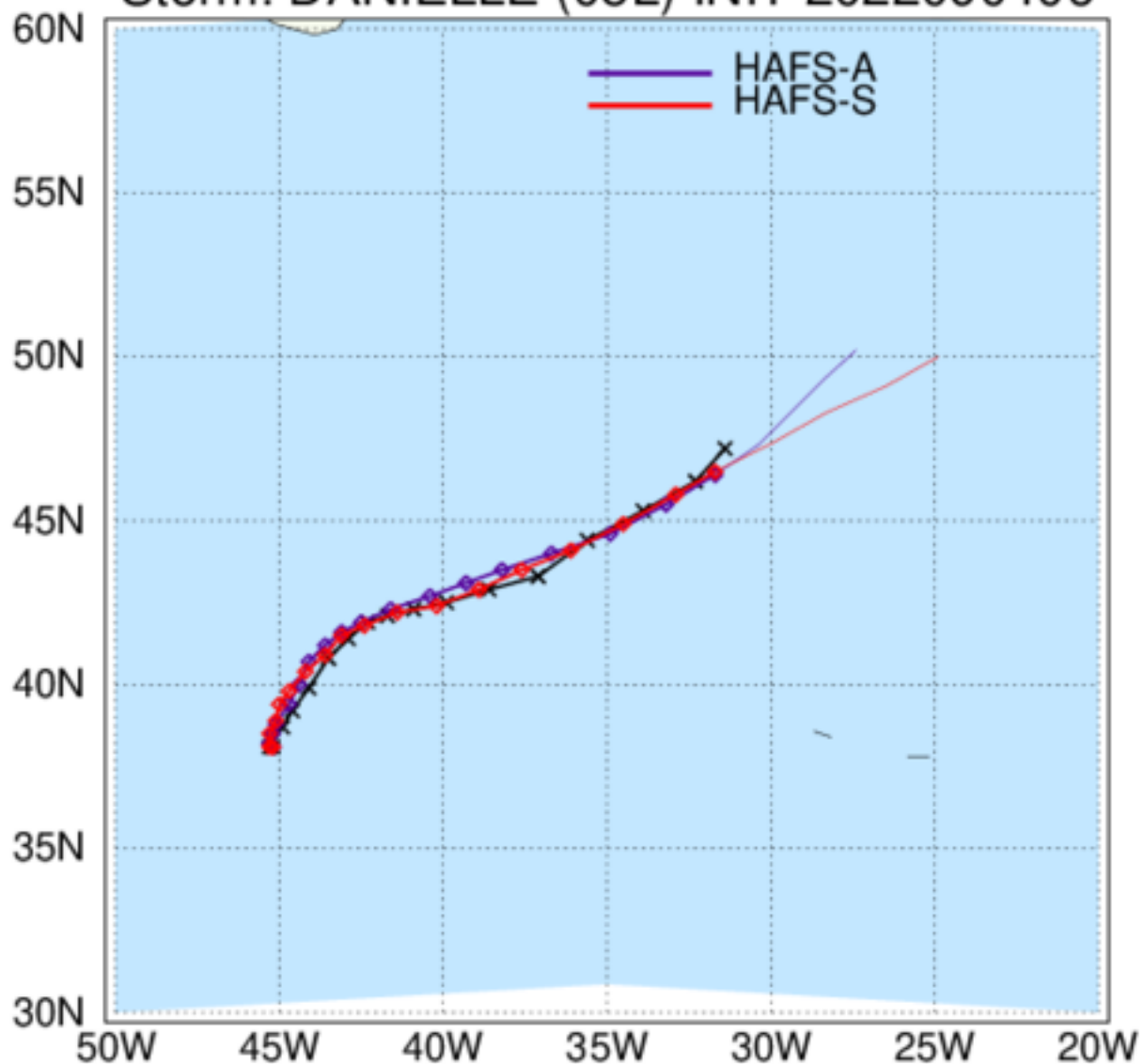
HAFS: TC Tracks Storm: DANIELLE (05L) INIT 2022090406
