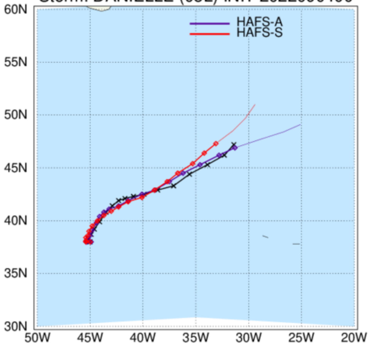
HAFS: TC Tracks Storm: DANIELLE (05L) INIT 2022090400
