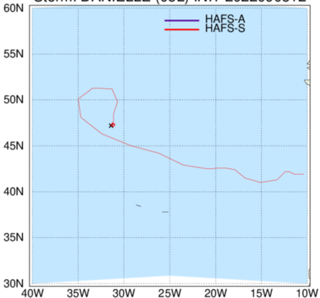
HAFS: TC Tracks Storm: DANIELLE (05L) INIT 2022090812
