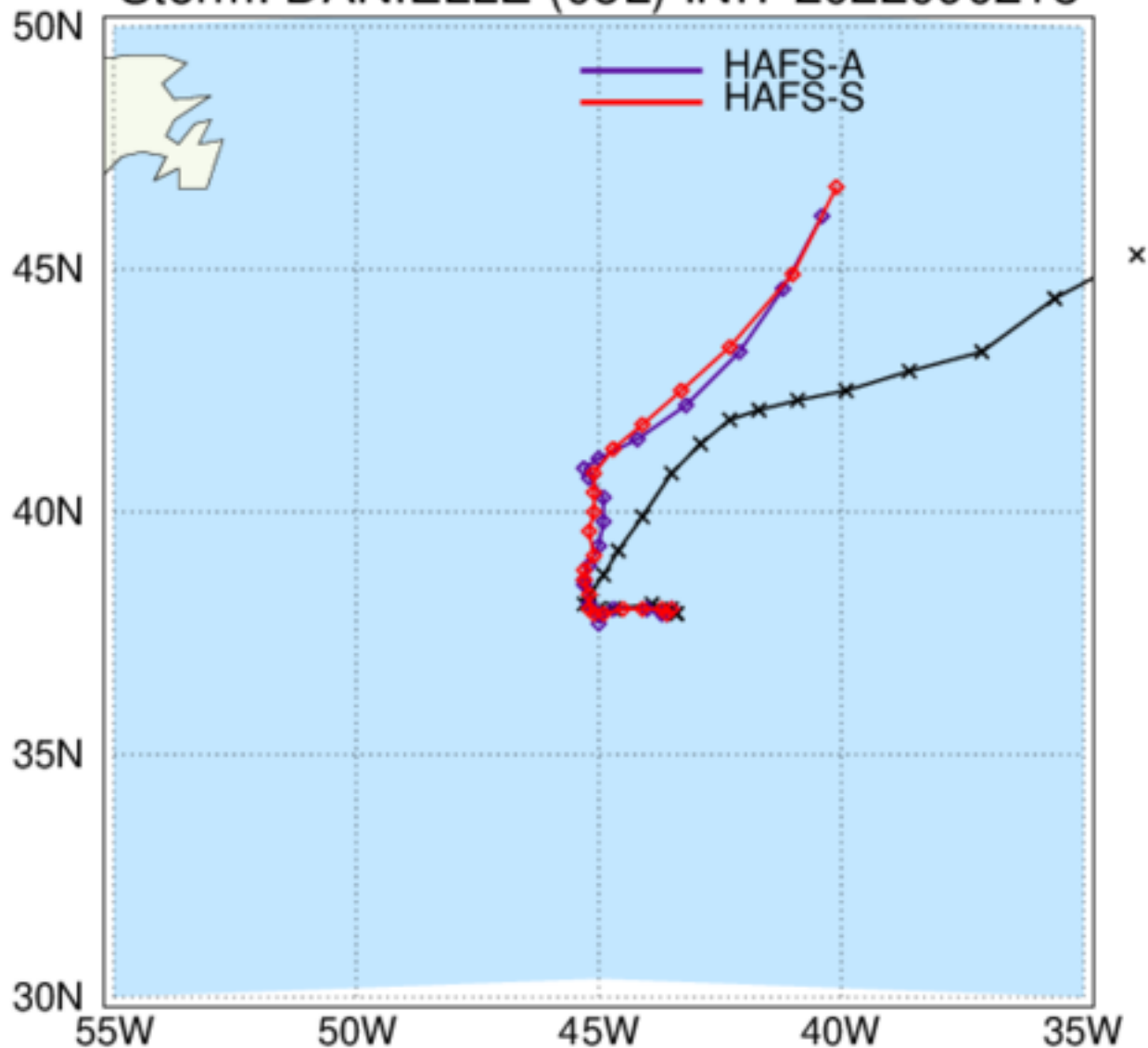
HAFS: TC Tracks Storm: DANIELLE (05L) INIT 2022090218
