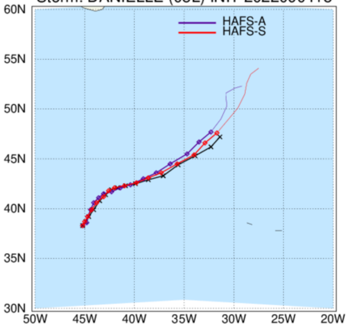
HAFS: TC Tracks Storm: DANIELLE (05L) INIT 2022090418
