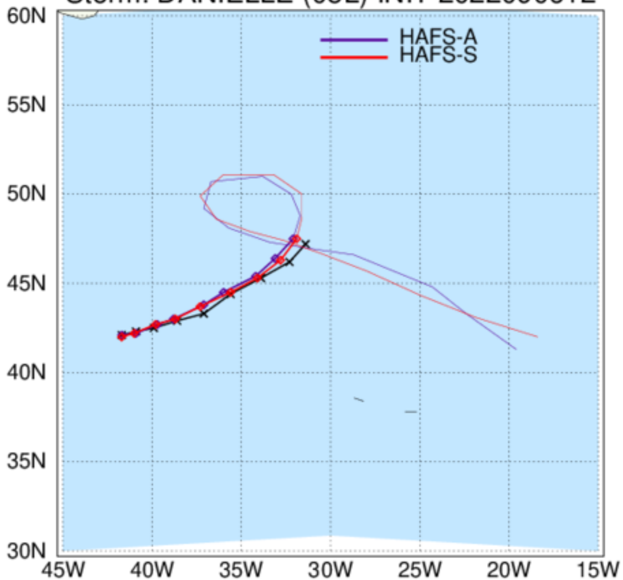
HAFS: TC Tracks Storm: DANIELLE (05L) INIT 2022090612
