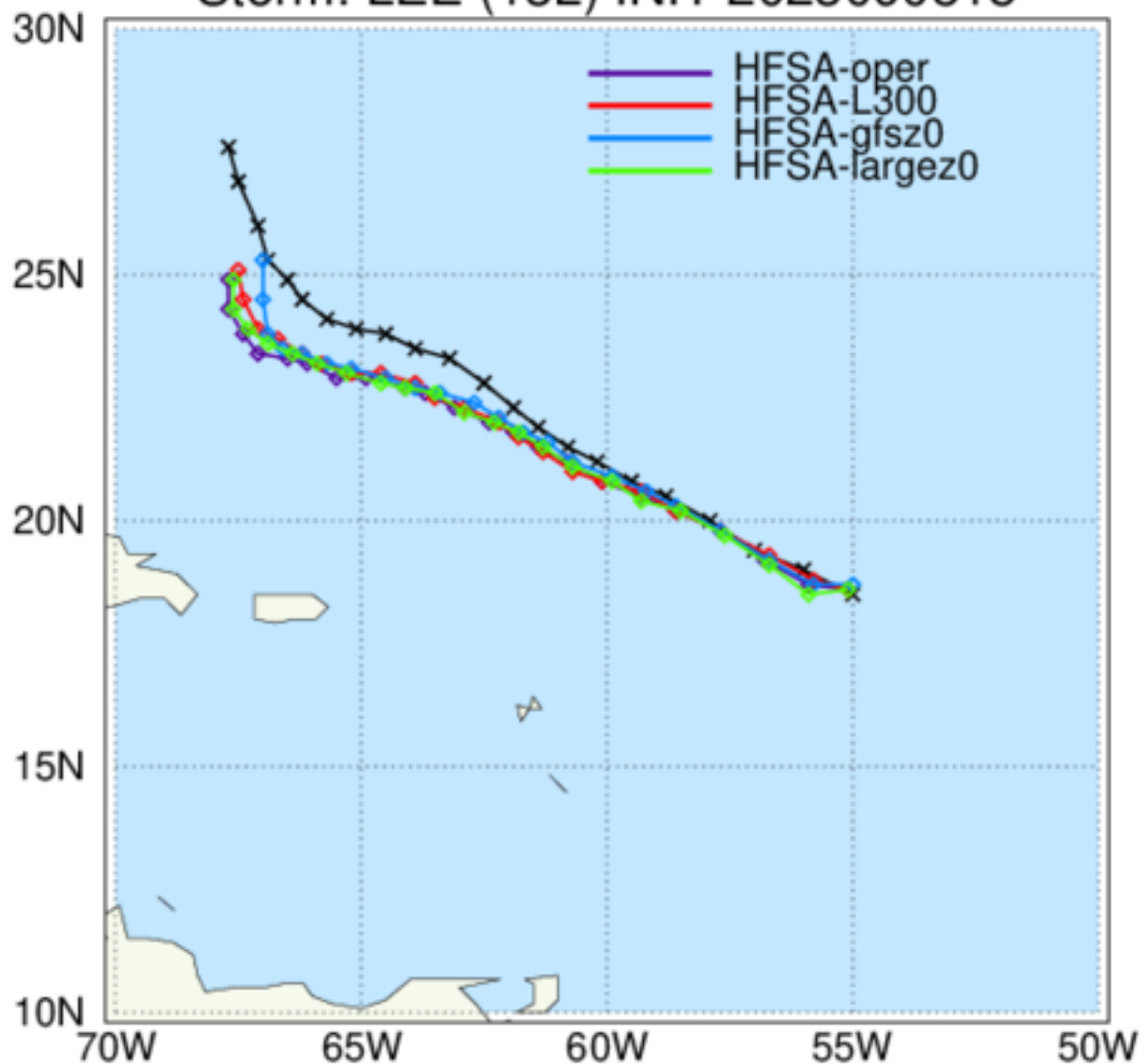
HAFS: TC Tracks Storm: LEE (13L) INIT 2023090818
