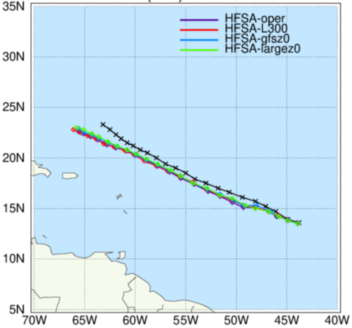
HAFS: TC Tracks Storm: LEE (13L) INIT 2023090606
