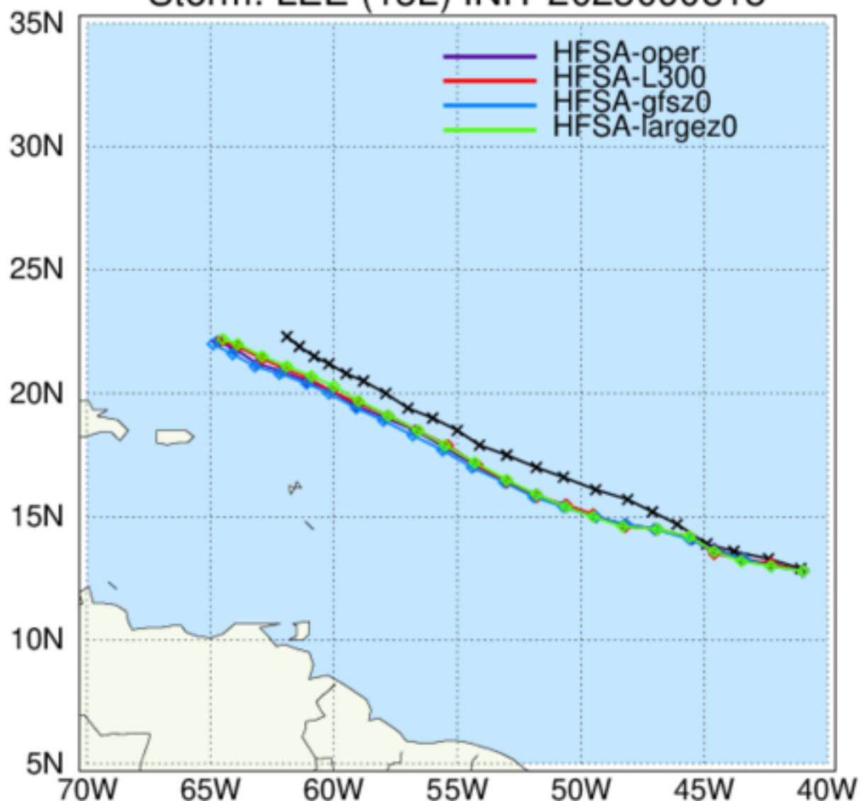
HAFS: TC Tracks Storm: LEE (13L) INIT 2023090518
