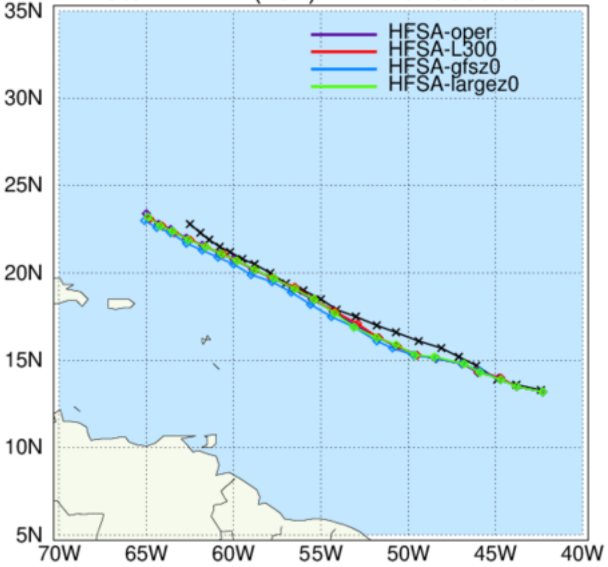
HAFS: TC Tracks Storm: LEE (13L) INIT 2023090600
