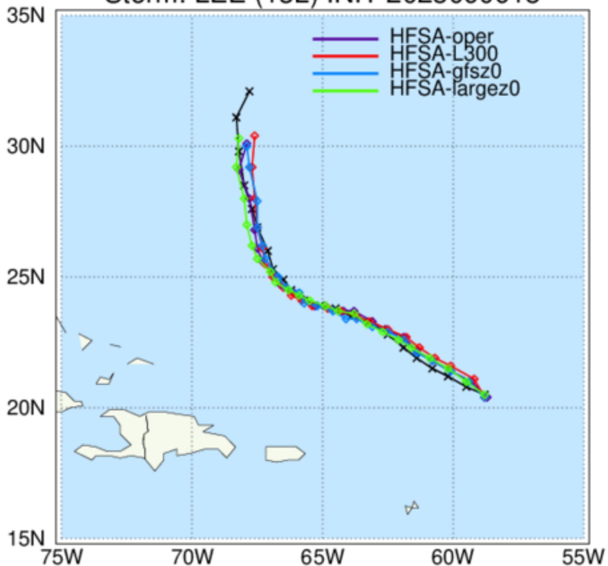
HAFS: TC Tracks Storm: LEE (13L) INIT 2023090918
