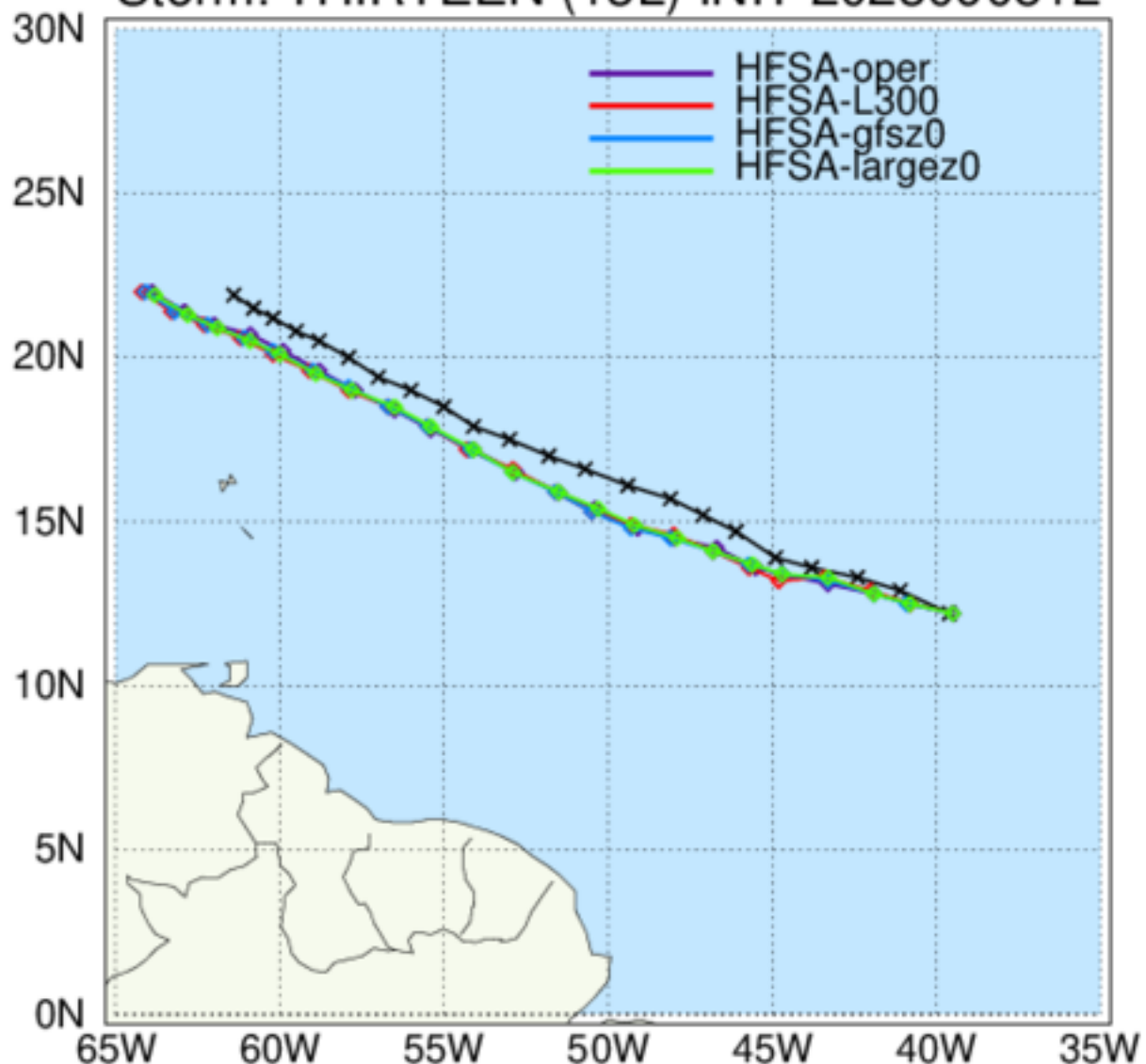
HAFS: TC Tracks Storm: THIRTEEN (13L) INIT 2023090512
