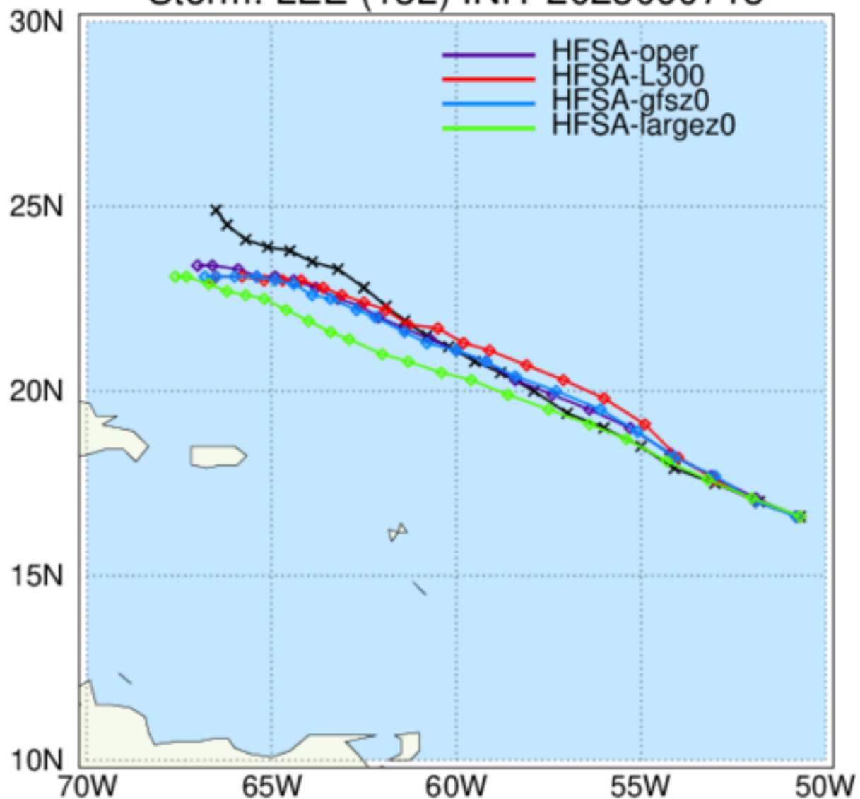
HAFS: TC Tracks Storm: LEE (13L) INIT 2023090718
