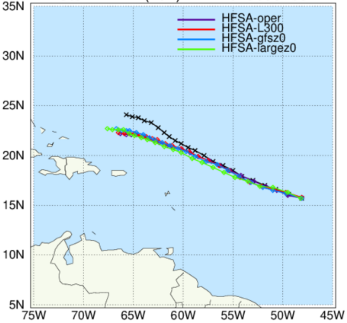
HAFS: TC Tracks Storm: LEE (13L) INIT 2023090706
