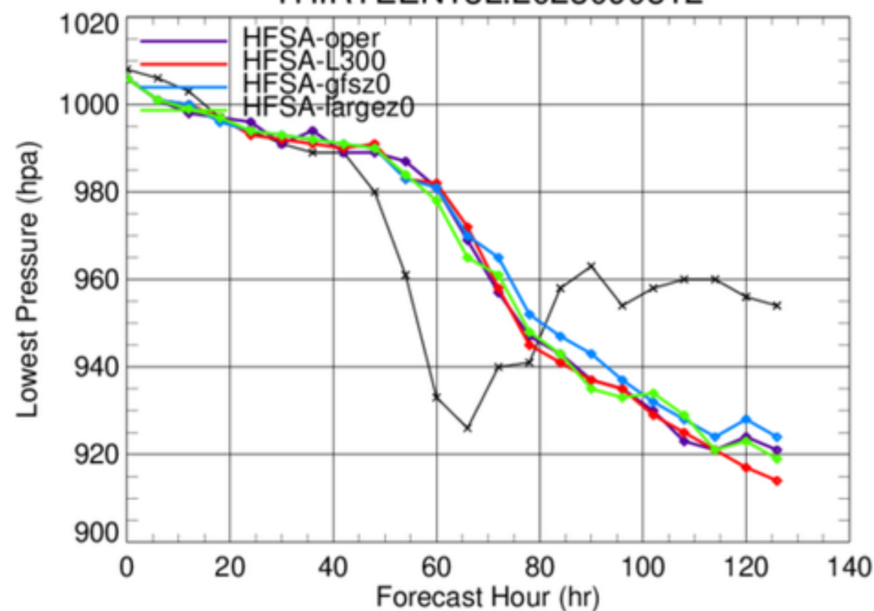
THIRTEEN13L.2023090512
