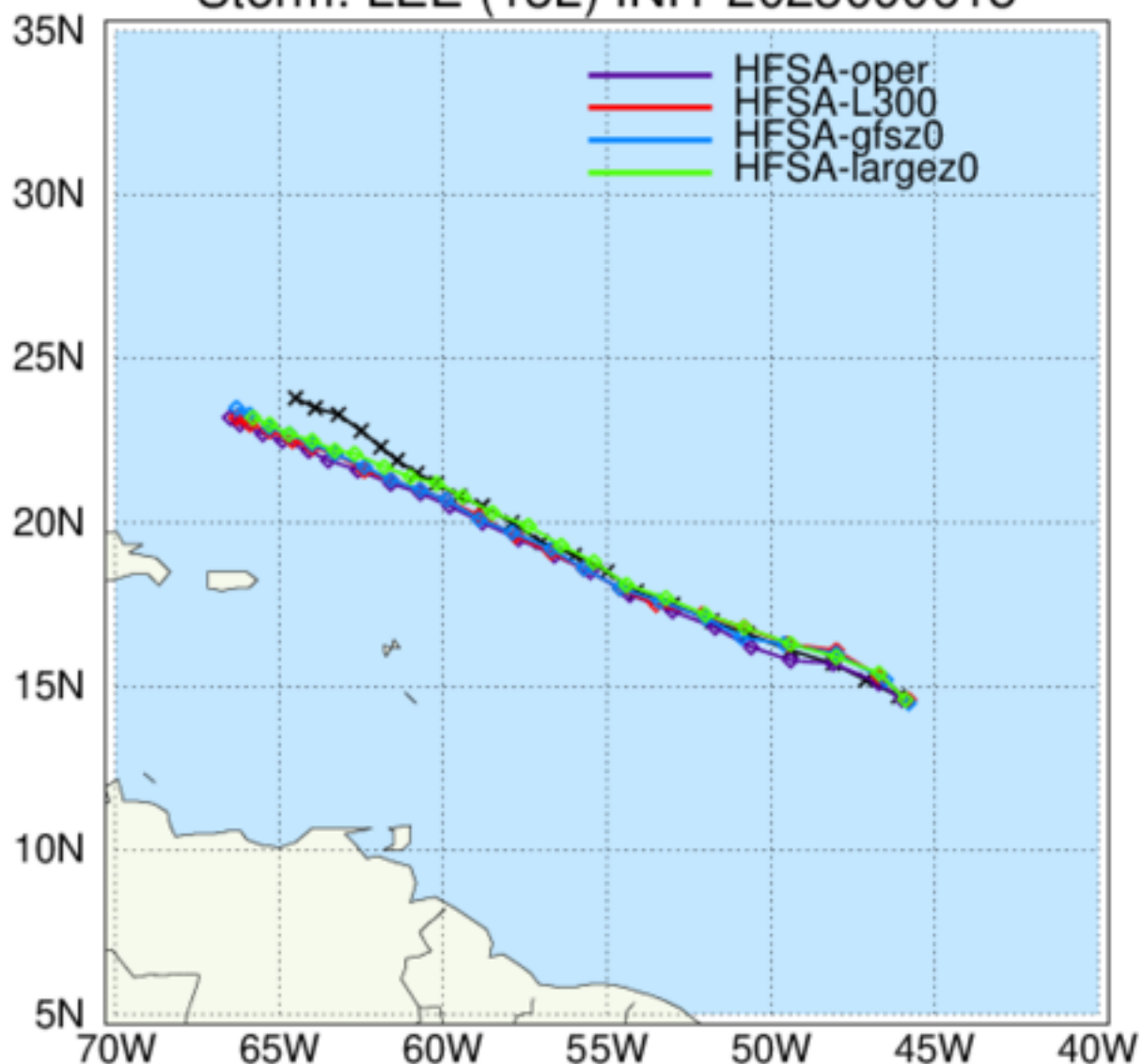
HAFS: TC Tracks Storm: LEE (13L) INIT 2023090618
