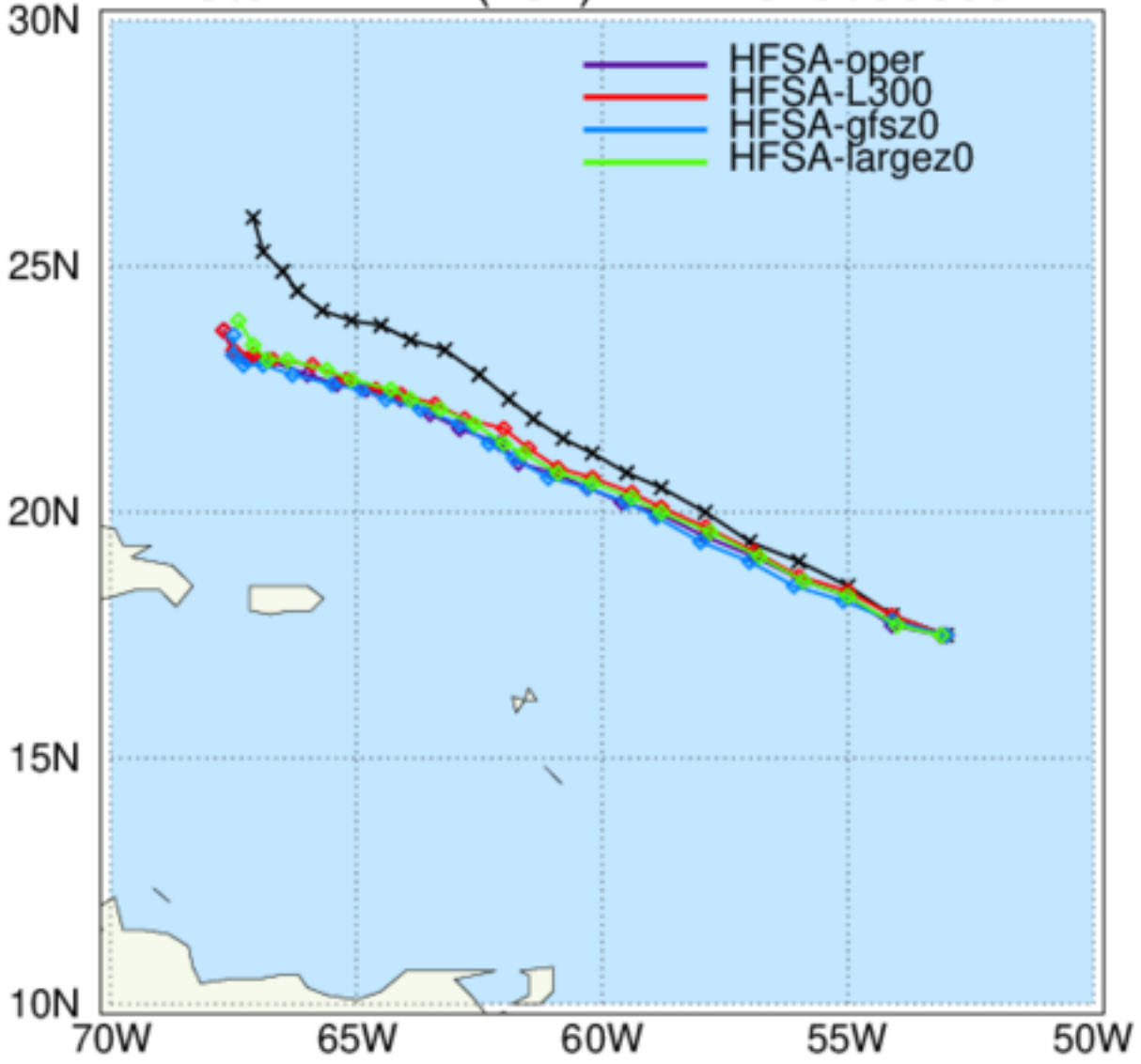
HAFS: TC Tracks Storm: LEE (13L) INIT 2023090806
