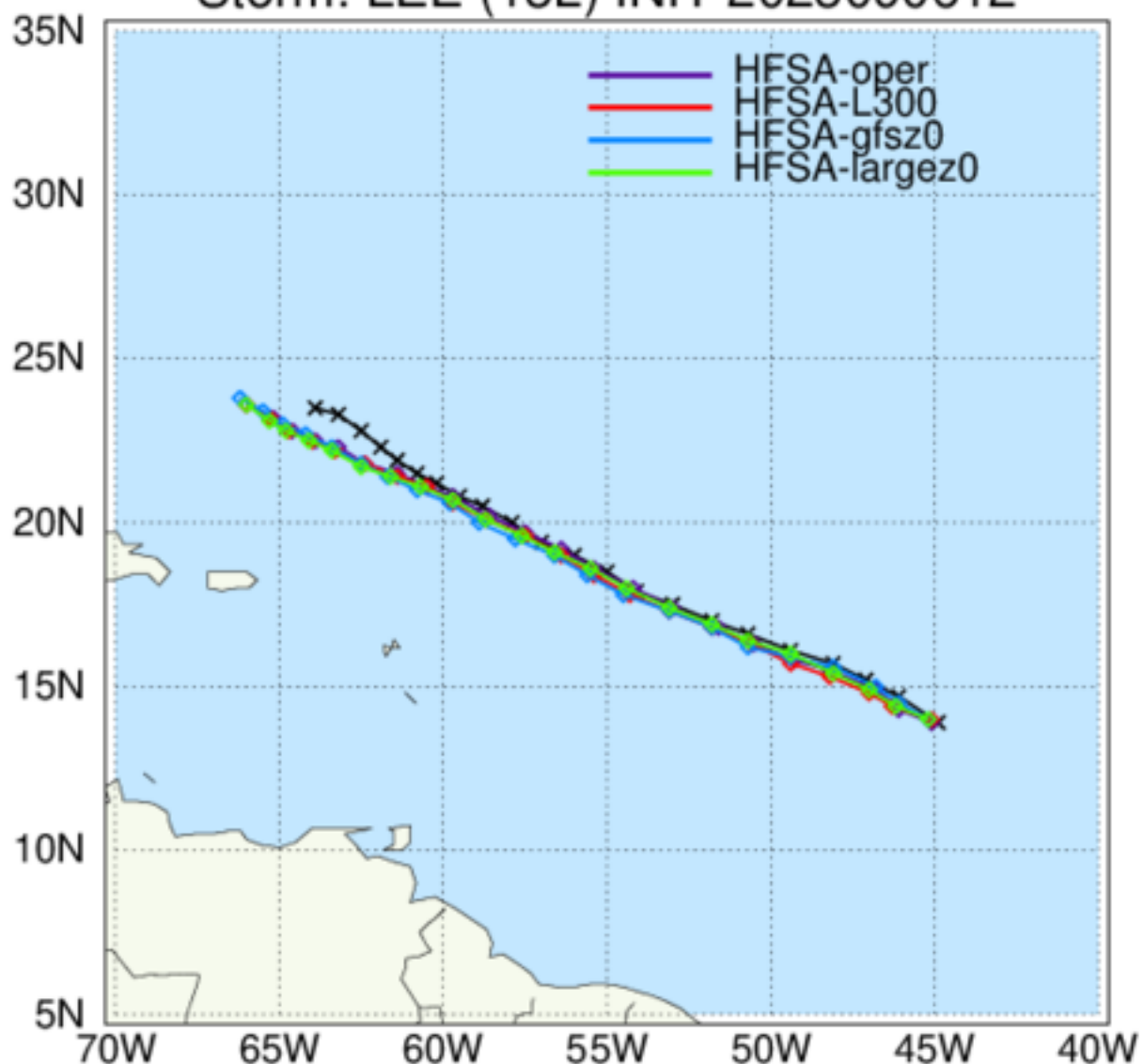
HAFS: TC Tracks Storm: LEE (13L) INIT 2023090612
