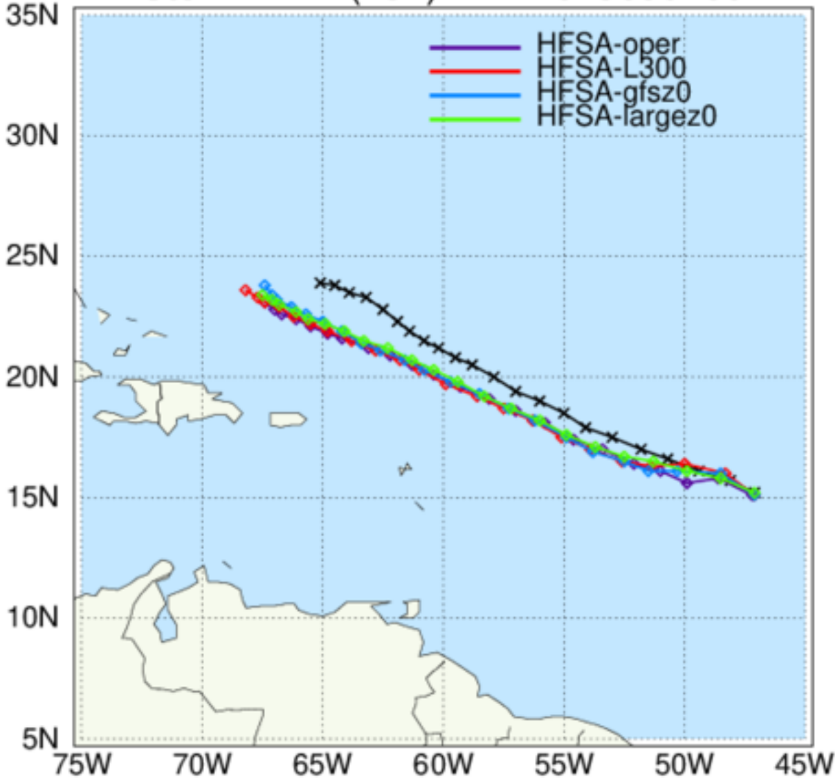
HAFS: TC Tracks Storm: LEE (13L) INIT 2023090700
