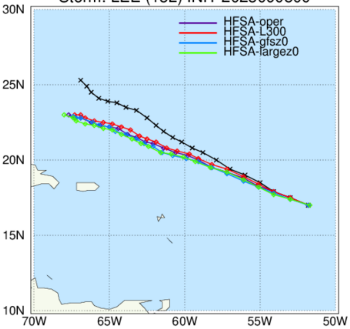
HAFS: TC Tracks Storm: LEE (13L) INIT 2023090800
