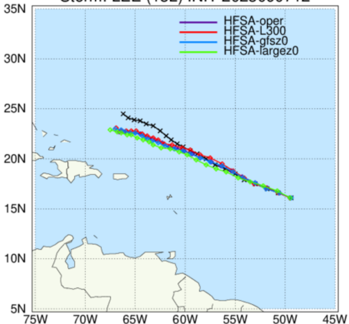
HAFS: TC Tracks Storm: LEE (13L) INIT 2023090712
