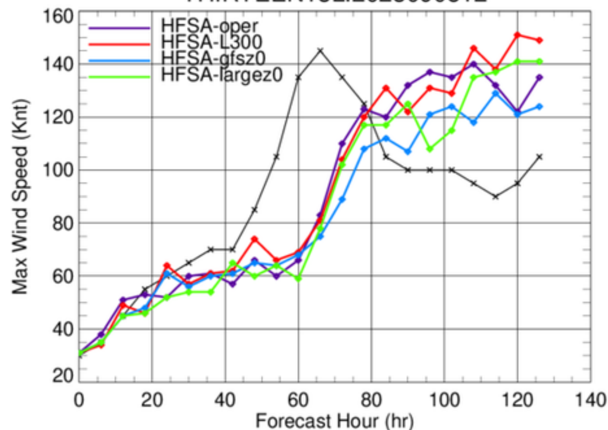
THIRTEEN13L.2023090512
