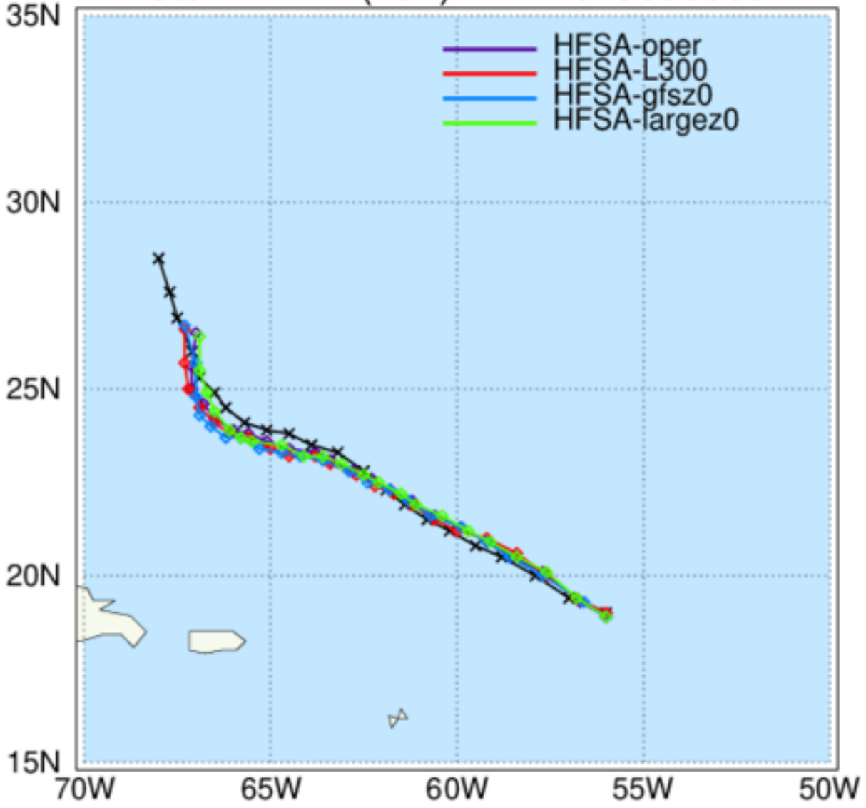
HAFS: TC Tracks Storm: LEE (13L) INIT 2023090900
