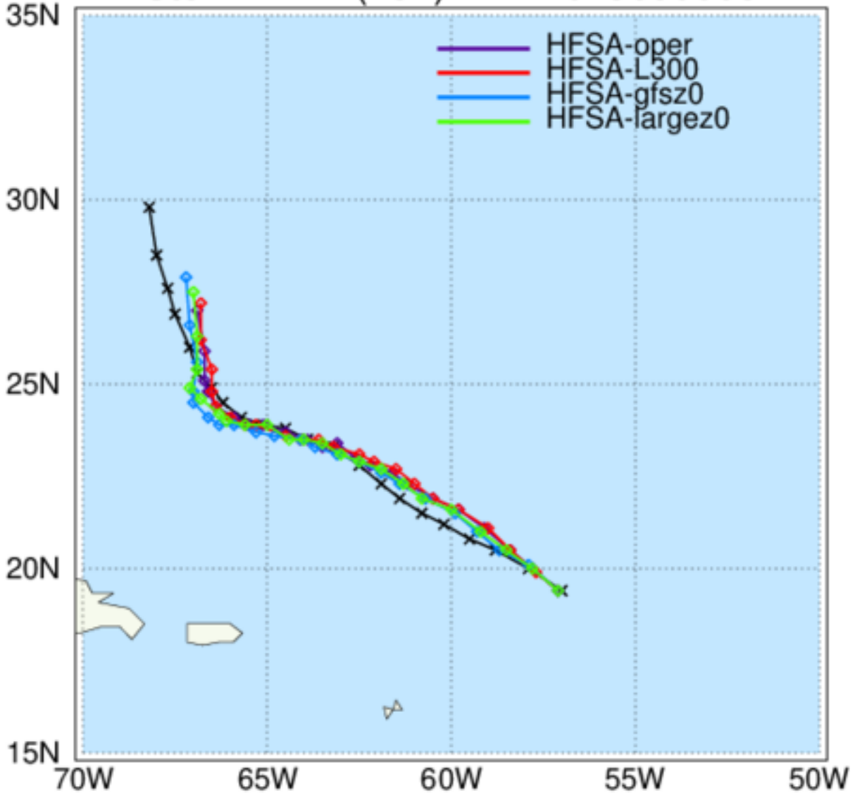
HAFS: TC Tracks Storm: LEE (13L) INIT 2023090906
