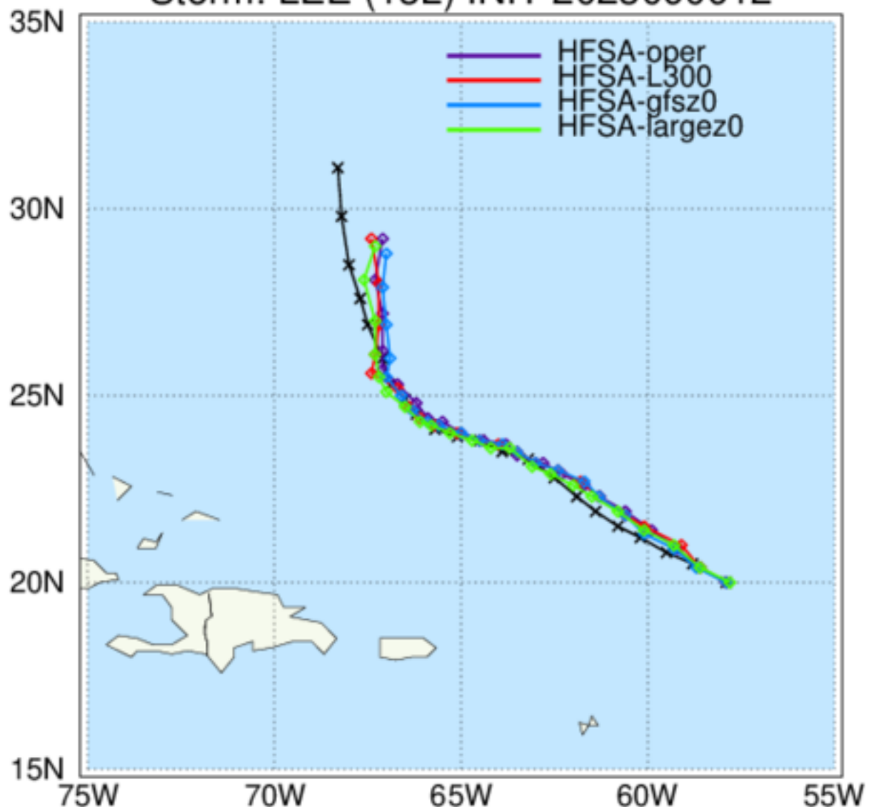
HAFS: TC Tracks Storm: LEE (13L) INIT 2023090912
