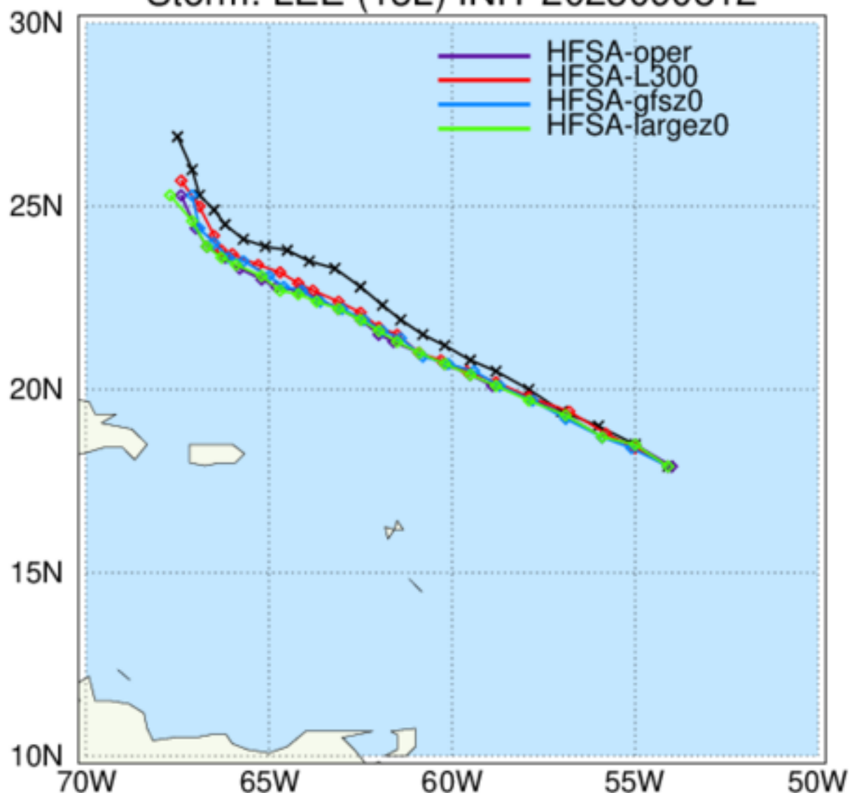
HAFS: TC Tracks Storm: LEE (13L) INIT 2023090812
