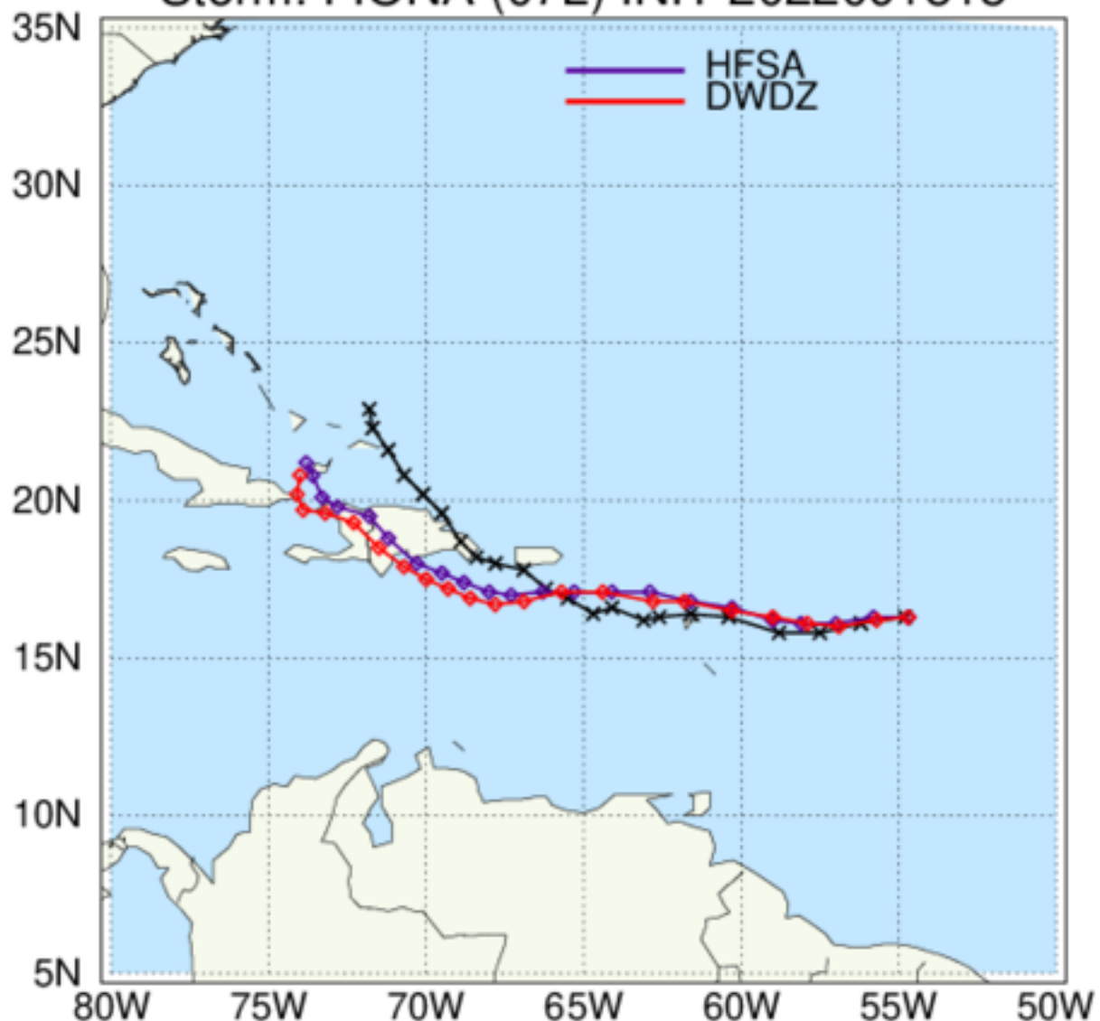
HAFS: TC Tracks Storm: FIONA (07L) INIT 2022091518
