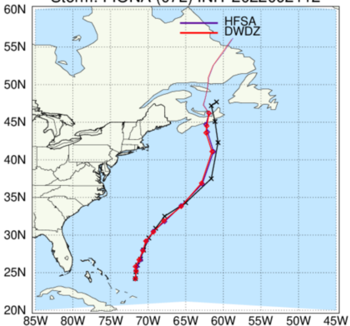
HAFS: TC Tracks Storm: FIONA (07L) INIT 2022092112
