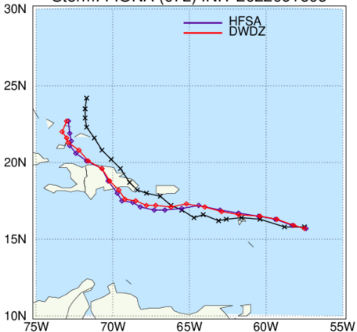
HAFS: TC Tracks Storm: FIONA (07L) INIT 2022091606
