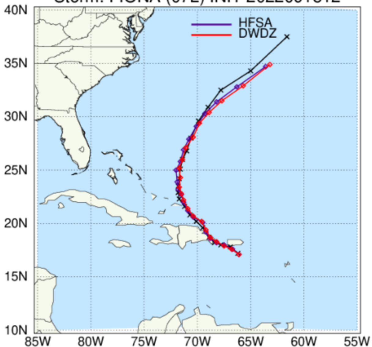
HAFS: TC Tracks Storm: FIONA (07L) INIT 2022091812
