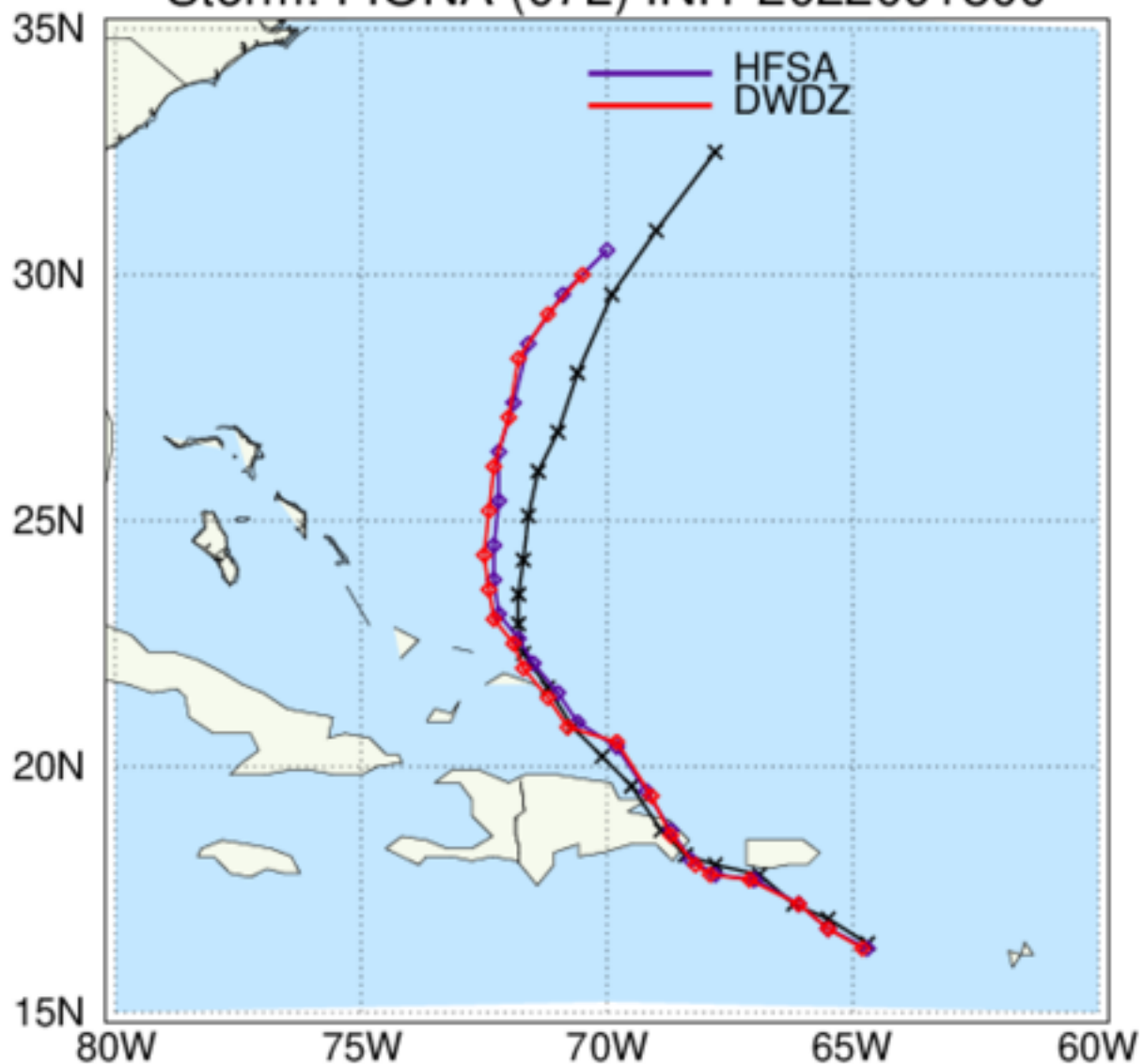
HAFS: TC Tracks Storm: FIONA (07L) INIT 2022091800
