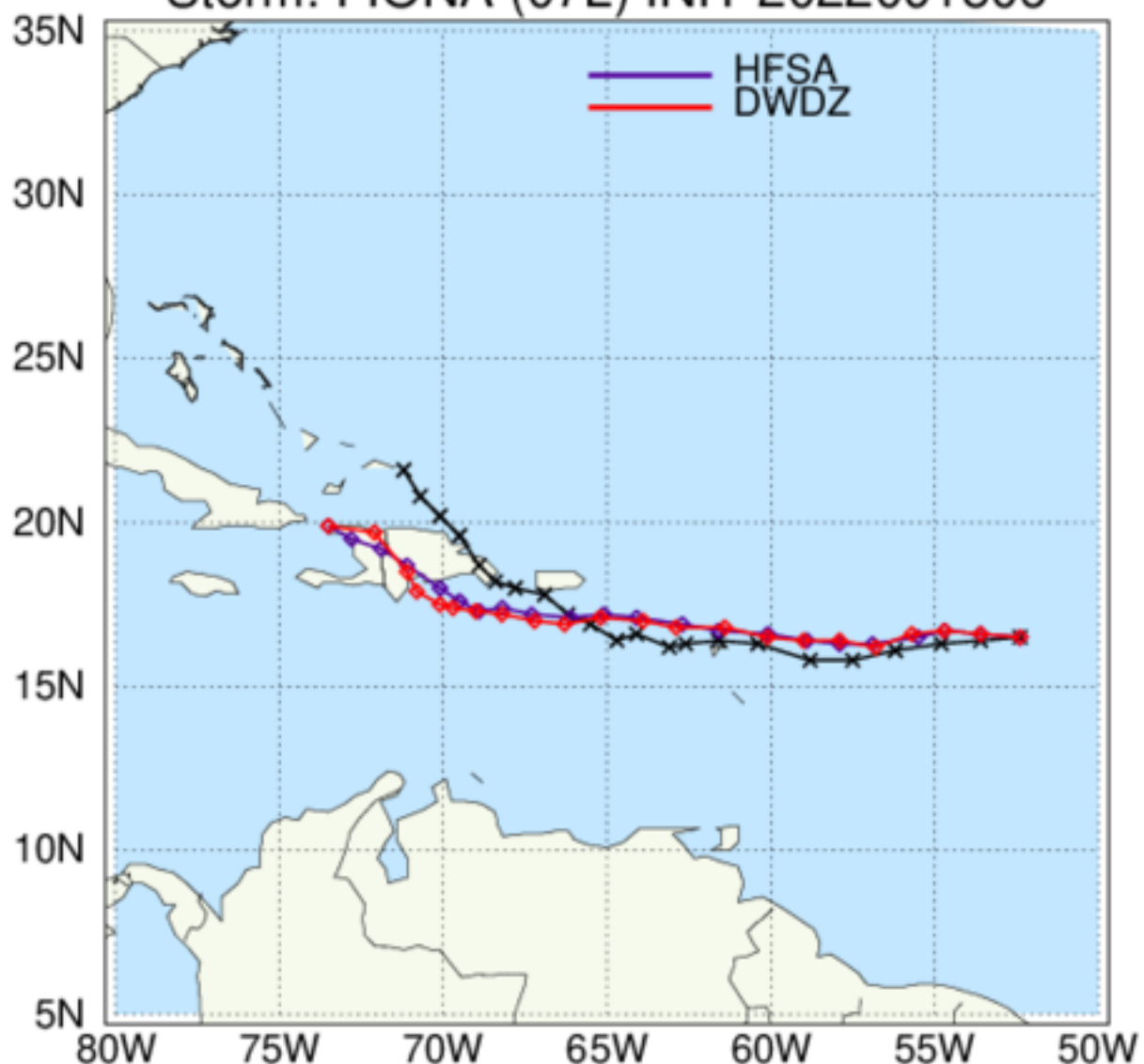
HAFS: TC Tracks Storm: FIONA (07L) INIT 2022091506
