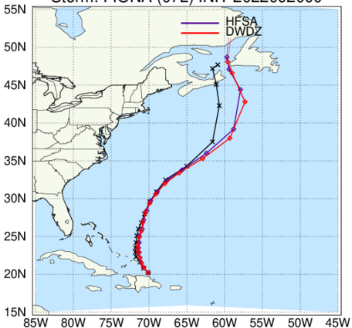
HAFS: TC Tracks Storm: FIONA (07L) INIT 2022092000
