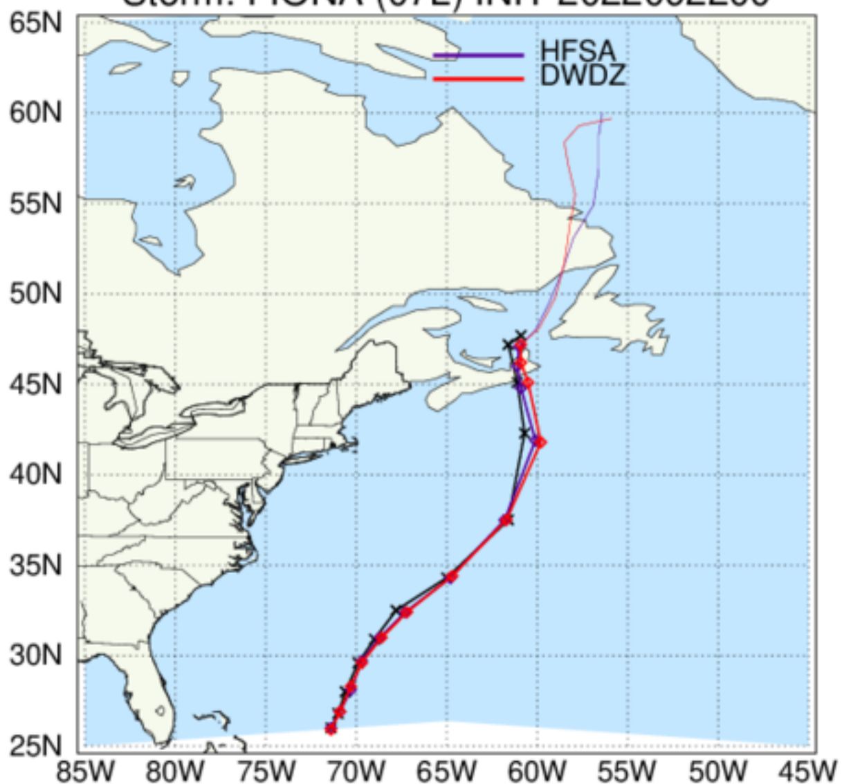
HAFS: TC Tracks Storm: FIONA (07L) INIT 2022092200
