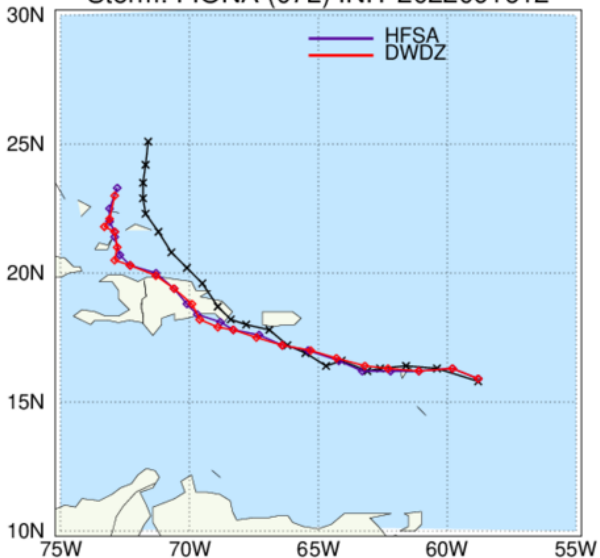
HAFS: TC Tracks Storm: FIONA (07L) INIT 2022091612
