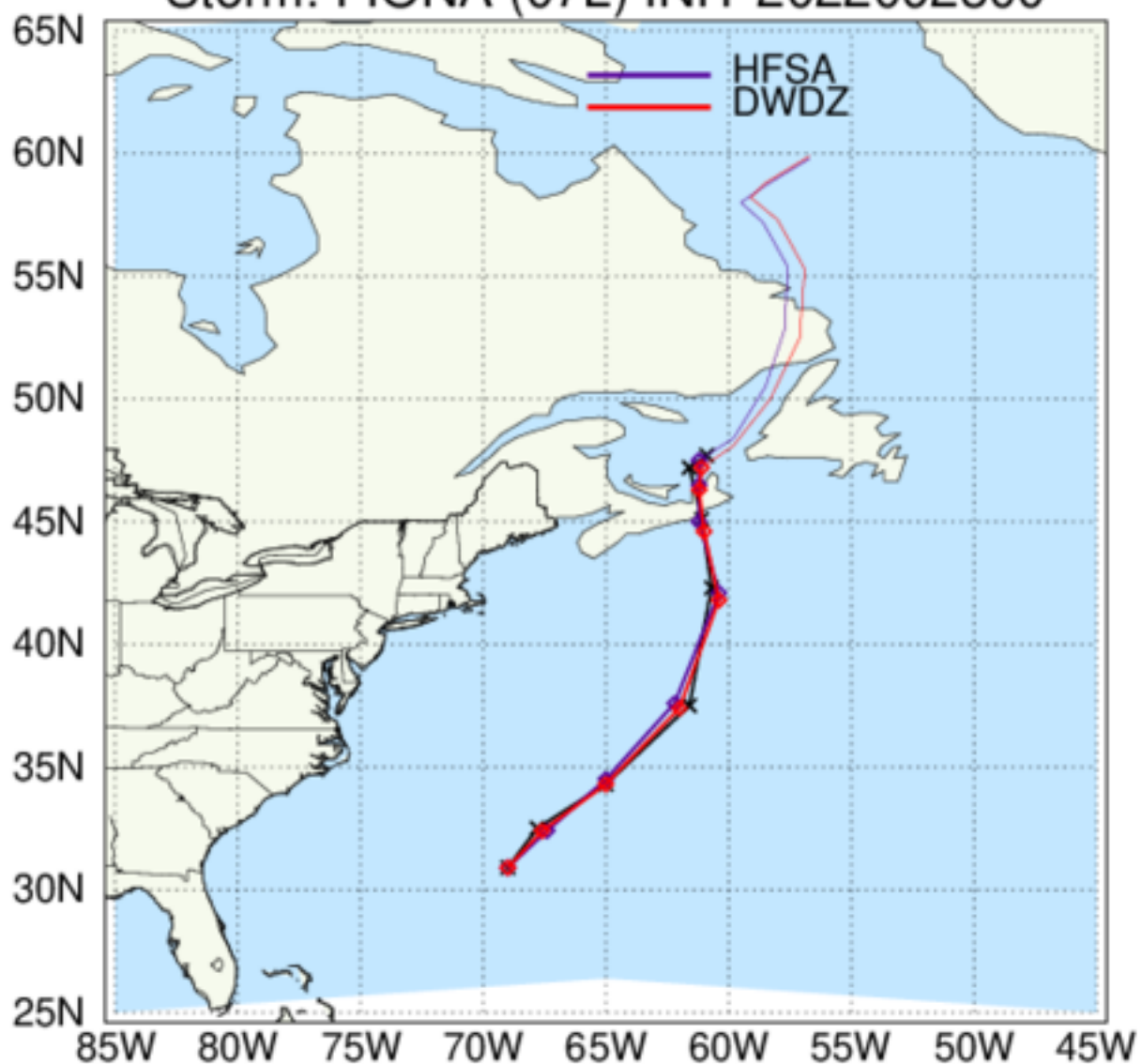
HAFS: TC Tracks Storm: FIONA (07L) INIT 2022092300
