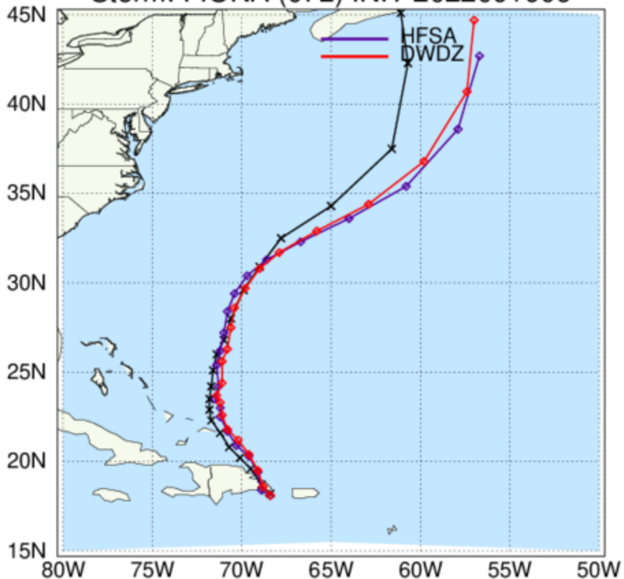
HAFS: TC Tracks Storm: FIONA (07L) INIT 2022091906
