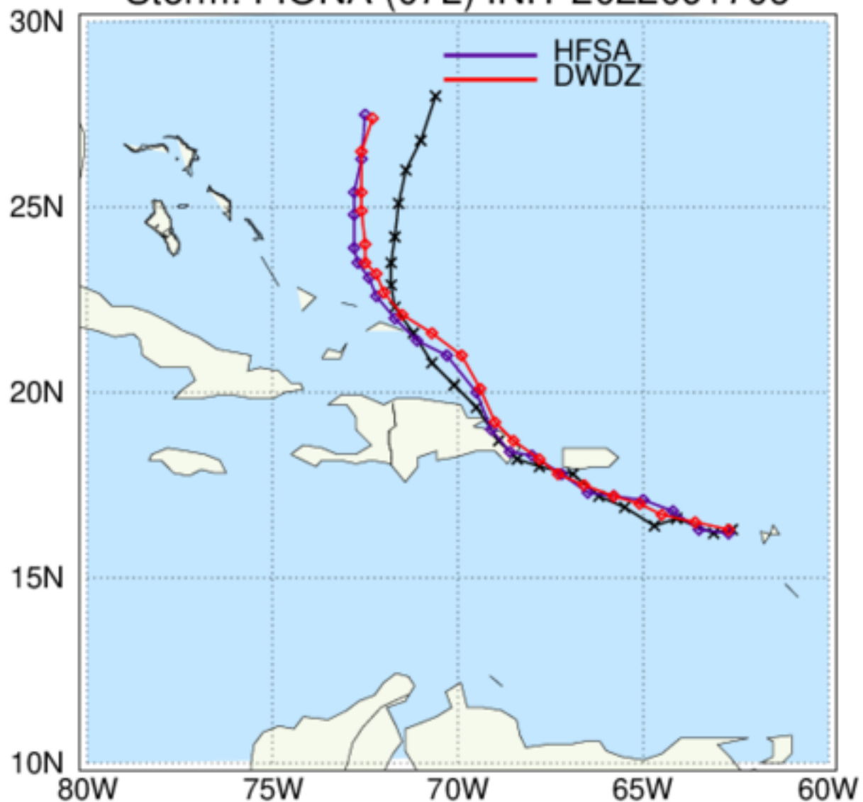
HAFS: TC Tracks Storm: FIONA (07L) INIT 2022091706
