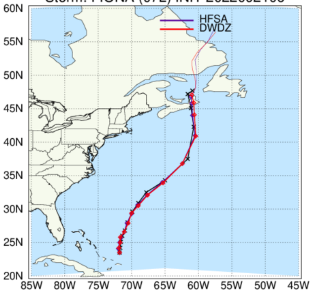
HAFS: TC Tracks Storm: FIONA (07L) INIT 2022092106
