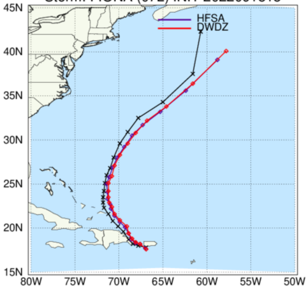
HAFS: TC Tracks Storm: FIONA (07L) INIT 2022091818
