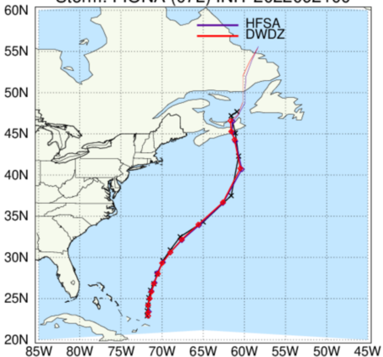
HAFS: TC Tracks Storm: FIONA (07L) INIT 2022092100
