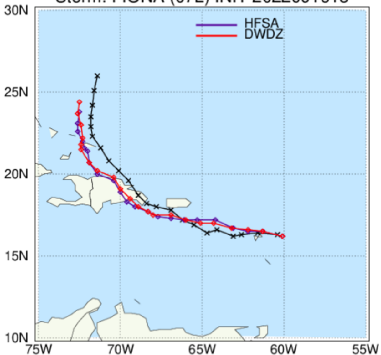
HAFS: TC Tracks Storm: FIONA (07L) INIT 2022091618
