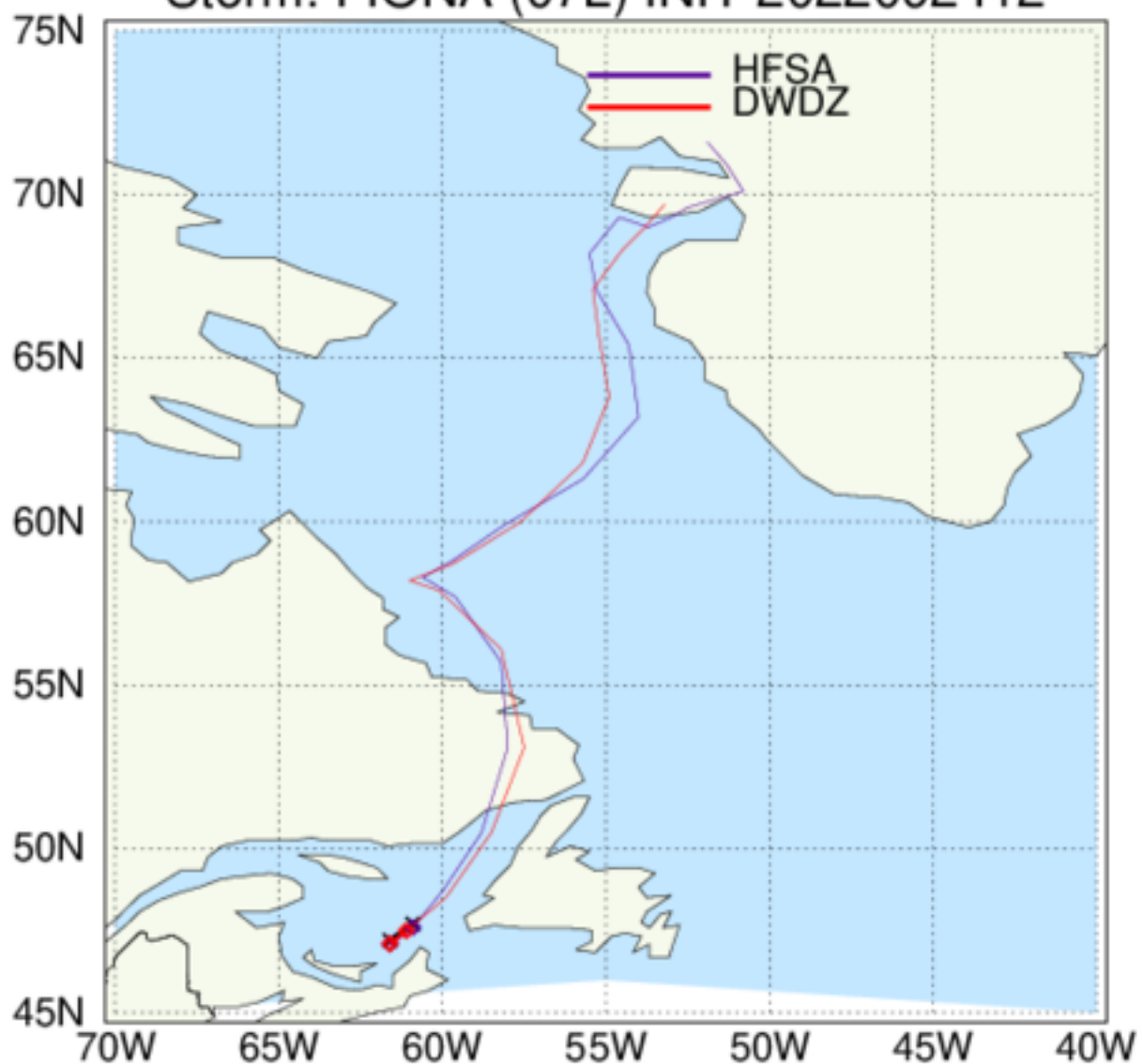
HAFS: TC Tracks Storm: FIONA (07L) INIT 2022092412
