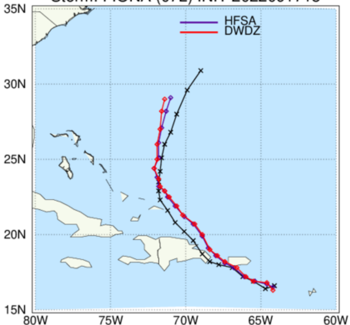
HAFS: TC Tracks Storm: FIONA (07L) INIT 2022091718
