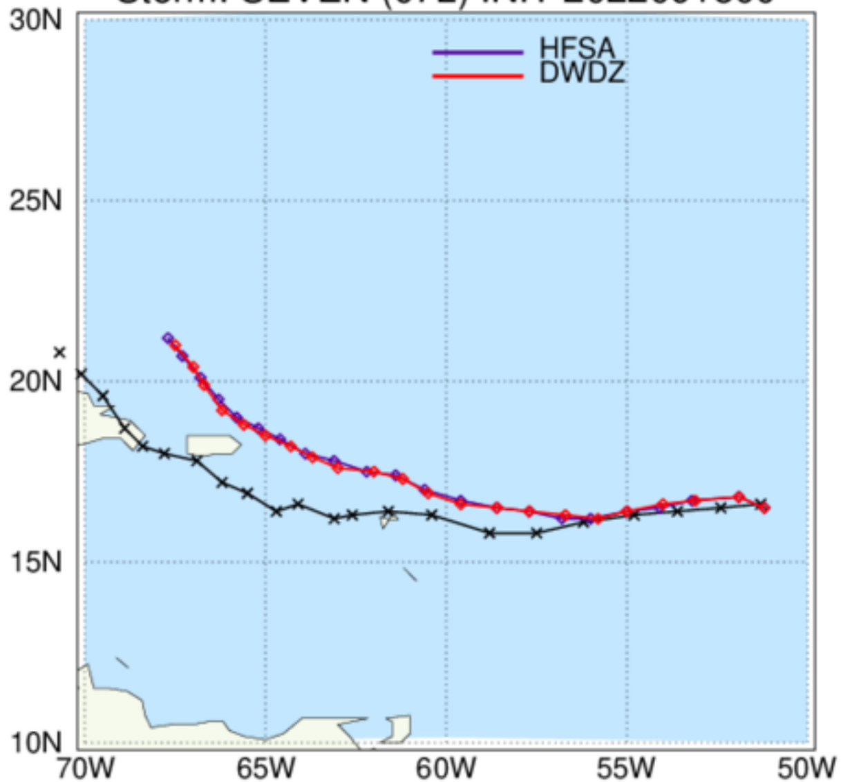
HAFS: TC Tracks Storm: SEVEN (07L) INIT 2022091500
