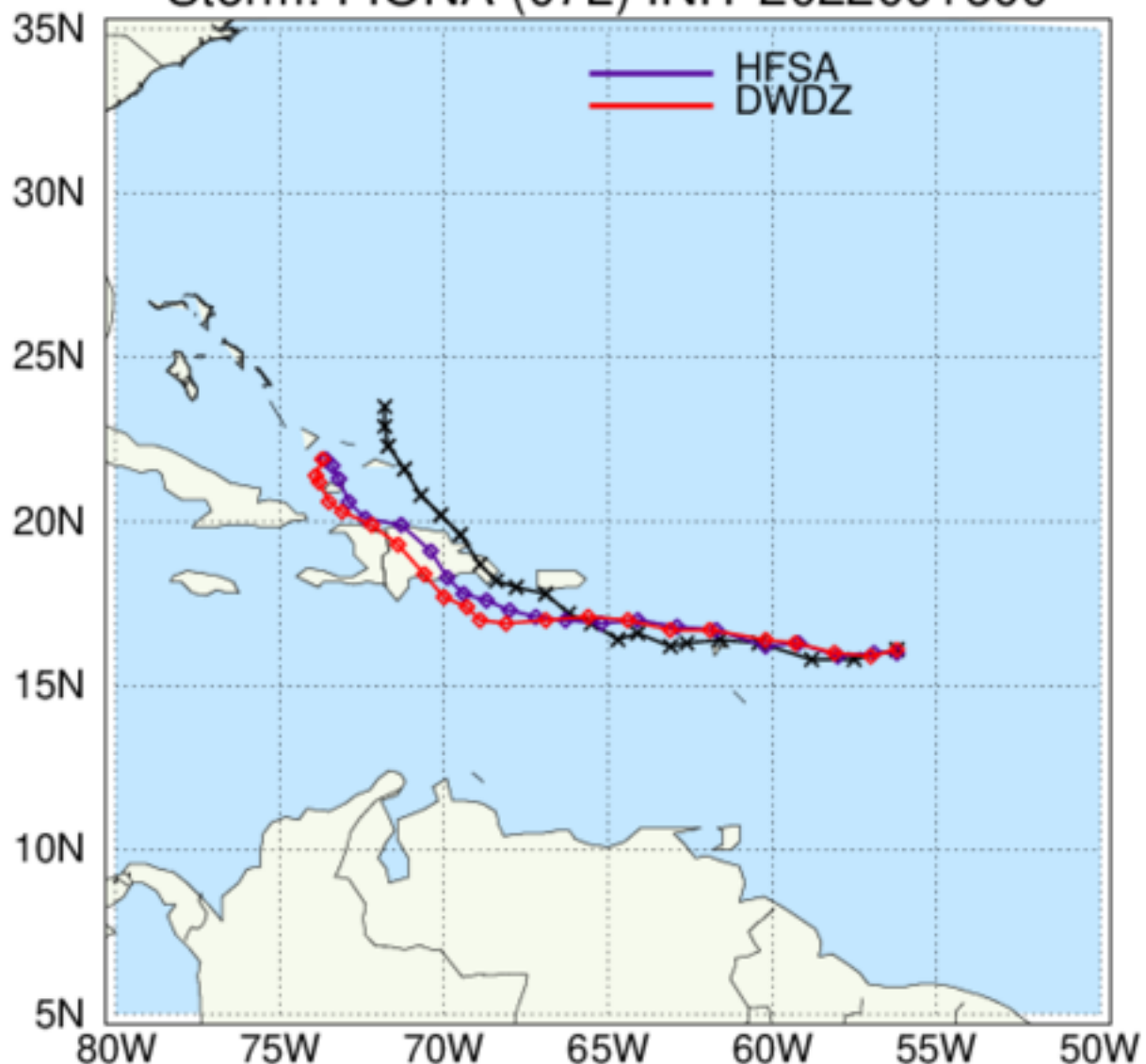
HAFS: TC Tracks Storm: FIONA (07L) INIT 2022091600
