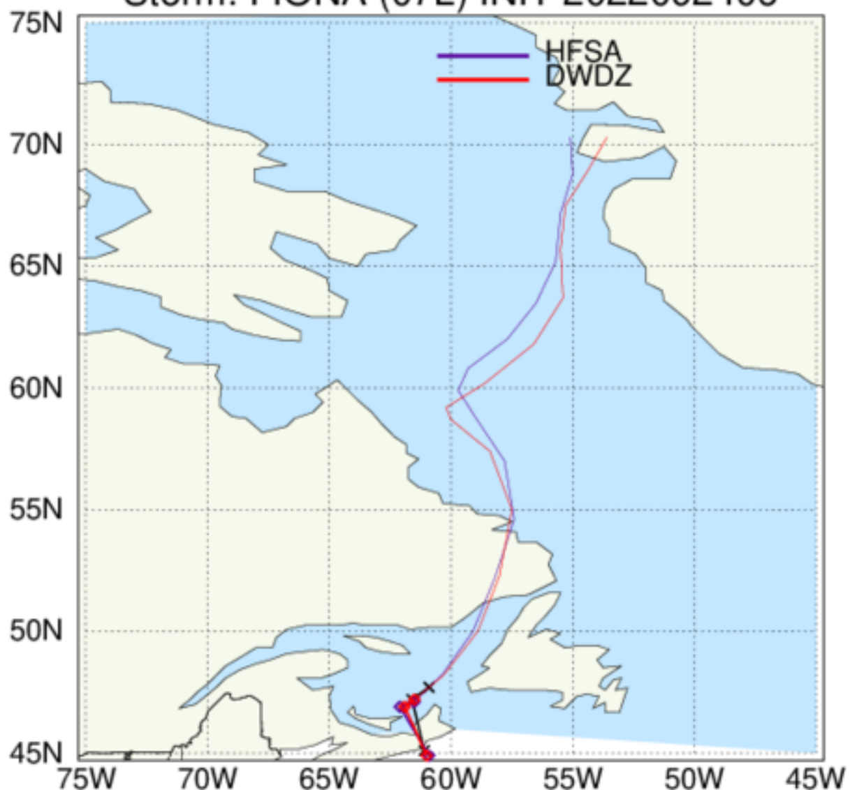
HAFS: TC Tracks Storm: FIONA (07L) INIT 2022092406
