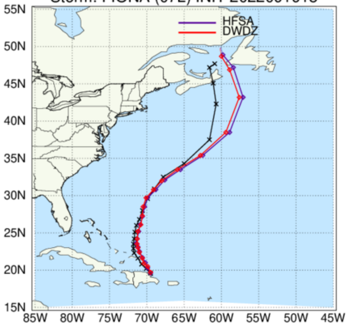
HAFS: TC Tracks Storm: FIONA (07L) INIT 2022091918
