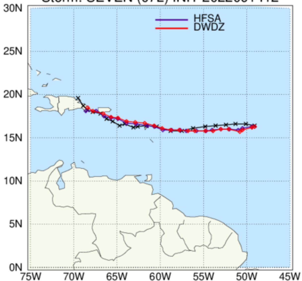
HAFS: TC Tracks Storm: SEVEN (07L) INIT 2022091412
