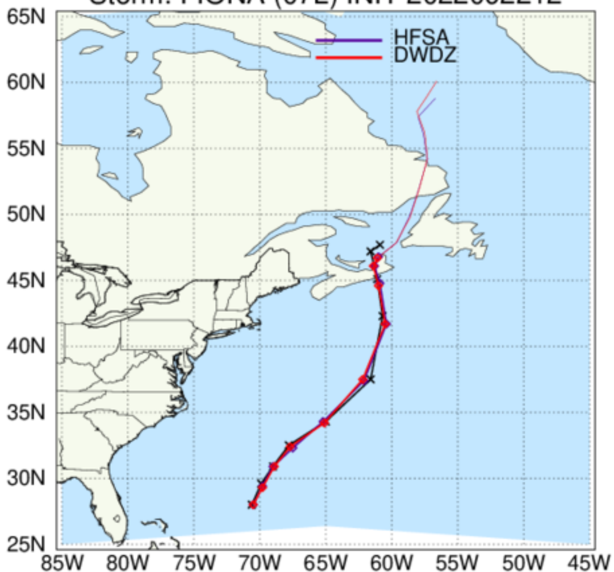
HAFS: TC Tracks Storm: FIONA (07L) INIT 2022092212
