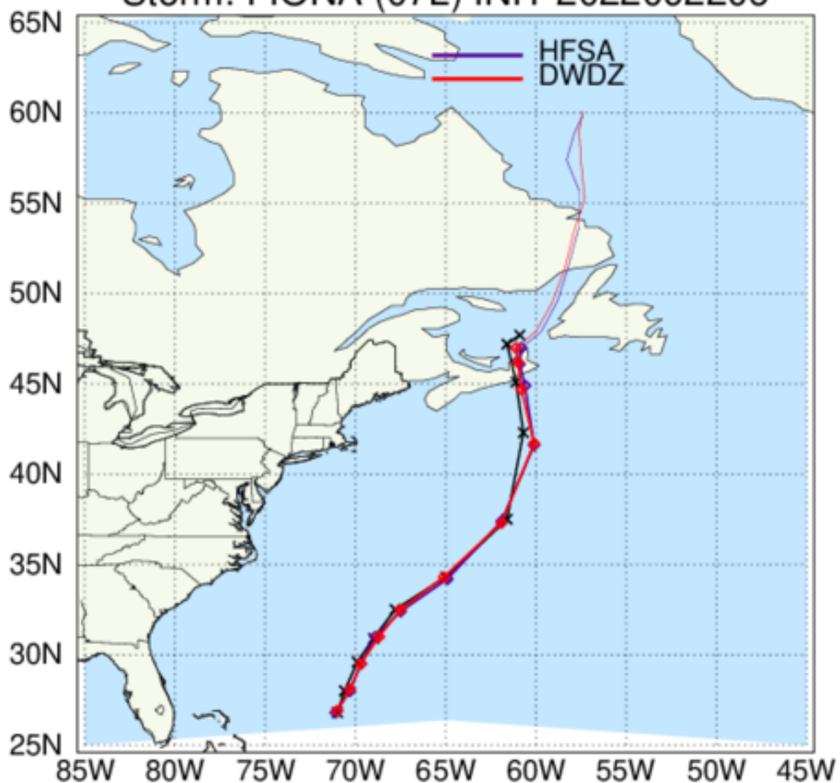
HAFS: TC Tracks Storm: FIONA (07L) INIT 2022092206
