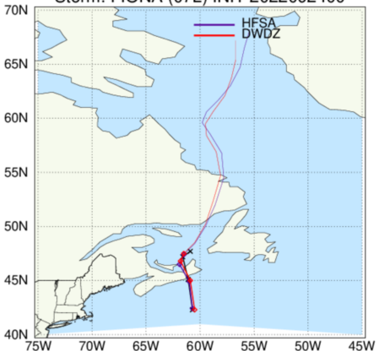
HAFS: TC Tracks Storm: FIONA (07L) INIT 2022092400
