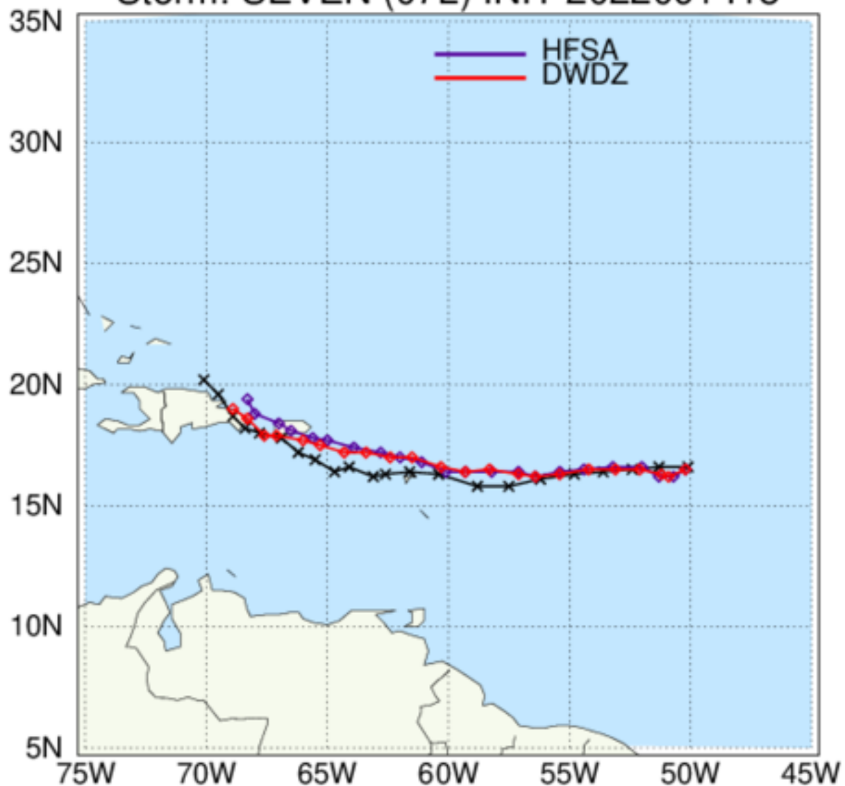
HAFS: TC Tracks Storm: SEVEN (07L) INIT 2022091418
