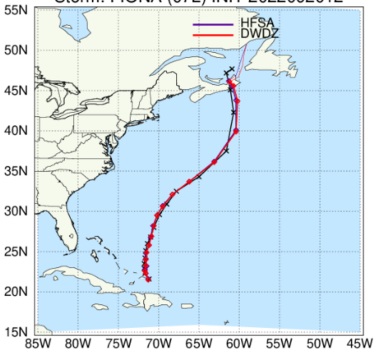
HAFS: TC Tracks Storm: FIONA (07L) INIT 2022092012
