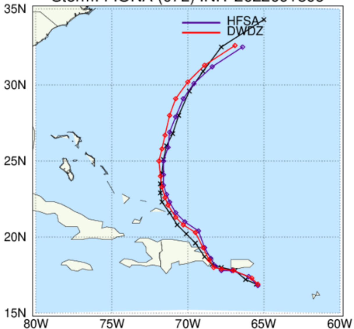
HAFS: TC Tracks Storm: FIONA (07L) INIT 2022091806
