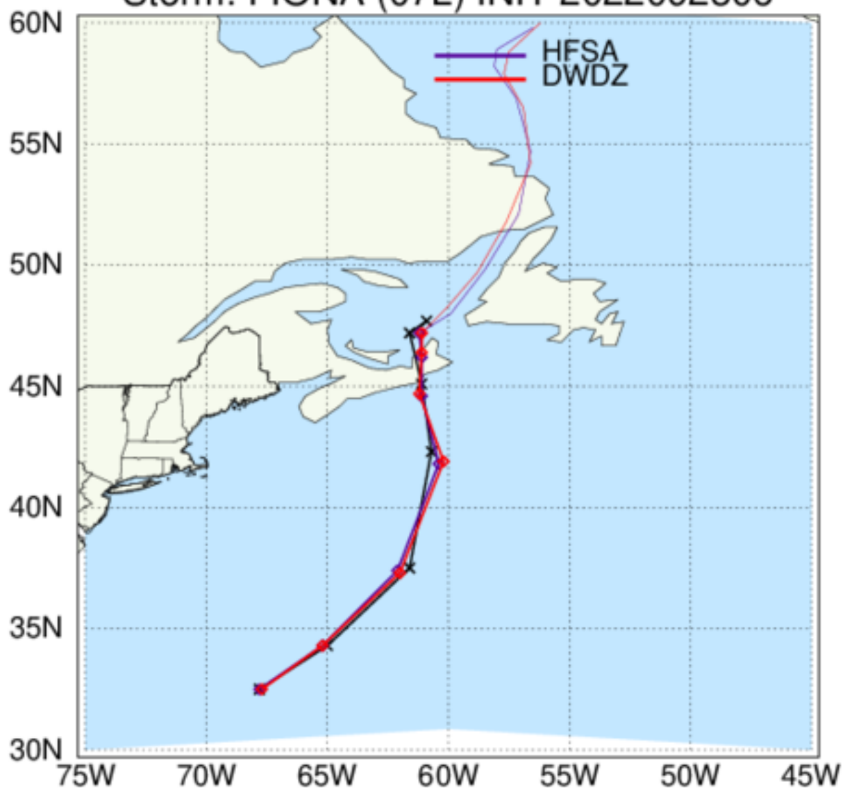
HAFS: TC Tracks Storm: FIONA (07L) INIT 2022092306
