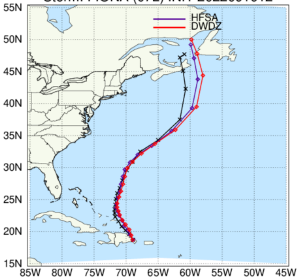
HAFS: TC Tracks Storm: FIONA (07L) INIT 2022091912
