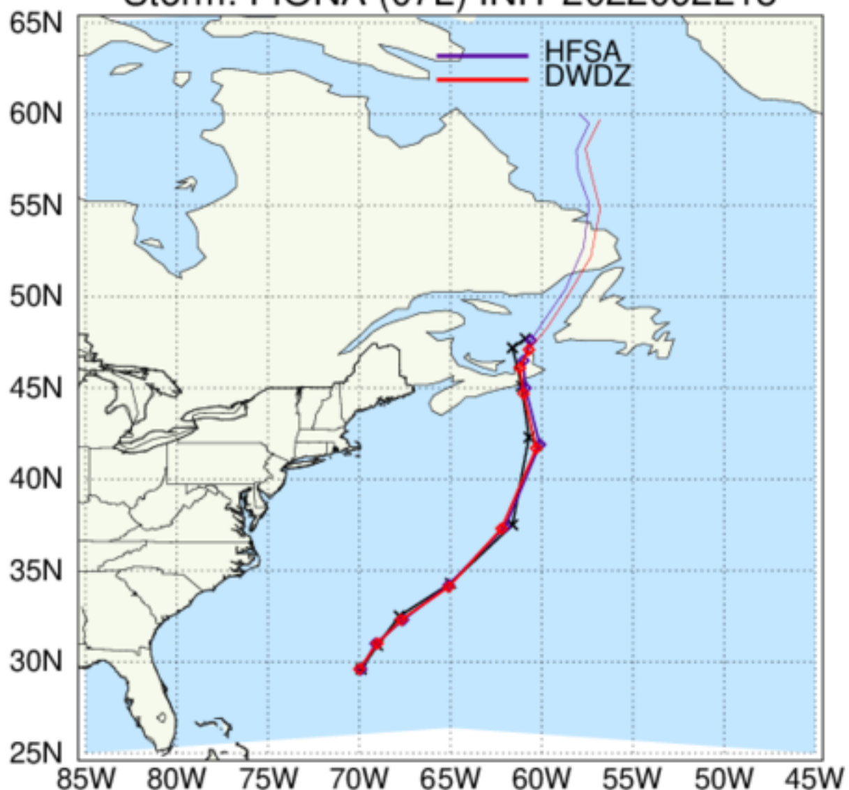
HAFS: TC Tracks Storm: FIONA (07L) INIT 2022092218
