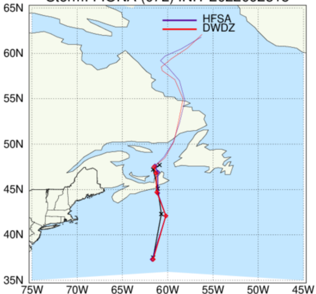
HAFS: TC Tracks Storm: FIONA (07L) INIT 2022092318
