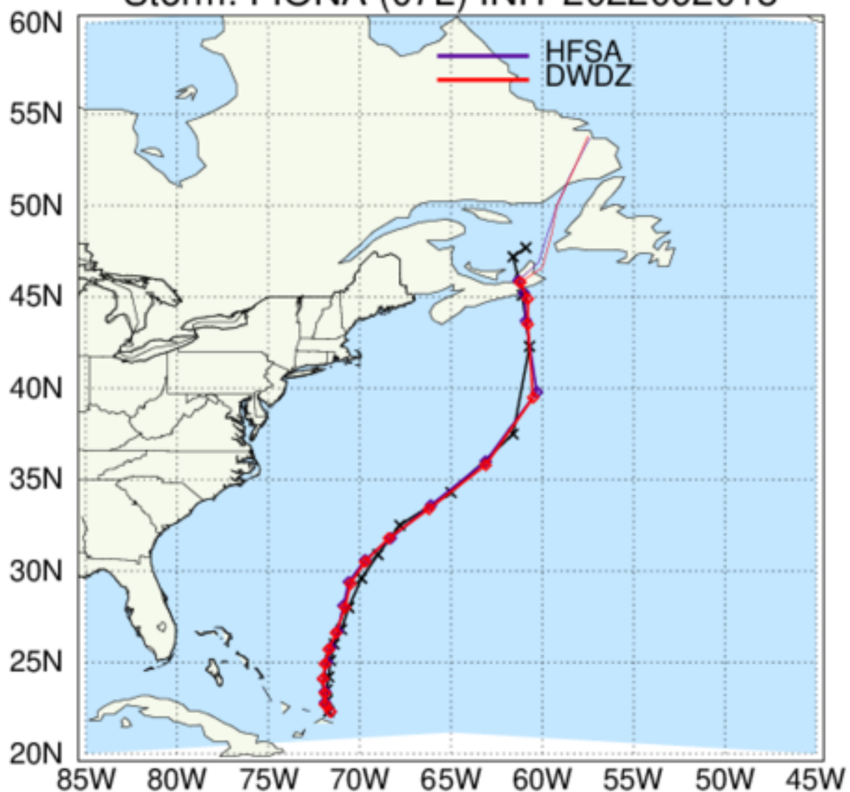
HAFS: TC Tracks Storm: FIONA (07L) INIT 2022092018
