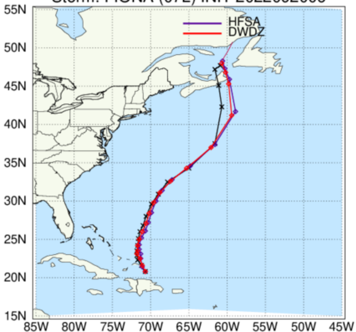
HAFS: TC Tracks Storm: FIONA (07L) INIT 2022092006
