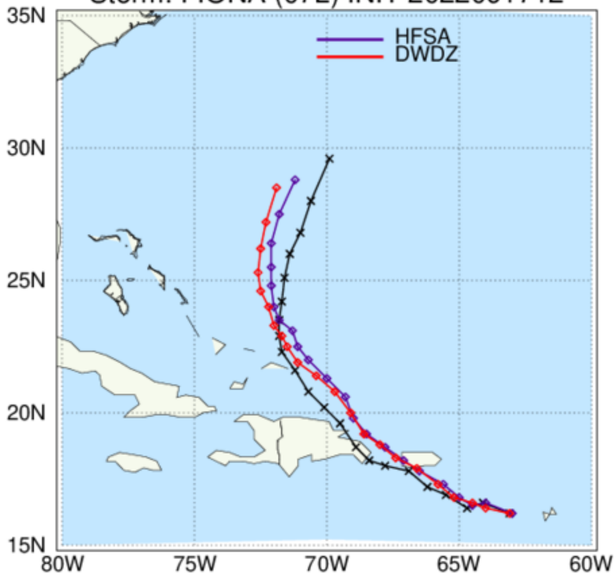
HAFS: TC Tracks Storm: FIONA (07L) INIT 2022091712
