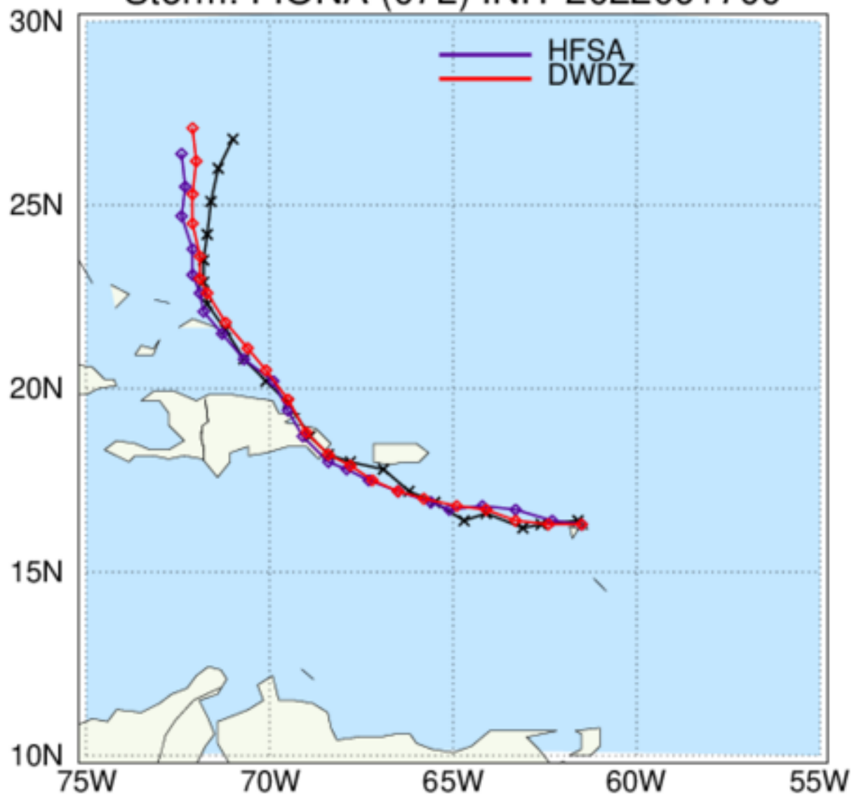
HAFS: TC Tracks Storm: FIONA (07L) INIT 2022091700
