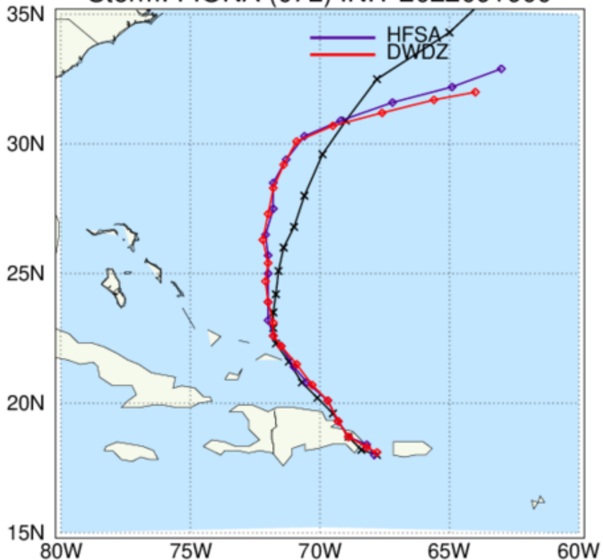
HAFS: TC Tracks Storm: FIONA (07L) INIT 2022091900
