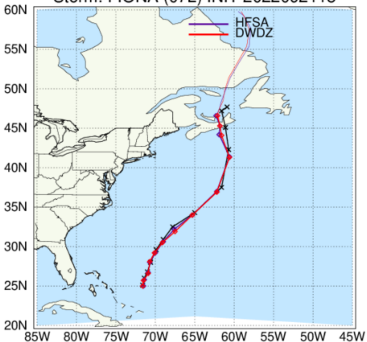
HAFS: TC Tracks Storm: FIONA (07L) INIT 2022092118
