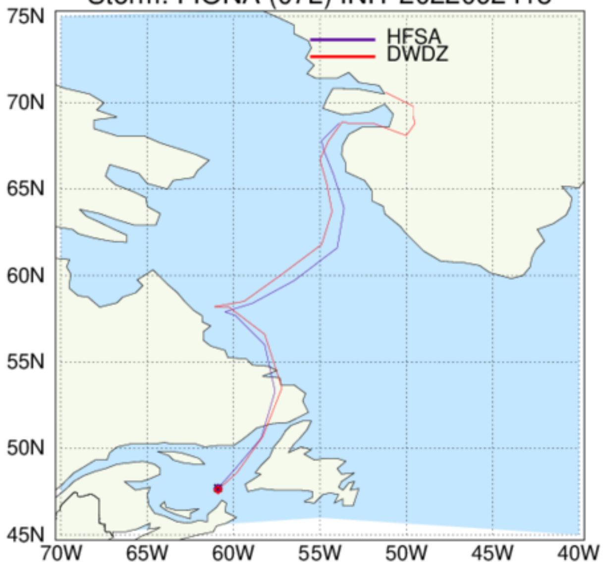
HAFS: TC Tracks Storm: FIONA (07L) INIT 2022092418
