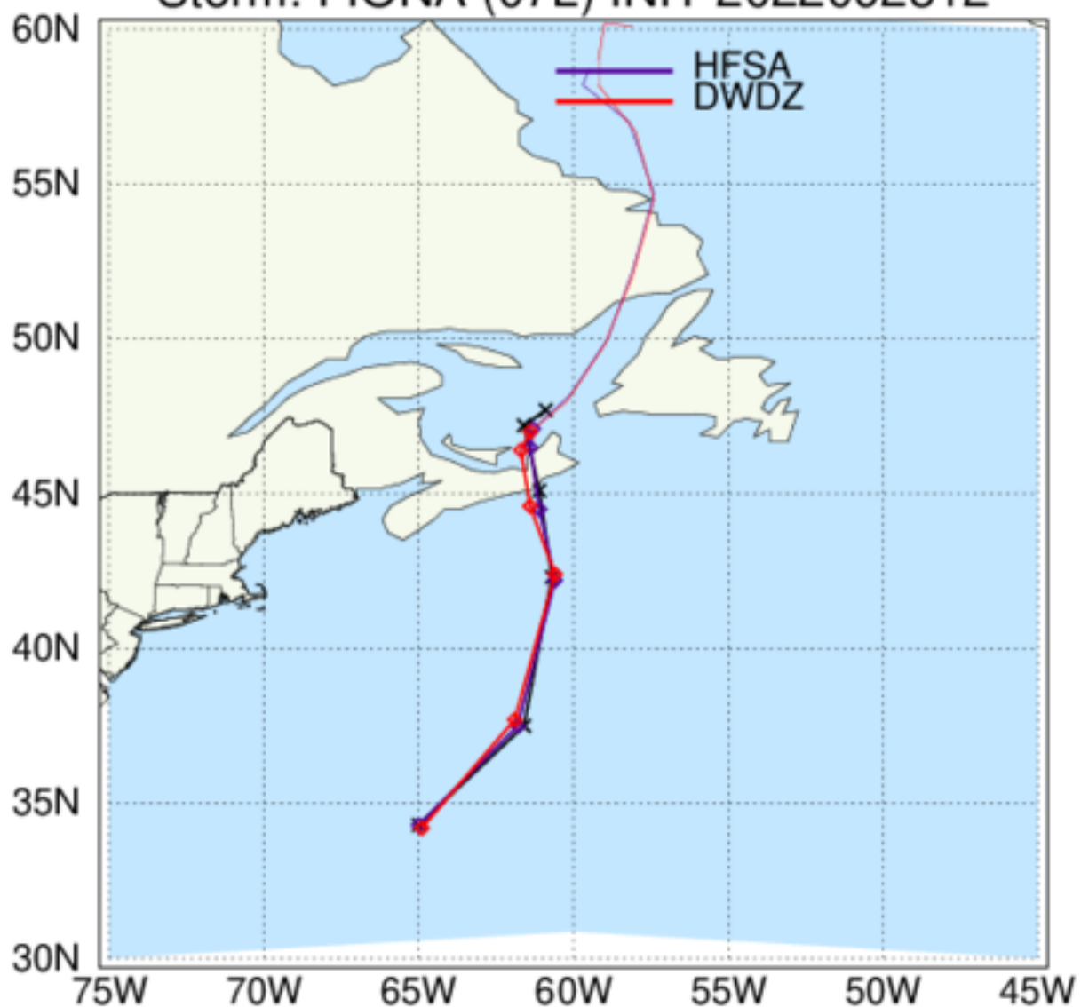
HAFS: TC Tracks Storm: FIONA (07L) INIT 2022092312
