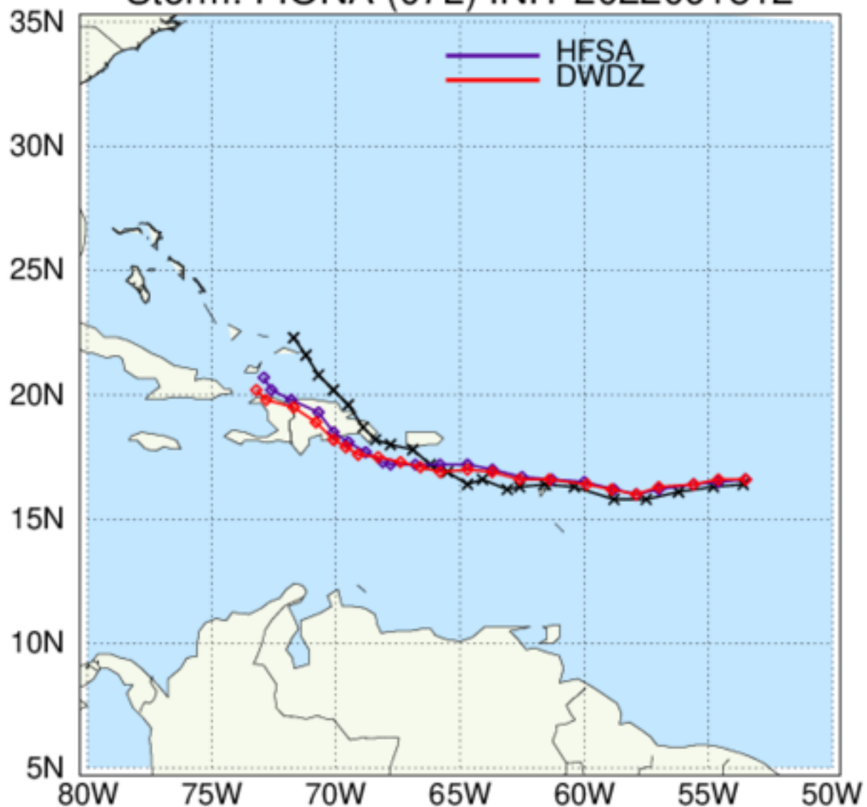
HAFS: TC Tracks Storm: FIONA (07L) INIT 2022091512
