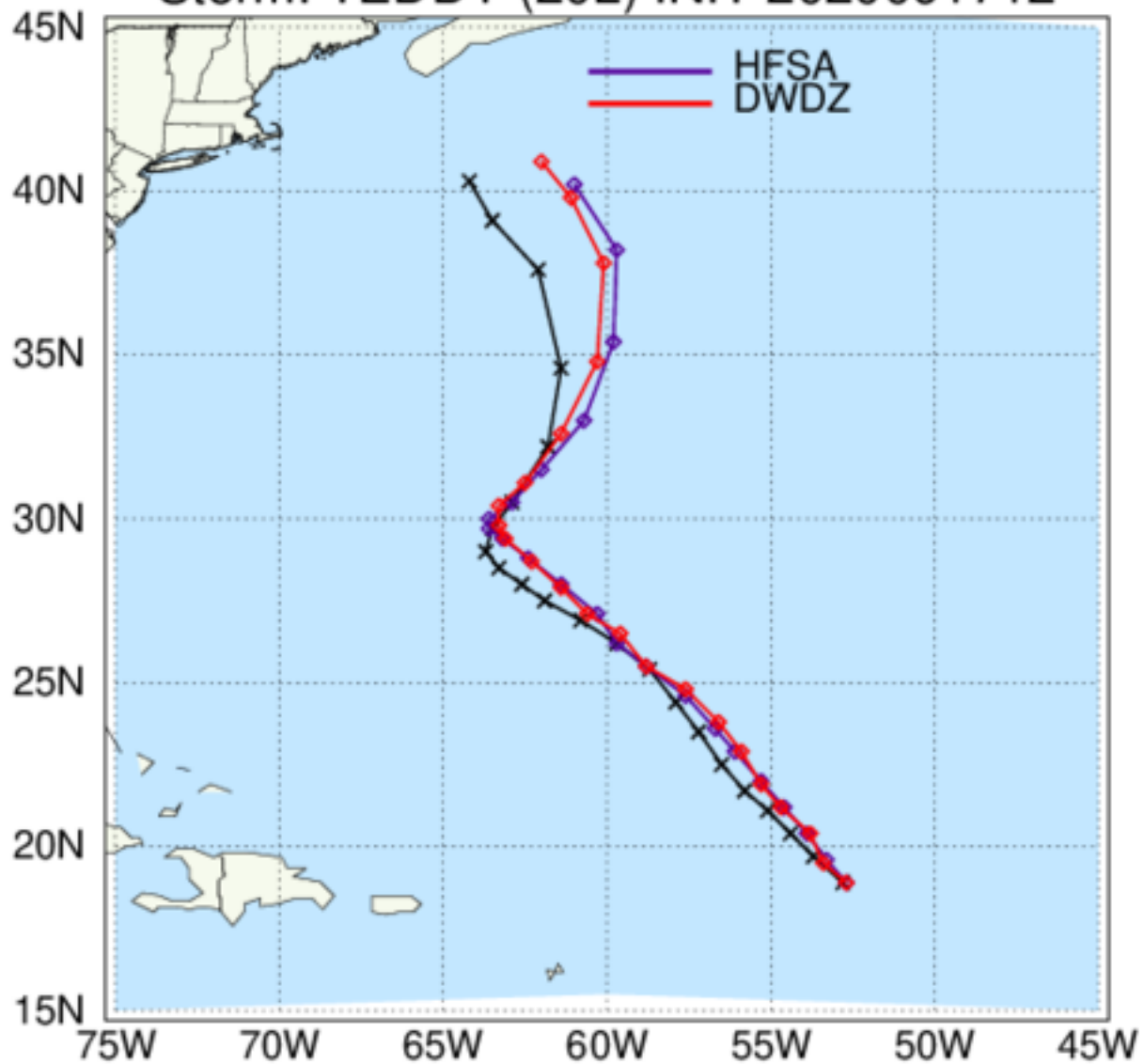
HAFS: TC Tracks Storm: TEDDY (20L) INIT 2020091712
