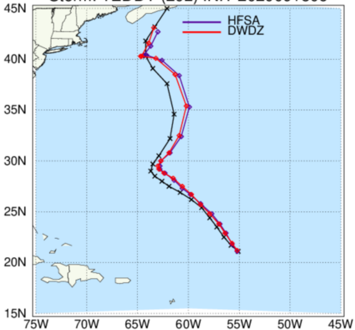
HAFS: TC Tracks Storm: TEDDY (20L) INIT 2020091806
