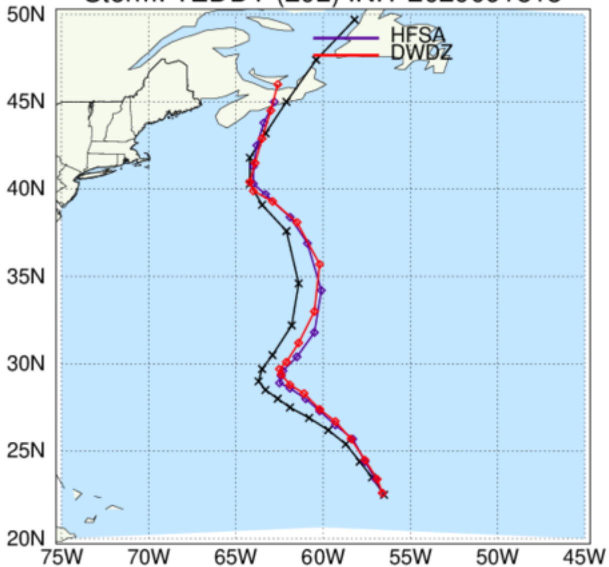
HAFS: TC Tracks Storm: TEDDY (20L) INIT 2020091818
