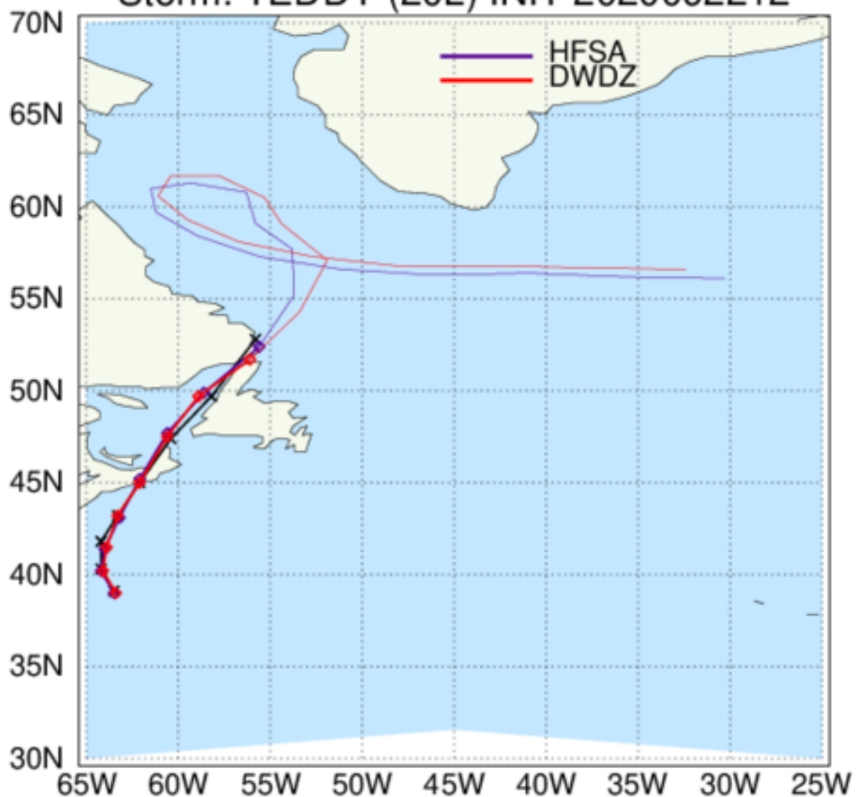
HAFS: TC Tracks Storm: TEDDY (20L) INIT 2020092212
