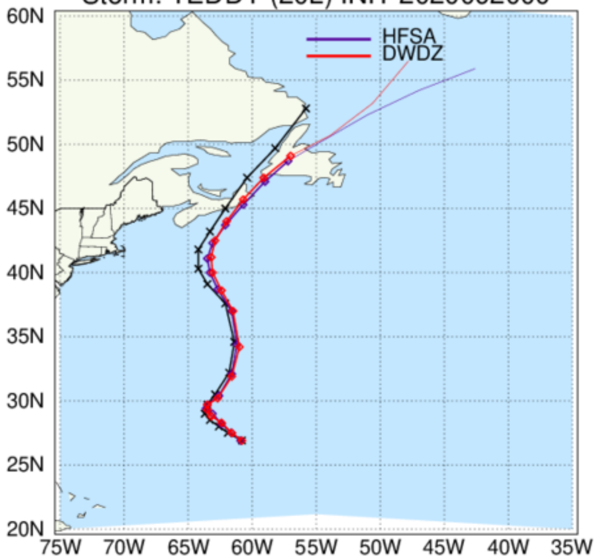
HAFS: TC Tracks Storm: TEDDY (20L) INIT 2020092000
