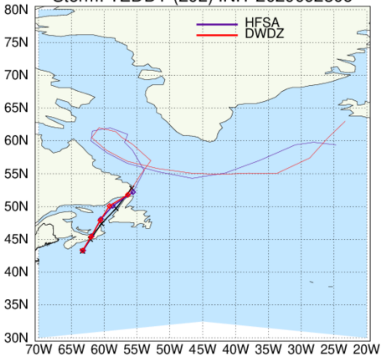
HAFS: TC Tracks Storm: TEDDY (20L) INIT 2020092306
