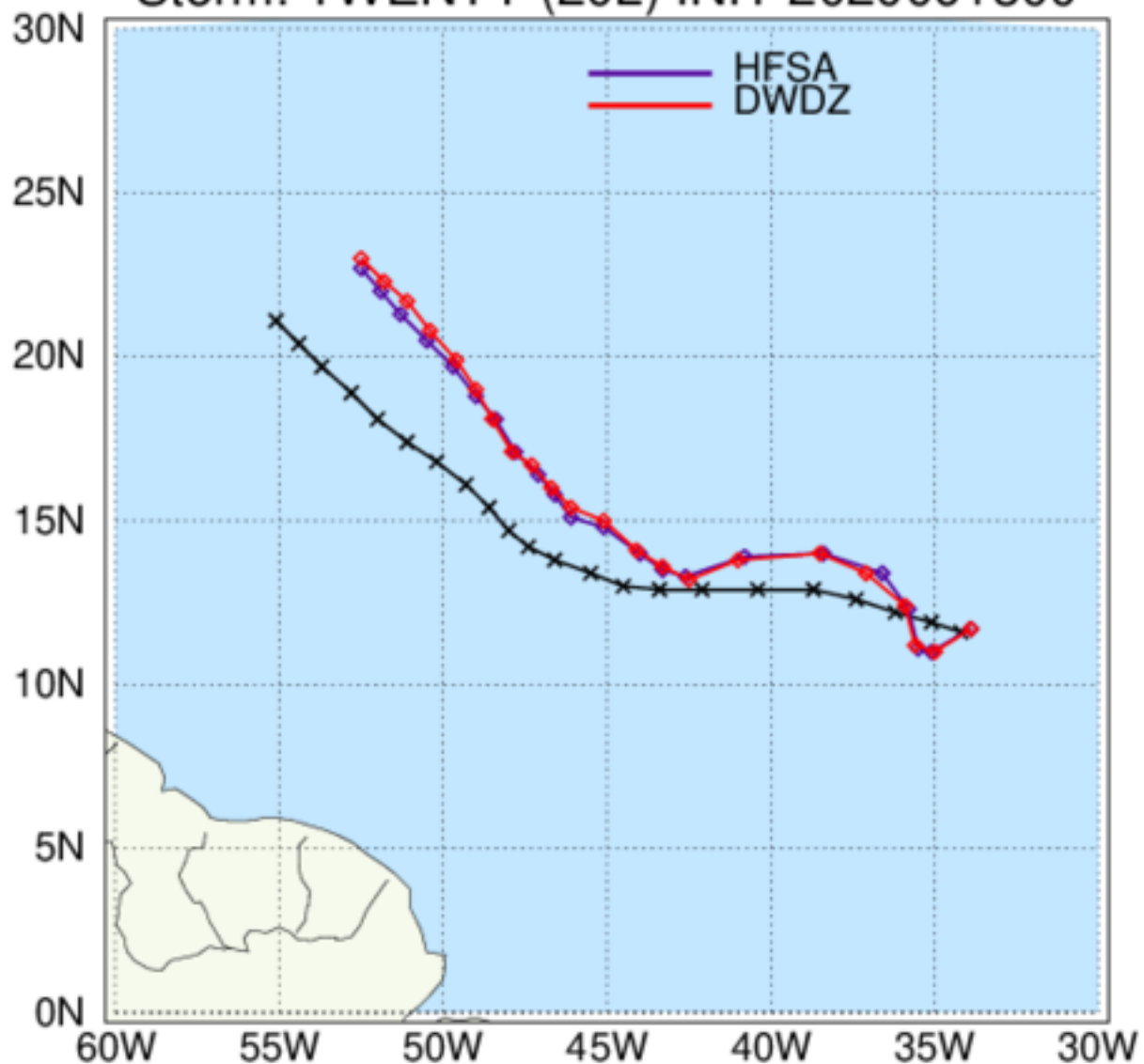
HAFS: TC Tracks Storm: TWENTY (20L) INIT 2020091300
