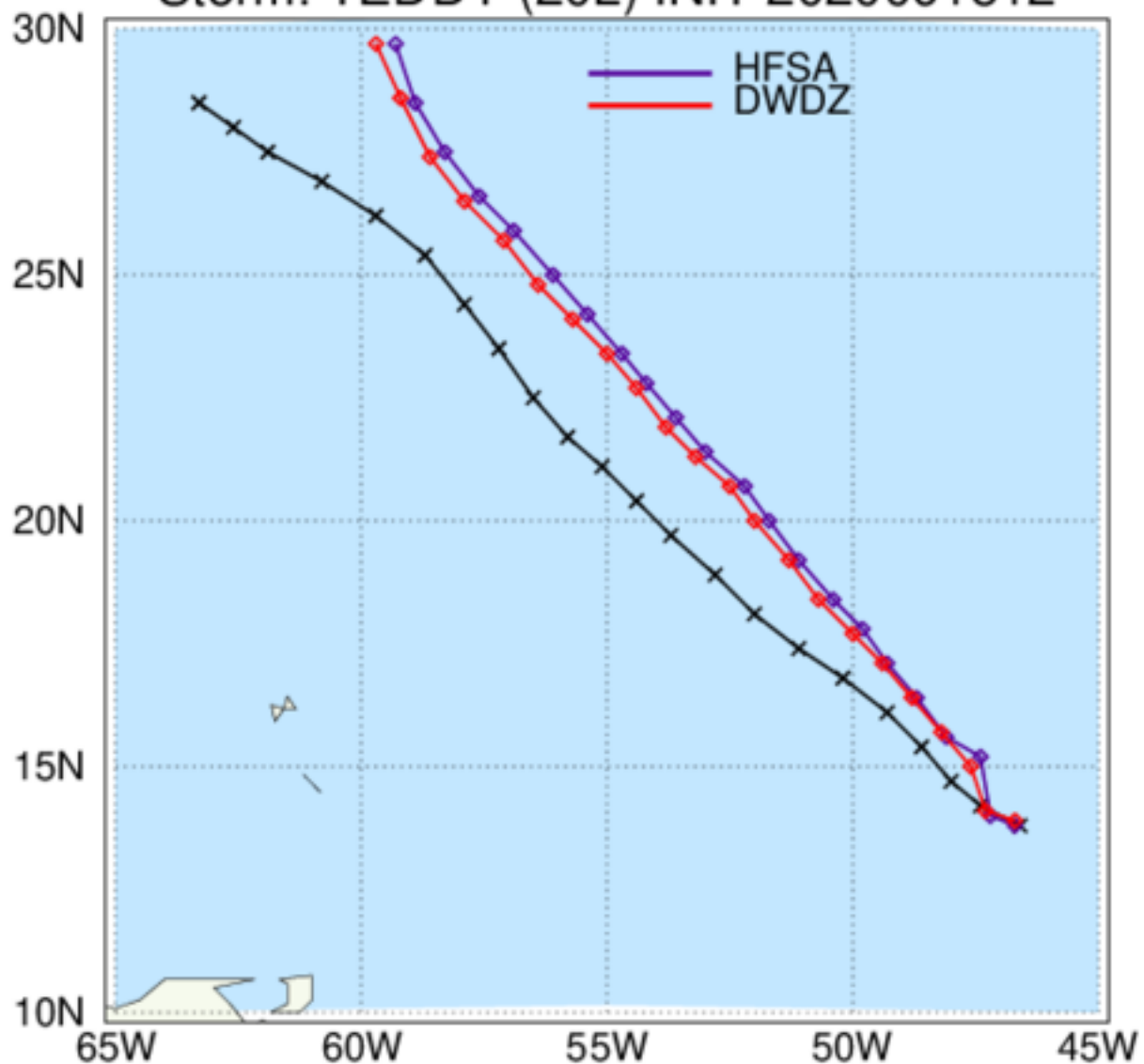
HAFS: TC Tracks Storm: TEDDY (20L) INIT 2020091512
