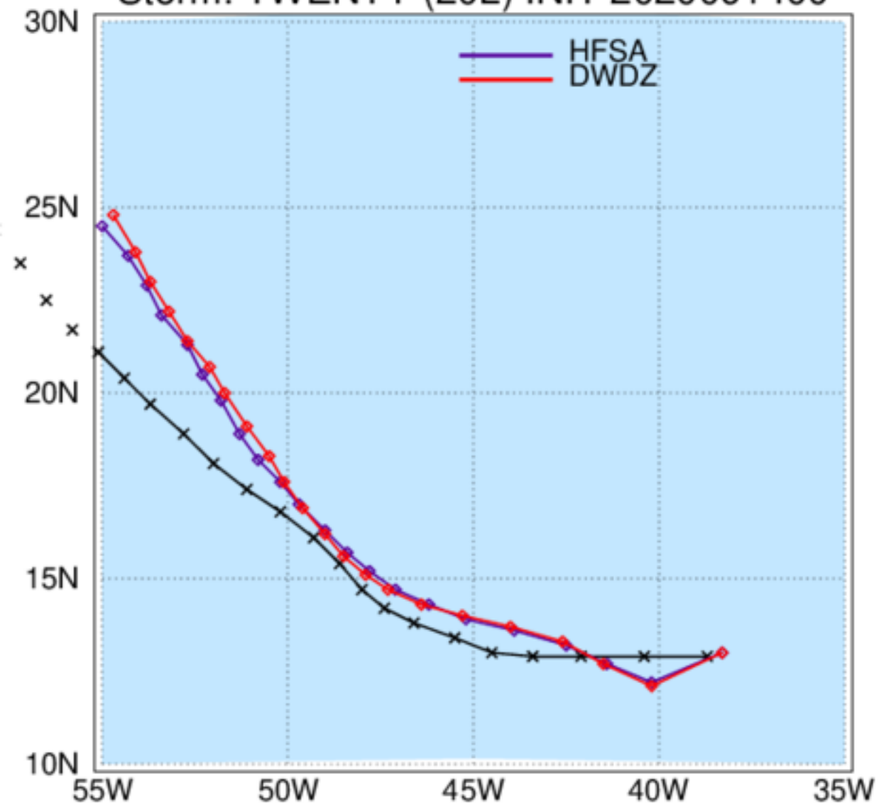
HAFS: TC Tracks Storm: TWENTY (20L) INIT 2020091400
