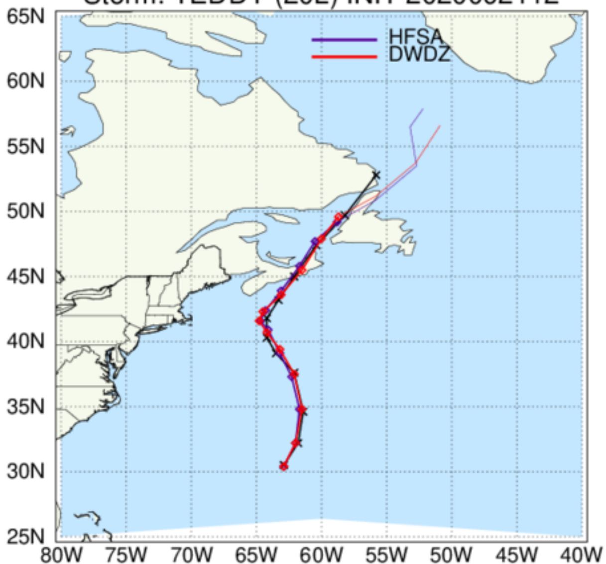
HAFS: TC Tracks Storm: TEDDY (20L) INIT 2020092112
