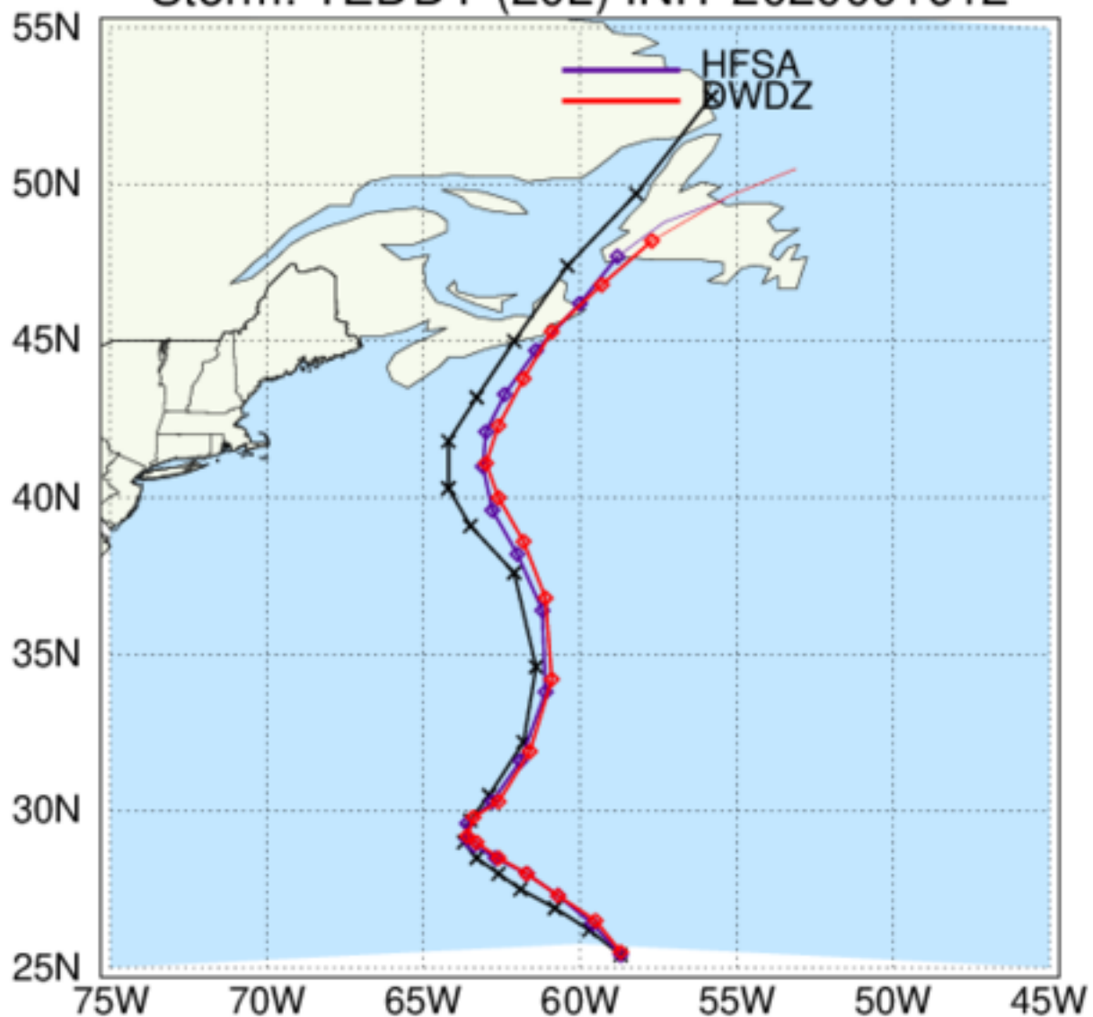
HAFS: TC Tracks Storm: TEDDY (20L) INIT 2020091912
