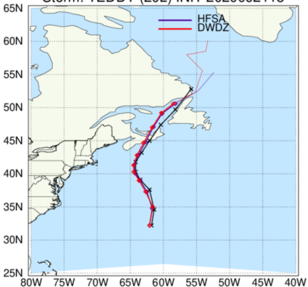
HAFS: TC Tracks Storm: TEDDY (20L) INIT 2020092118
