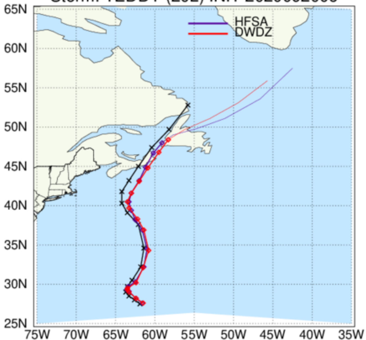
HAFS: TC Tracks Storm: TEDDY (20L) INIT 2020092006
