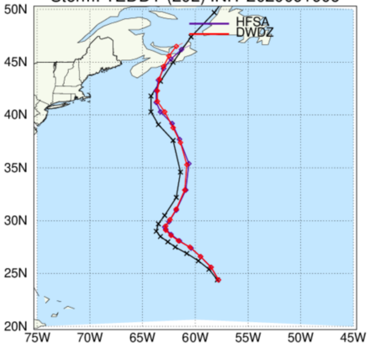
HAFS: TC Tracks Storm: TEDDY (20L) INIT 2020091906
