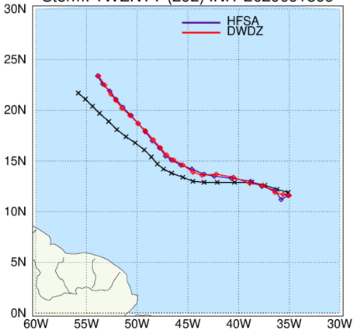
HAFS: TC Tracks Storm: TWENTY (20L) INIT 2020091306
