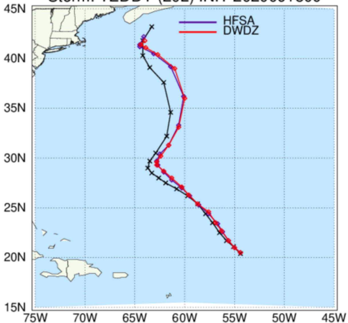
HAFS: TC Tracks Storm: TEDDY (20L) INIT 2020091800
