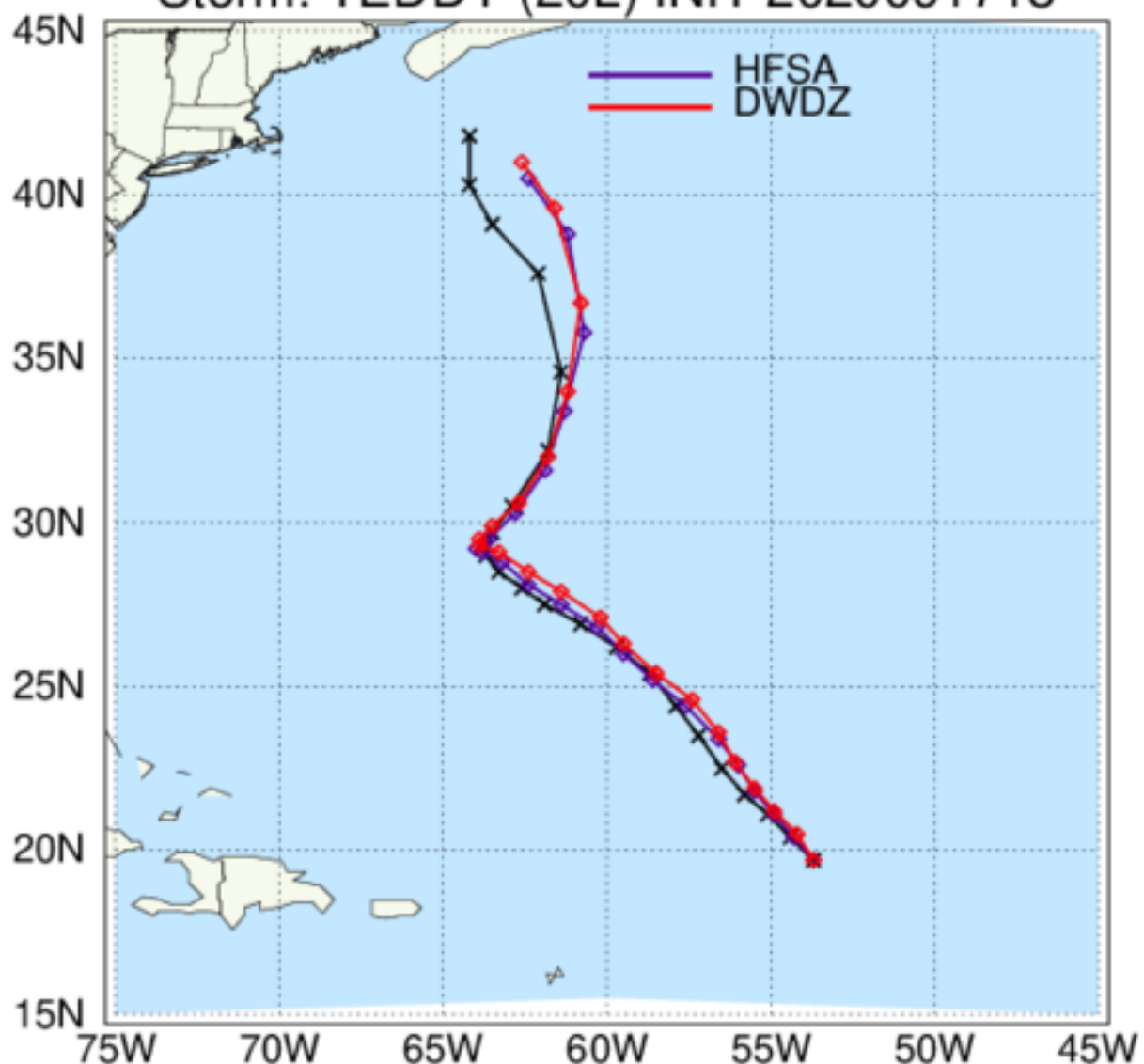
HAFS: TC Tracks Storm: TEDDY (20L) INIT 2020091718
