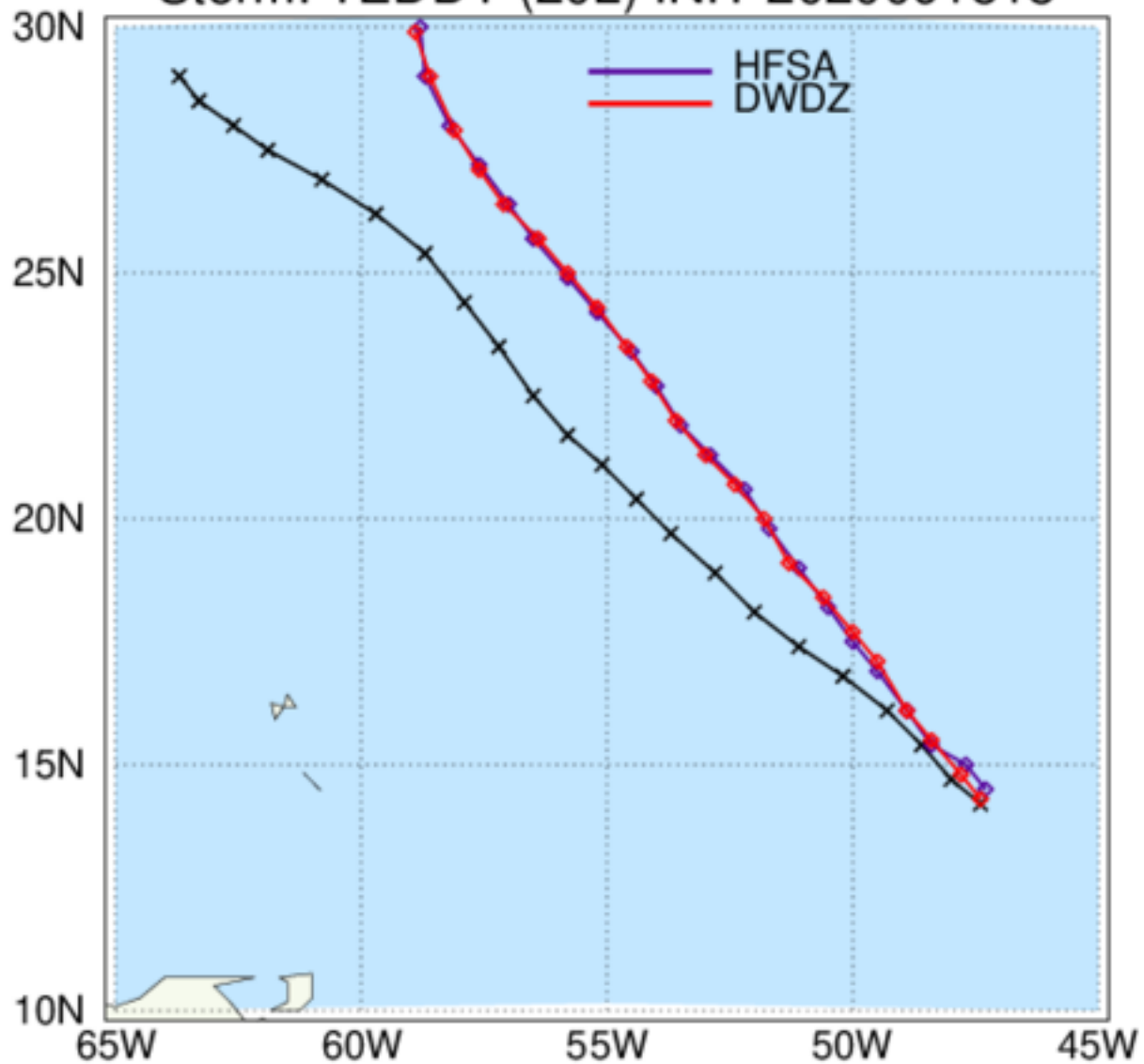
HAFS: TC Tracks Storm: TEDDY (20L) INIT 2020091518
