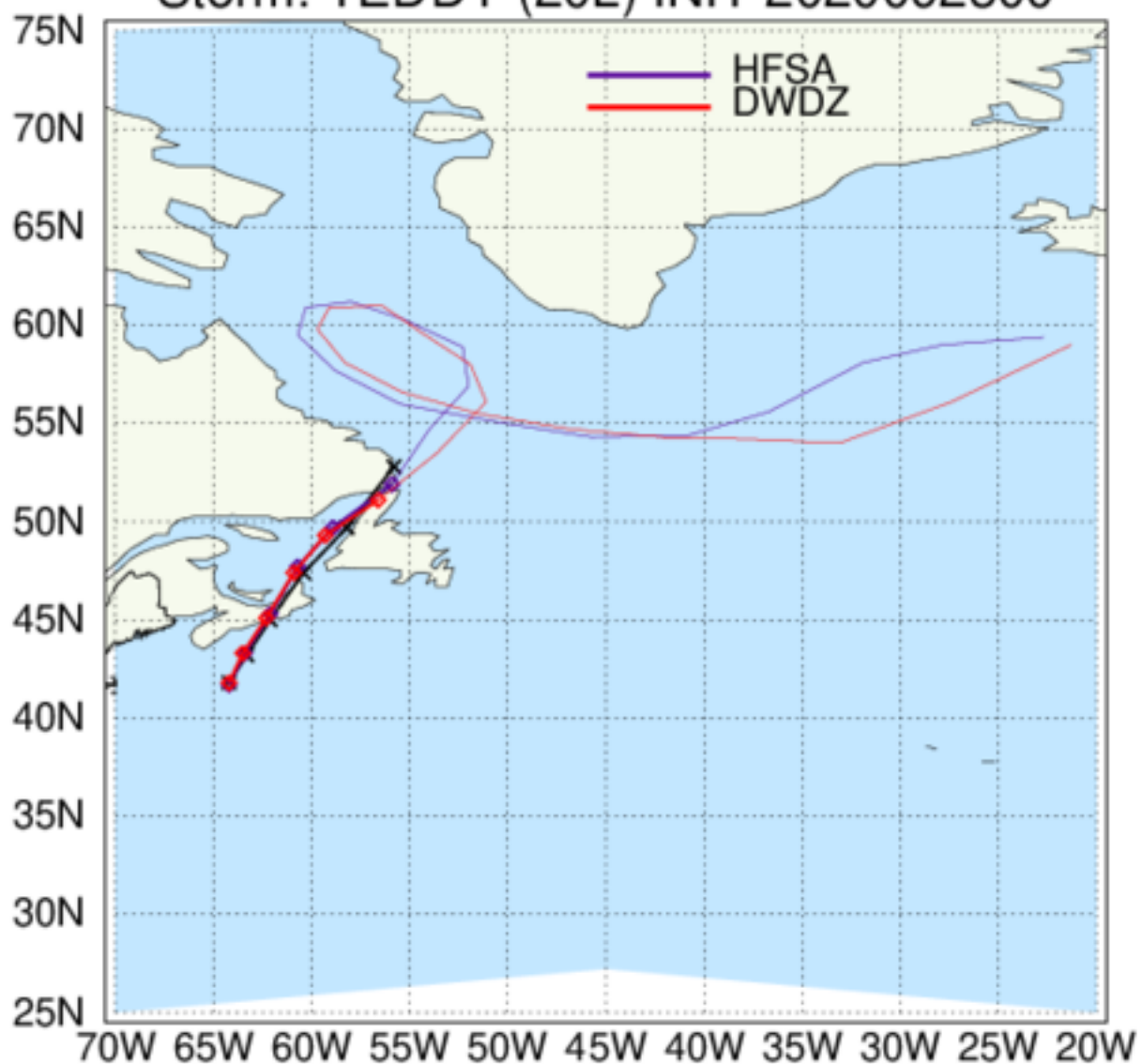
HAFS: TC Tracks Storm: TEDDY (20L) INIT 2020092300
