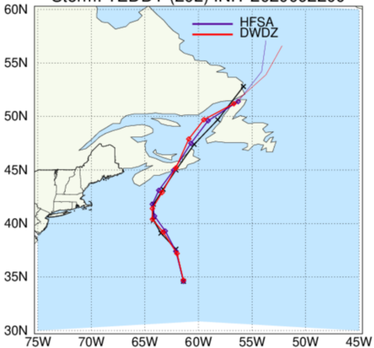
HAFS: TC Tracks Storm: TEDDY (20L) INIT 2020092200
