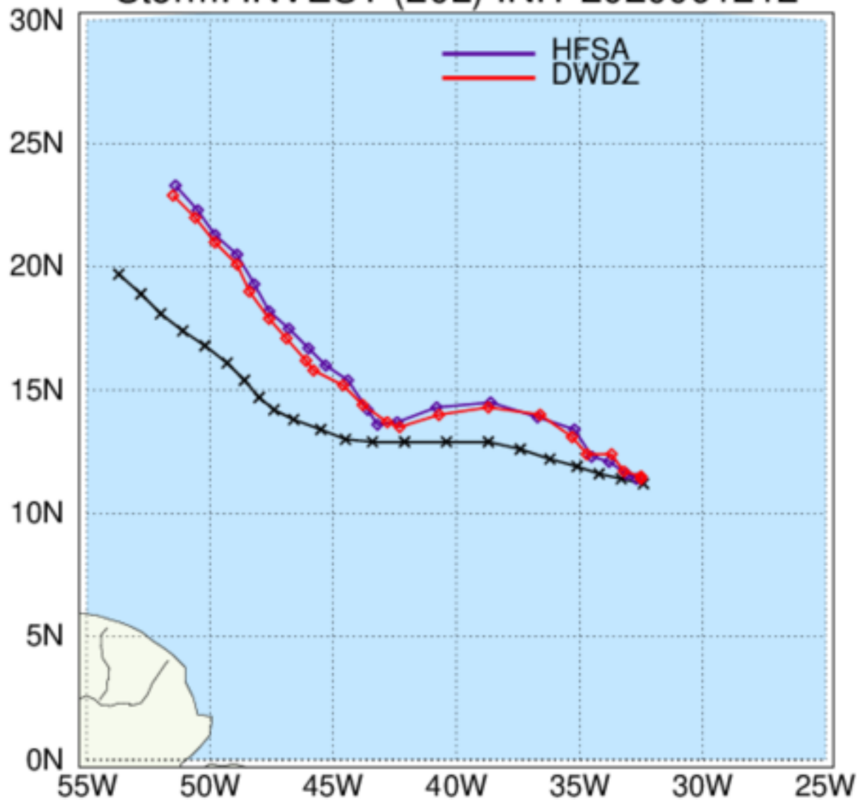
HAFS: TC Tracks Storm: INVEST (20L) INIT 2020091212
