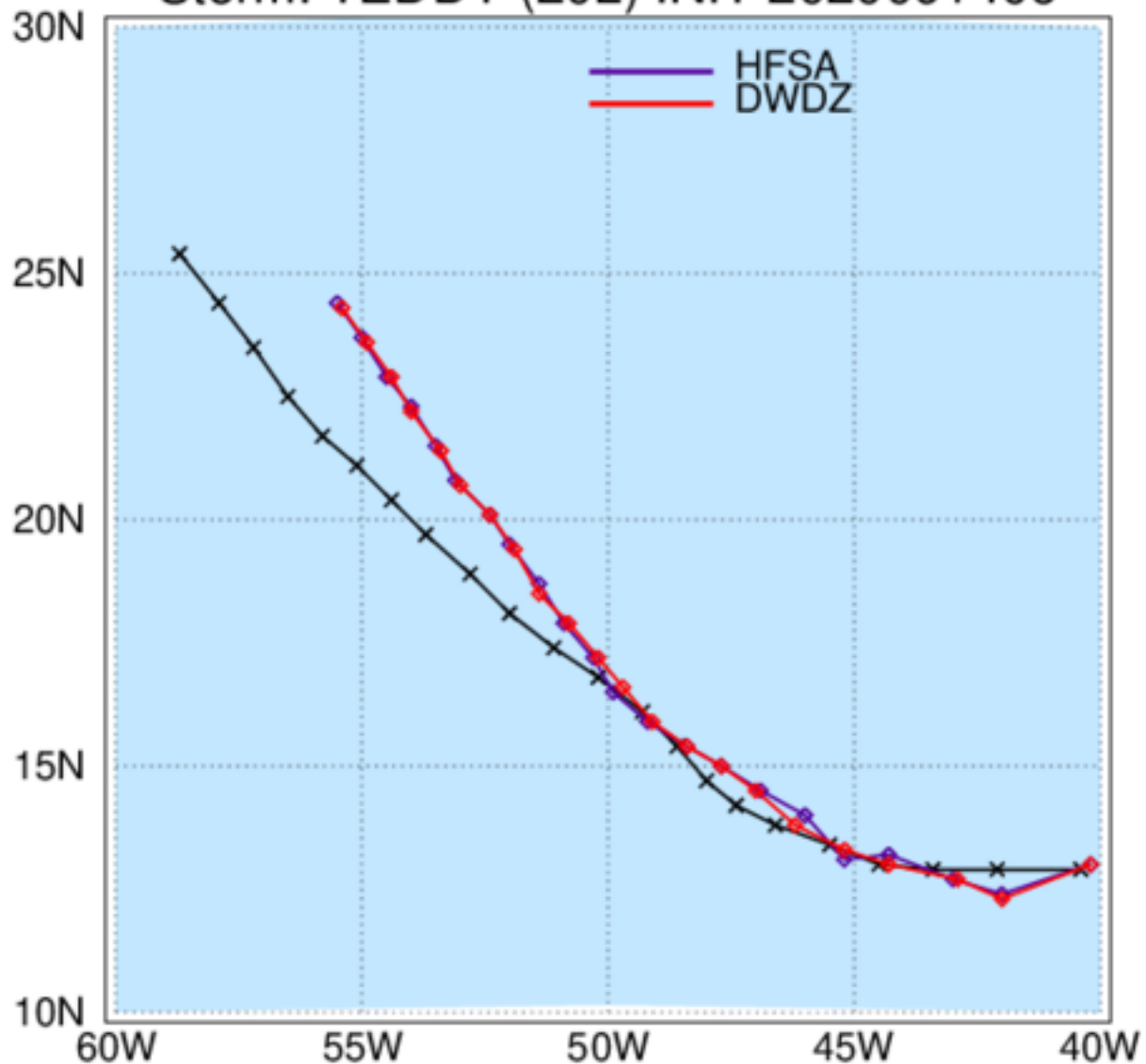
HAFS: TC Tracks Storm: TEDDY (20L) INIT 2020091406
