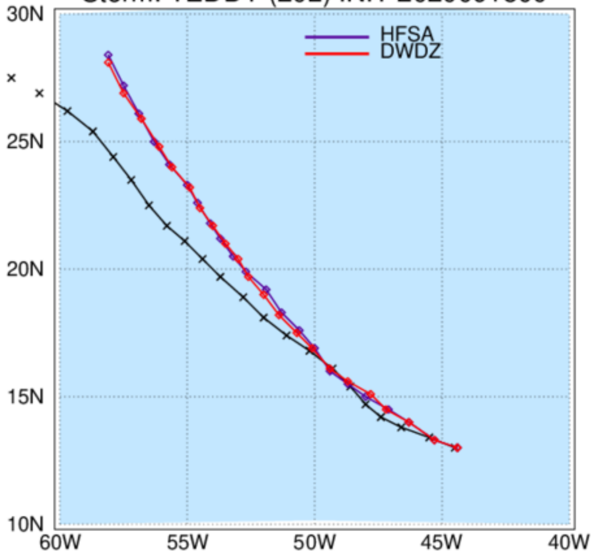
HAFS: TC Tracks Storm: TEDDY (20L) INIT 2020091500
