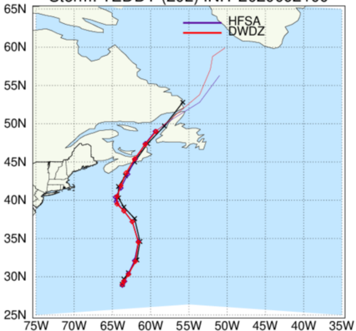
HAFS: TC Tracks Storm: TEDDY (20L) INIT 2020092100
