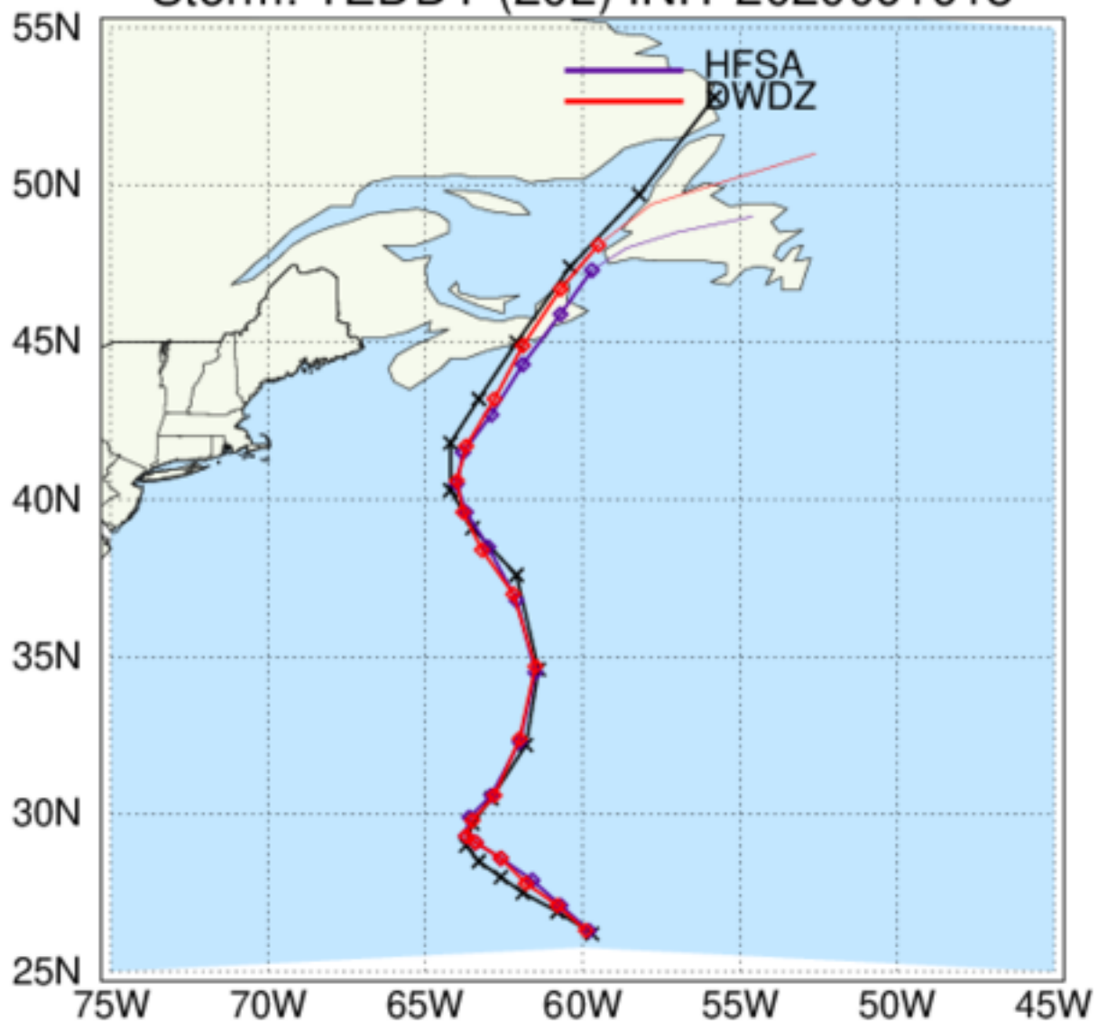
HAFS: TC Tracks Storm: TEDDY (20L) INIT 2020091918
