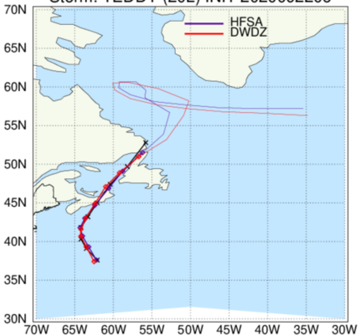
HAFS: TC Tracks Storm: TEDDY (20L) INIT 2020092206
