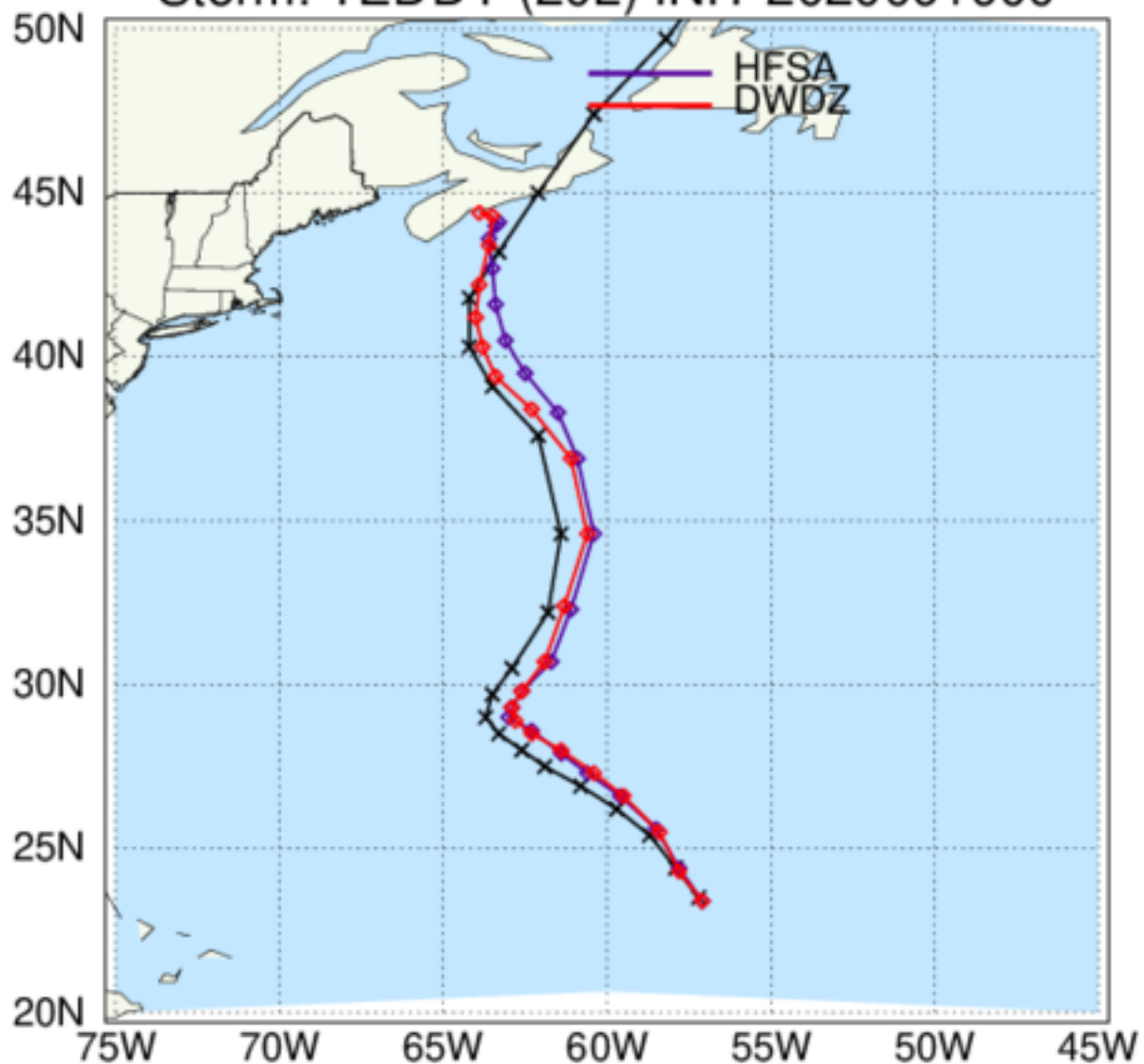
HAFS: TC Tracks Storm: TEDDY (20L) INIT 2020091900
