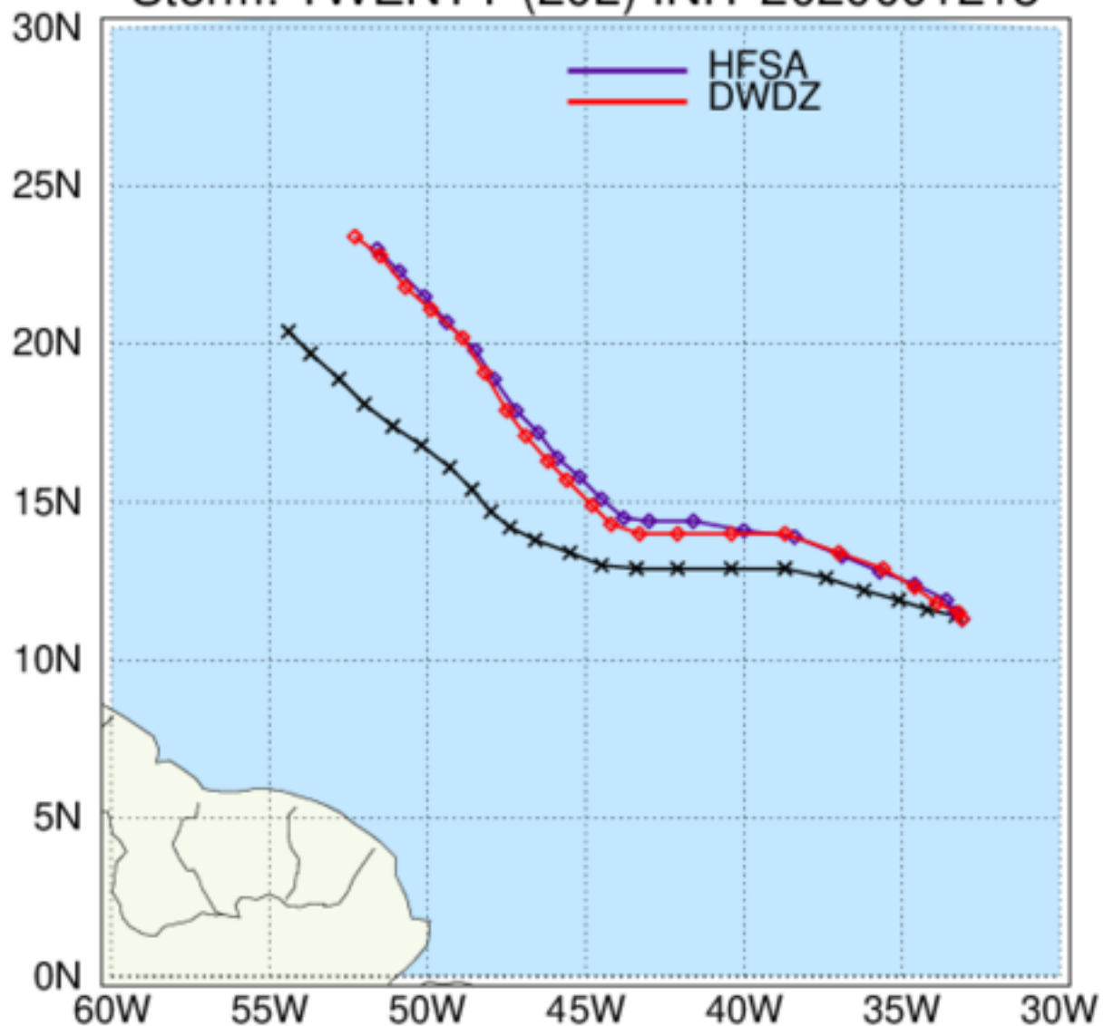
HAFS: TC Tracks Storm: TWENTY (20L) INIT 2020091218
