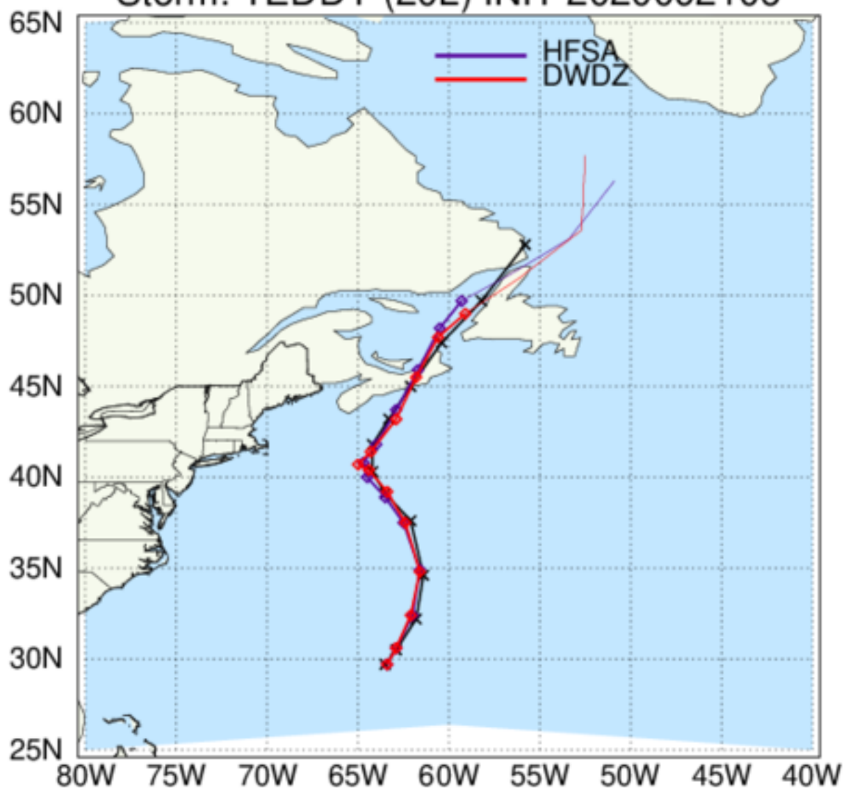
HAFS: TC Tracks Storm: TEDDY (20L) INIT 2020092106
