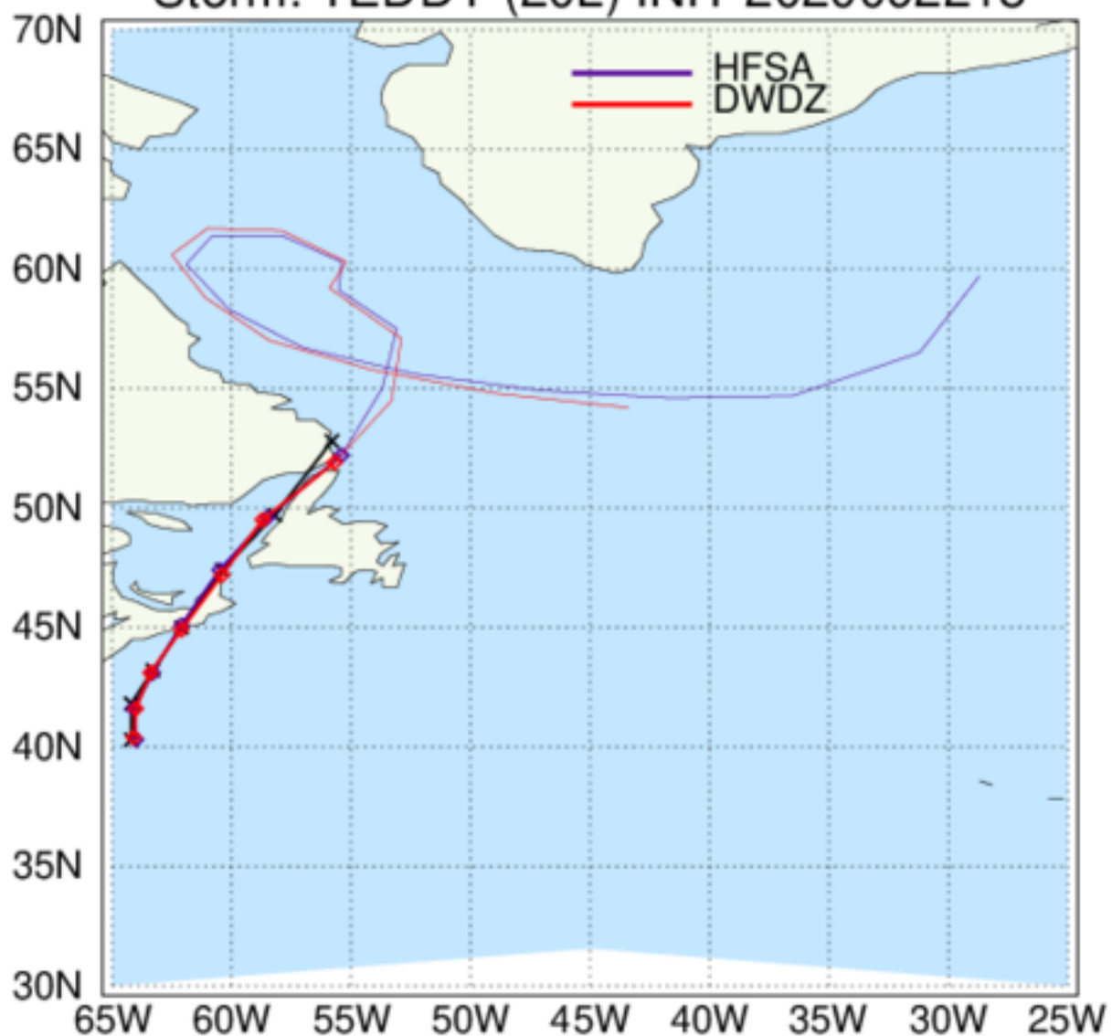
HAFS: TC Tracks Storm: TEDDY (20L) INIT 2020092218
