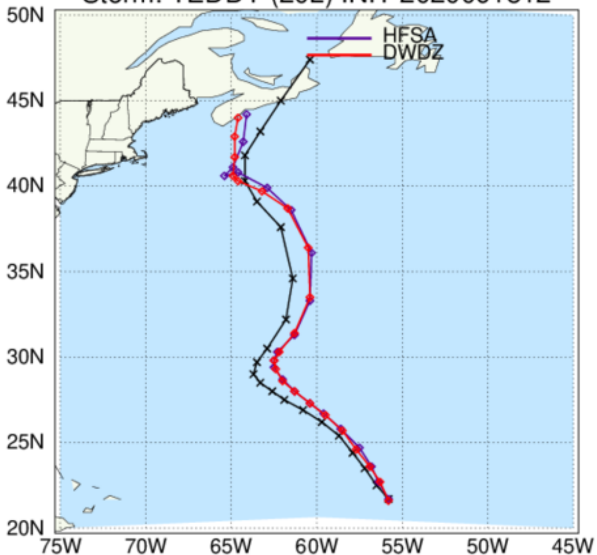
HAFS: TC Tracks Storm: TEDDY (20L) INIT 2020091812
