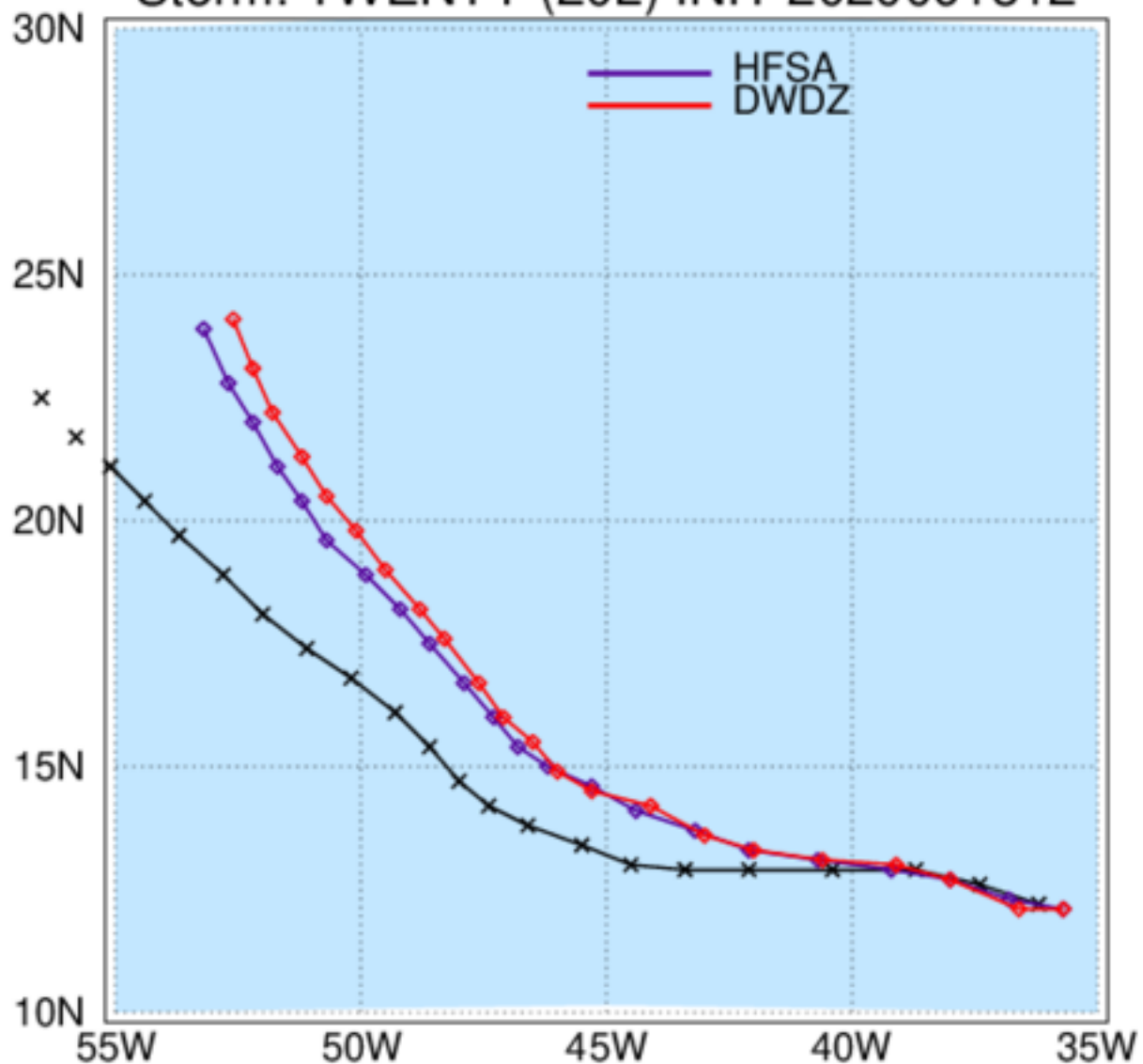
HAFS: TC Tracks Storm: TWENTY (20L) INIT 2020091312
