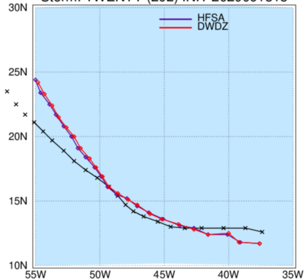
HAFS: TC Tracks Storm: TWENTY (20L) INIT 2020091318
