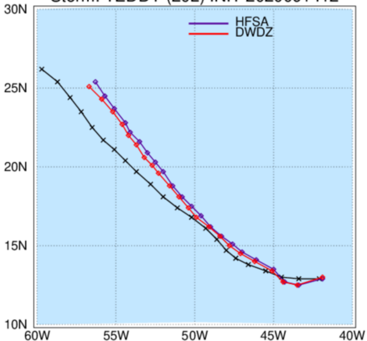
HAFS: TC Tracks Storm: TEDDY (20L) INIT 2020091412
