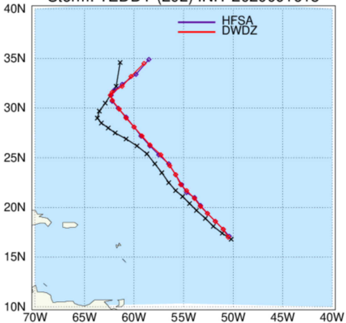
HAFS: TC Tracks Storm: TEDDY (20L) INIT 2020091618
