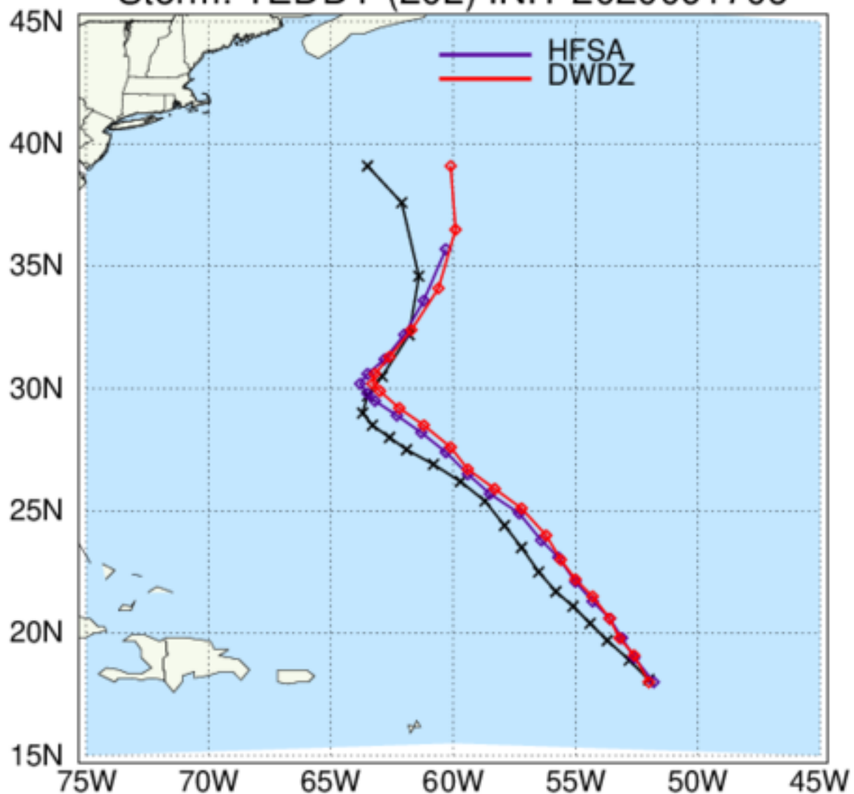
HAFS: TC Tracks Storm: TEDDY (20L) INIT 2020091706
