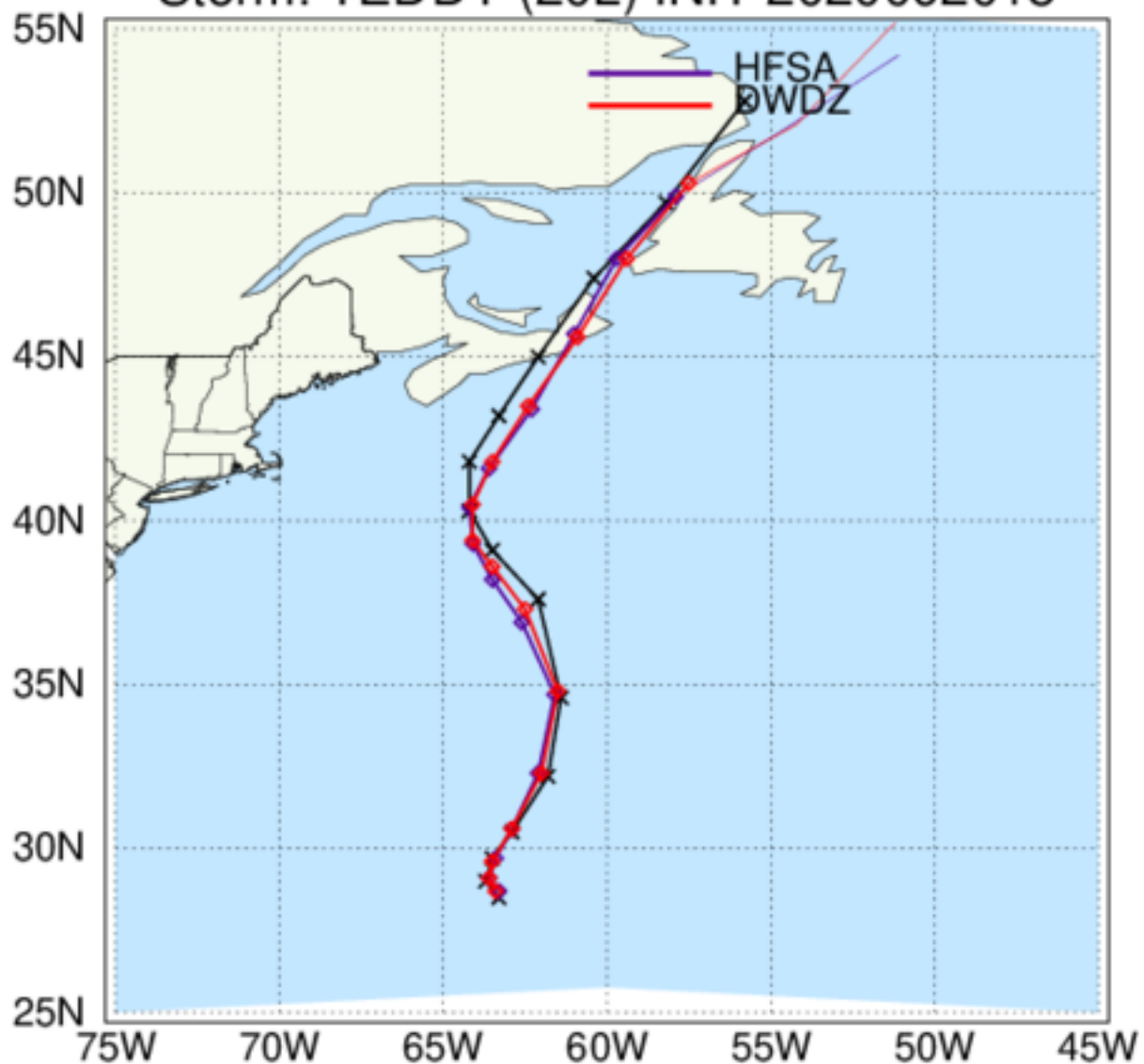
HAFS: TC Tracks Storm: TEDDY (20L) INIT 2020092018
