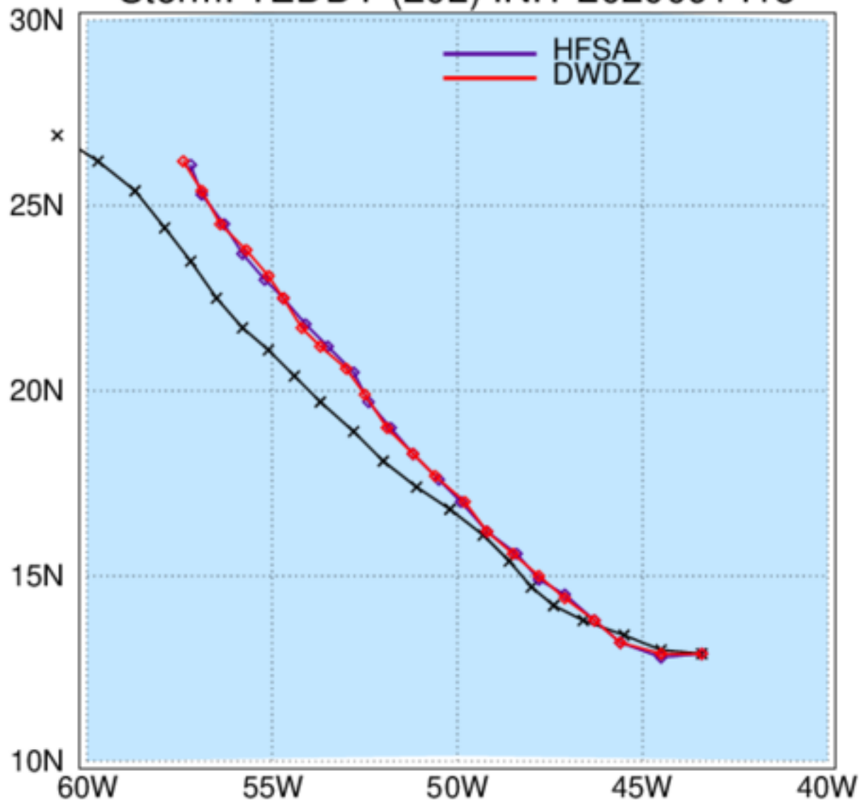
HAFS: TC Tracks Storm: TEDDY (20L) INIT 2020091418
