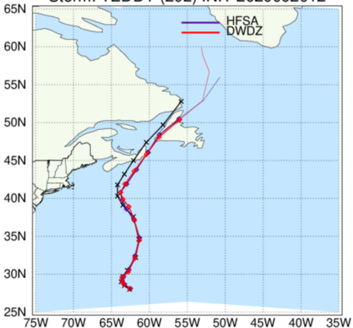
HAFS: TC Tracks Storm: TEDDY (20L) INIT 2020092012
